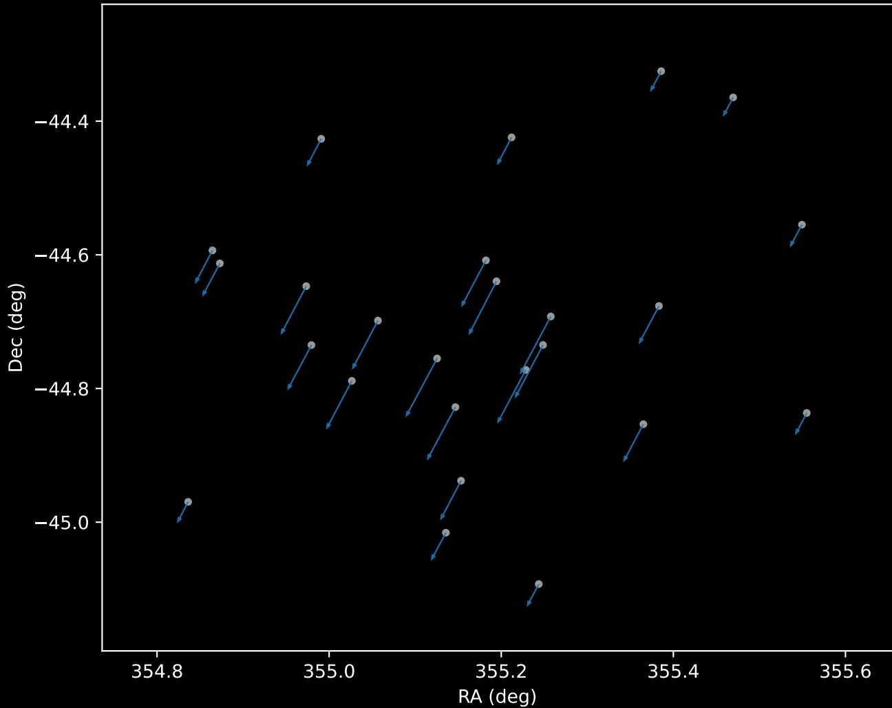
Gaia DR3 Cluster 120 Proper Motion Vectors (n=25)
