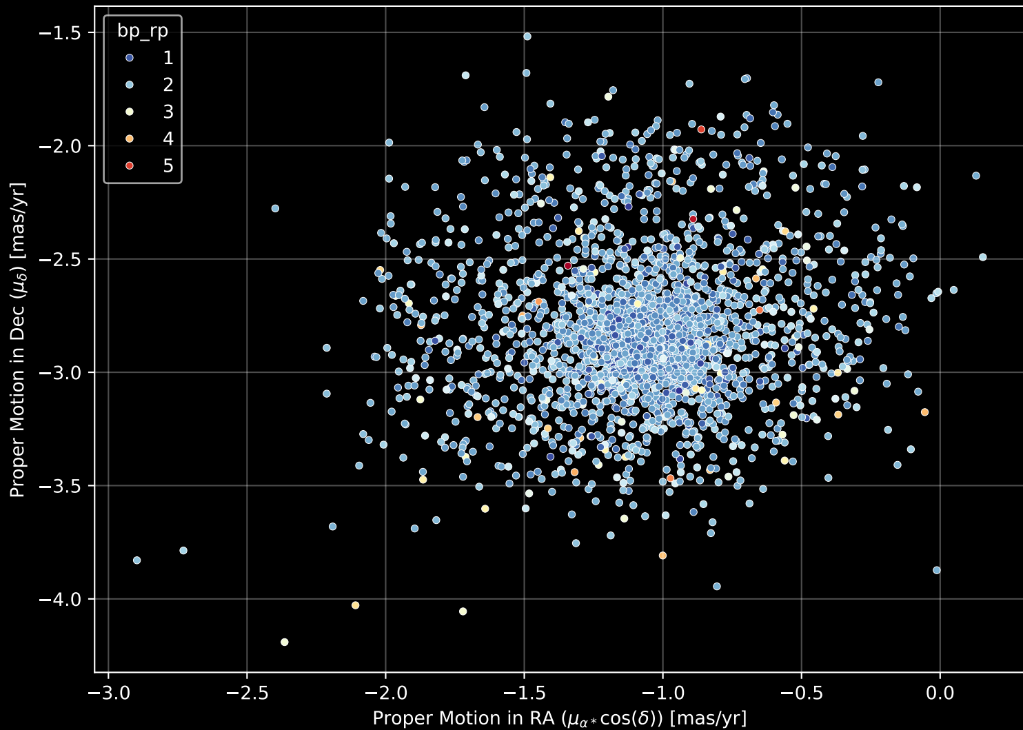
Gaia Cluster: [NGC_6259] Proper Motion Diagram (n= 2578)
