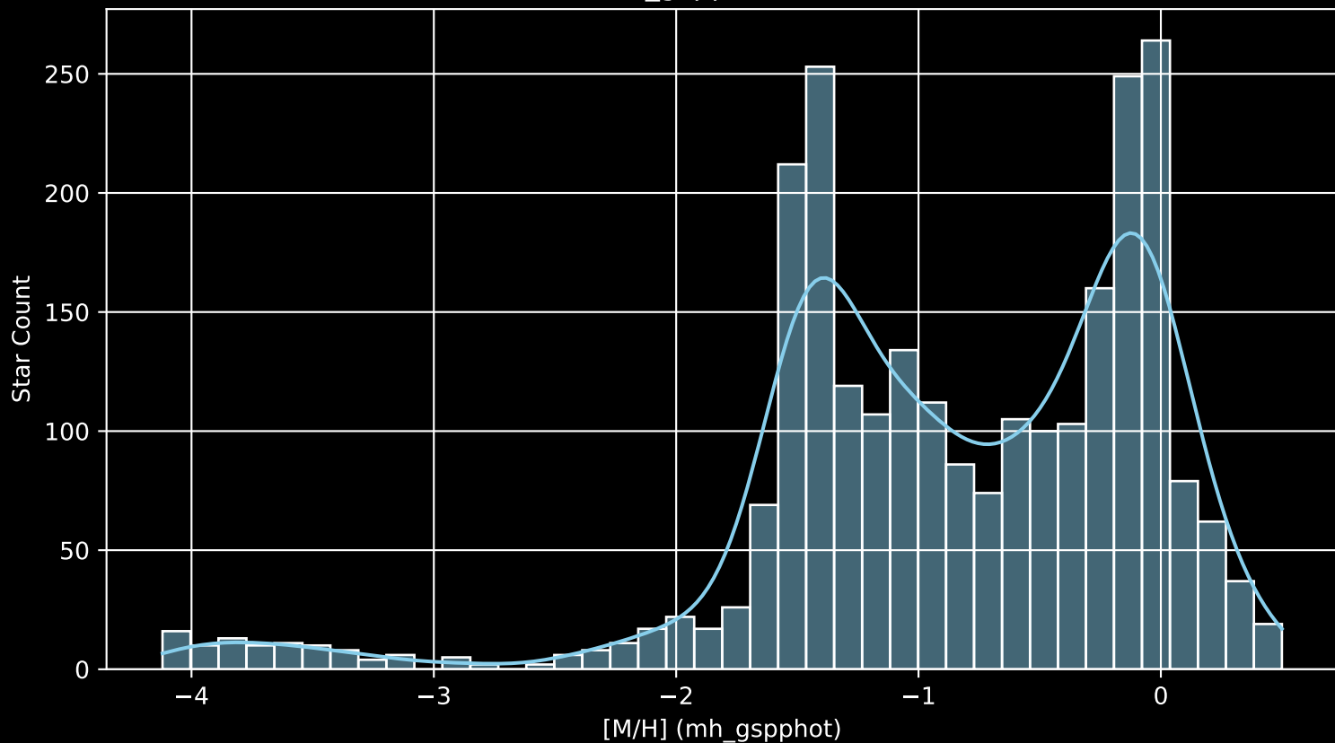
Gaia Cluster: [NGC_6259 [M/H] (mh_gspphot) (n= 2548)
