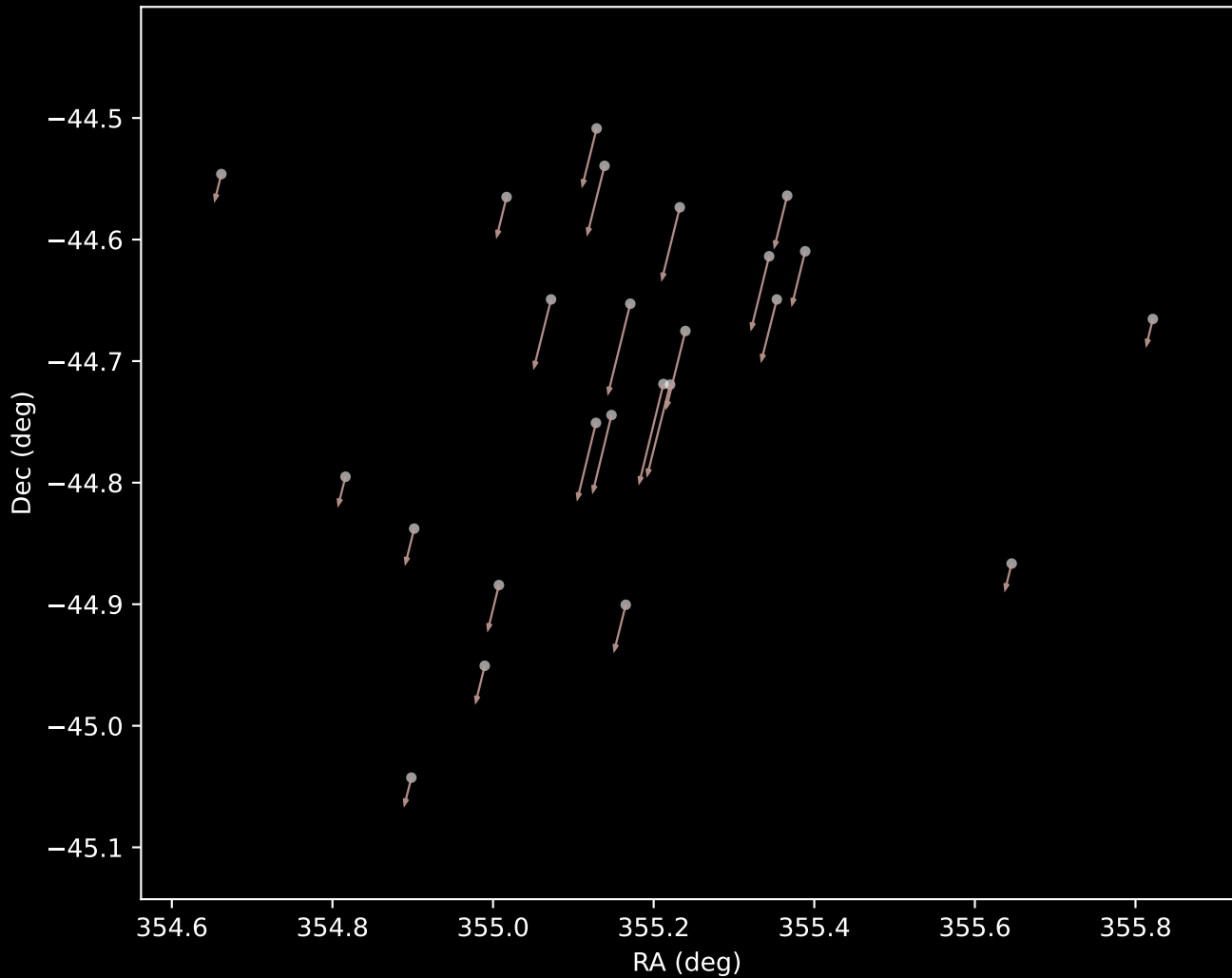
Gaia DR3 Cluster 131 Proper Motion Vectors (n=24)
