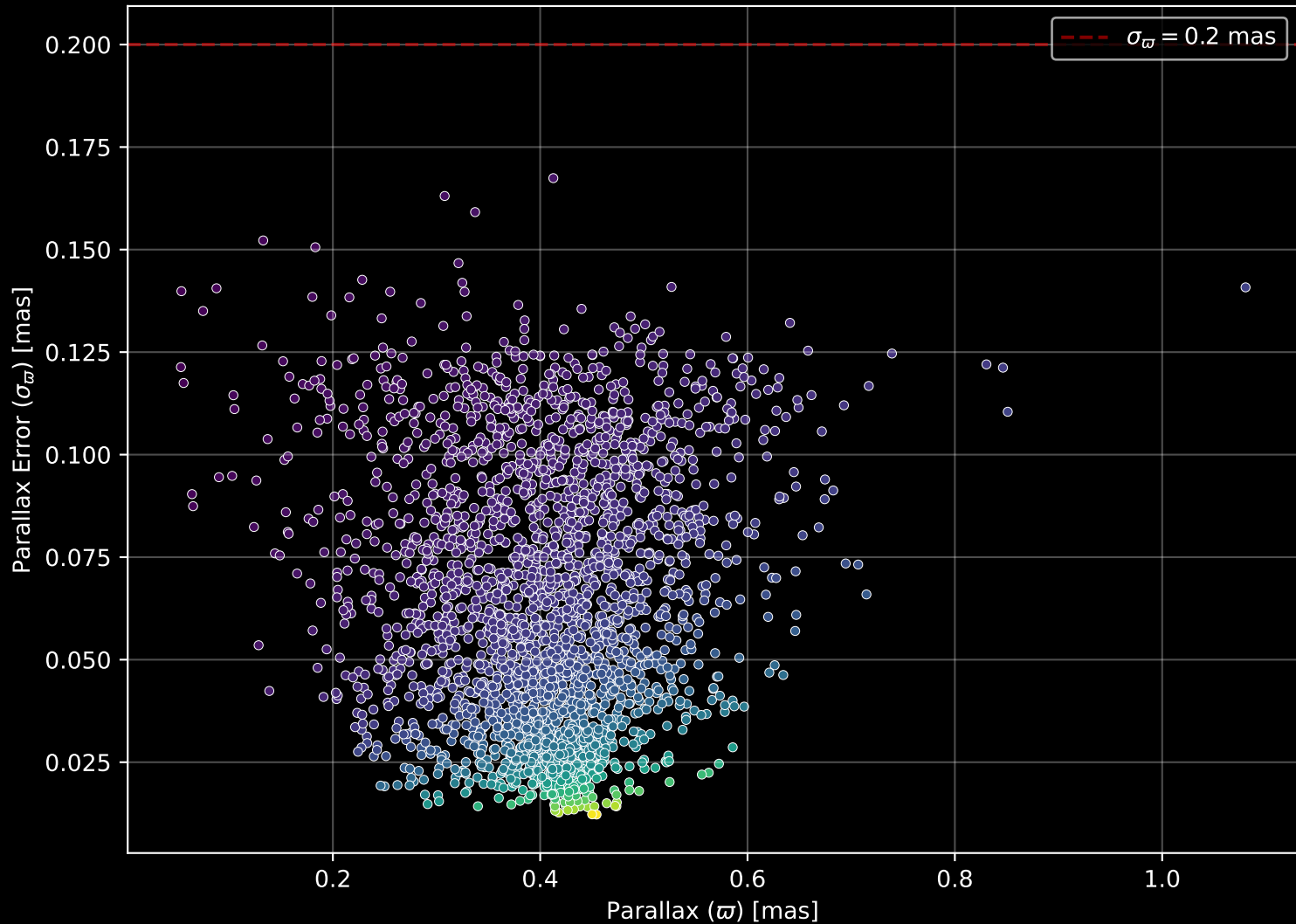
Gaia Cluster: [NGC_6259] Parallax Quality (n= 2578)
