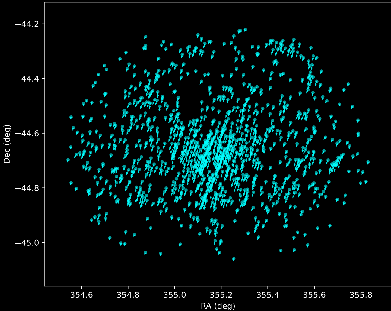
Gaia DR3 Noise Stream Proper Motion Vectors (n=986)
