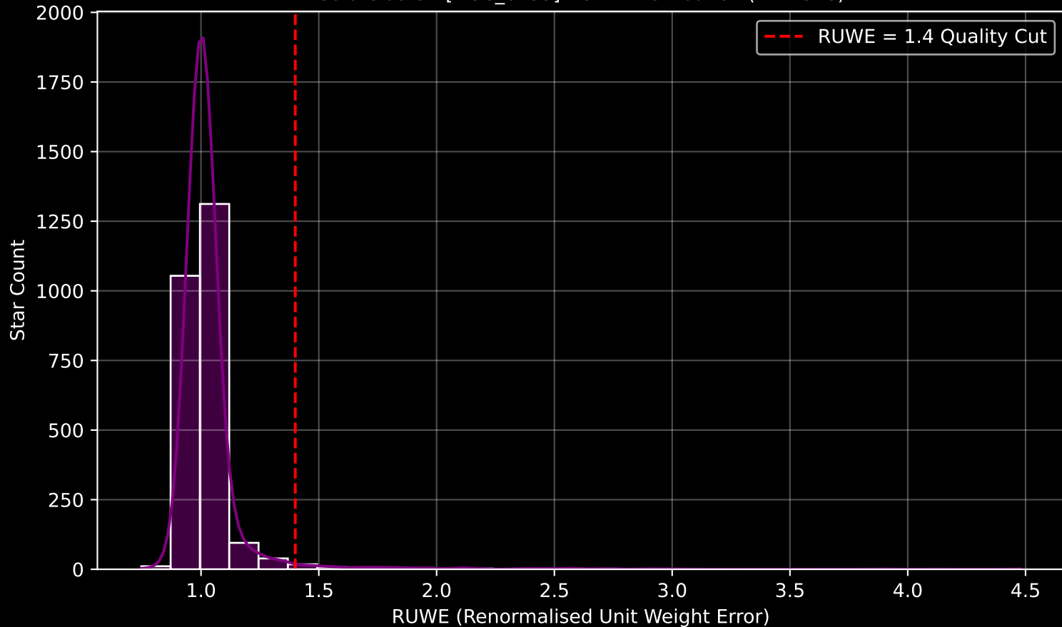
Gaia Cluster: [NGC_6259] RUWE Distribution (n= 2578)
