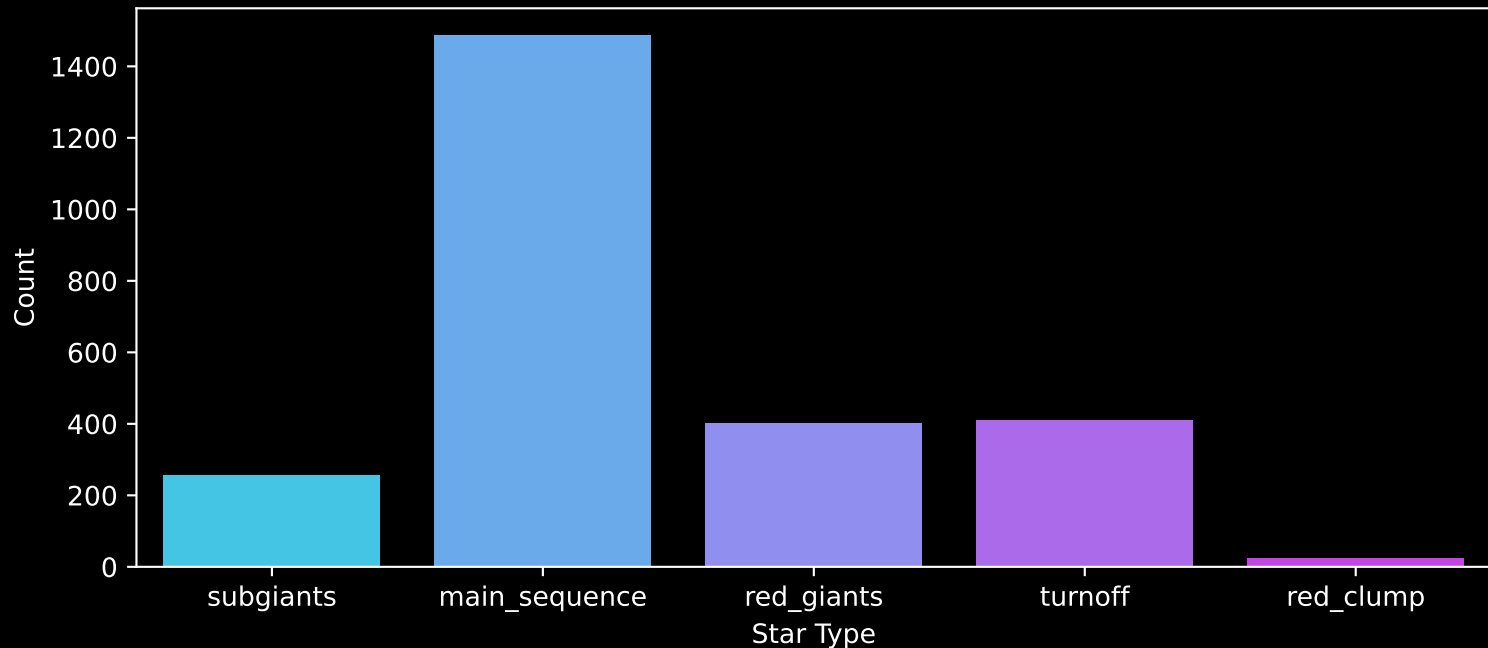
Gaia Cluster: [NGC_6259] Count plot of Star Type
