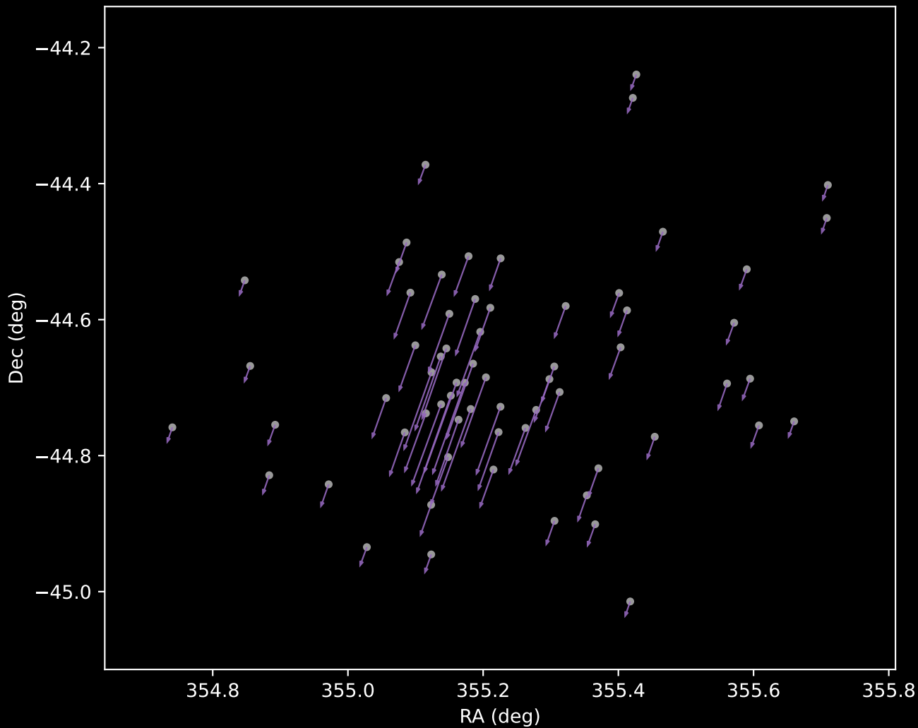
Gaia DR3 Cluster 148 Proper Motion Vectors (n=65)
