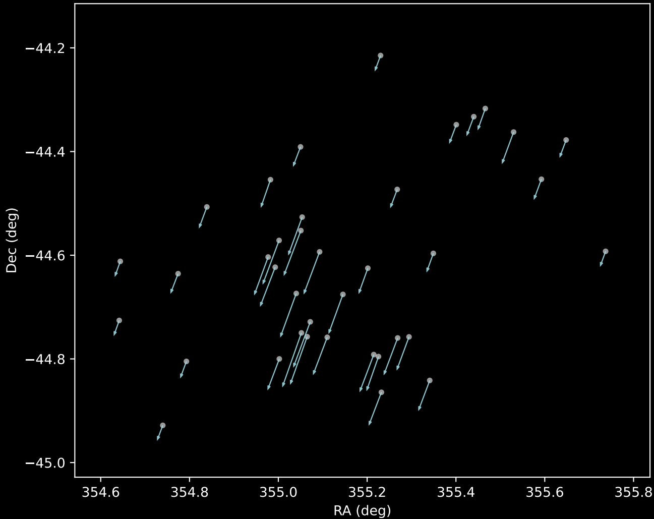
Gaia DR3 Cluster 119 Proper Motion Vectors (n=38)
