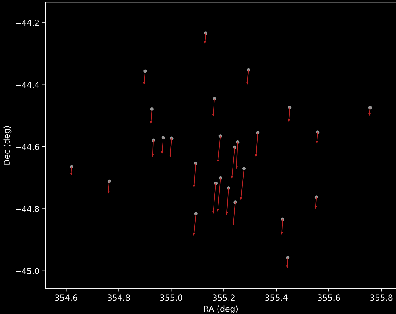
Gaia DR3 Cluster 6 Proper Motion Vectors (n=27)
