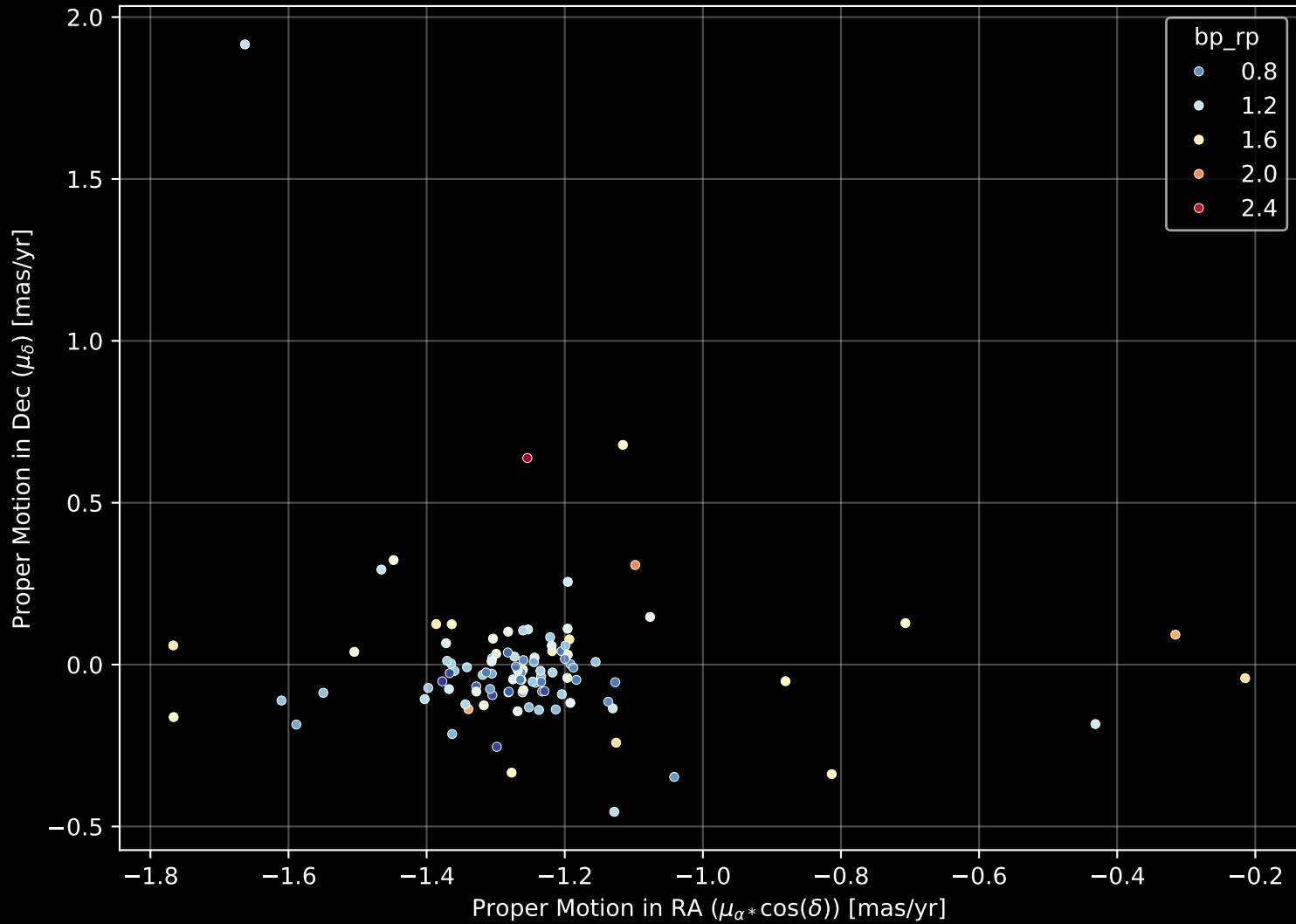
Gaia Cluster: [NGC_637] Proper Motion Diagram (n= 104)
