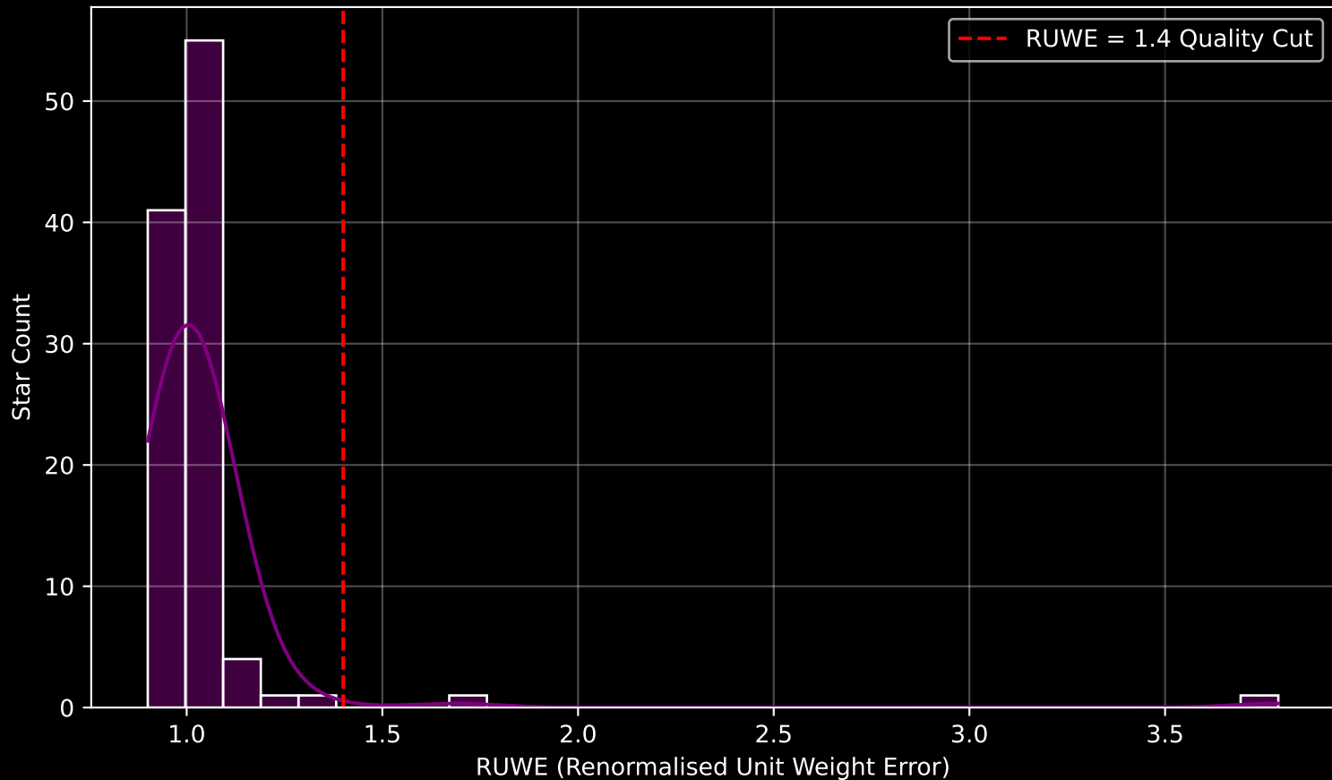
Gaia Cluster: [NGC_637] RUWE Distribution (n= 104)
