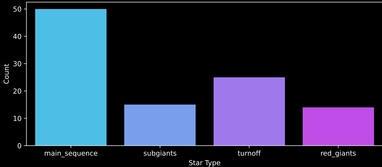
Gaia Cluster: [NGC_637] Count plot of Star Type
