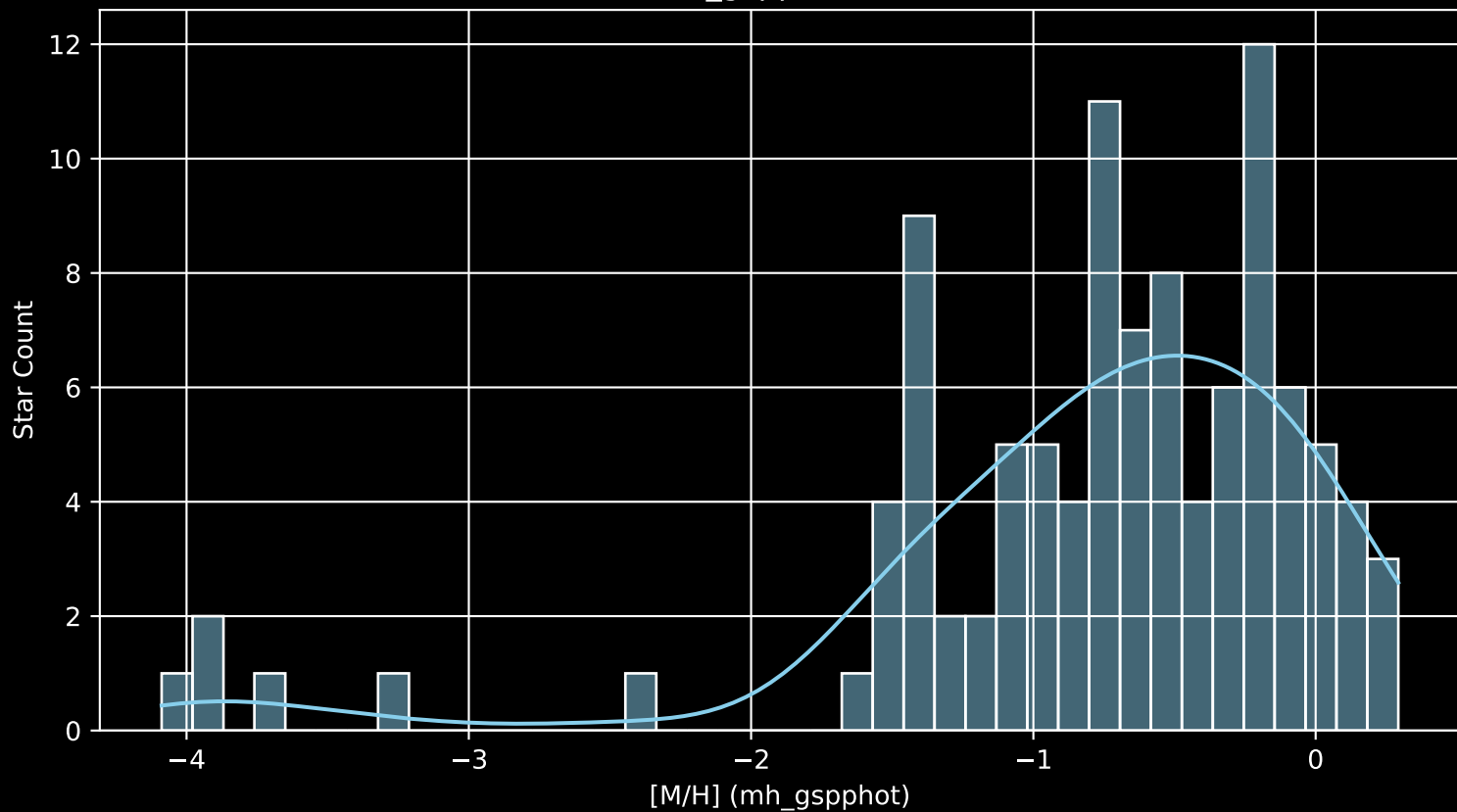
Gaia Cluster: [NGC_637 [M/H] (mh_gspphot) (n= 104)
