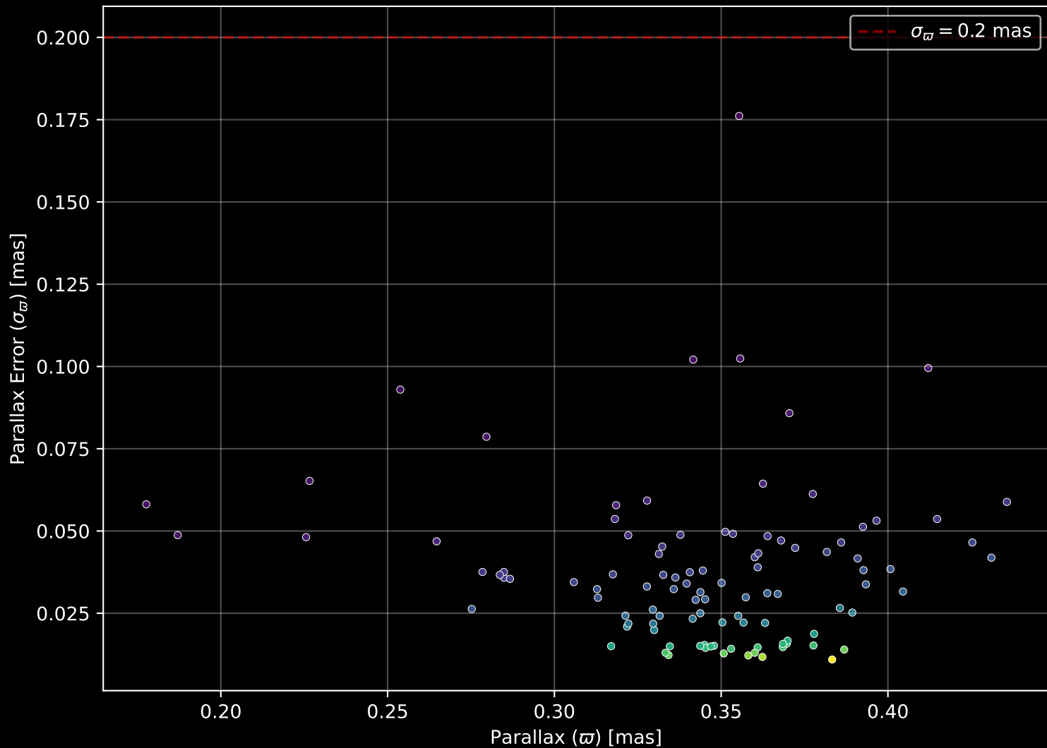
Gaia Cluster: [NGC_637] Parallax Quality (n= 104)
