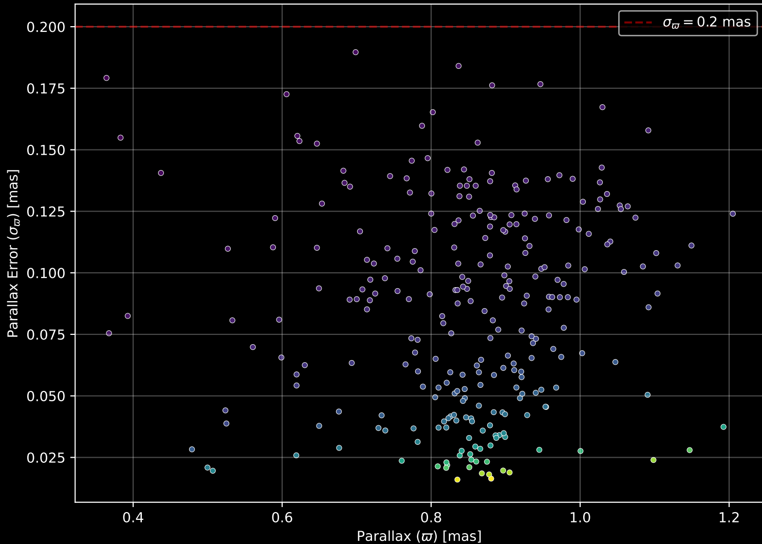
Gaia Cluster: [NGC_6383] Parallax Quality (n= 271)
