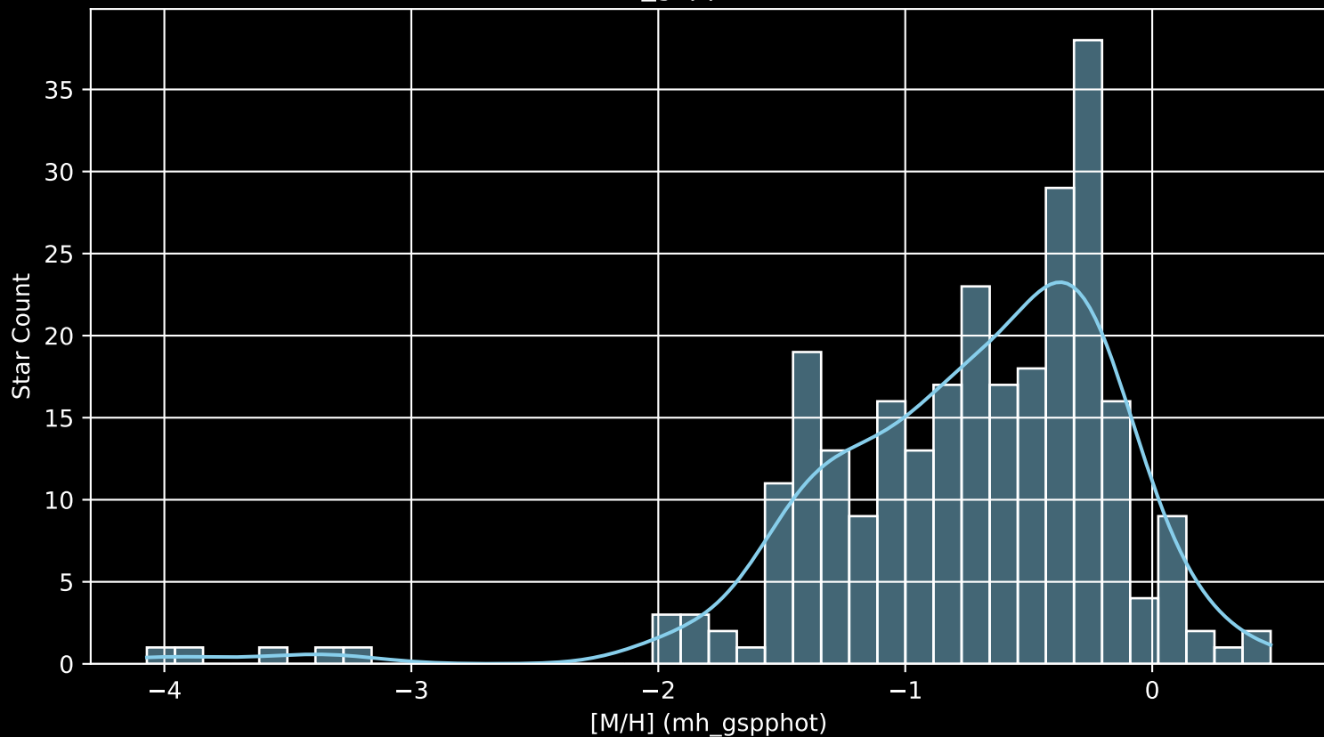
Gaia Cluster: [NGC_6383 [M/H] (mh_gspphot) (n= 271)
