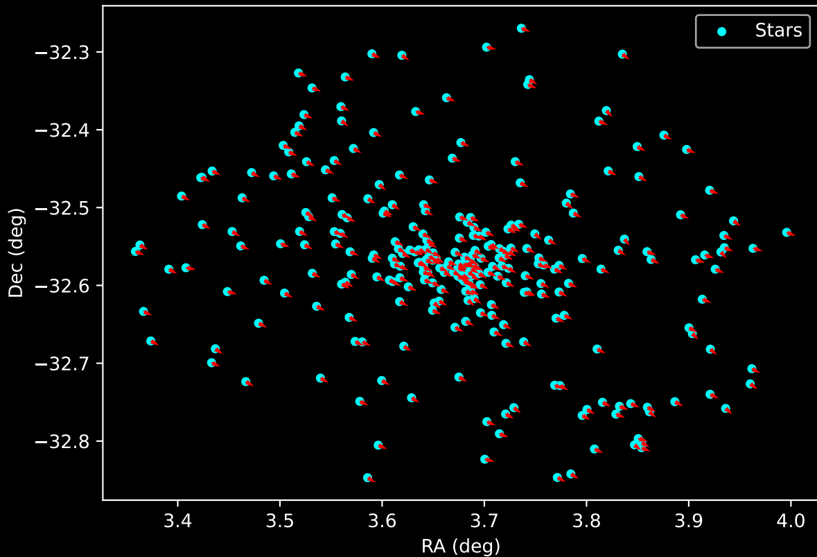
Gaia Cluster: [NGC_6383] Proper Motion Vectors for Gaia Star Field (n= 271)
