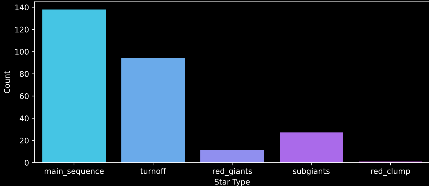
Gaia Cluster: [NGC_6383] Count plot of Star Type
