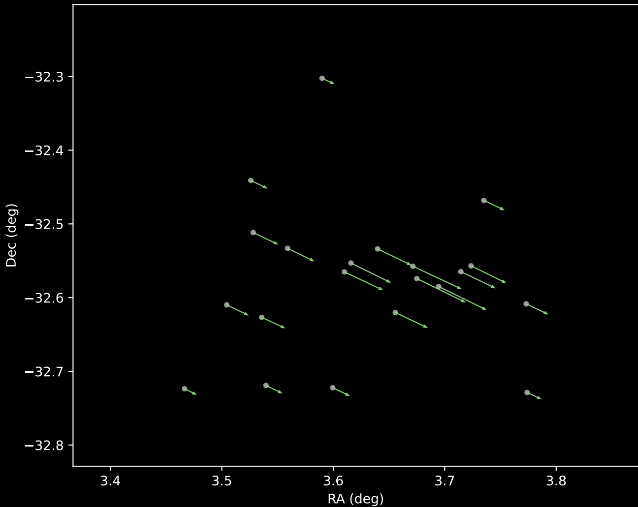
Gaia DR3 Cluster 5 Proper Motion Vectors (n=21)
