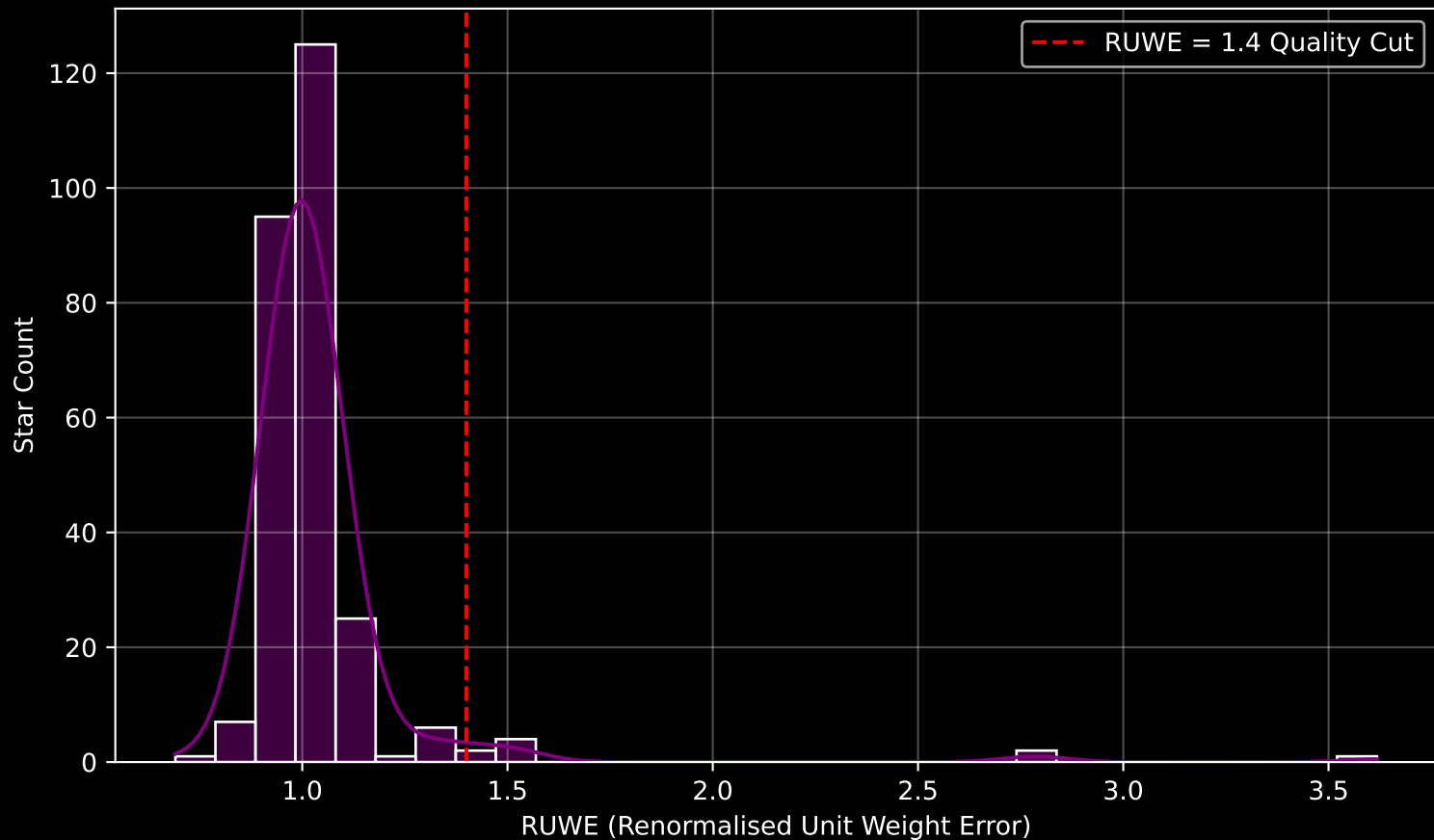
Gaia Cluster: [NGC_6383] RUWE Distribution (n= 269)
