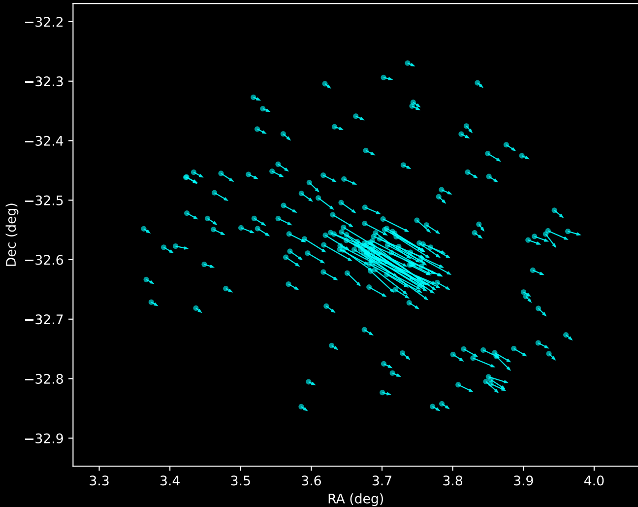
Gaia DR3 Noise Stream Proper Motion Vectors (n=161)
