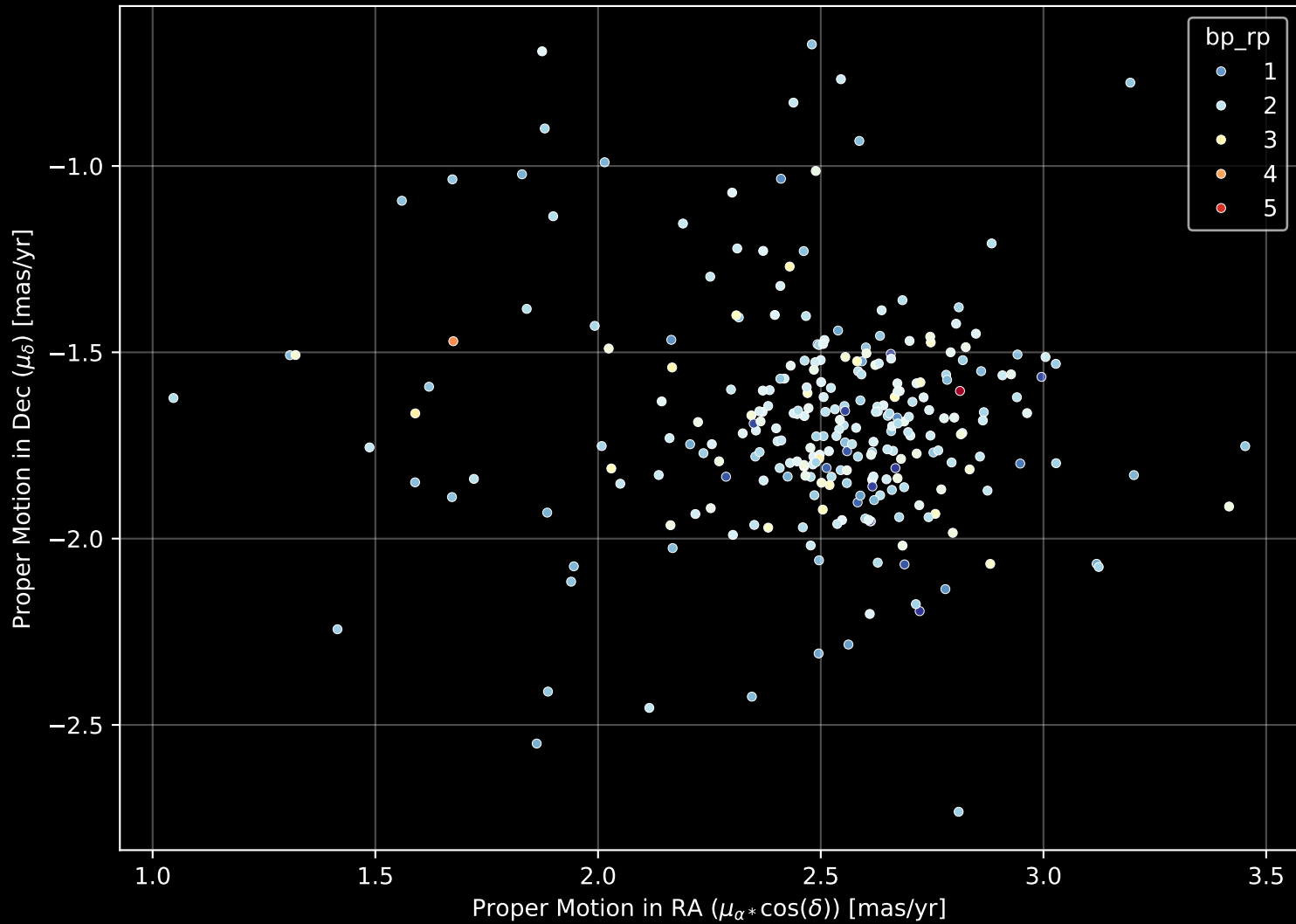
Gaia Cluster: [NGC_6383] Proper Motion Diagram (n= 271)
