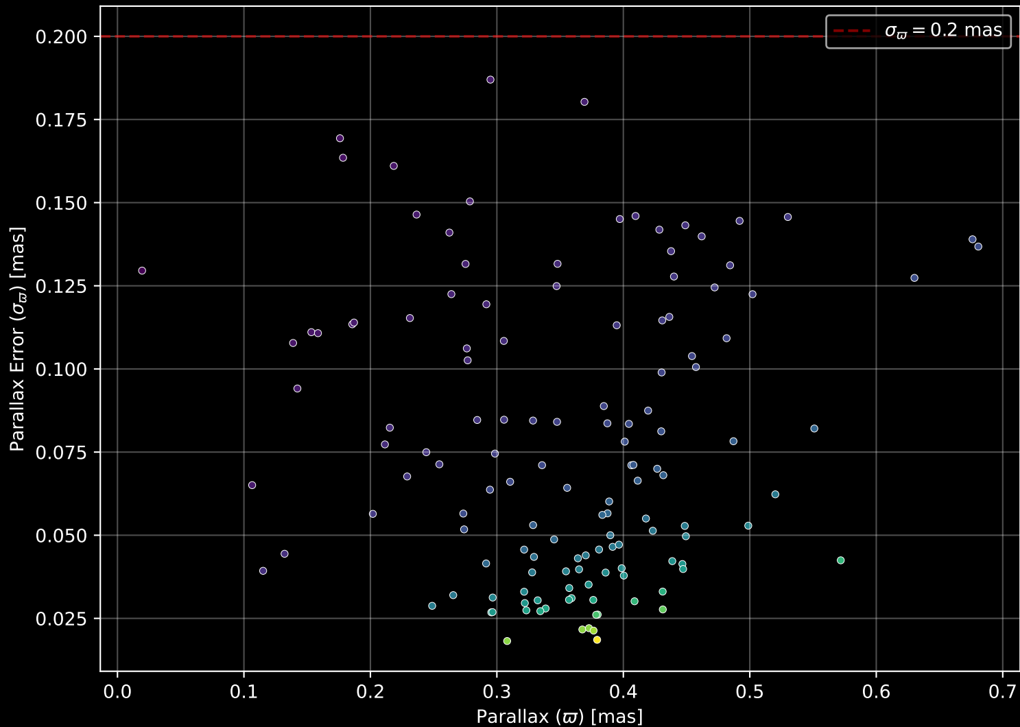
Gaia Cluster: [NGC_6396] Parallax Quality (n= 135)
