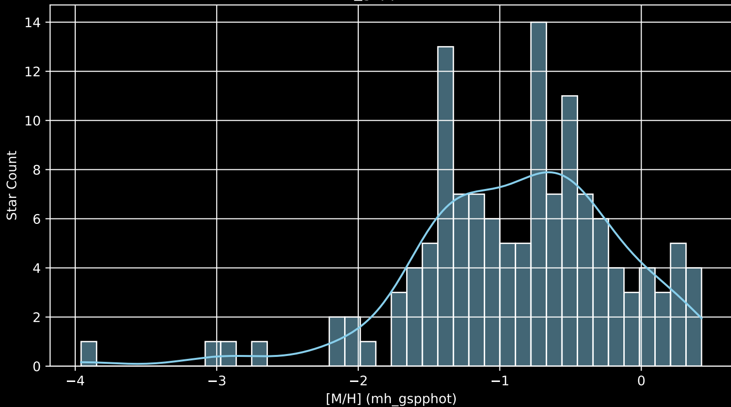
Gaia Cluster: [NGC_6396 [M/H] (mh_gspphot) (n= 132)
