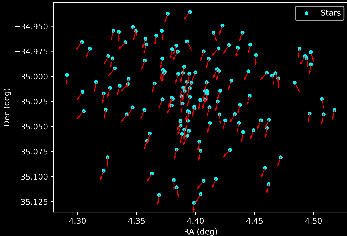
Gaia Cluster: [NGC_6396] Proper Motion Vectors for Gaia Star Field (n= 135)
