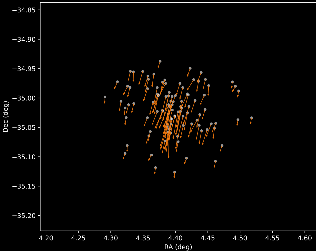
Gaia DR3 Cluster 2 Proper Motion Vectors (n=100)
