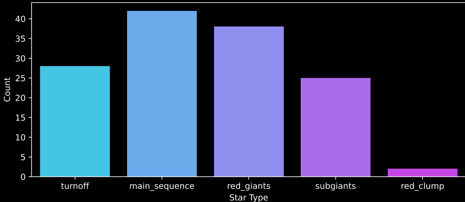
Gaia Cluster: [NGC_6396] Count plot of Star Type
