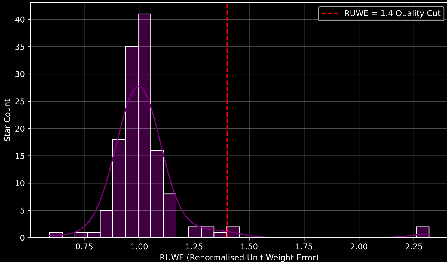
Gaia Cluster: [NGC_6396] RUWE Distribution (n= 135)
