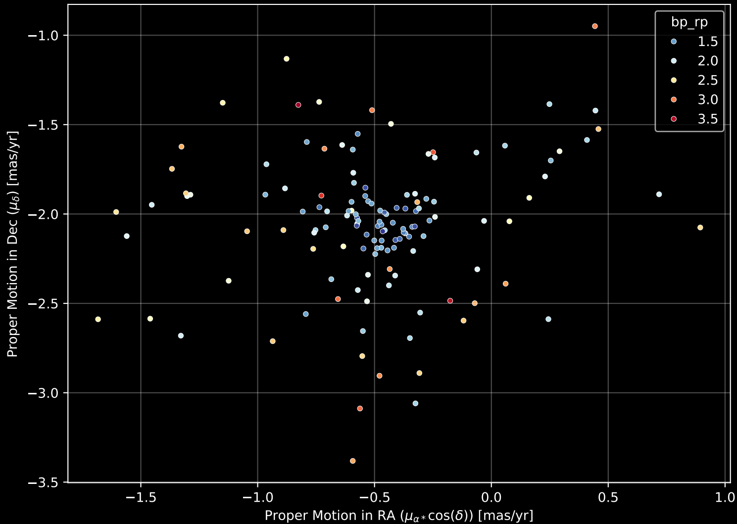
Gaia Cluster: [NGC_6396] Proper Motion Diagram (n= 135)
