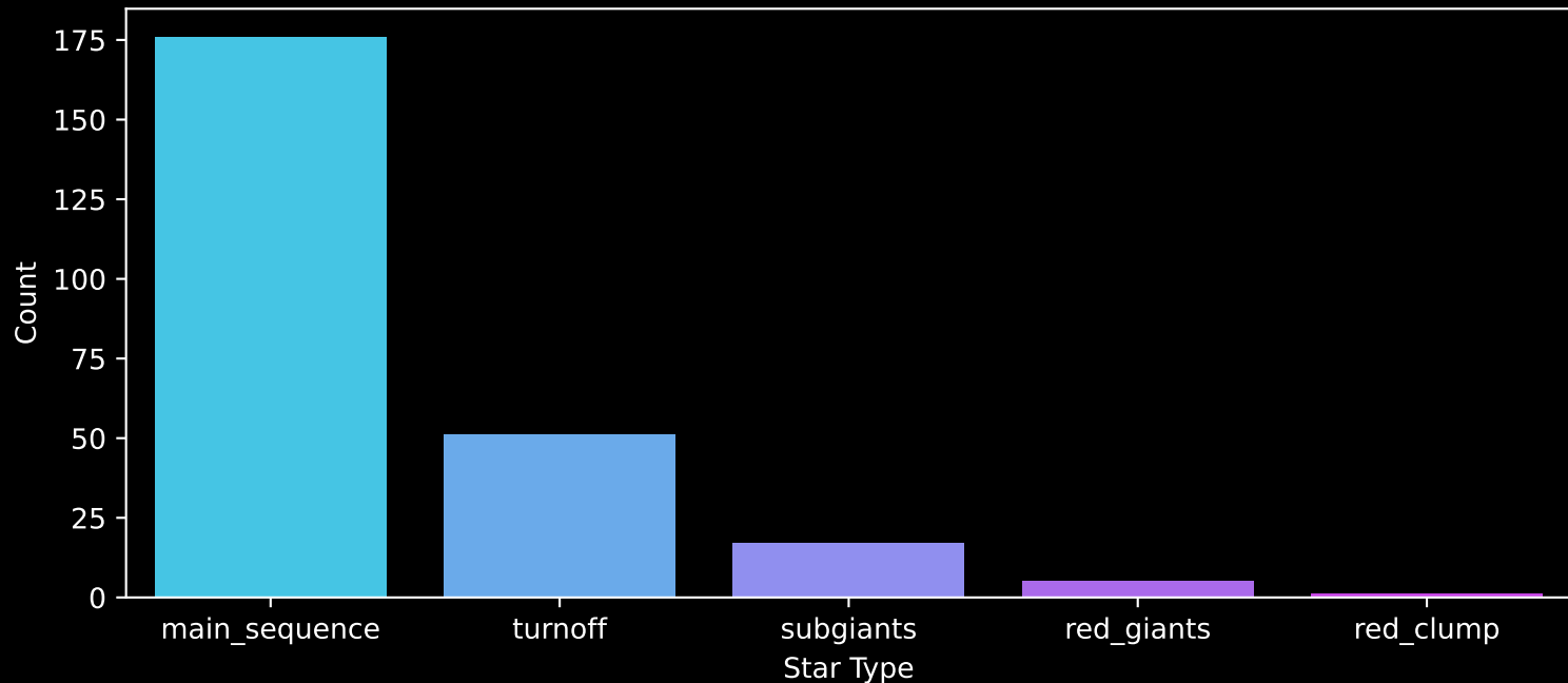
Gaia Cluster: [NGC_6400] Count plot of Star Type
