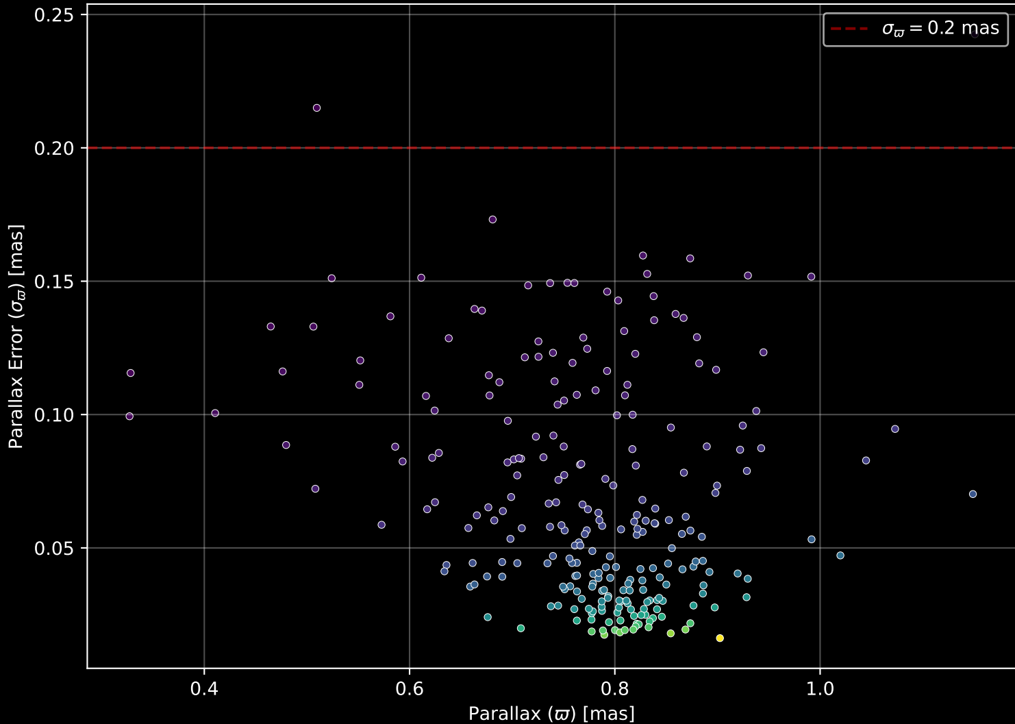
Gaia Cluster: [NGC_6400] Parallax Quality (n= 250)
