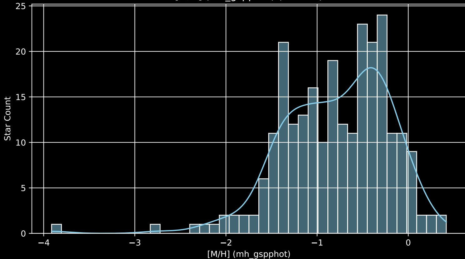
Gaia Cluster: [NGC_6400 [M/H] (mh_gspphot) (n= 249)
