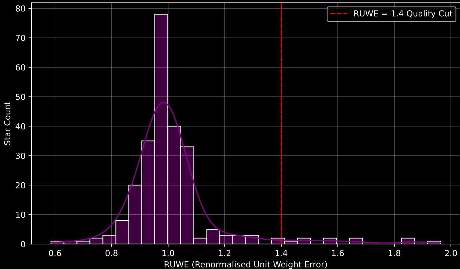
Gaia Cluster: [NGC_6400] RUWE Distribution (n= 250)
