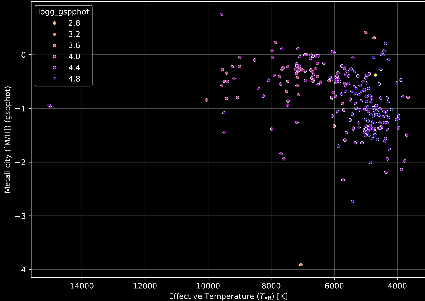
Gaia Cluster: [NGC_6400] Stellar Population Parameters (n= 250)
