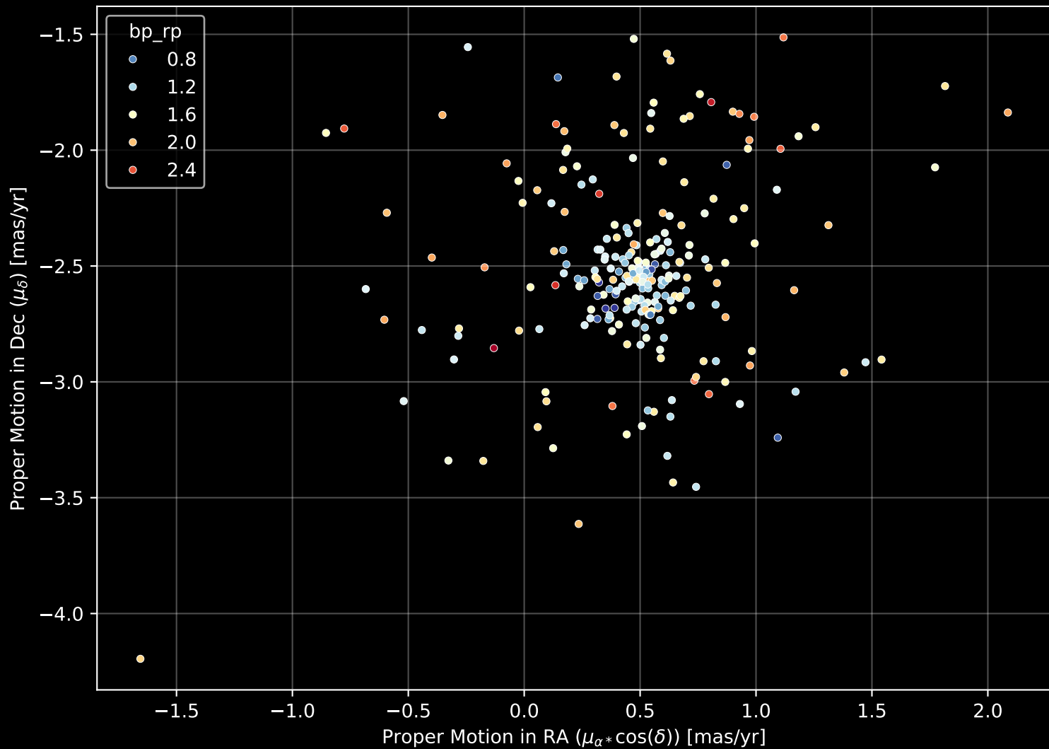
Gaia Cluster: [NGC_6400] Proper Motion Diagram (n= 250)
