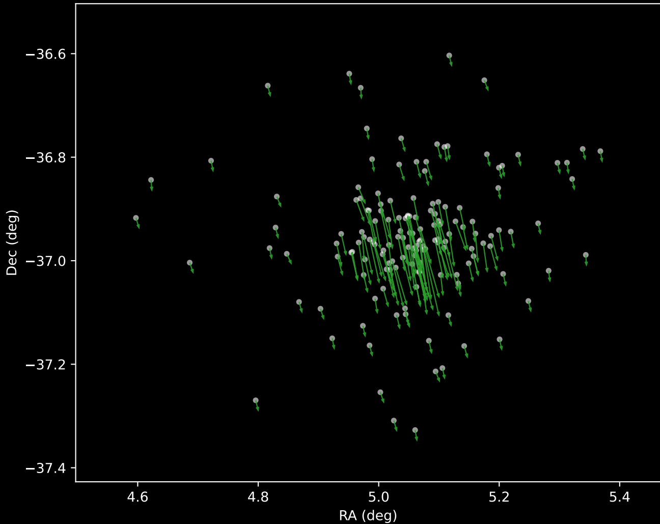
Gaia DR3 Cluster 4 Proper Motion Vectors (n=149)
