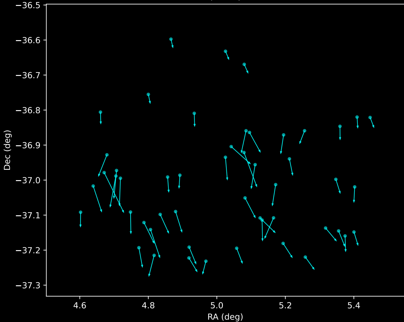
Gaia DR3 Noise Stream Proper Motion Vectors (n=51)
