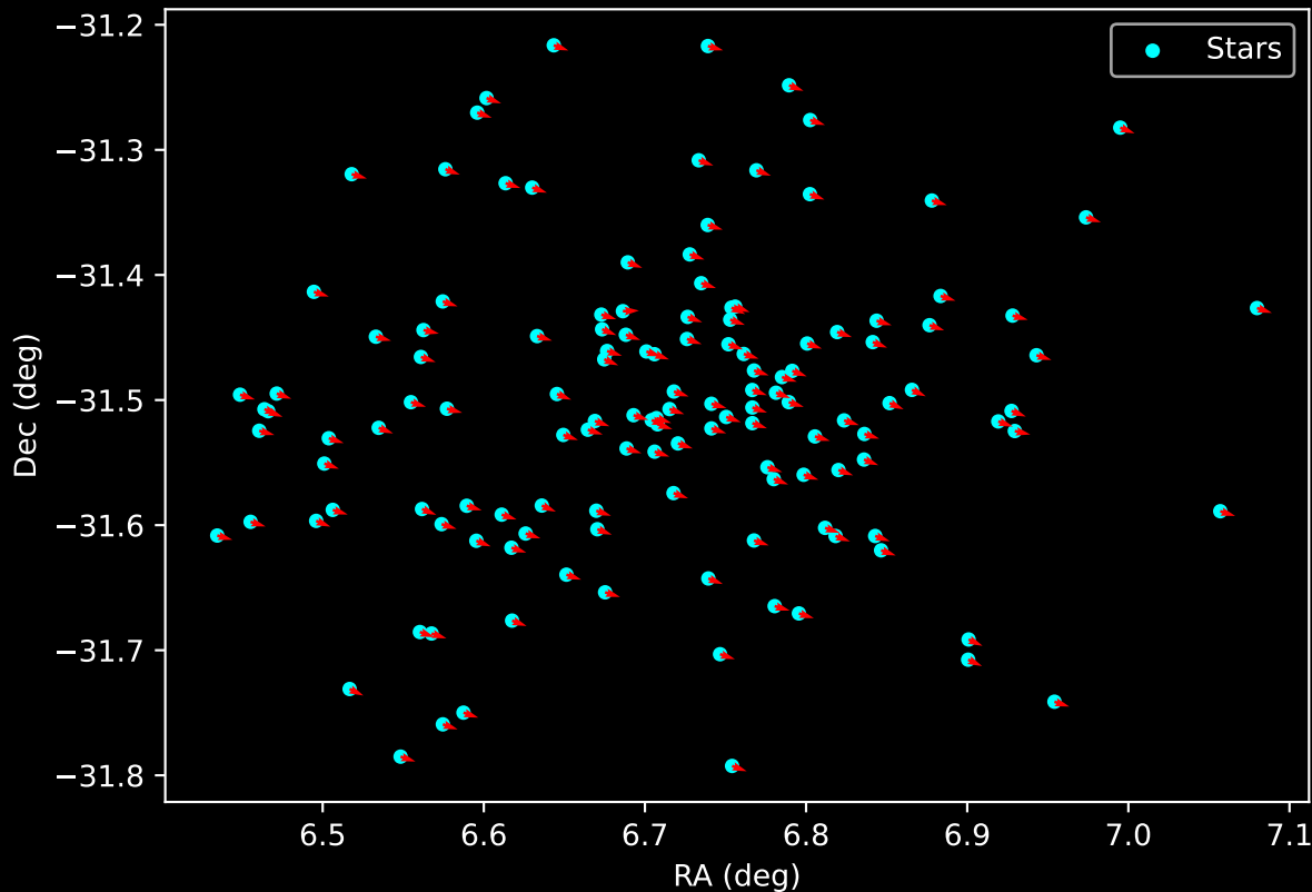
Gaia Cluster: [NGC_6425] Proper Motion Vectors for Gaia Star Field (n= 135)
