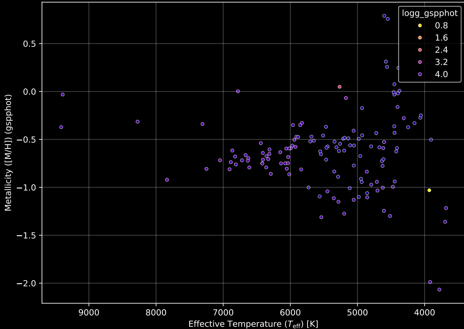
Gaia Cluster: [NGC_6425] Stellar Population Parameters (n= 135)
