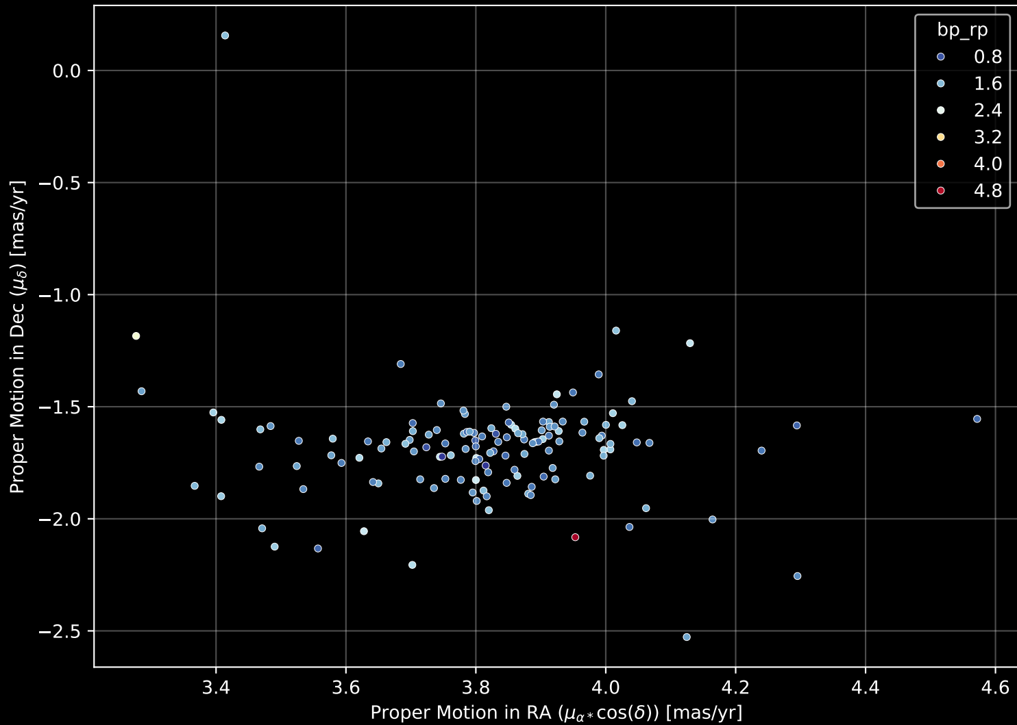
Gaia Cluster: [NGC_6425] Proper Motion Diagram (n= 135)
