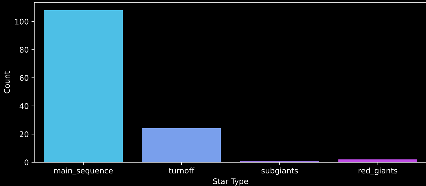
Gaia Cluster: [NGC_6425] Count plot of Star Type
