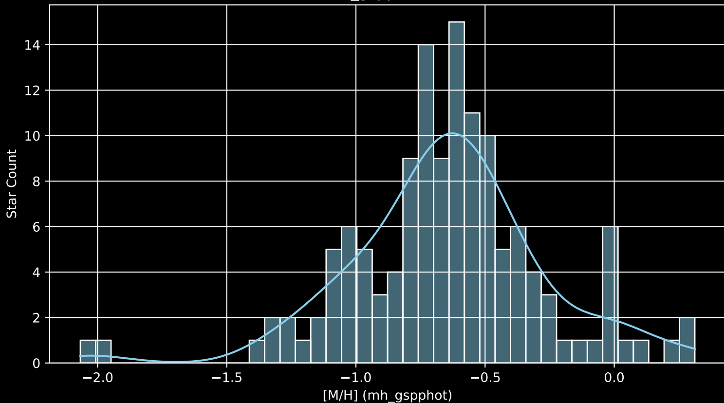
Gaia Cluster: [NGC_6425 [M/H] (mh_gspphot) (n= 133)
