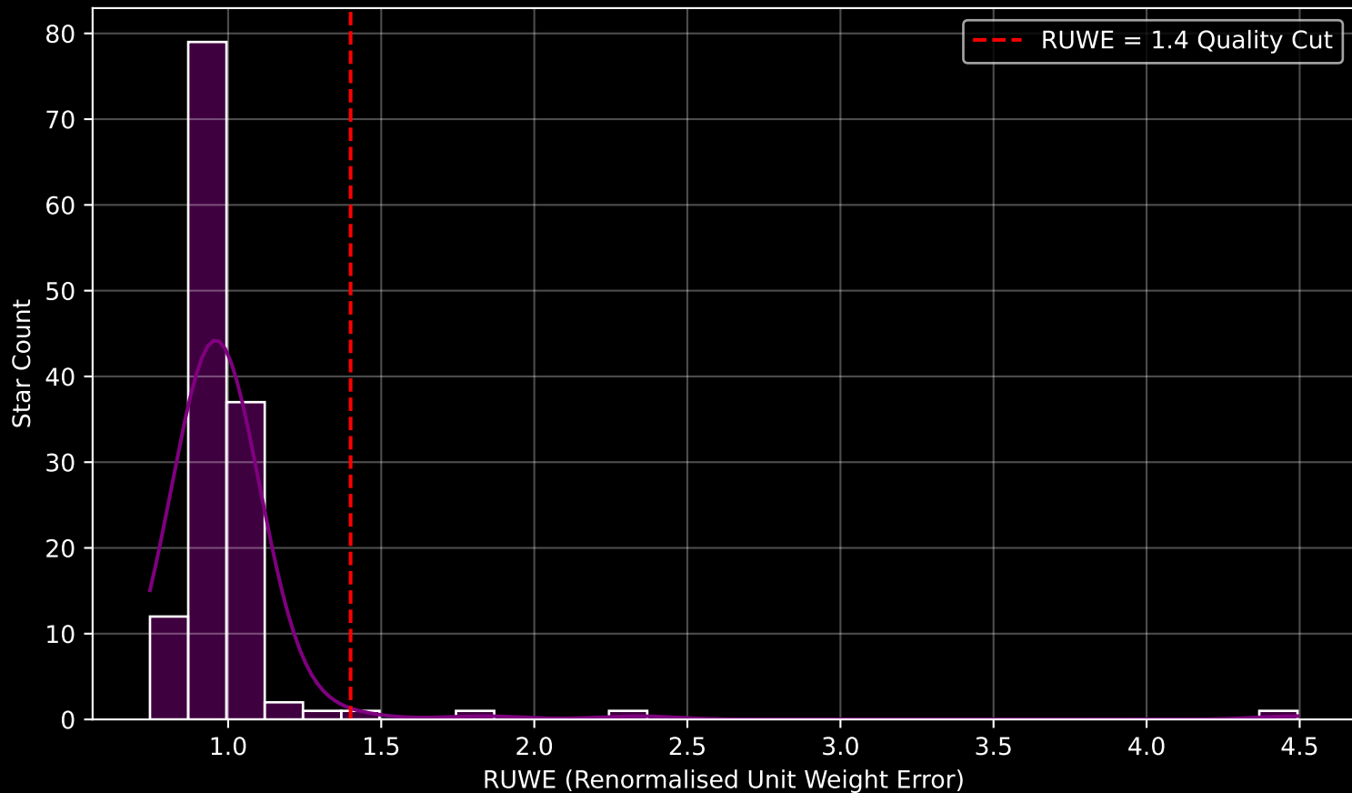
Gaia Cluster: [NGC_6425] RUWE Distribution (n= 135)
