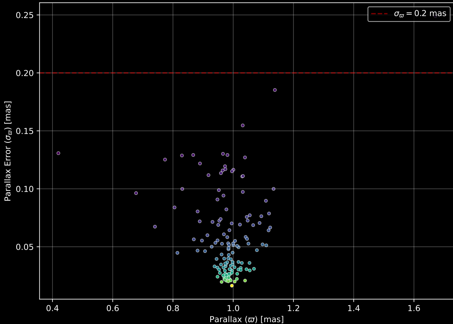
Gaia Cluster: [NGC_6425] Parallax Quality (n= 135)
