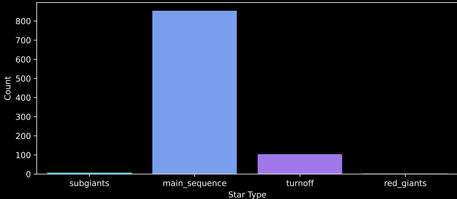
Gaia Cluster: [NGC_6475] Count plot of Star Type
