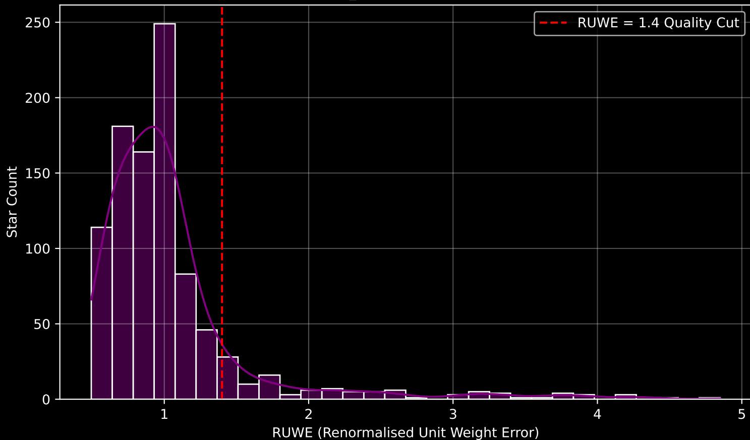
Gaia Cluster: [NGC_6475] RUWE Distribution (n= 950)
