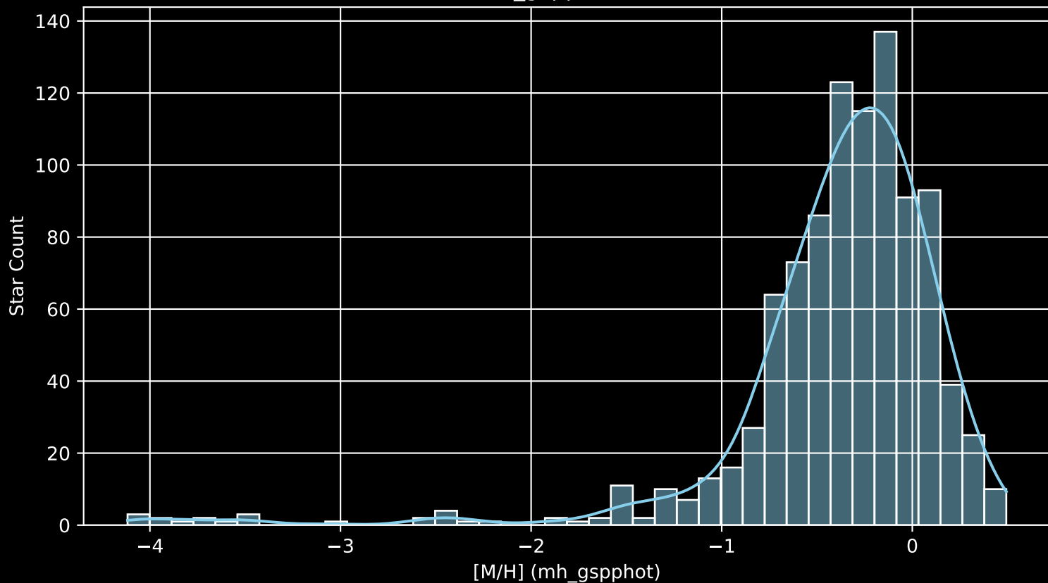
Gaia Cluster: [NGC_6475 [M/H] (mh_gspphot) (n= 968)
