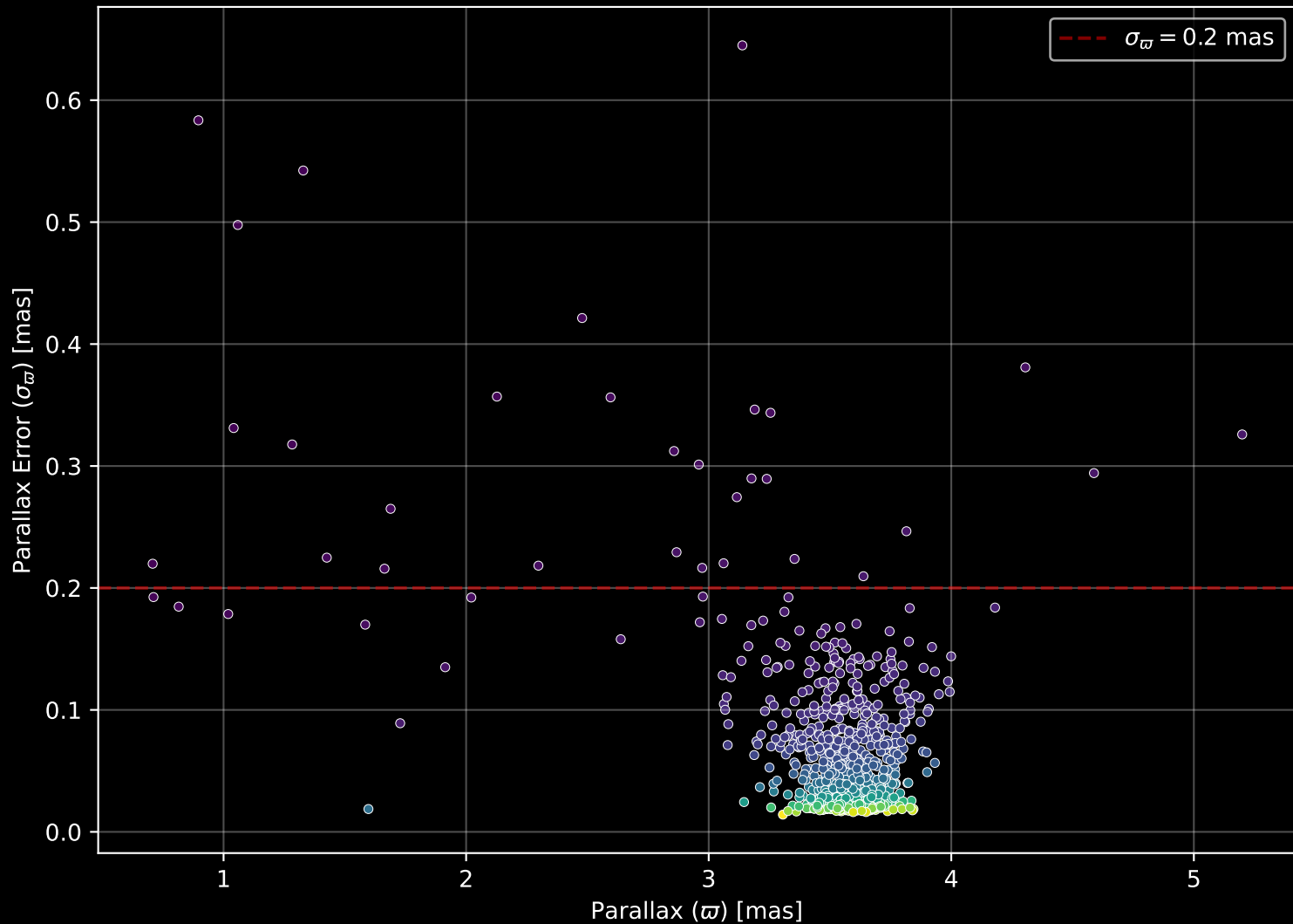
Gaia Cluster: [NGC_6475] Parallax Quality (n= 968)
