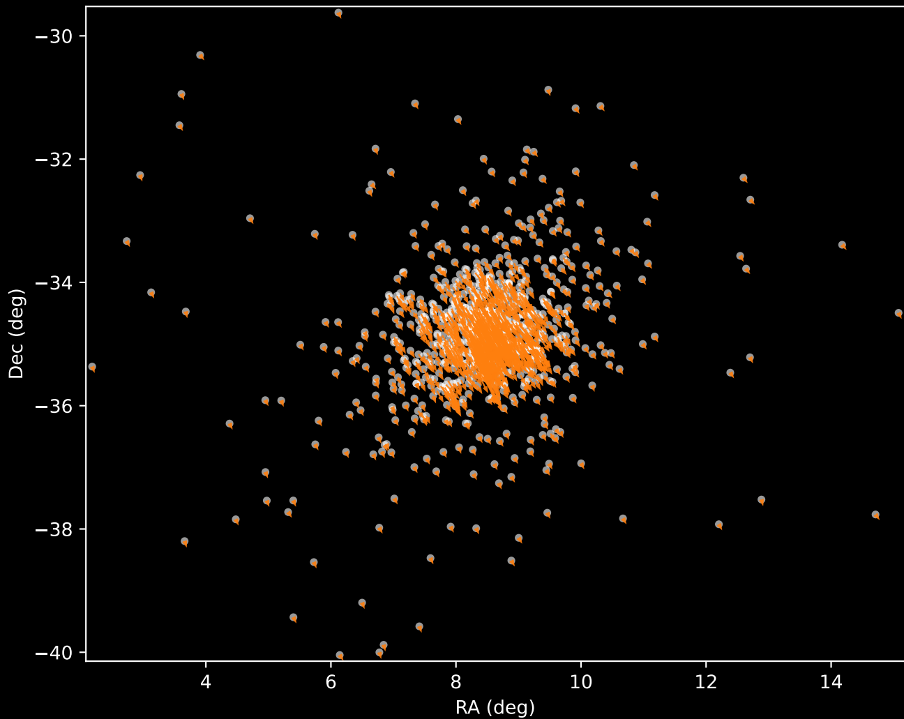
Gaia DR3 Cluster 2 Proper Motion Vectors (n=898)
