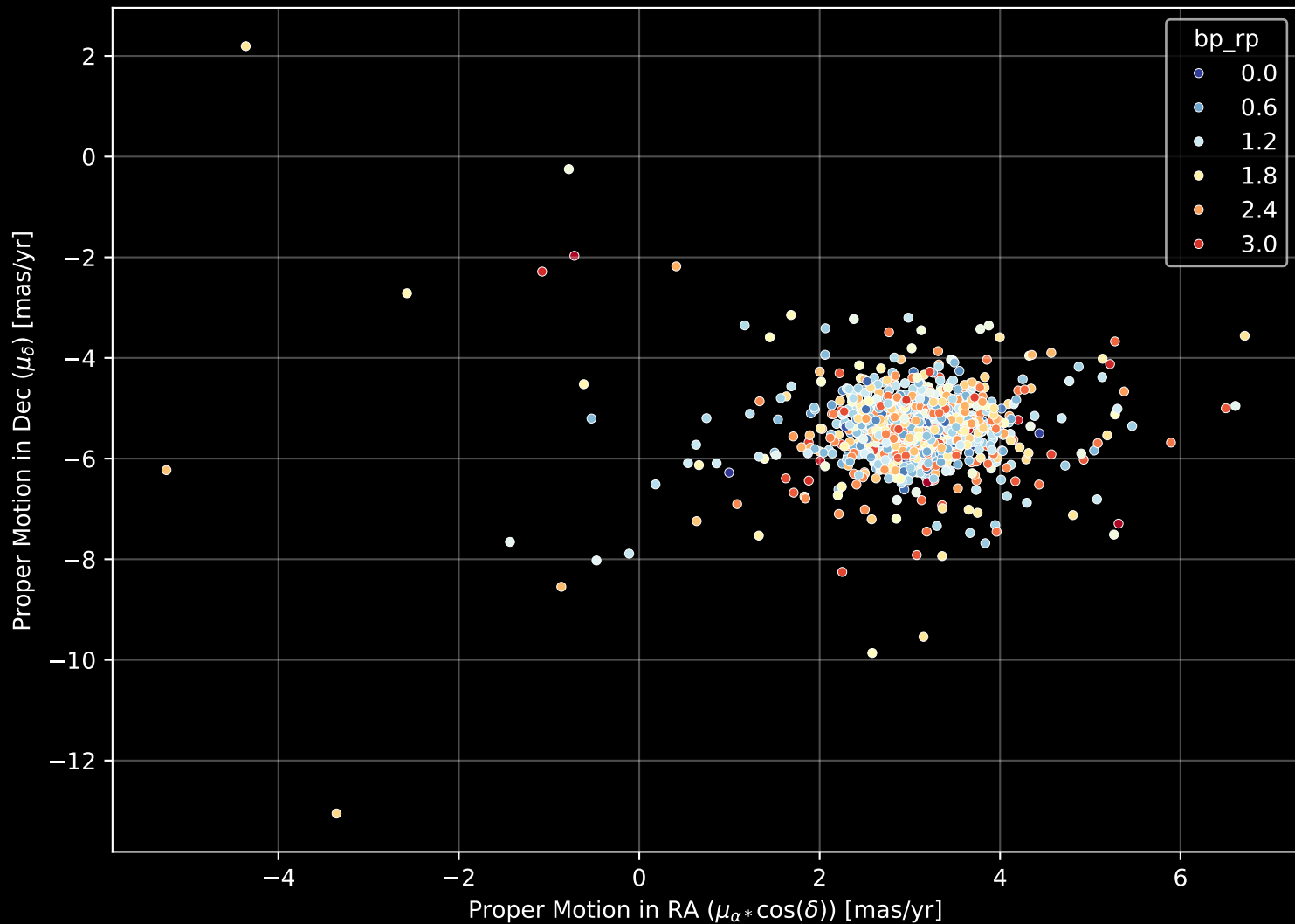
Gaia Cluster: [NGC_6475] Proper Motion Diagram (n= 968)
