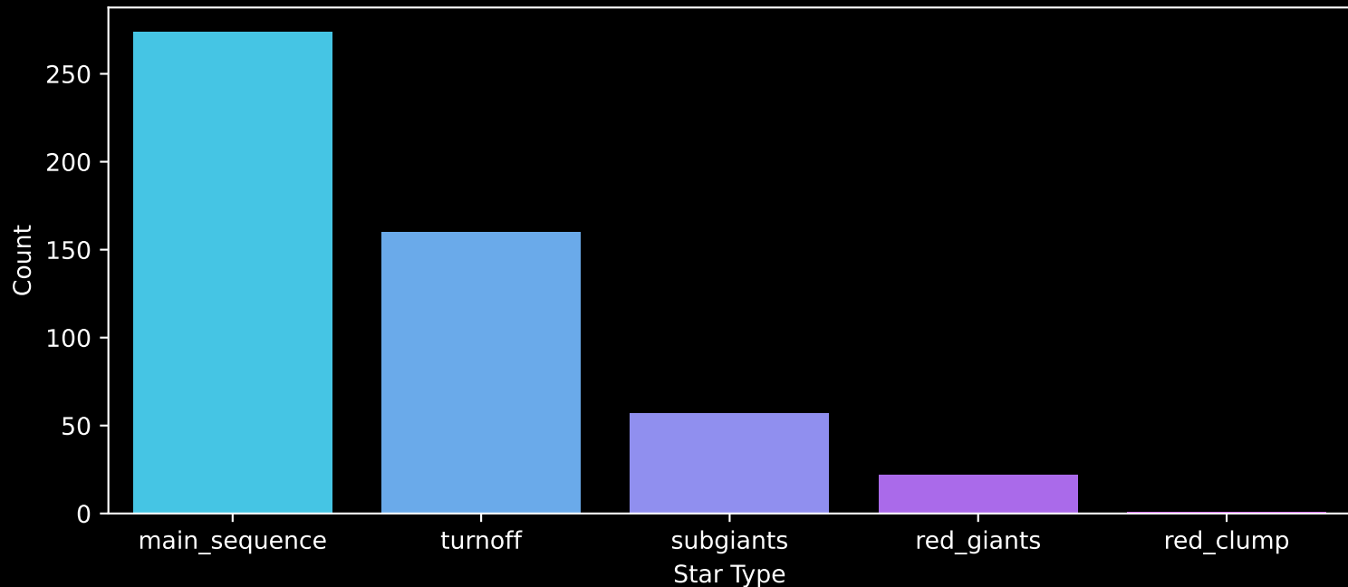
Gaia Cluster: [NGC_6531] Count plot of Star Type
