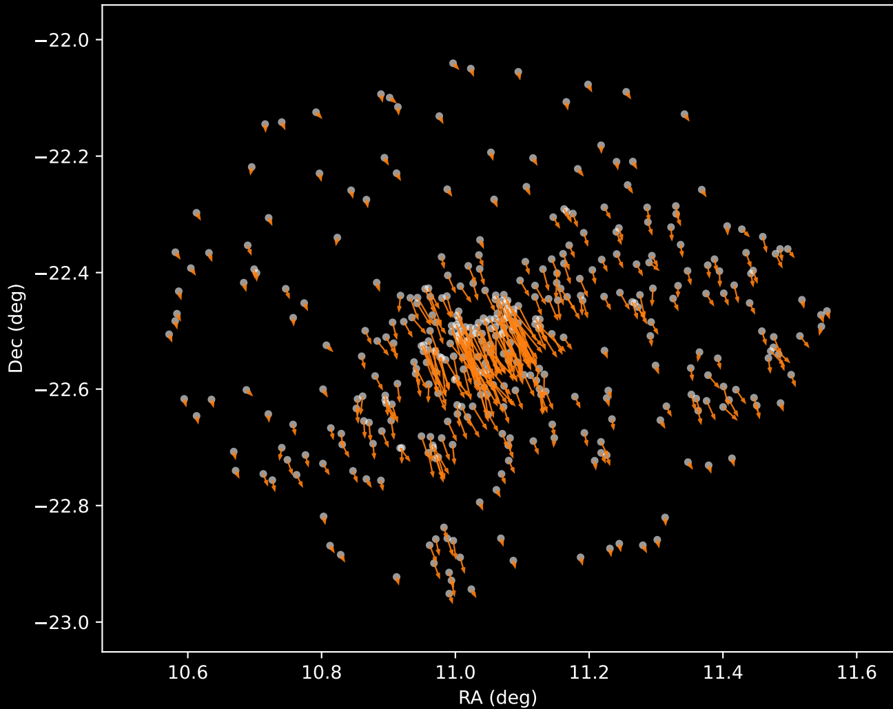
Gaia DR3 Cluster 2 Proper Motion Vectors (n=391)
