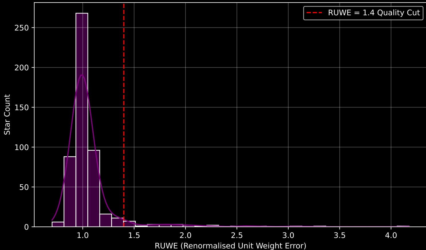
Gaia Cluster: [NGC_6531] RUWE Distribution (n= 513)
