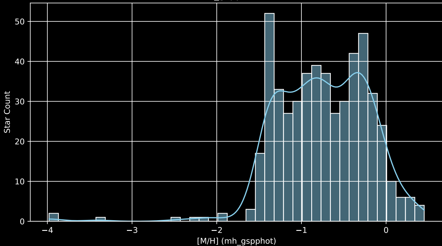
Gaia Cluster: [NGC_6531 [M/H] (mh_gspphot) (n= 511)
