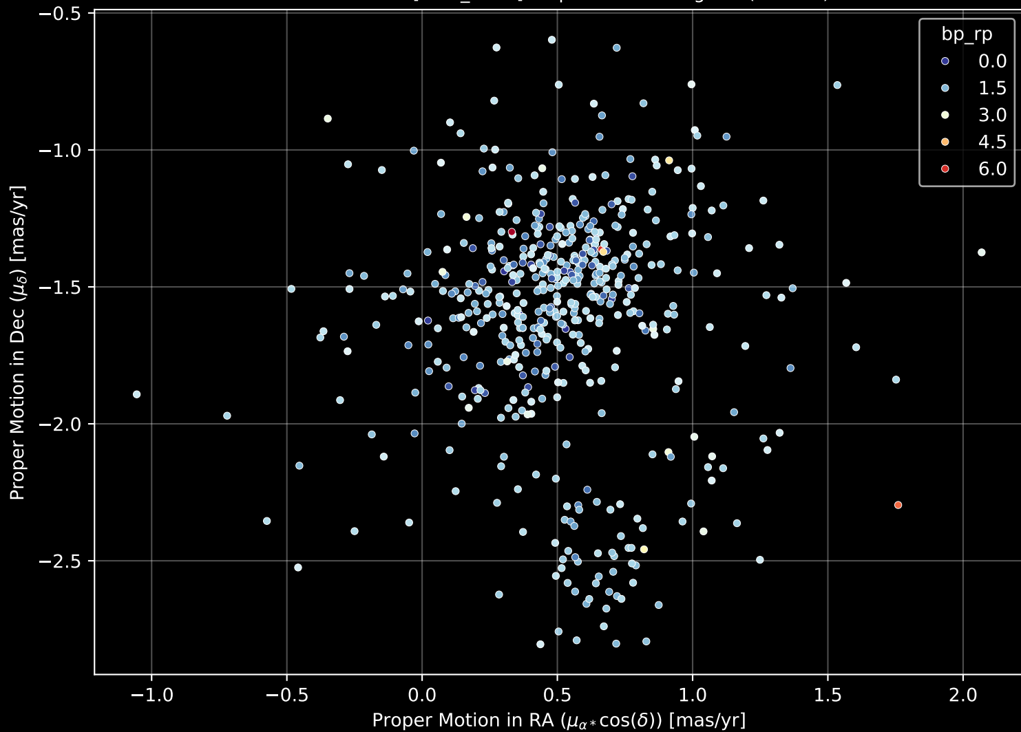
Gaia Cluster: [NGC_6531] Proper Motion Diagram (n= 514)
