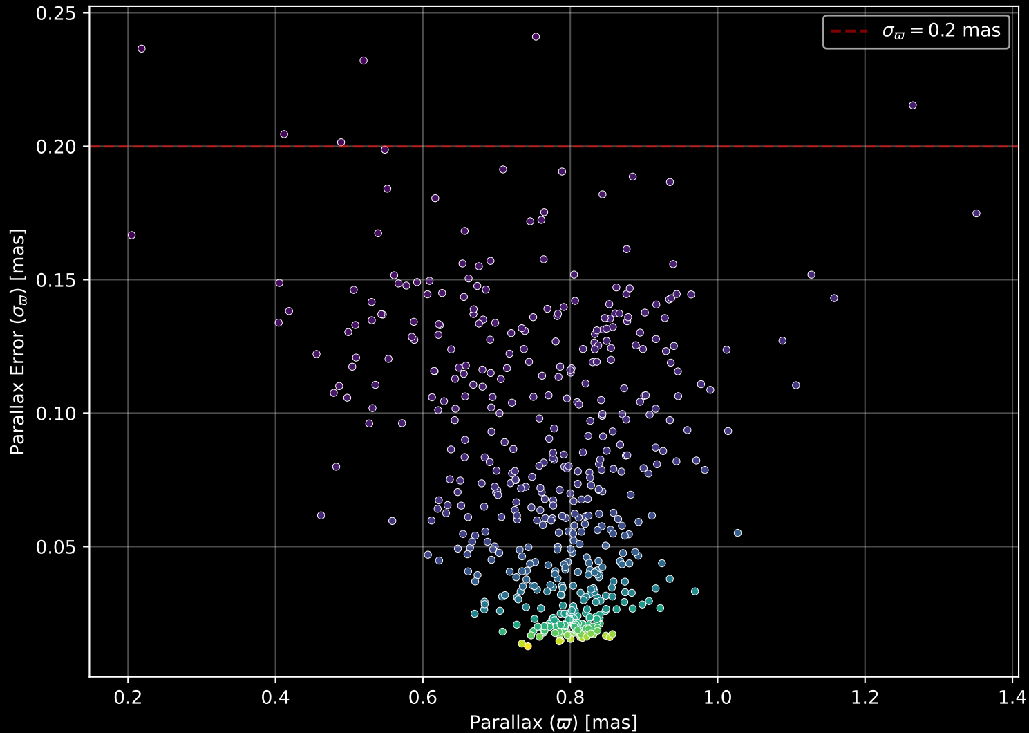
Gaia Cluster: [NGC_6531] Parallax Quality (n= 514)
