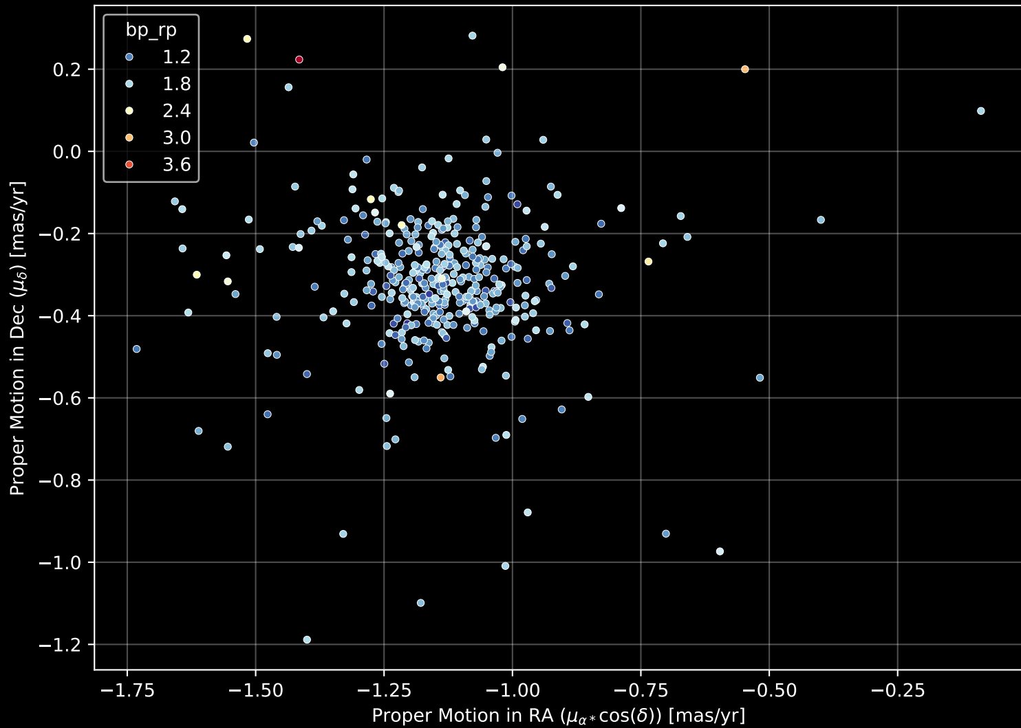
Gaia Cluster: [NGC_654] Proper Motion Diagram (n= 403)
