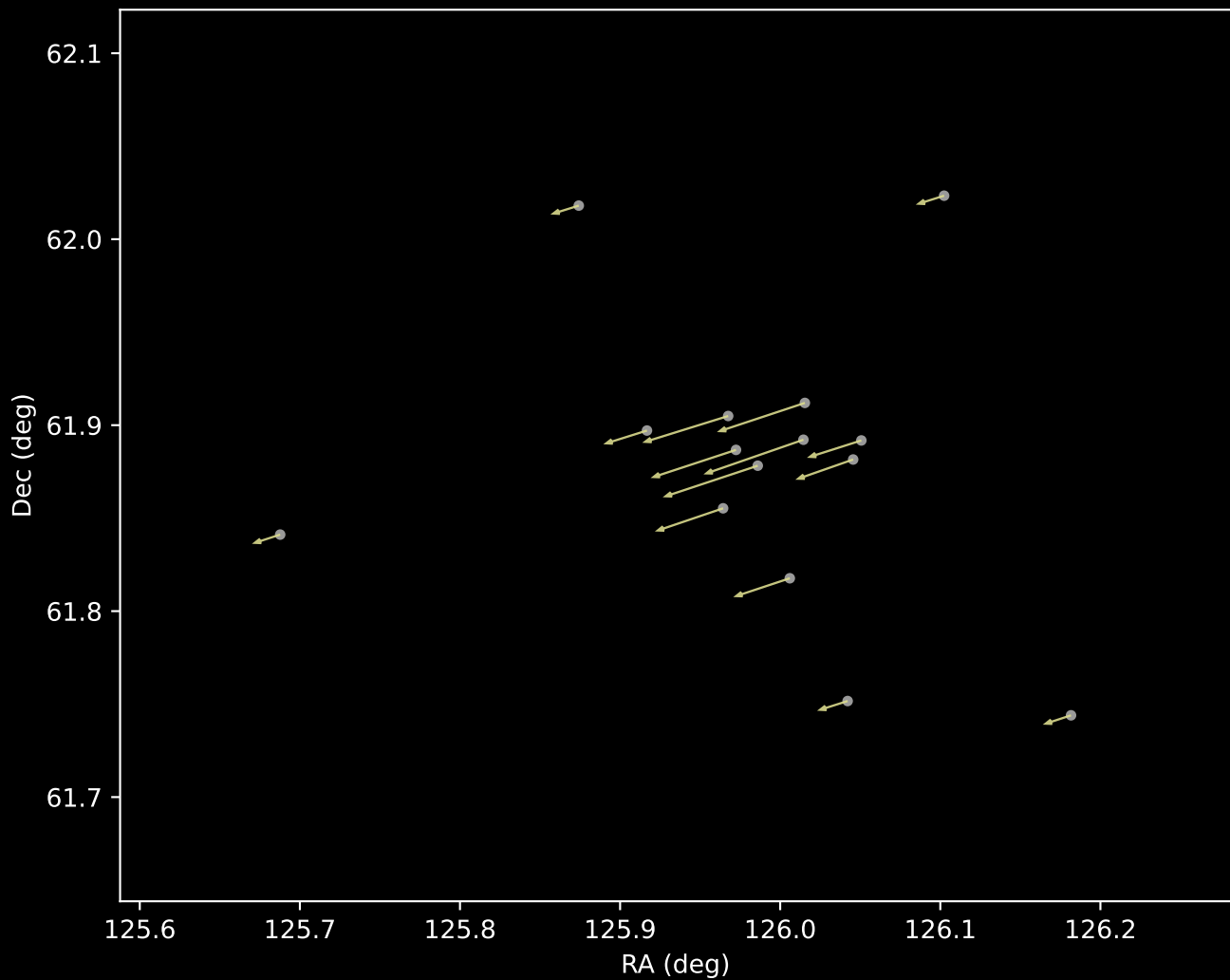
Gaia DR3 Cluster 17 Proper Motion Vectors (n=15)
