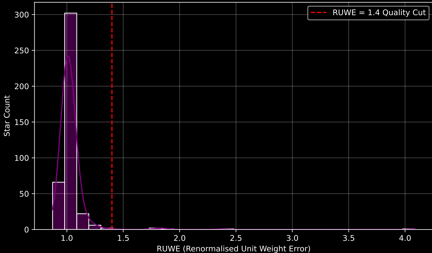
Gaia Cluster: [NGC_654] RUWE Distribution (n= 403)
