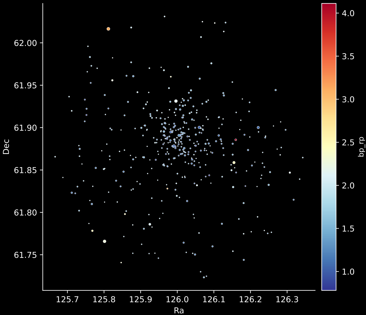
Gaia Cluster: [NGC_654] Stars: 403
