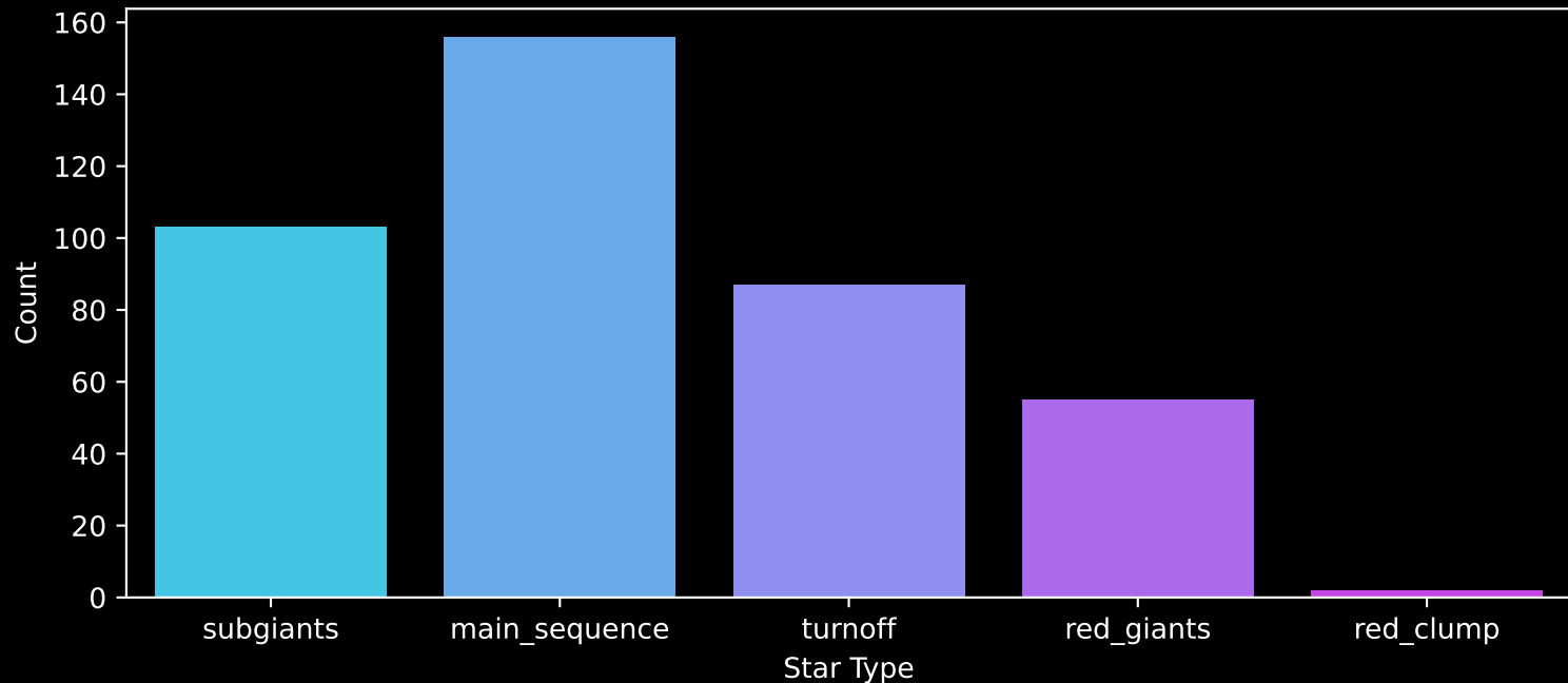
Gaia Cluster: [NGC_654] Count plot of Star Type
