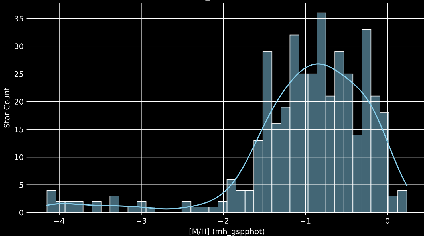
Gaia Cluster: [NGC_654 [M/H] (mh_gspphot) (n= 403)
