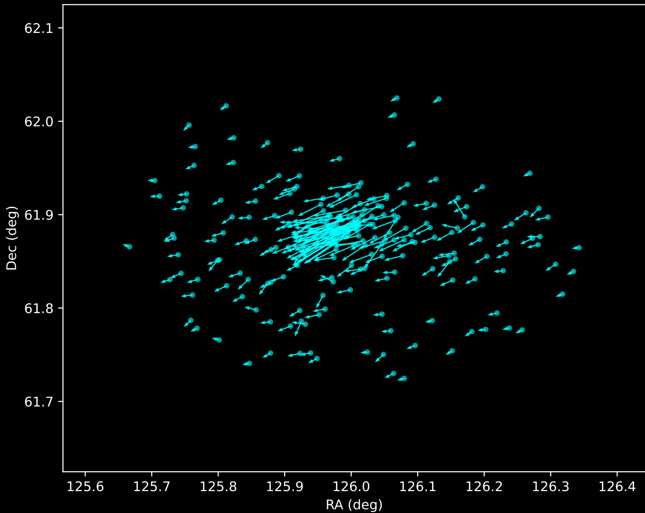
Gaia DR3 Noise Stream Proper Motion Vectors (n=222)
