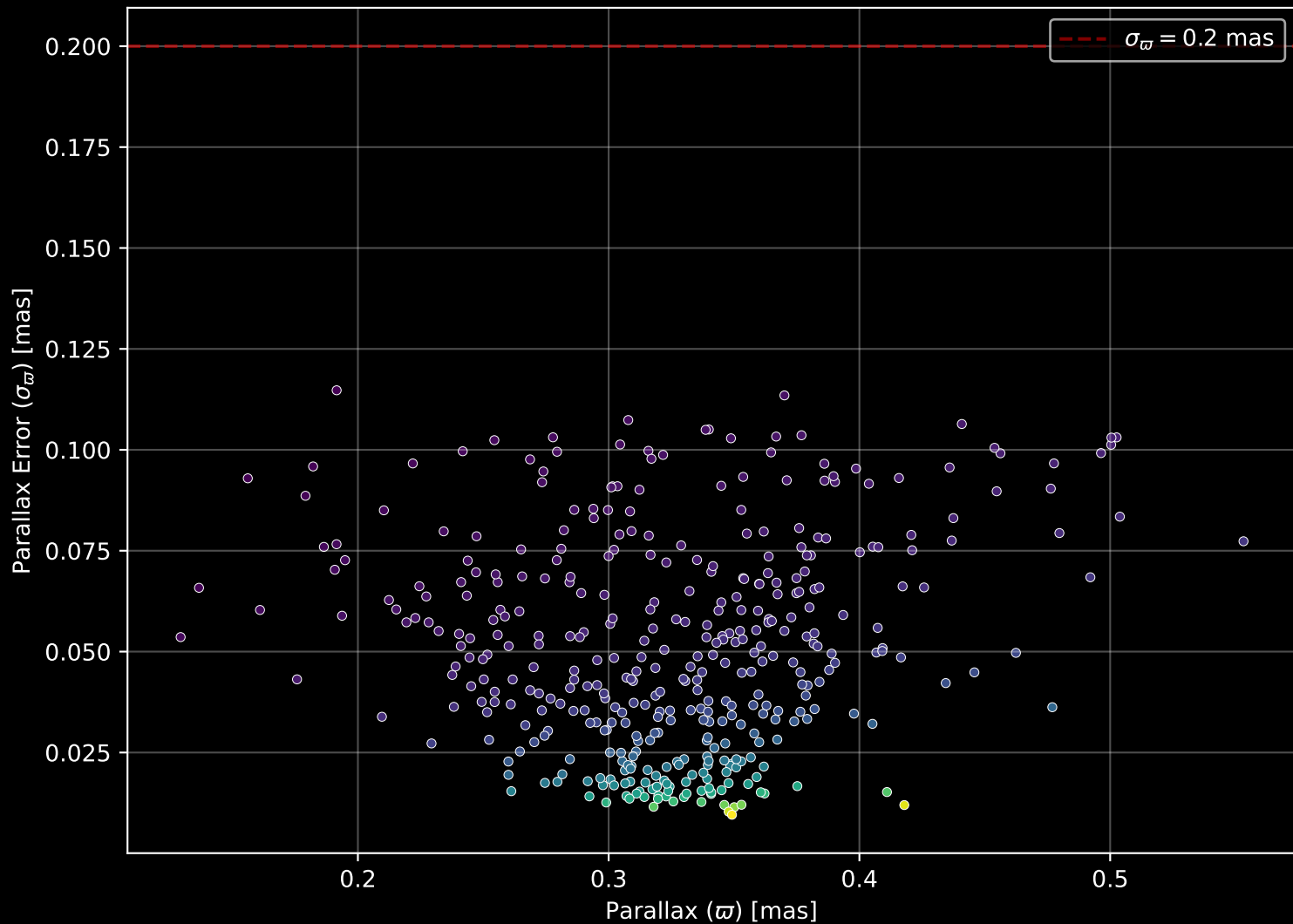
Gaia Cluster: [NGC_654] Parallax Quality (n= 403)
