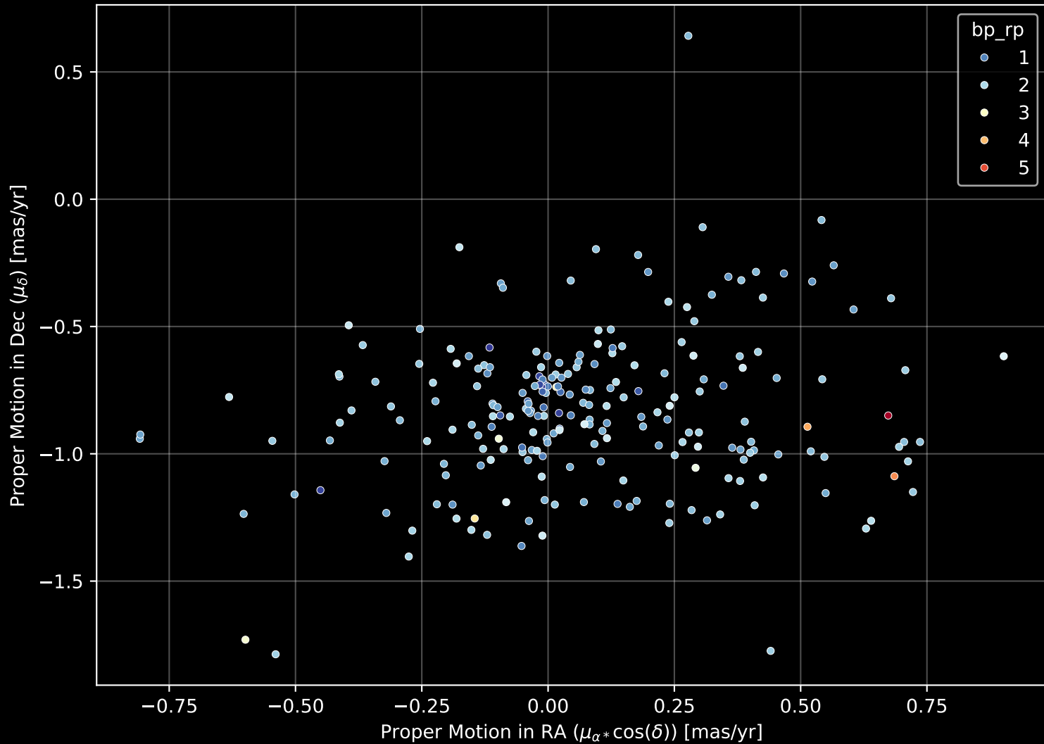
Gaia Cluster: [NGC_6561] Proper Motion Diagram (n= 227)
