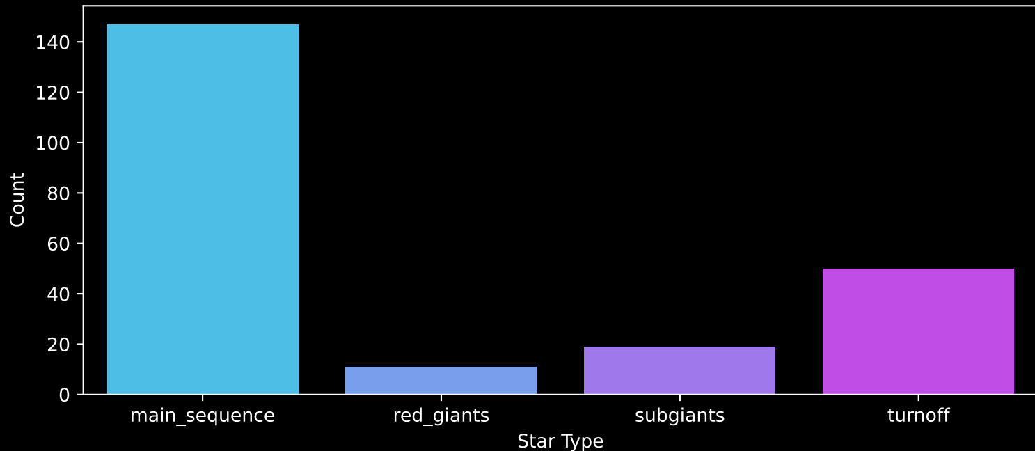
Gaia Cluster: [NGC_6561] Count plot of Star Type
