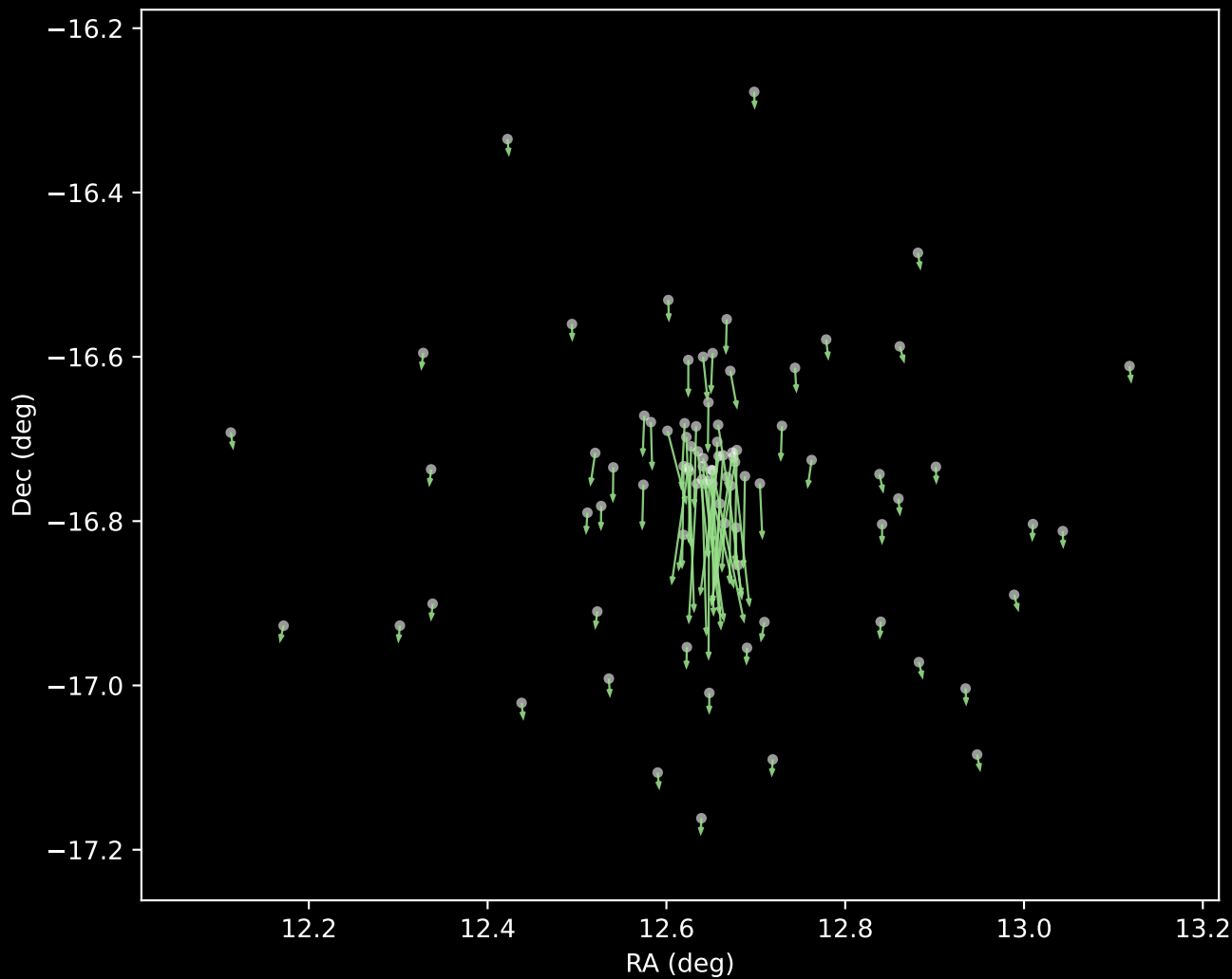
Gaia DR3 Cluster 5 Proper Motion Vectors (n=86)
