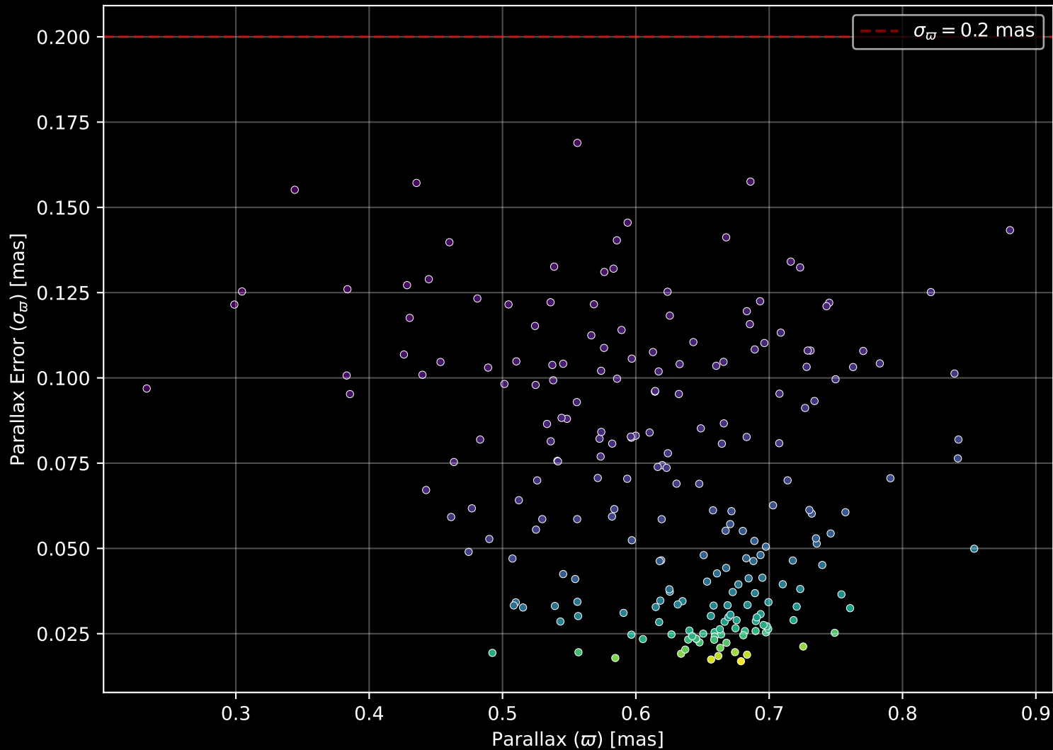
Gaia Cluster: [NGC_6561] Parallax Quality (n= 227)
