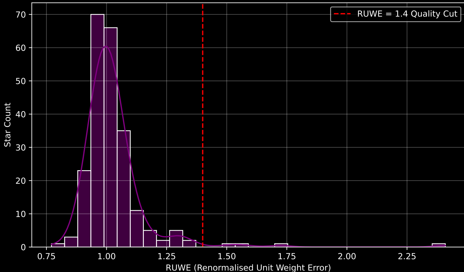
Gaia Cluster: [NGC_6561] RUWE Distribution (n= 227)
