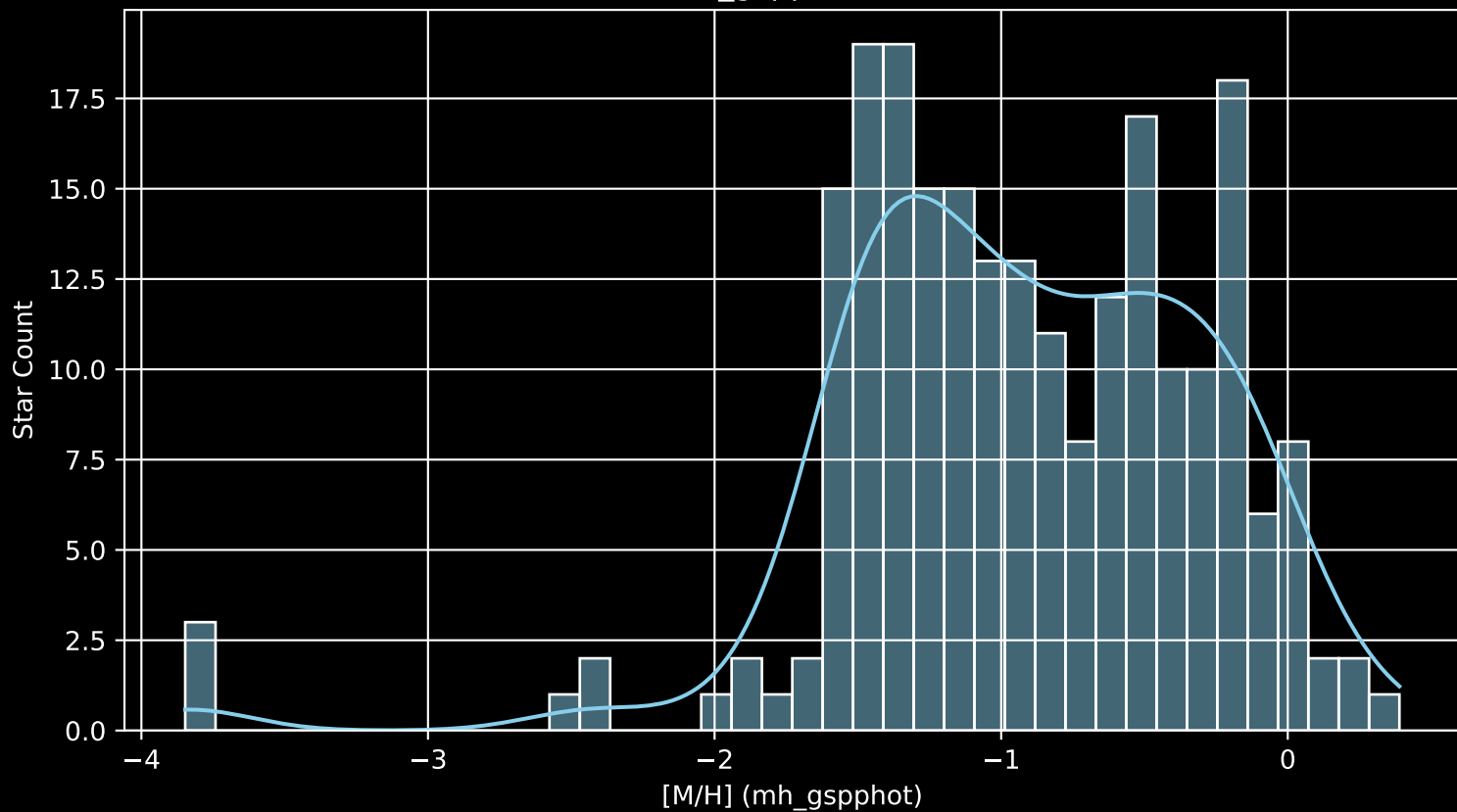
Gaia Cluster: [NGC_6561 [M/H] (mh_gspphot) (n= 226)
