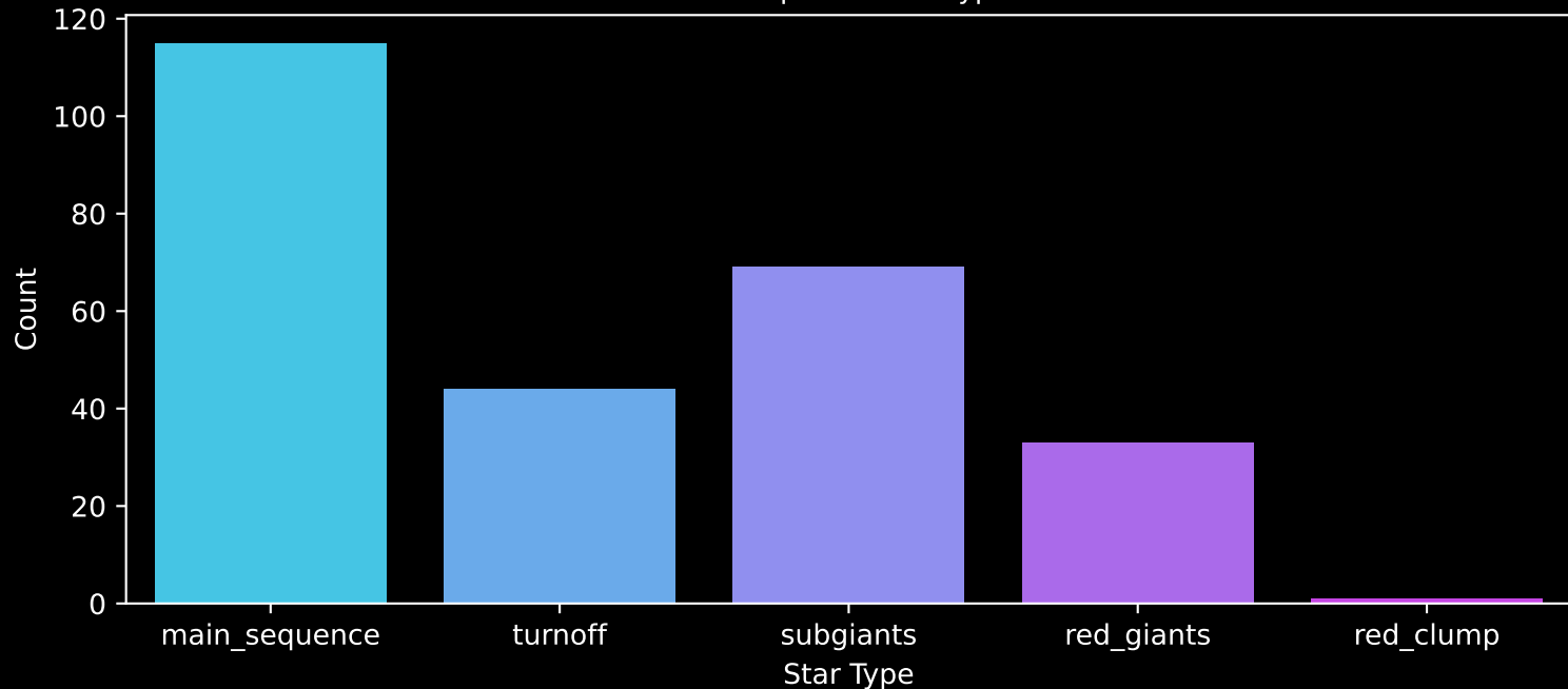
Gaia Cluster: [NGC_659] Count plot of Star Type
