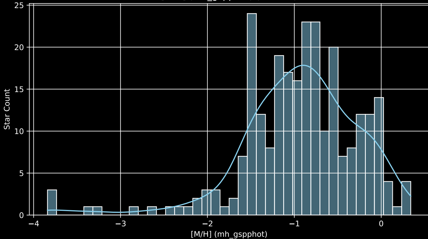
Gaia Cluster: [NGC_659 [M/H] (mh_gspphot) (n= 262)
