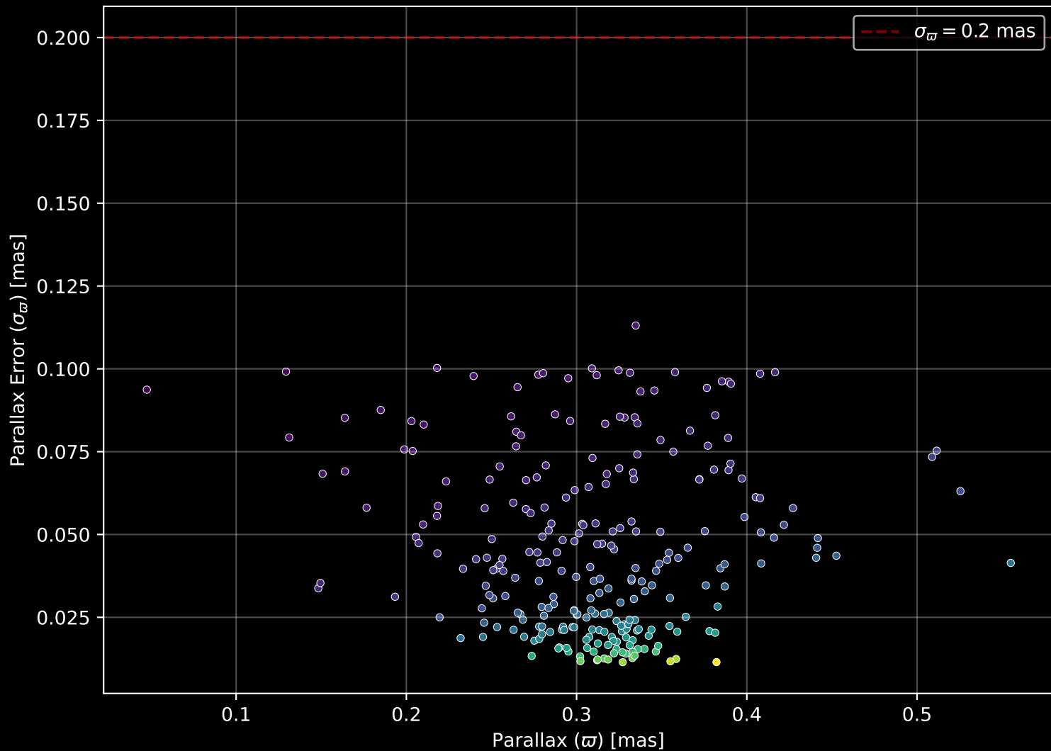
Gaia Cluster: [NGC_659] Parallax Quality (n= 262)
