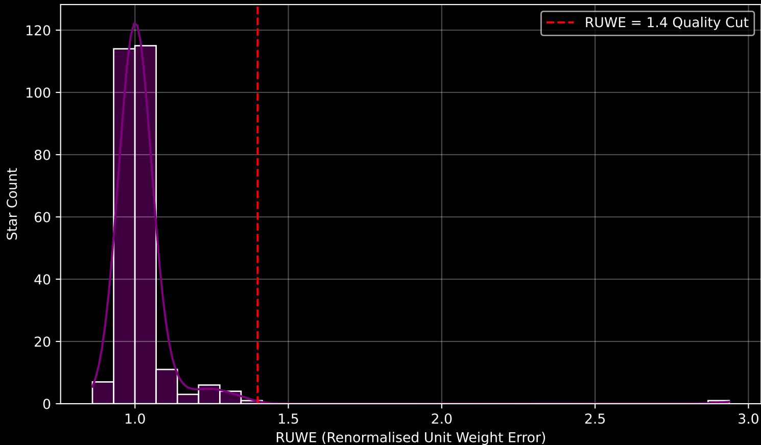
Gaia Cluster: [NGC_659] RUWE Distribution (n= 262)
