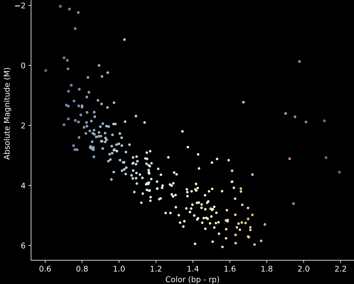
Gaia Cluster: [NGC_659] Stars (n= 262) Hertzsprung-Russel Diagram
