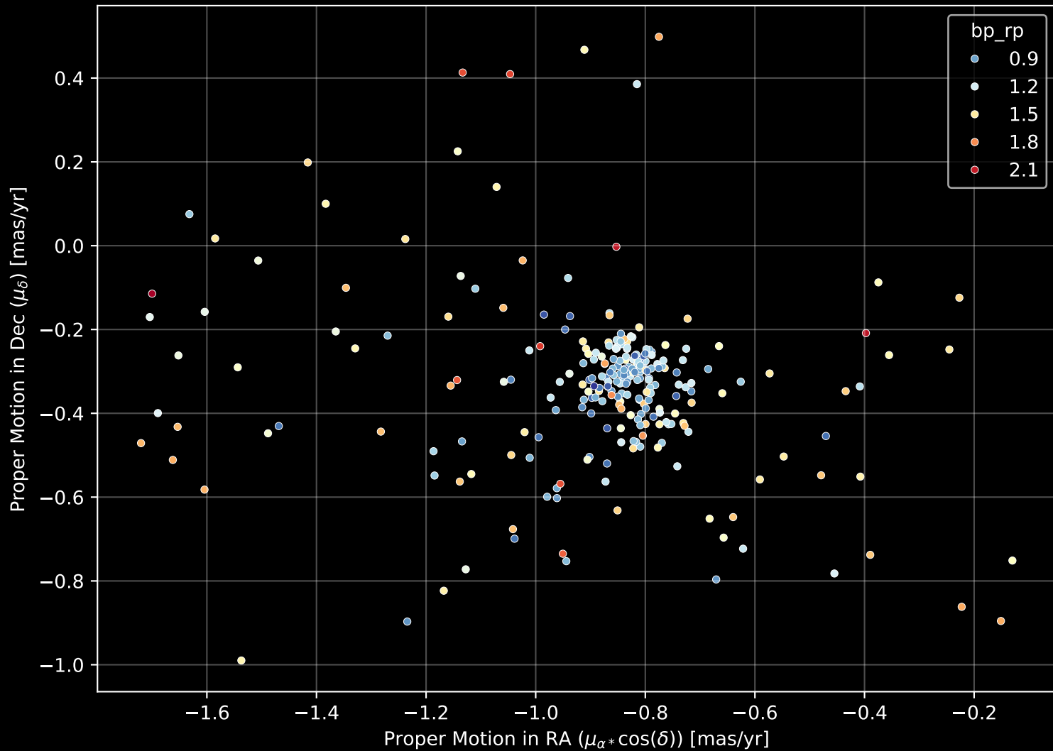
Gaia Cluster: [NGC_659] Proper Motion Diagram (n= 262)
