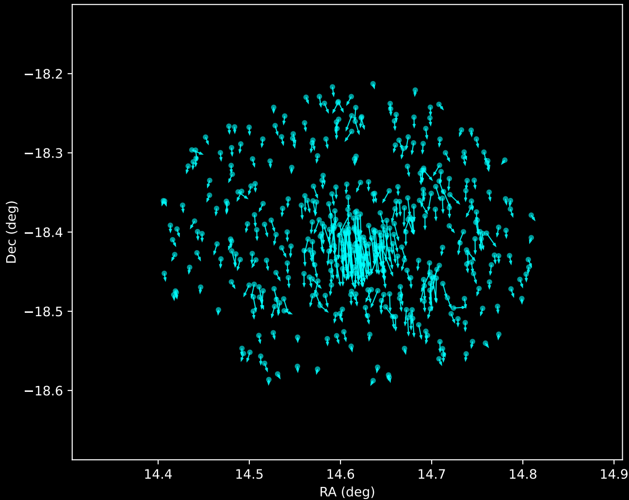
Gaia DR3 Noise Stream Proper Motion Vectors (n=429)
