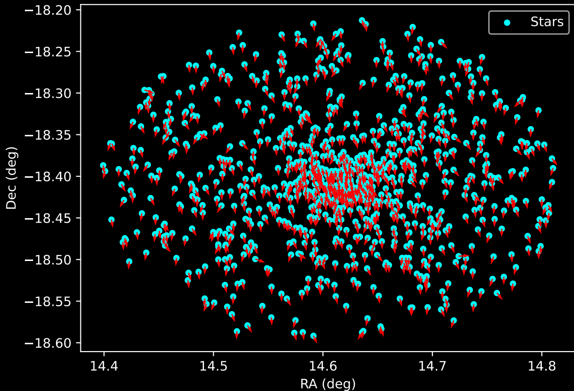
Gaia Cluster: [NGC_6603] Proper Motion Vectors for Gaia Star Field (n= 948)
