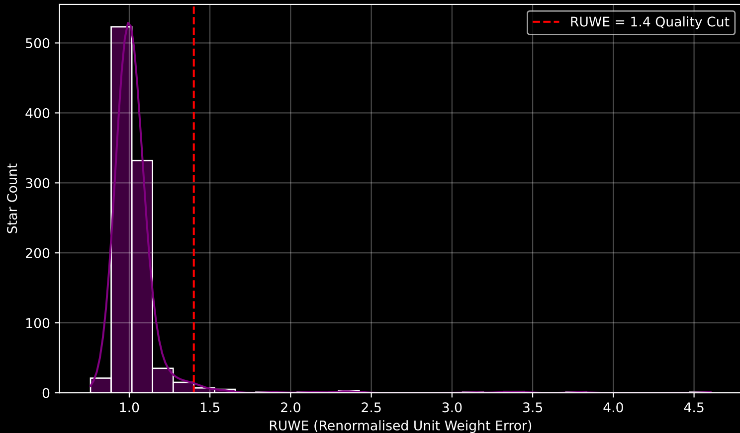
Gaia Cluster: [NGC_6603] RUWE Distribution (n= 948)
