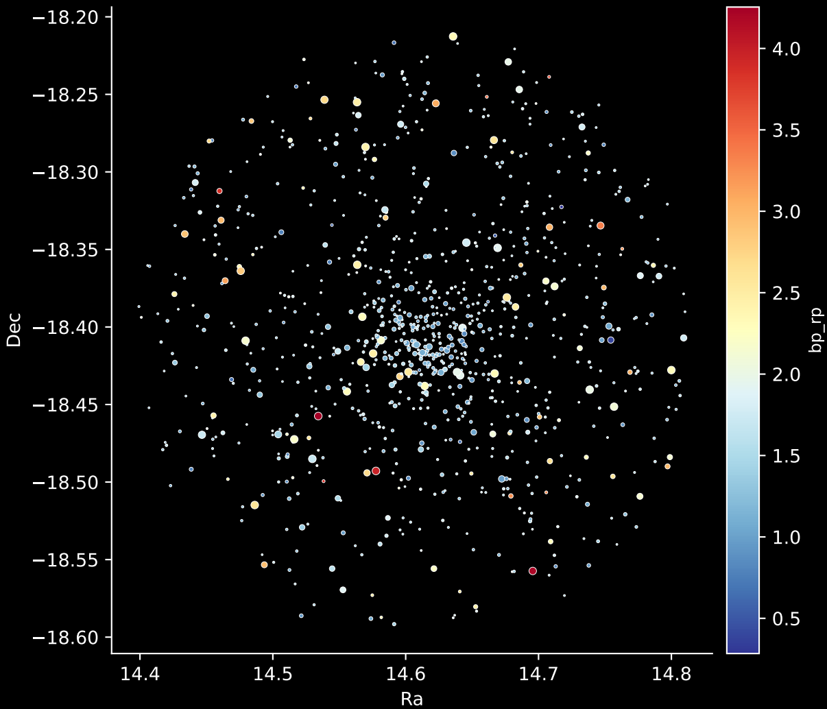
Gaia Cluster: [NGC_6603] Stars: 948
