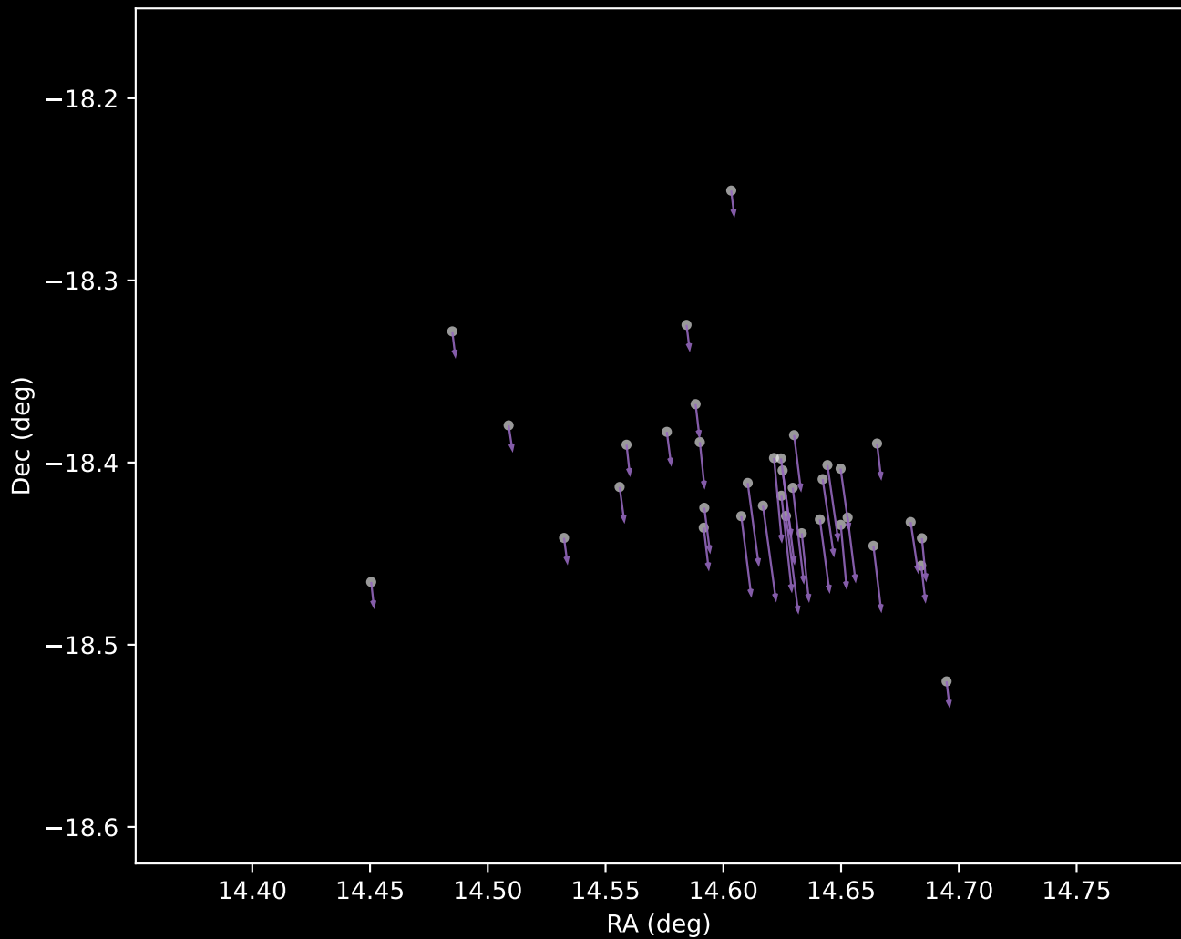
Gaia DR3 Cluster 48 Proper Motion Vectors (n=36)
