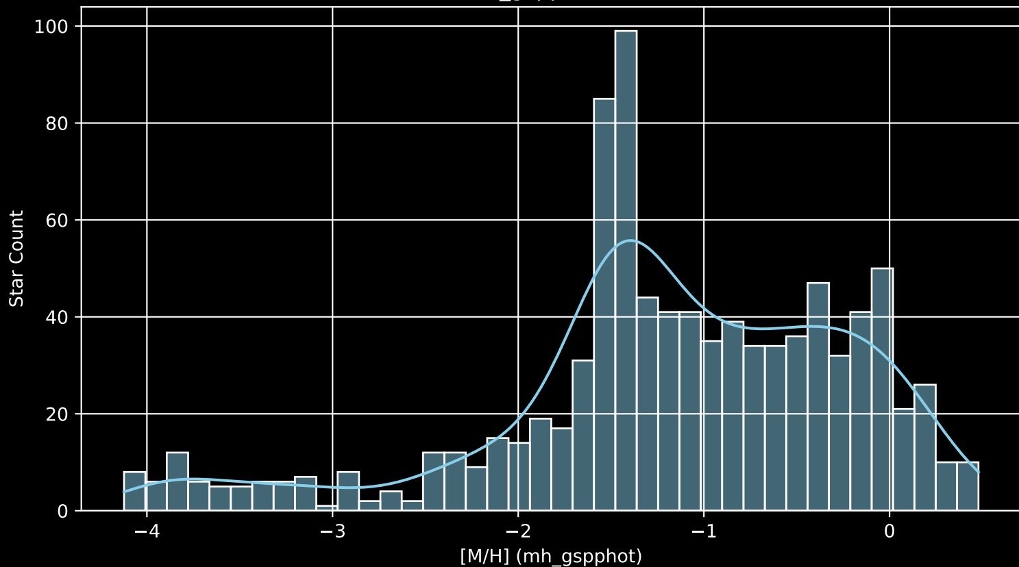
Gaia Cluster: [NGC_6603 [M/H] (mh_gspphot) (n= 932)
