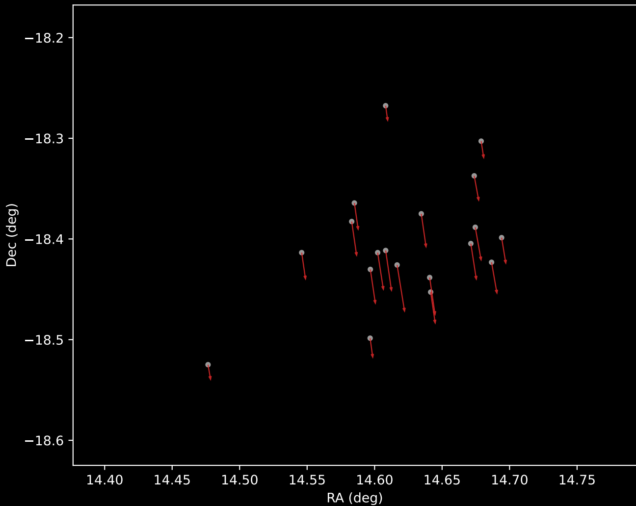
Gaia DR3 Cluster 46 Proper Motion Vectors (n=19)
