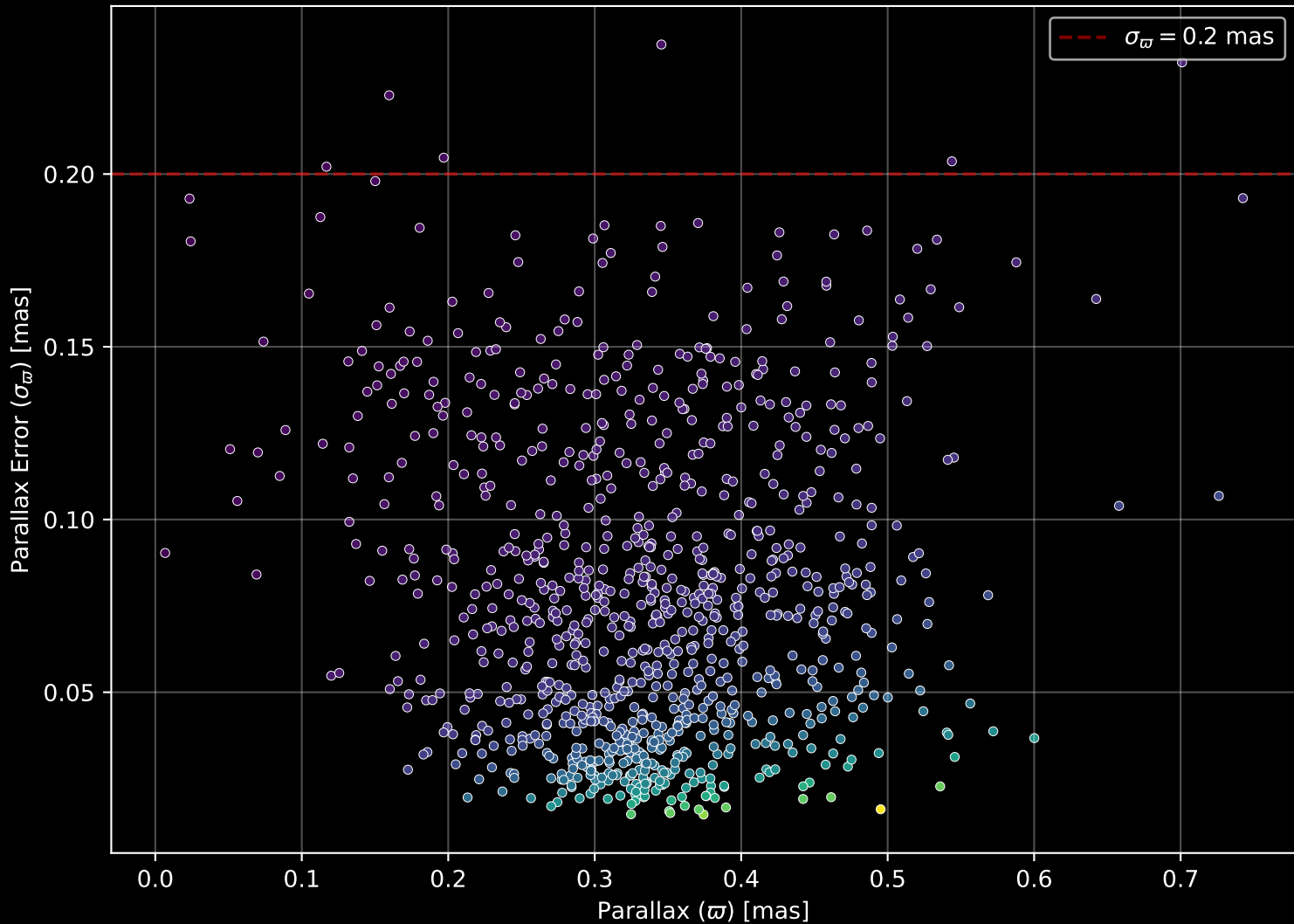
Gaia Cluster: [NGC_6603] Parallax Quality (n= 948)
