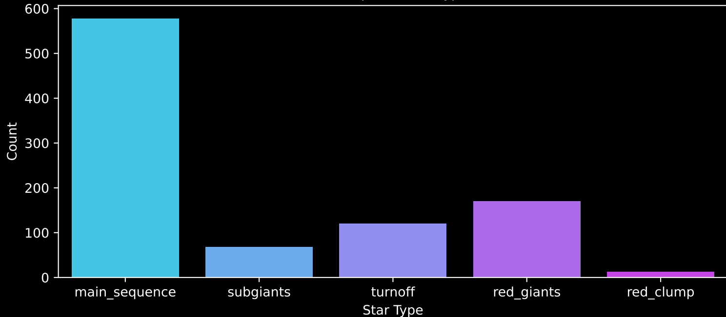
Gaia Cluster: [NGC_6603] Count plot of Star Type
