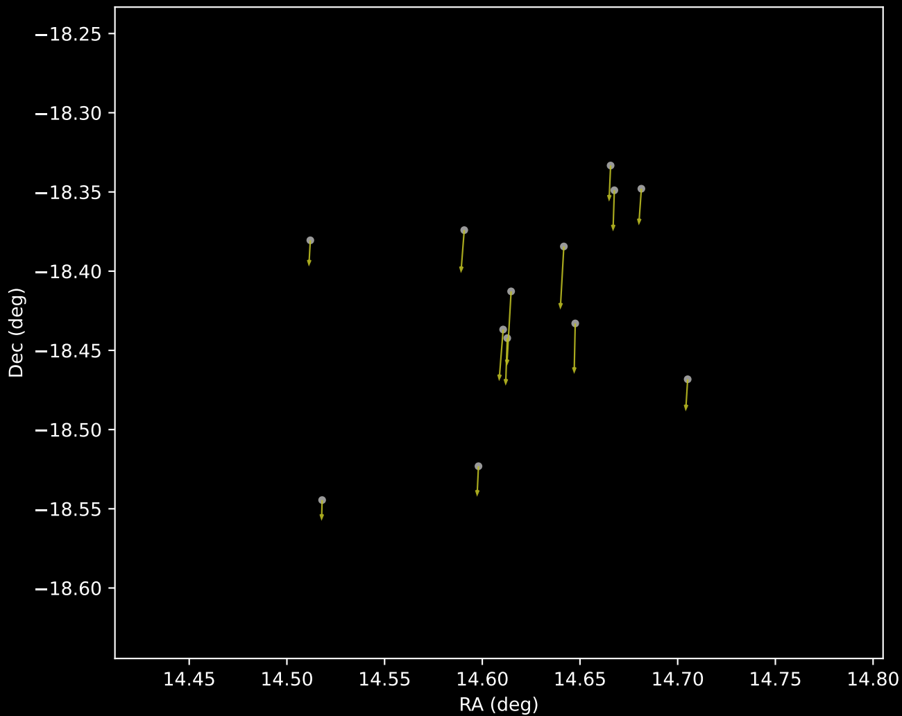
Gaia DR3 Cluster 36 Proper Motion Vectors (n=13)
