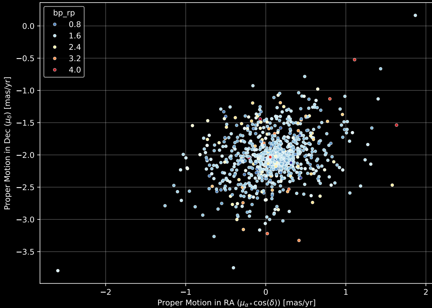
Gaia Cluster: [NGC_6603] Proper Motion Diagram (n= 948)
