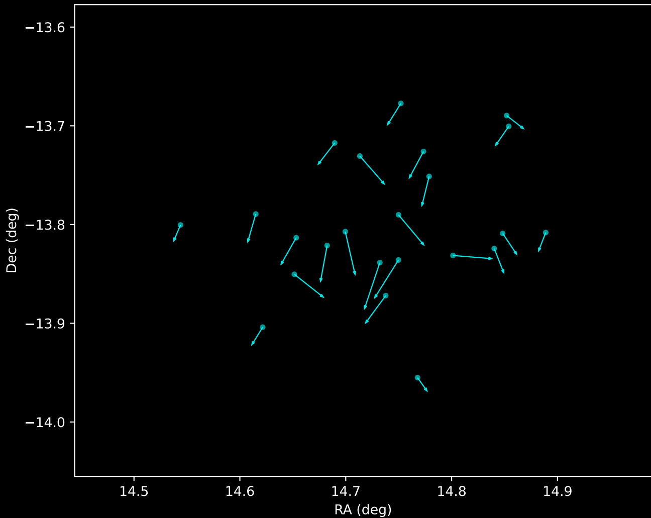
Gaia DR3 Noise Stream Proper Motion Vectors (n=23)
