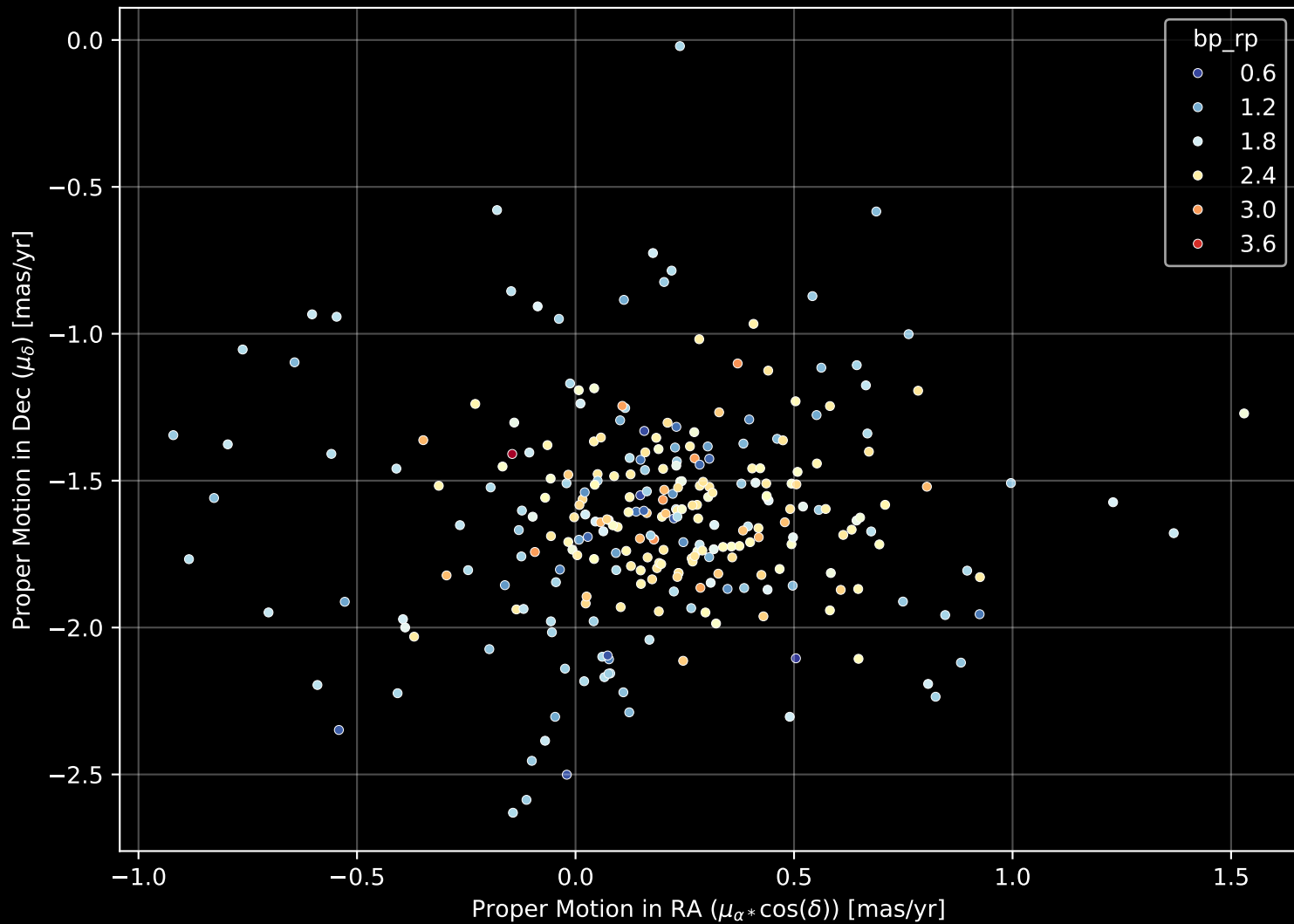
Gaia Cluster: [NGC_6611] Proper Motion Diagram (n= 278)
