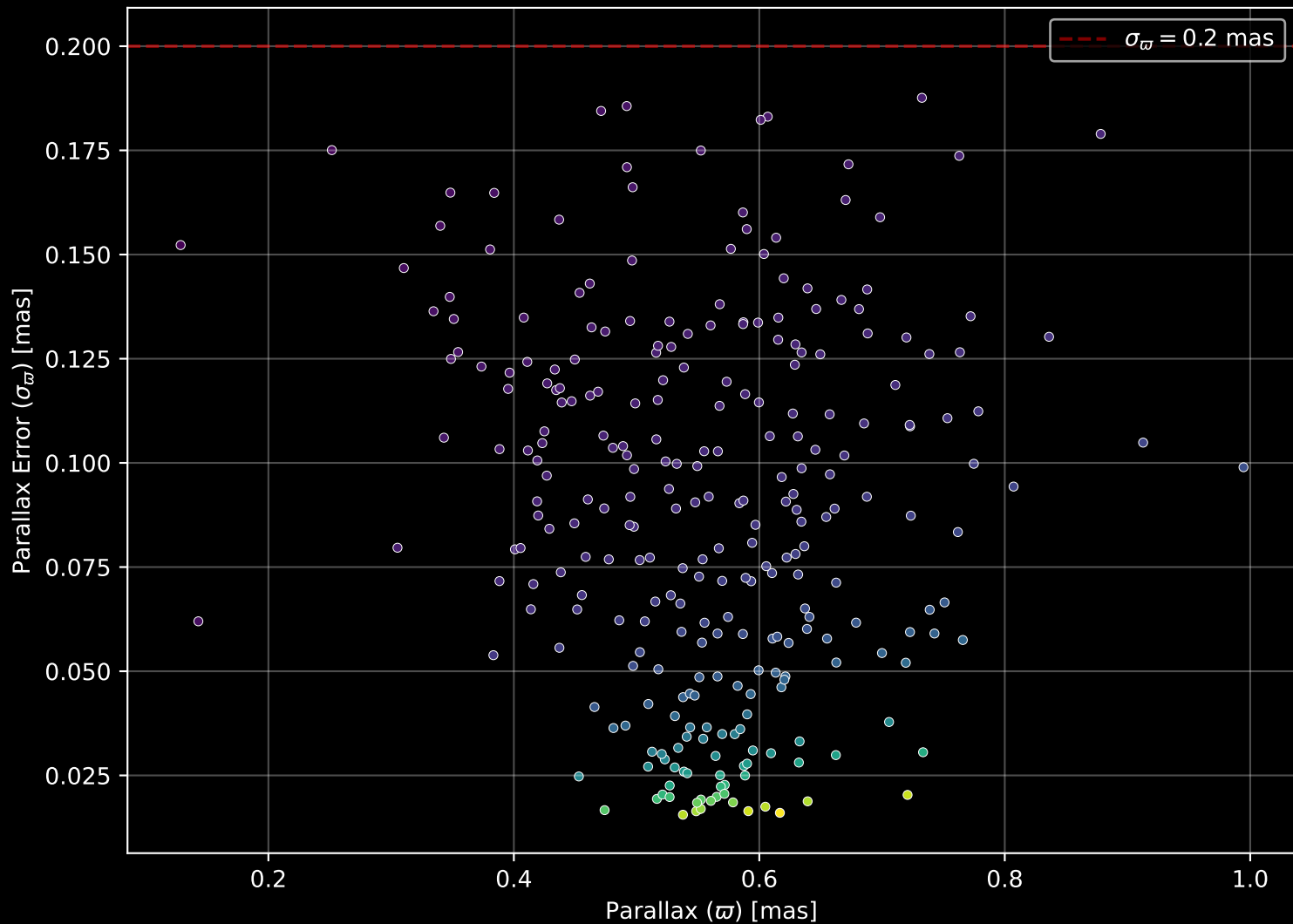
Gaia Cluster: [NGC_6611] Parallax Quality (n= 278)
