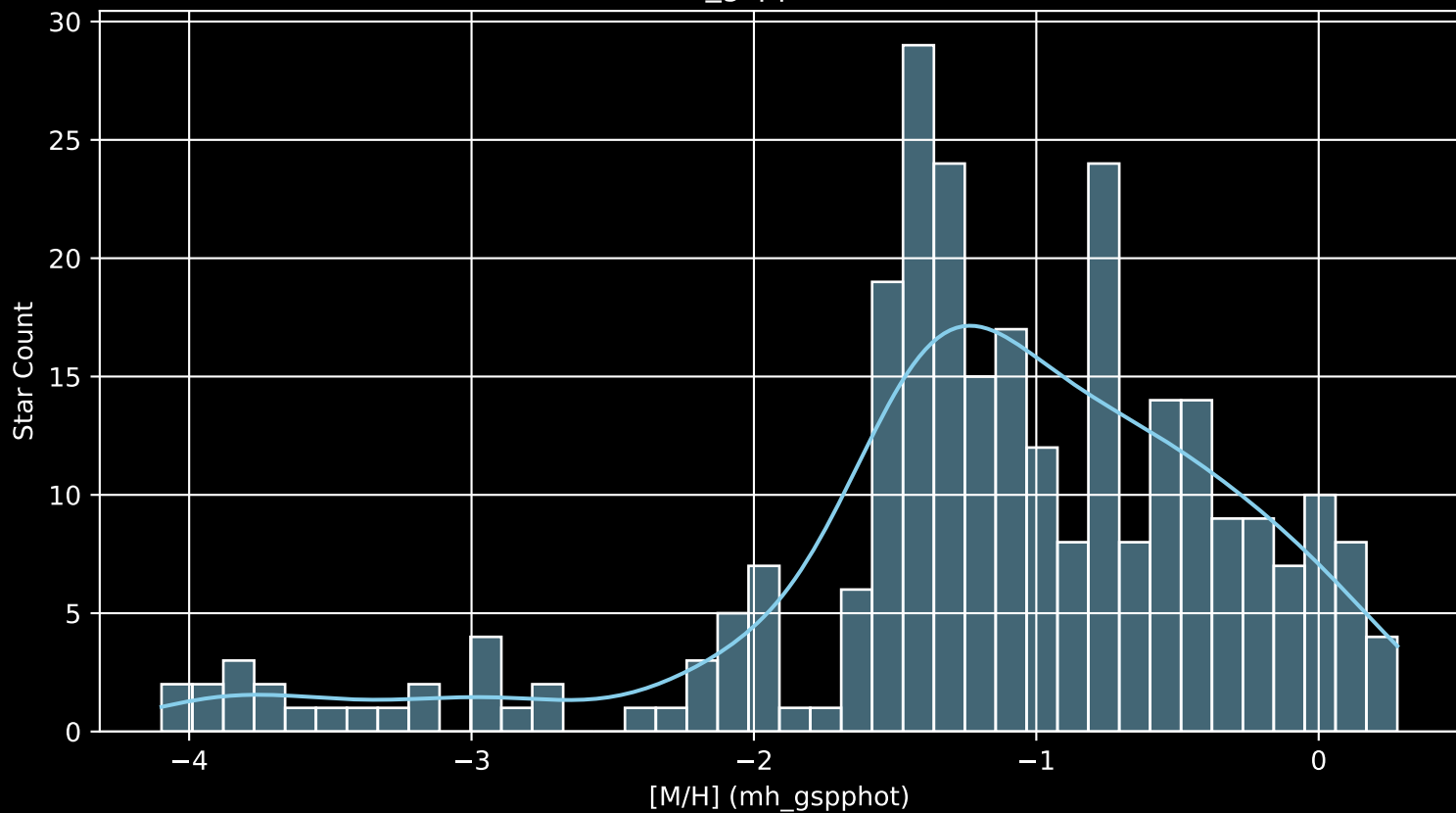
Gaia Cluster: [NGC_6611 [M/H] (mh_gspphot) (n= 278)
