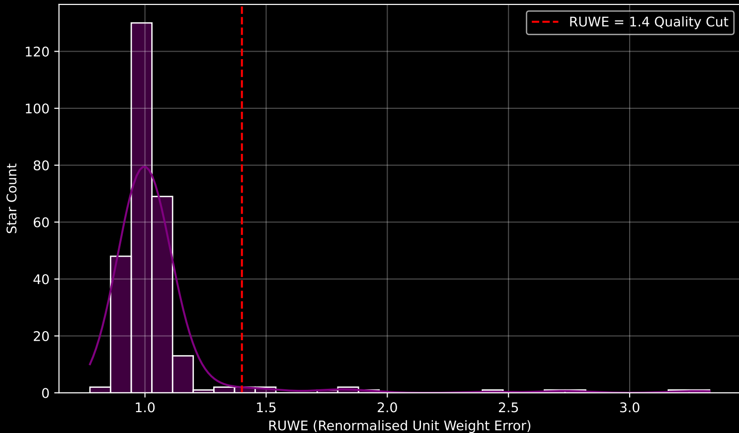
Gaia Cluster: [NGC_6611] RUWE Distribution (n= 278)
