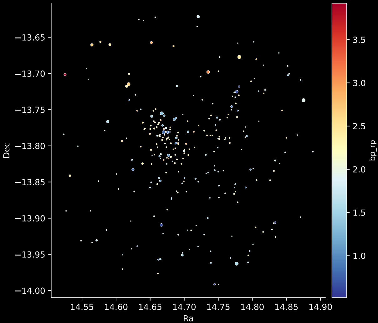
Gaia Cluster: [NGC_6611] Stars: 278
