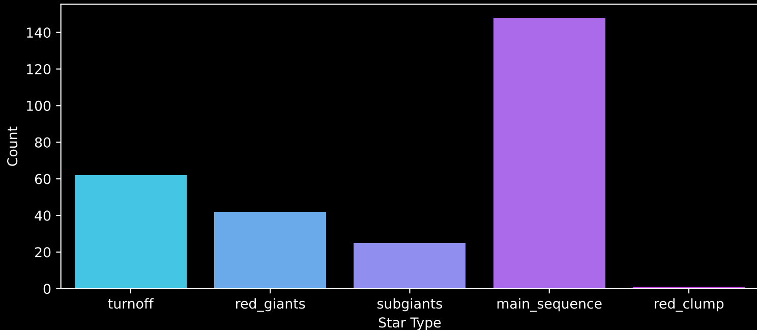
Gaia Cluster: [NGC_6611] Count plot of Star Type
