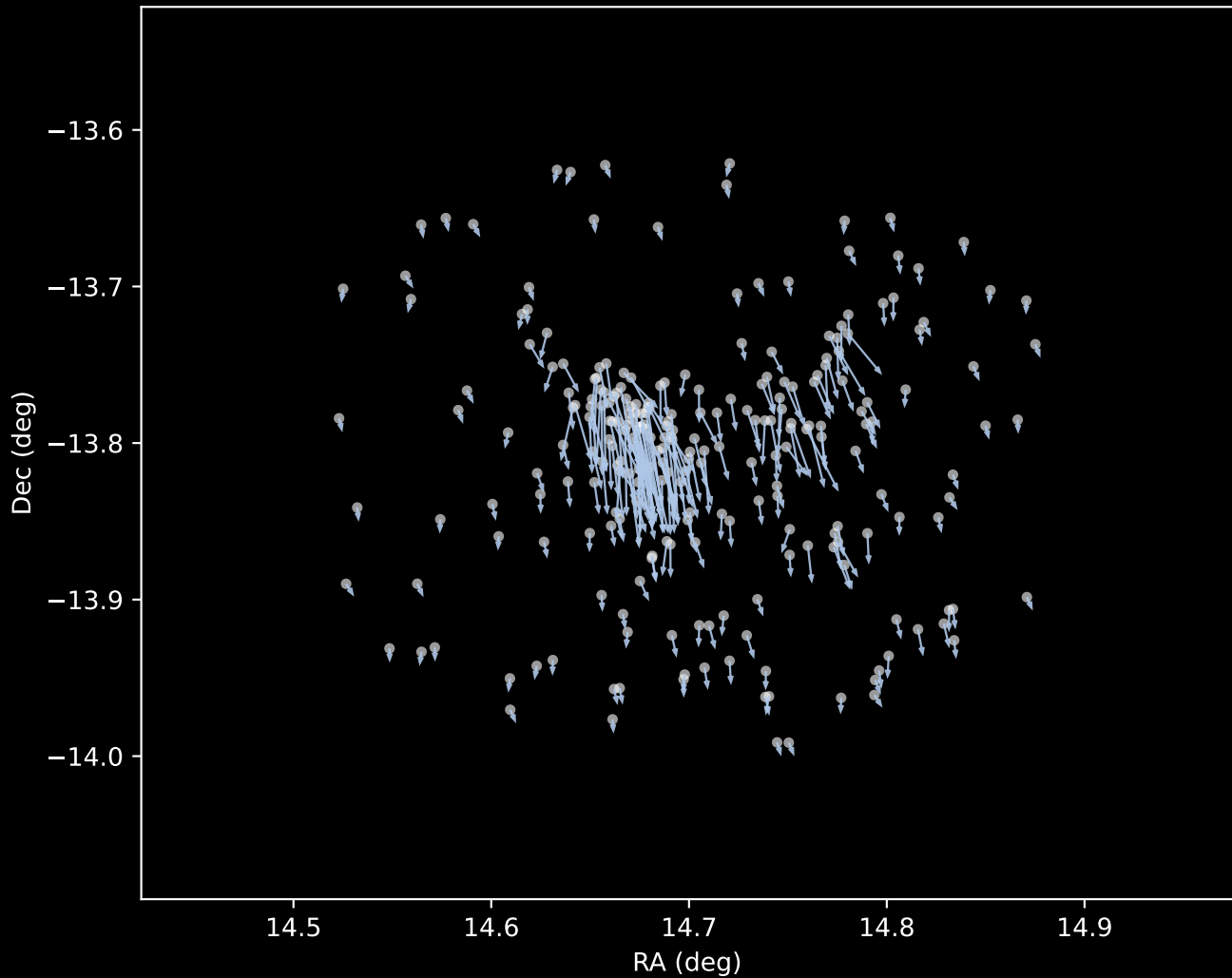
Gaia DR3 Cluster 1 Proper Motion Vectors (n=249)
