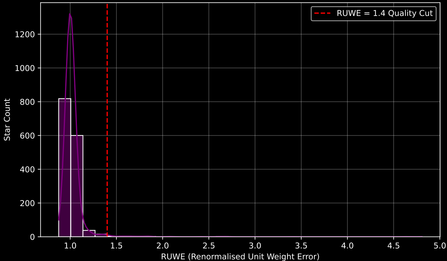
Gaia Cluster: [NGC_663] RUWE Distribution (n= 1494)
