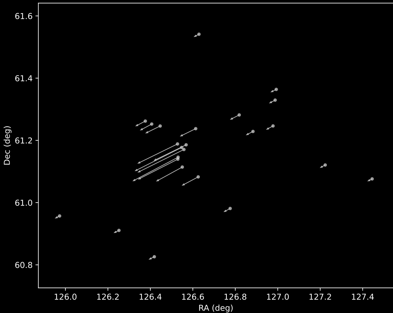
Gaia DR3 Cluster 55 Proper Motion Vectors (n=24)
