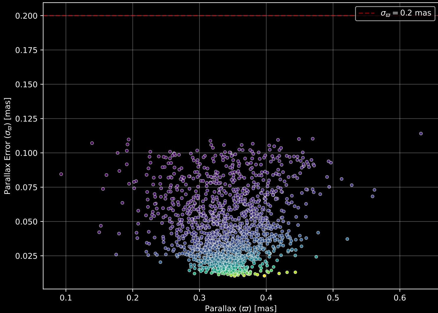
Gaia Cluster: [NGC_663] Parallax Quality (n= 1494)
