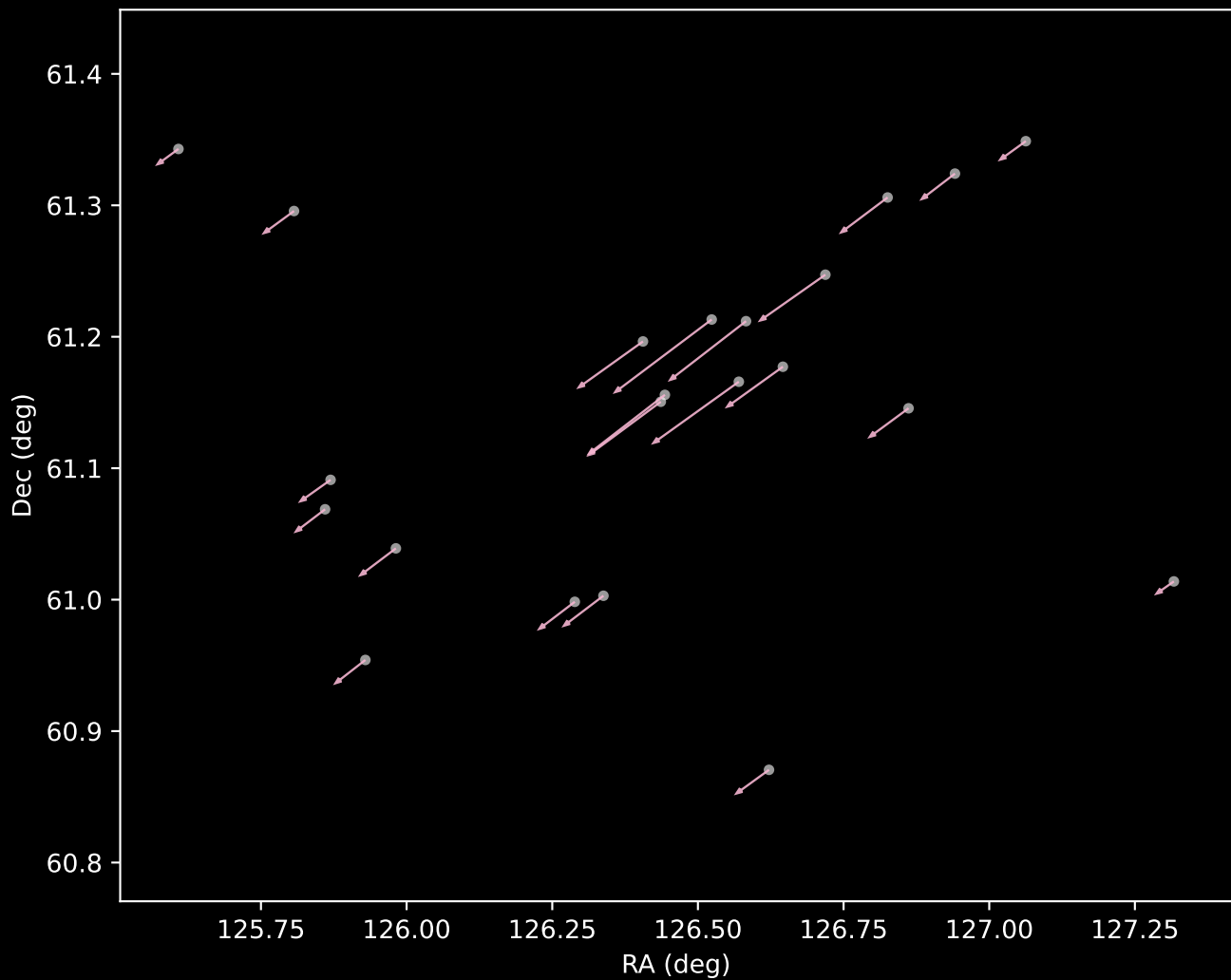
Gaia DR3 Cluster 33 Proper Motion Vectors (n=22)
