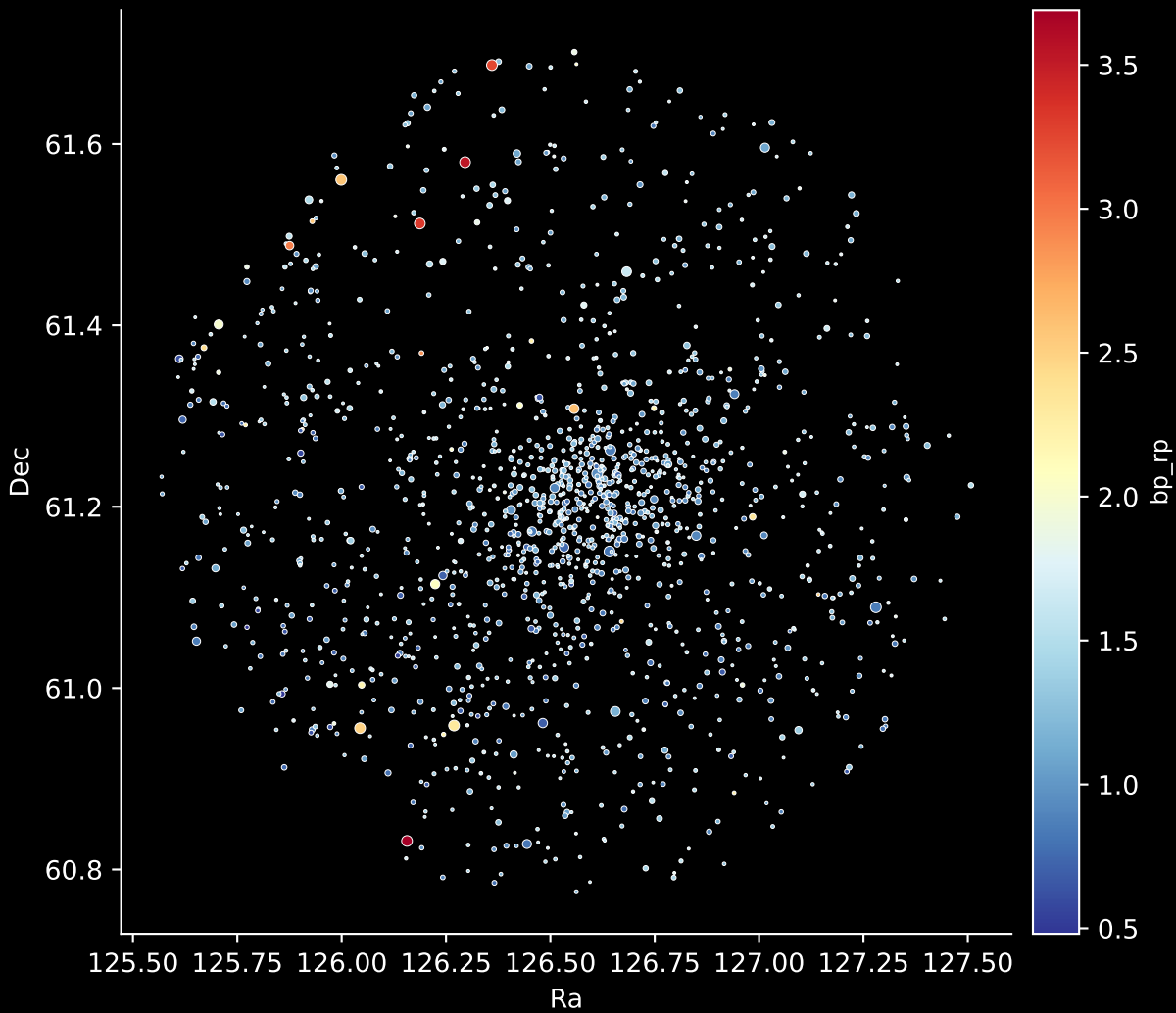
Gaia Cluster: [NGC_663] Stars: 1494
