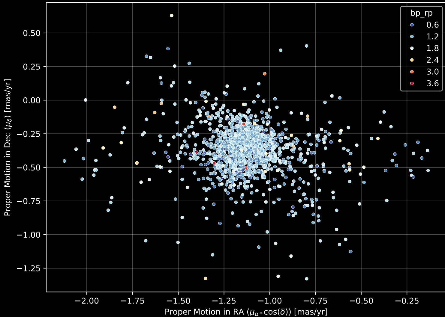
Gaia Cluster: [NGC_663] Proper Motion Diagram (n= 1494)
