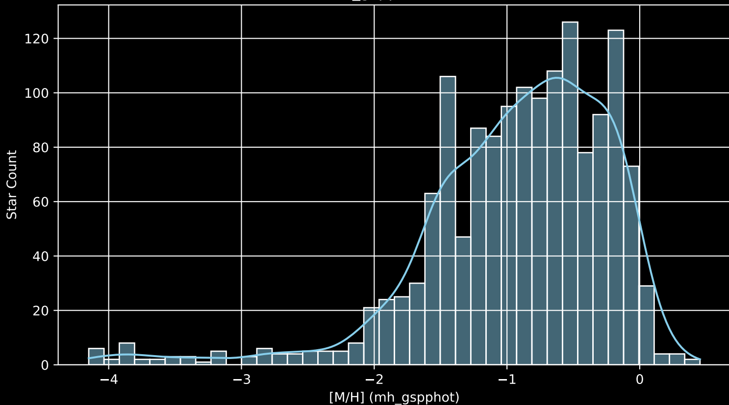
Gaia Cluster: [NGC_663 [M/H] (mh_gspphot) (n= 1493)
