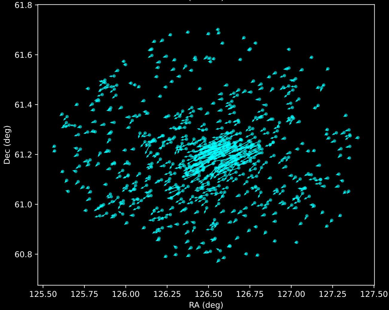
Gaia DR3 Noise Stream Proper Motion Vectors (n=664)
