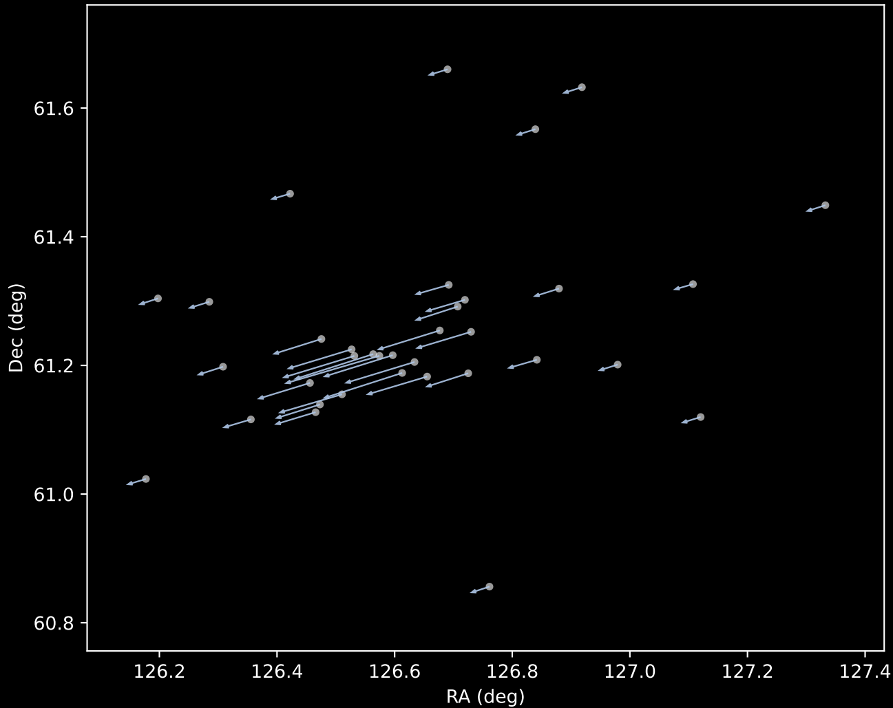
Gaia DR3 Cluster 81 Proper Motion Vectors (n=35)
