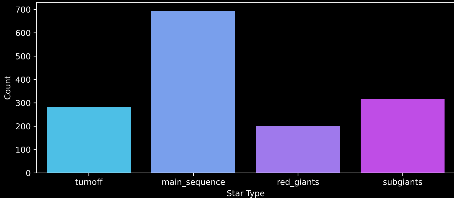
Gaia Cluster: [NGC_663] Count plot of Star Type
