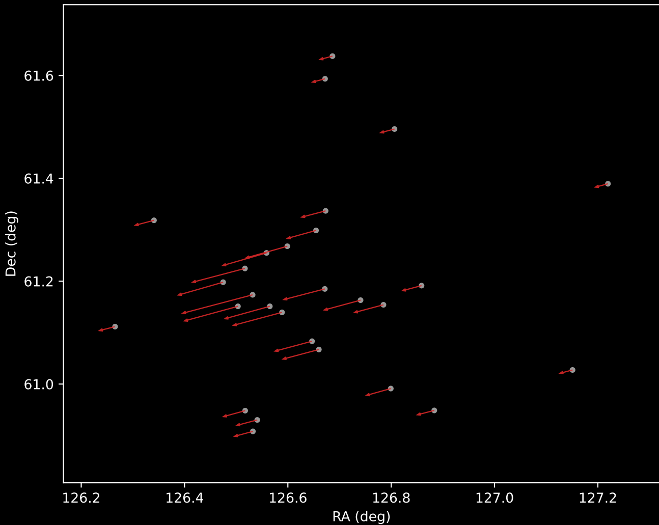
Gaia DR3 Cluster 66 Proper Motion Vectors (n=28)
