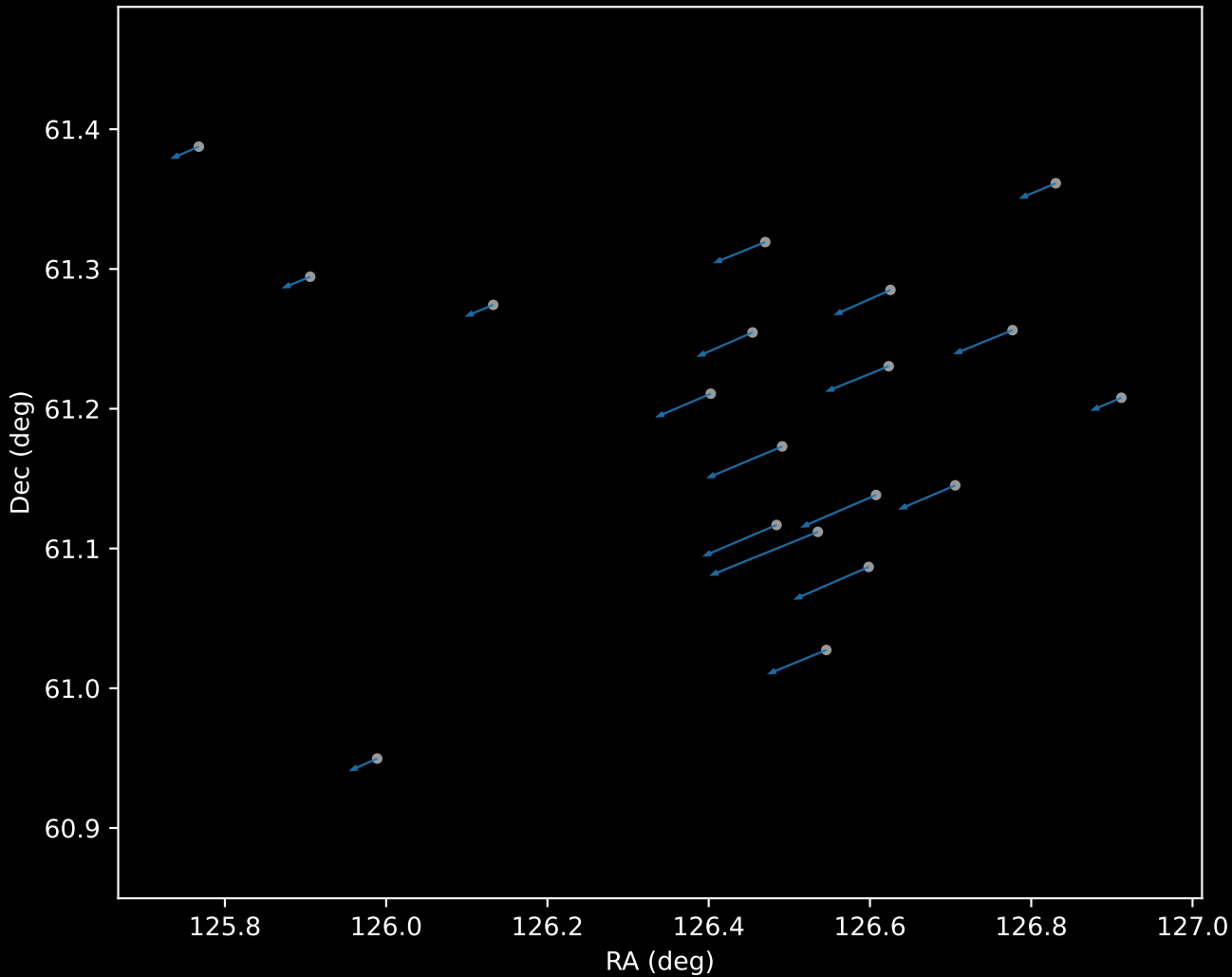
Gaia DR3 Cluster 60 Proper Motion Vectors (n=19)
