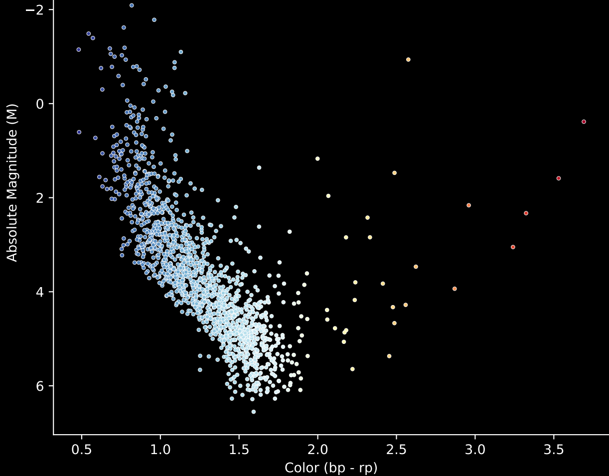
Gaia Cluster: [NGC_663] Stars (n= 1494) Hertzsprung-Russel Diagram
