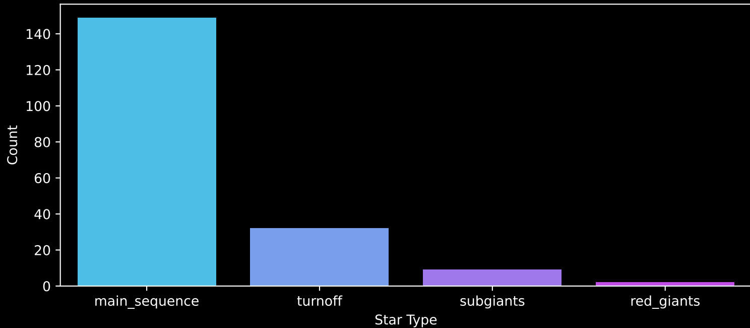
Gaia Cluster: [NGC_6633] Count plot of Star Type
