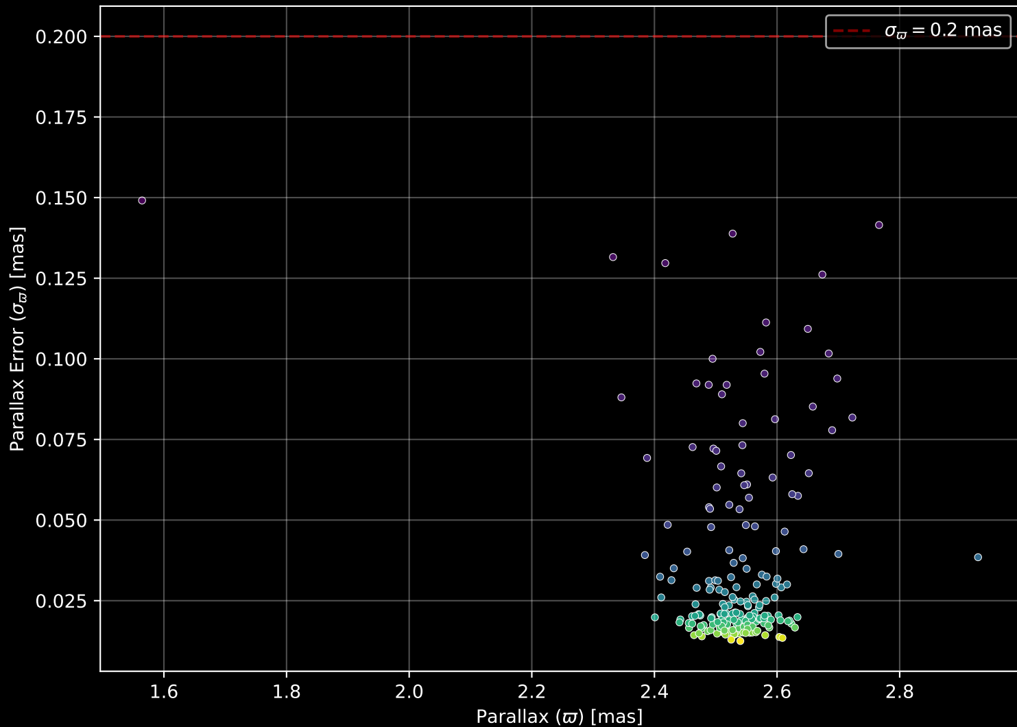
Gaia Cluster: [NGC_6633] Parallax Quality (n= 192)
