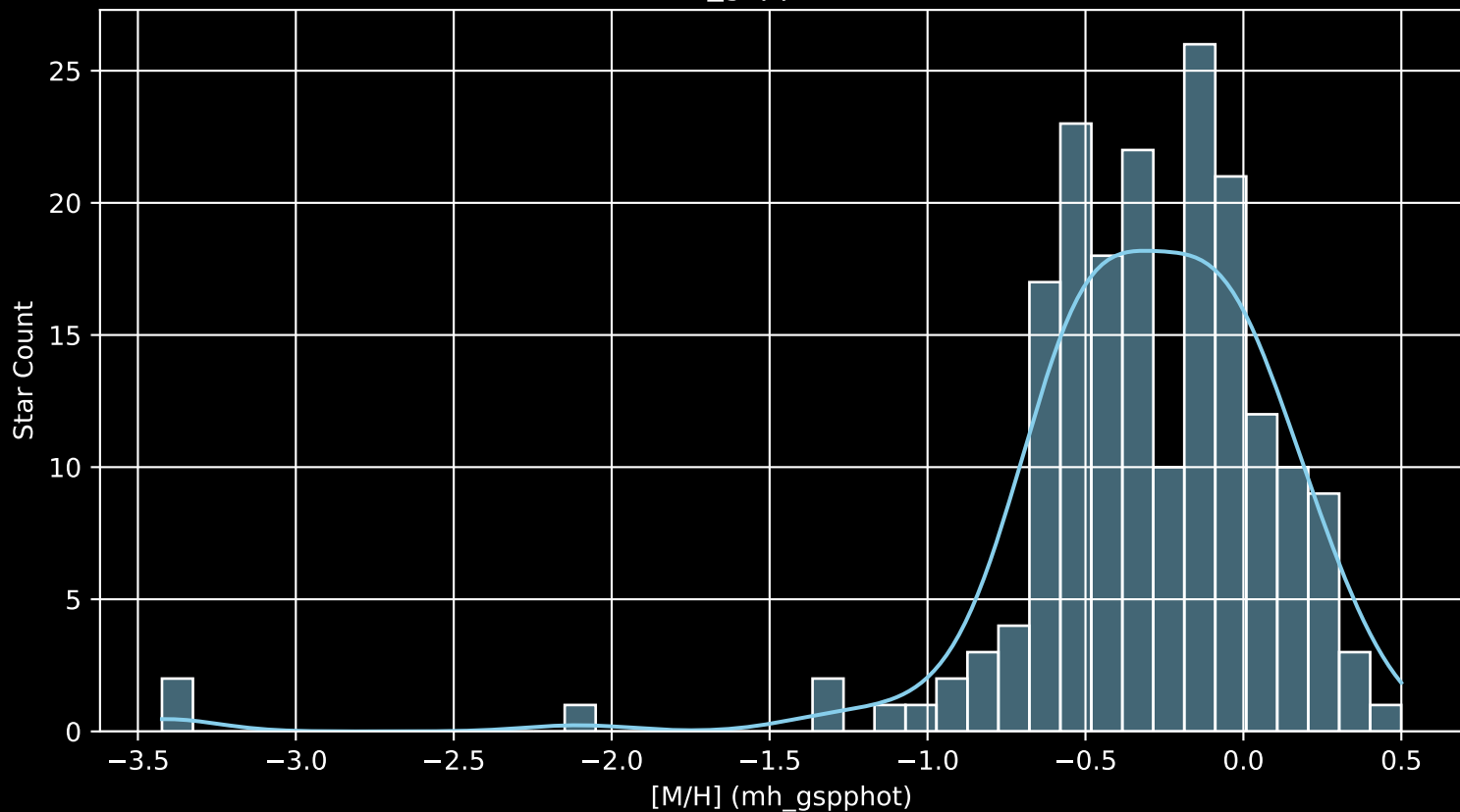
Gaia Cluster: [NGC_6633 [M/H] (mh_gspphot) (n= 188)
