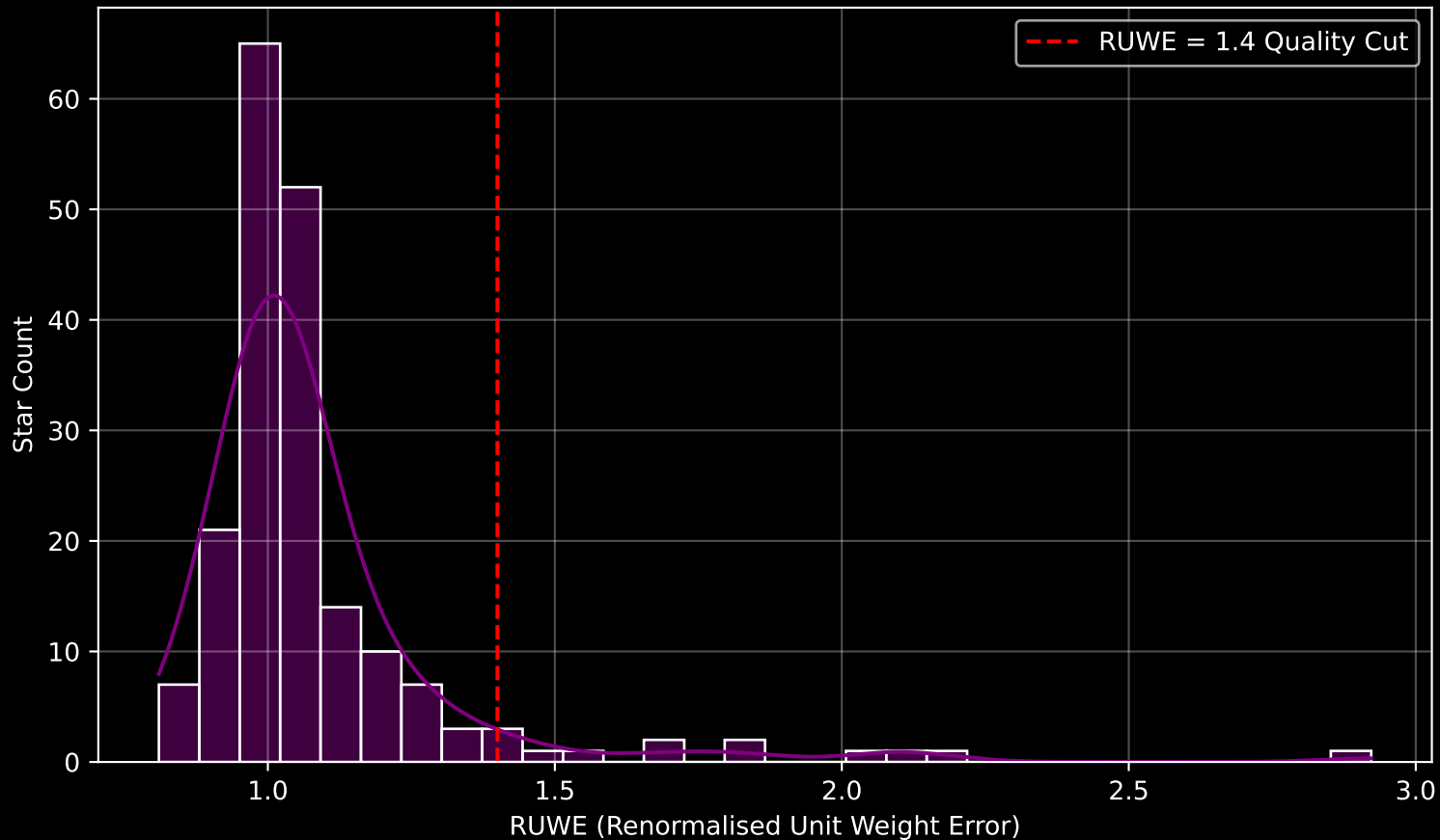
Gaia Cluster: [NGC_6633] RUWE Distribution (n= 192)
