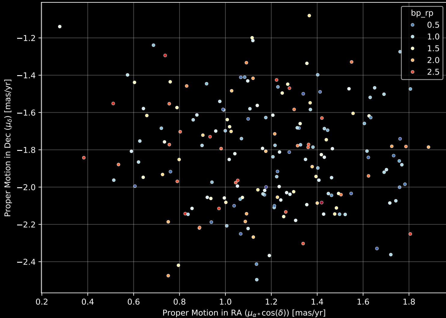
Gaia Cluster: [NGC_6633] Proper Motion Diagram (n= 192)
