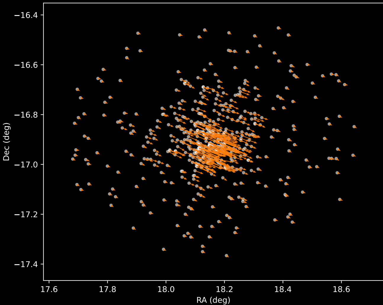
Gaia DR3 Cluster 22 Proper Motion Vectors (n=486)
