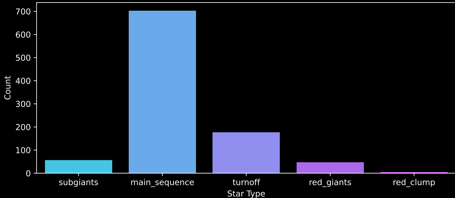
Gaia Cluster: [NGC_6645] Count plot of Star Type
