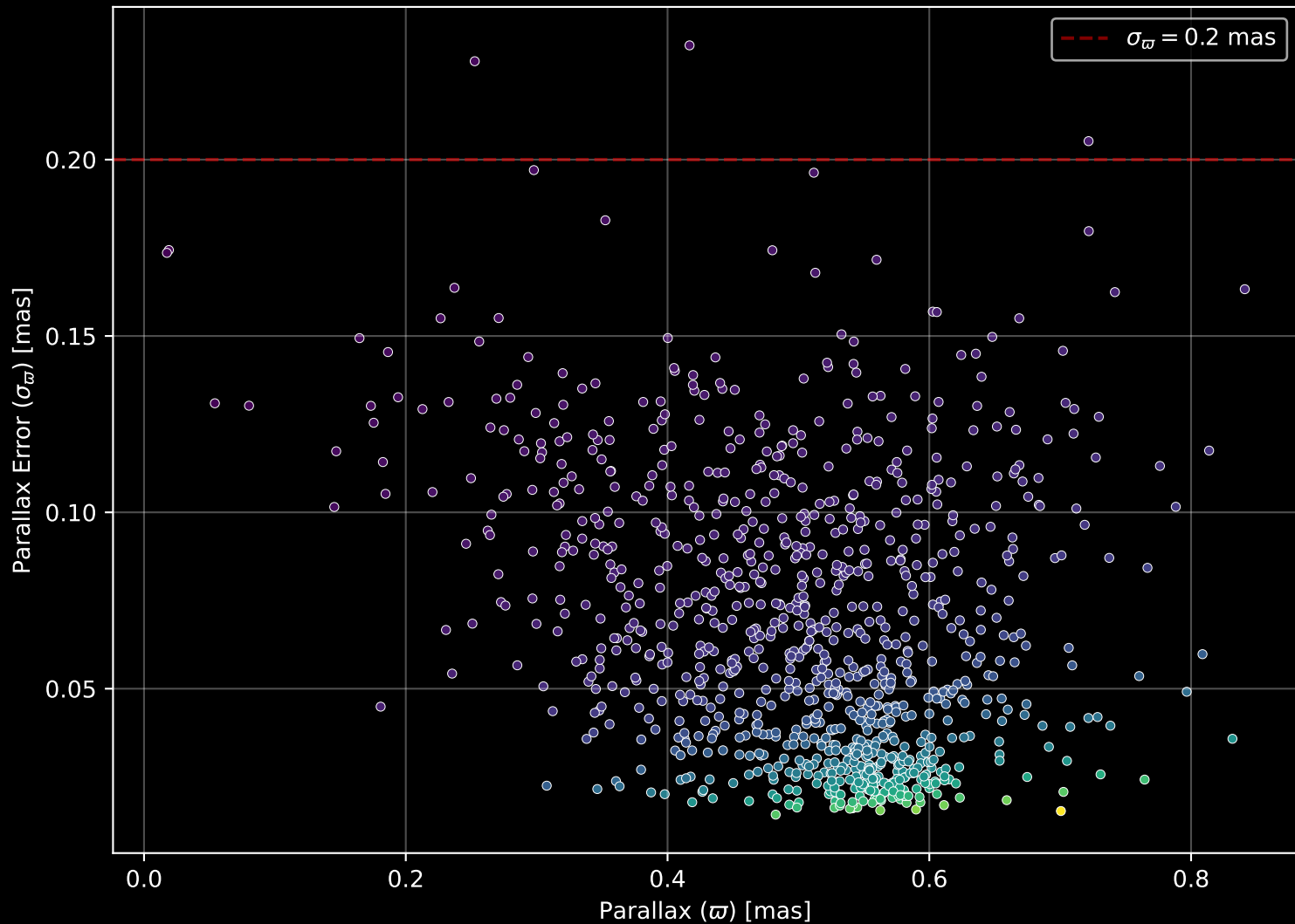
Gaia Cluster: [NGC_6645] Parallax Quality (n= 988)
