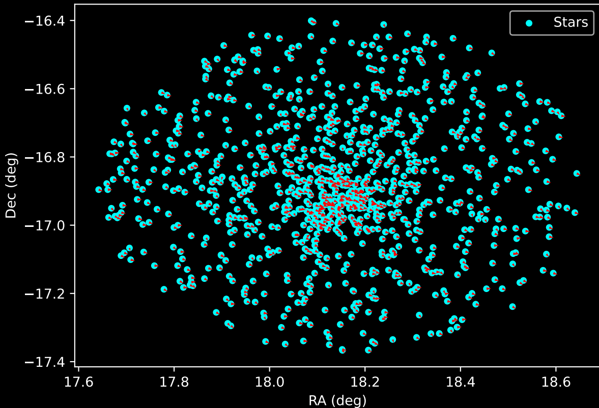
Gaia Cluster: [NGC_6645] Proper Motion Vectors for Gaia Star Field (n= 988)
