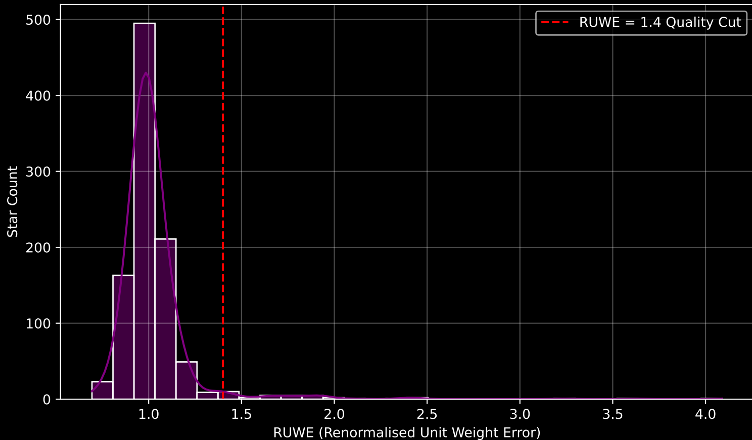
Gaia Cluster: [NGC_6645] RUWE Distribution (n= 986)
