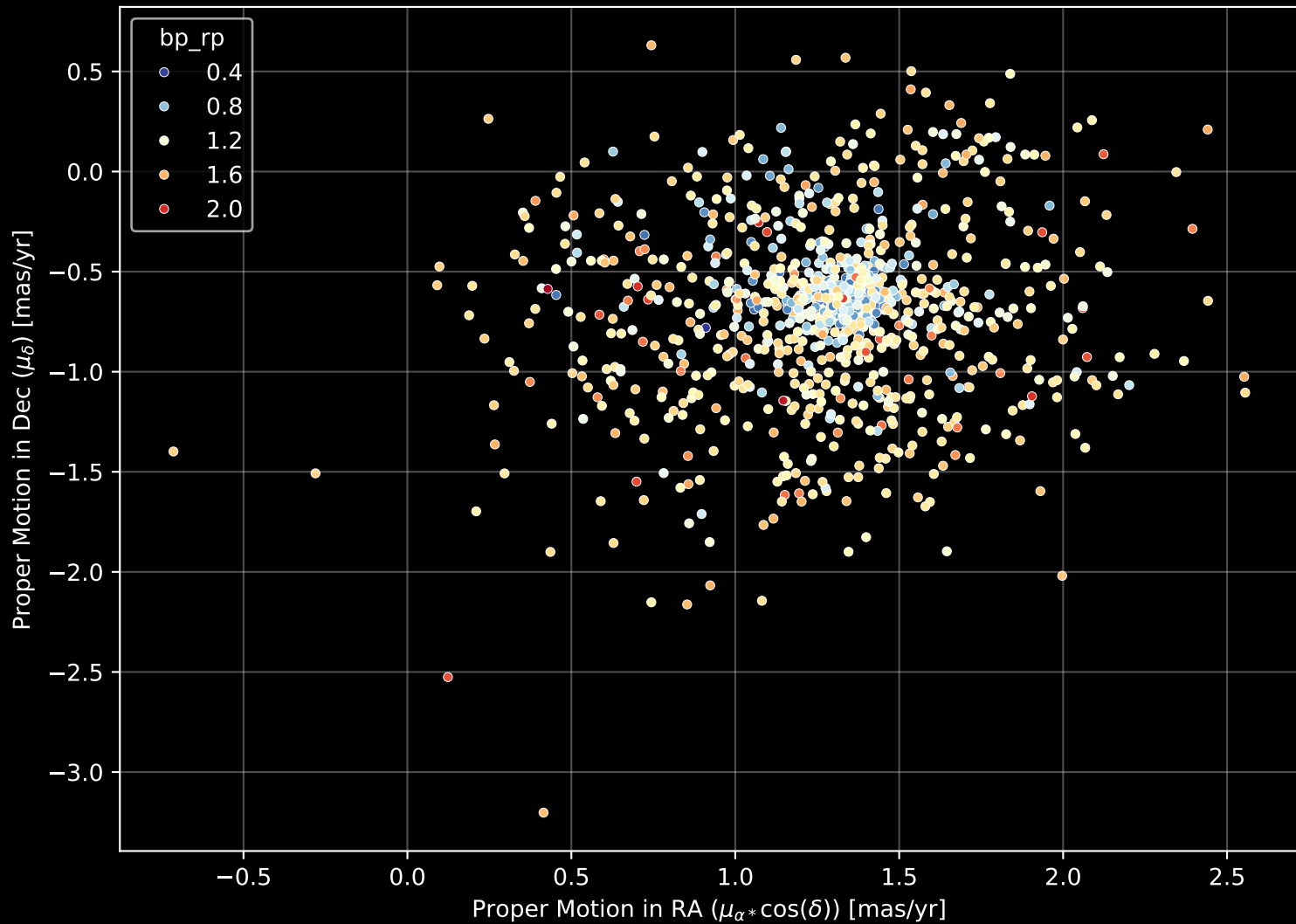
Gaia Cluster: [NGC_6645] Proper Motion Diagram (n= 988)
