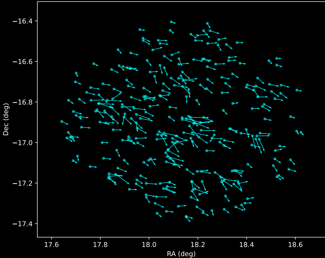
Gaia DR3 Noise Stream Proper Motion Vectors (n=268)
