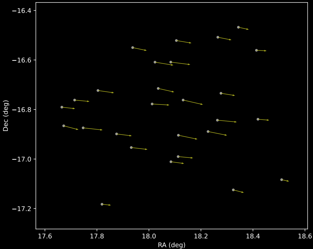
Gaia DR3 Cluster 16 Proper Motion Vectors (n=27)
