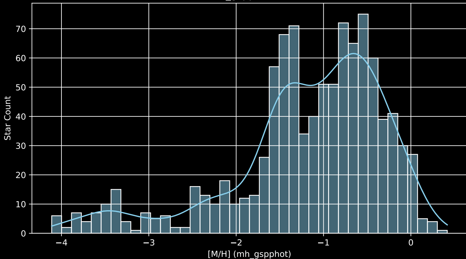
Gaia Cluster: [NGC_6645 [M/H] (mh_gspphot) (n= 987)
