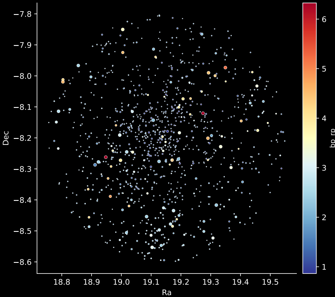
Gaia Cluster: [NGC_6664] Stars: 1048
