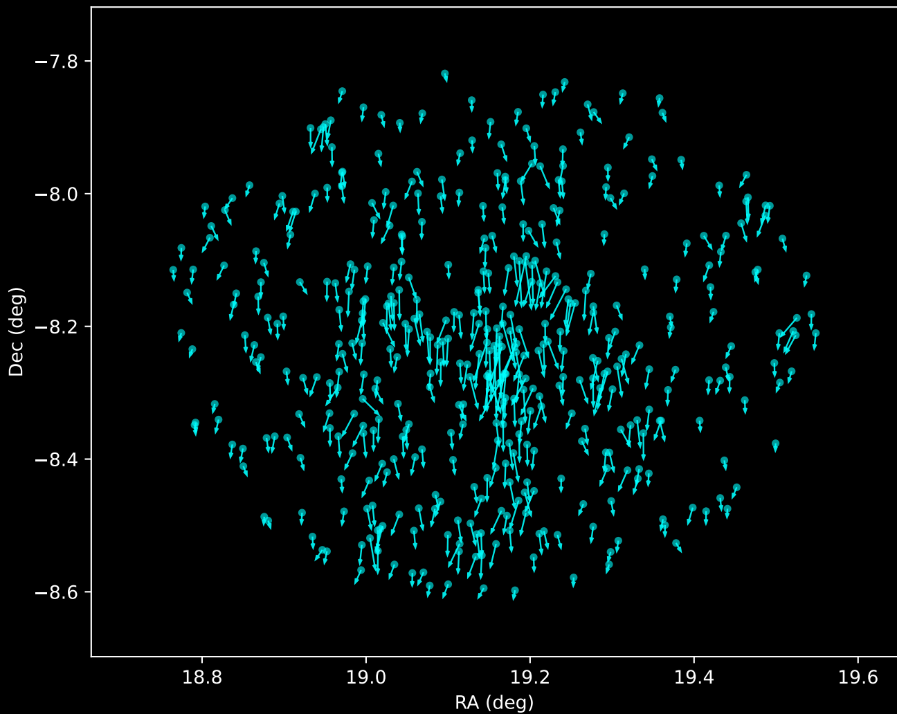
Gaia DR3 Noise Stream Proper Motion Vectors (n=432)
