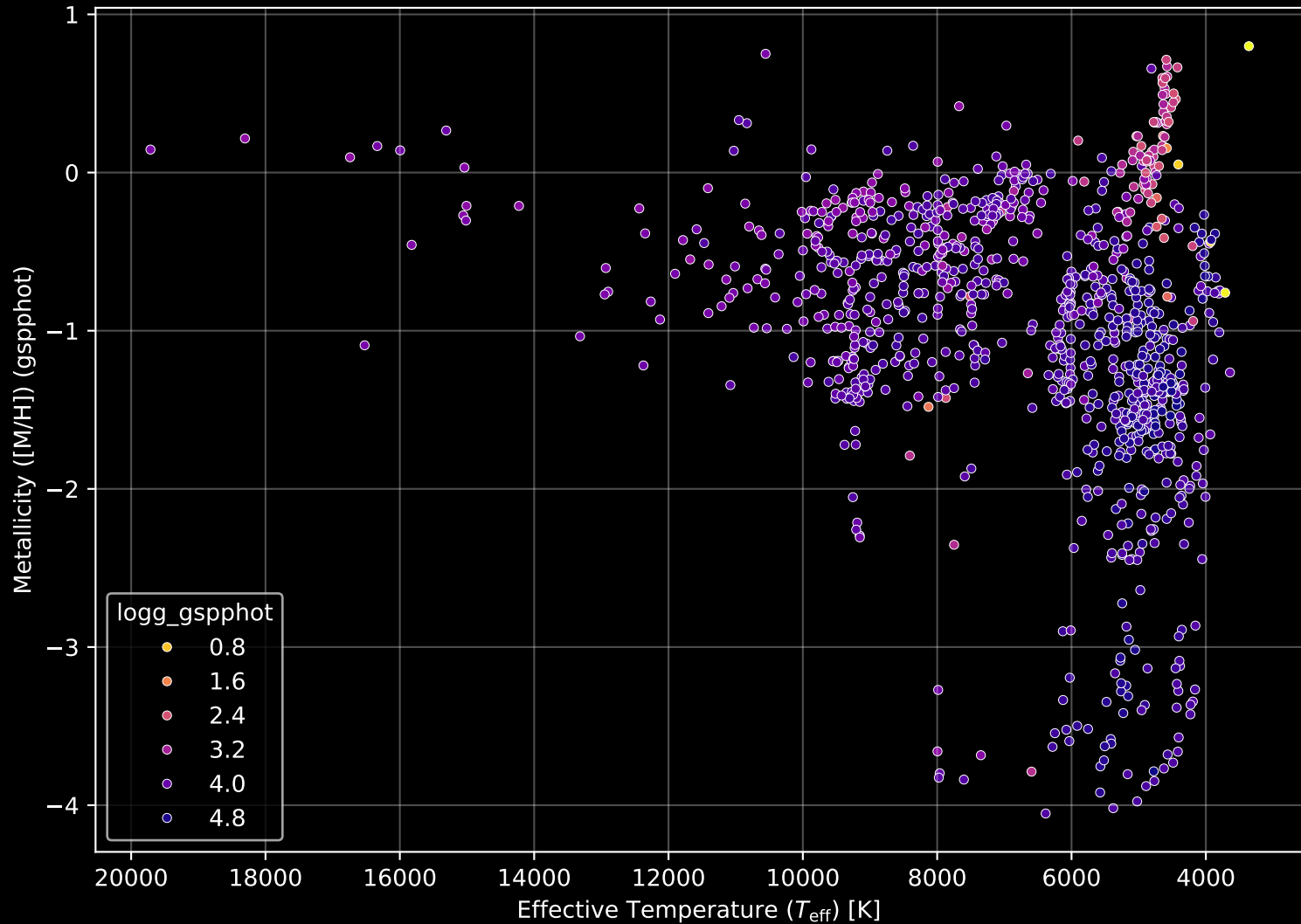
Gaia Cluster: [NGC_6664] Stellar Population Parameters (n= 1048)
