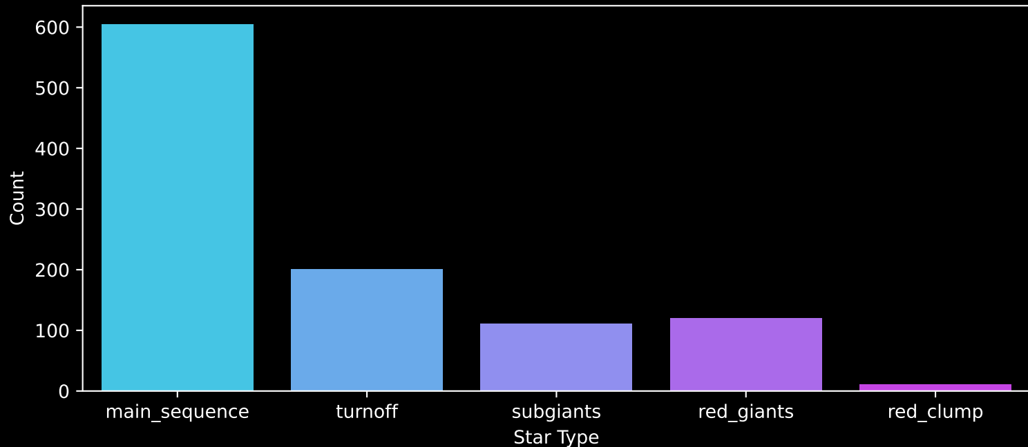
Gaia Cluster: [NGC_6664] Count plot of Star Type
