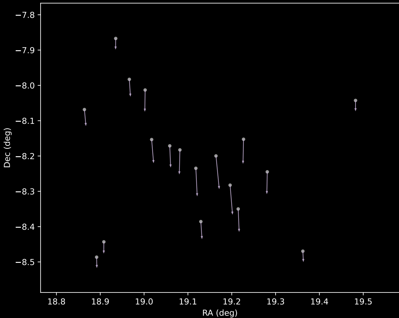
Gaia DR3 Cluster 29 Proper Motion Vectors (n=18)
