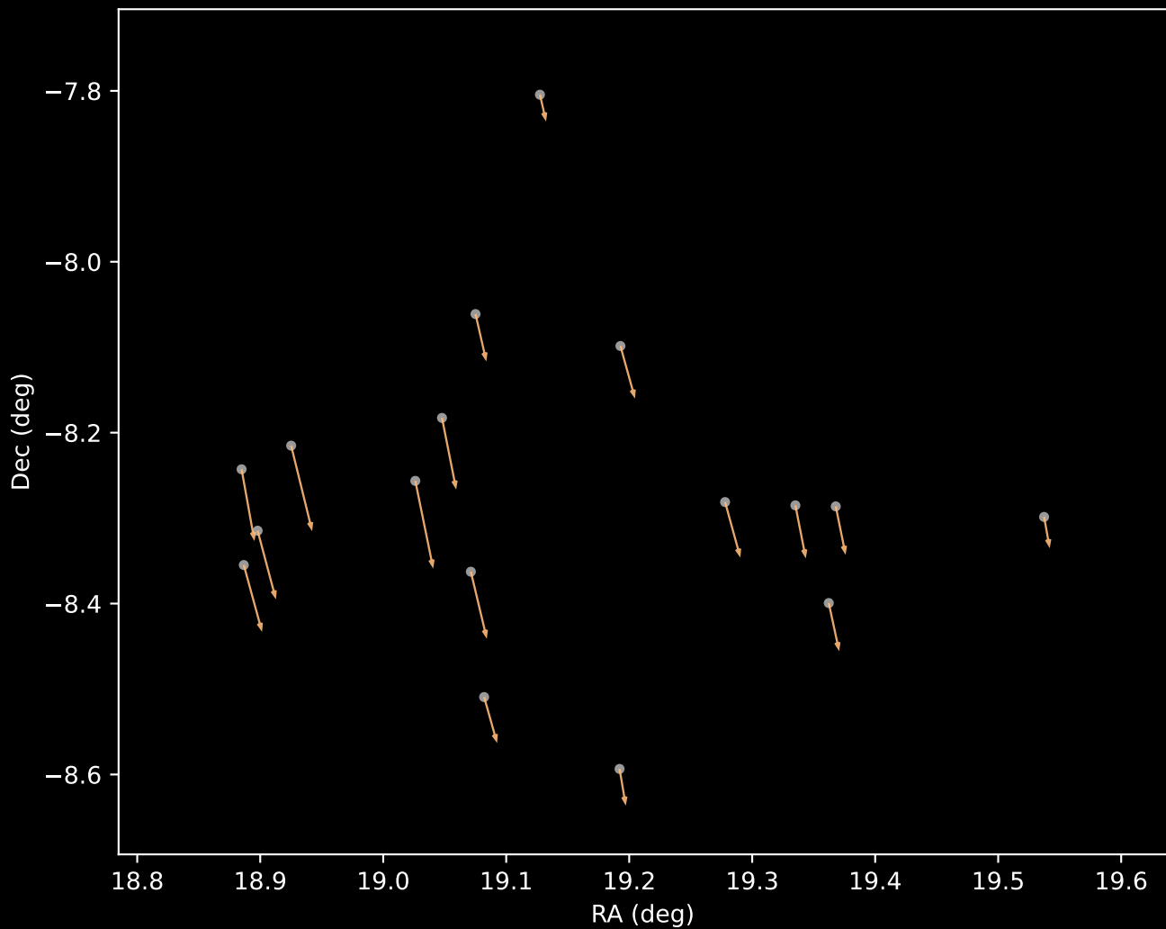
Gaia DR3 Cluster 23 Proper Motion Vectors (n=17)
