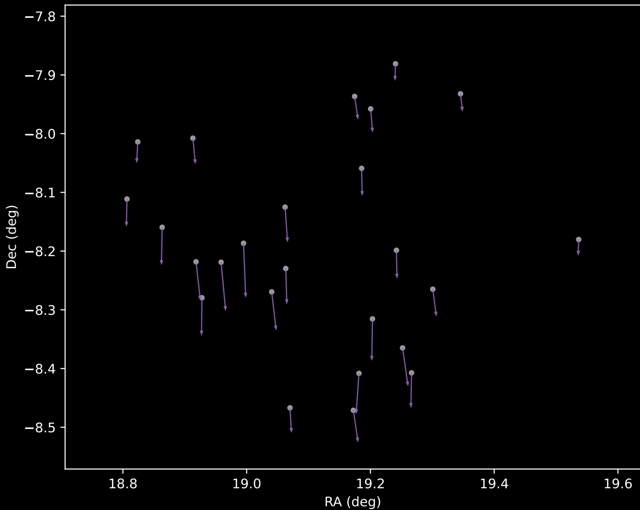
Gaia DR3 Cluster 8 Proper Motion Vectors (n=25)
