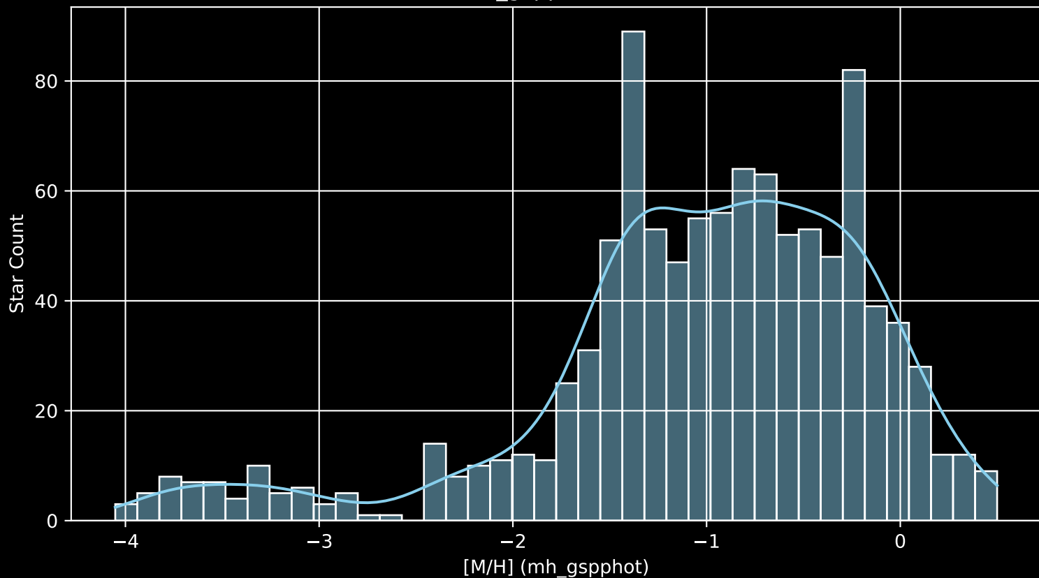
Gaia Cluster: [NGC_6664 [M/H] (mh_gspphot) ( \bar{n}= 1036 )
