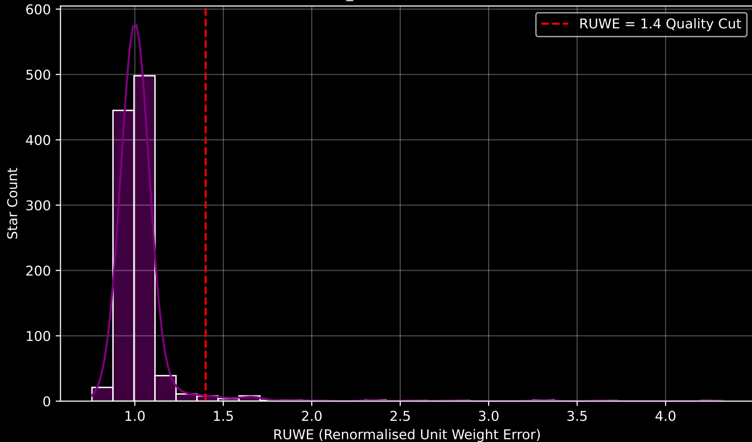
Gaia Cluster: [NGC_6664] RUWE Distribution (n= 1046)
