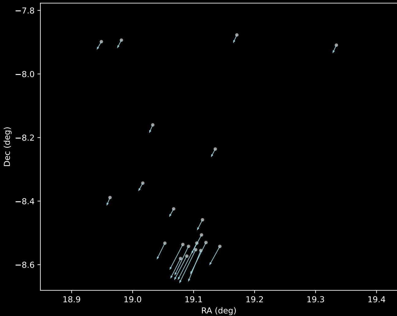
Gaia DR3 Cluster 19 Proper Motion Vectors (n=21)
