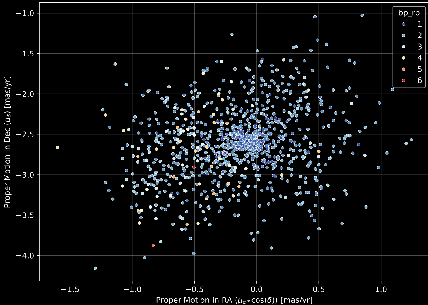
Gaia Cluster: [NGC_6664] Proper Motion Diagram (n= 1048)
