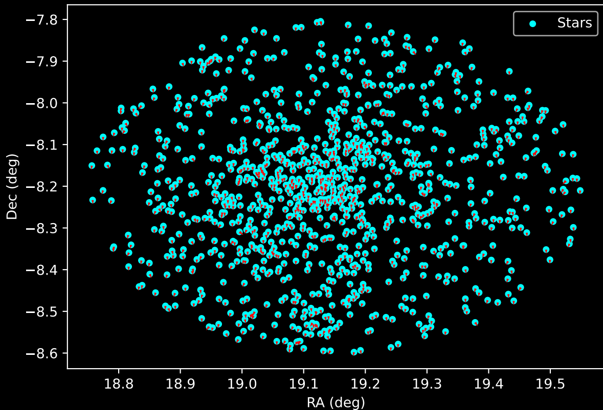
Gaia Cluster: [NGC_6664] Proper Motion Vectors for Gaia Star Field (n= 1048)
