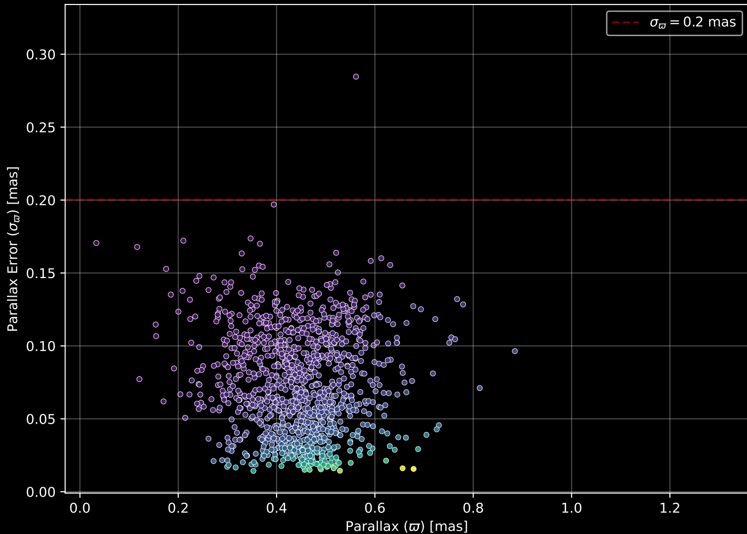
Gaia Cluster: [NGC_6664] Parallax Quality (n= 1048)
