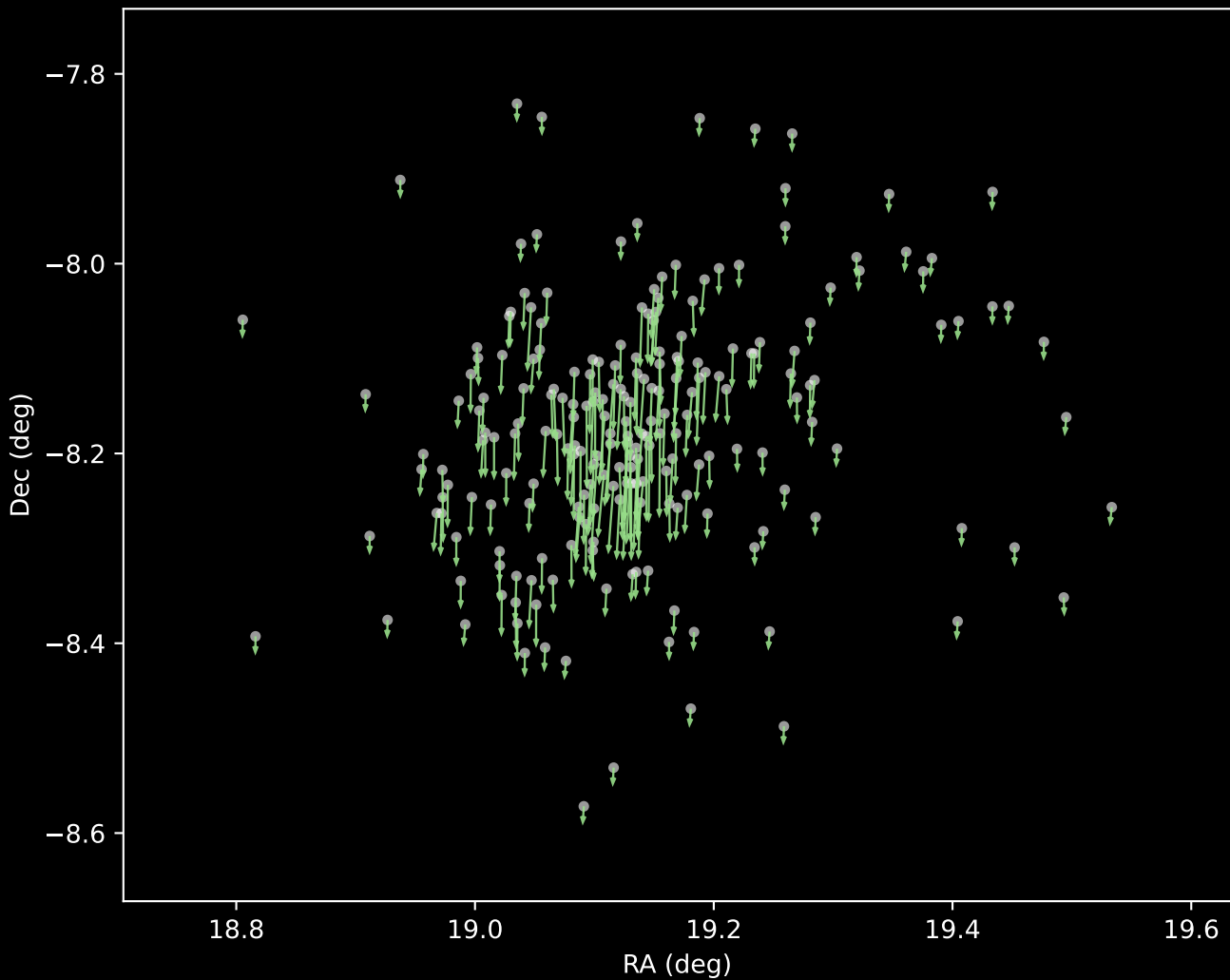
Gaia DR3 Cluster 45 Proper Motion Vectors (n=215)
