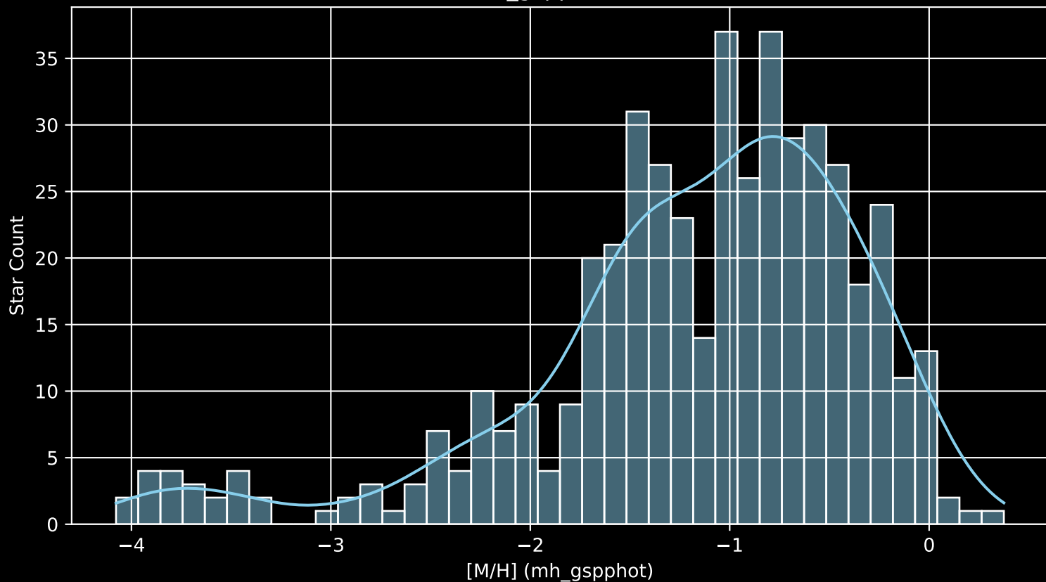
Gaia Cluster: [NGC_6694 [M/H] (mh_gspphot) (n= 473)
