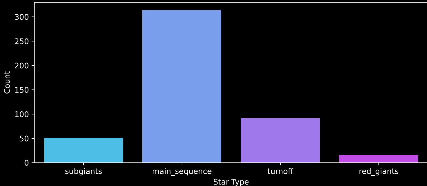
Gaia Cluster: [NGC_6694] Count plot of Star Type
