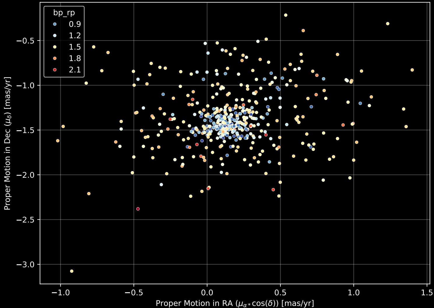
Gaia Cluster: [NGC_6694] Proper Motion Diagram (n= 473)
