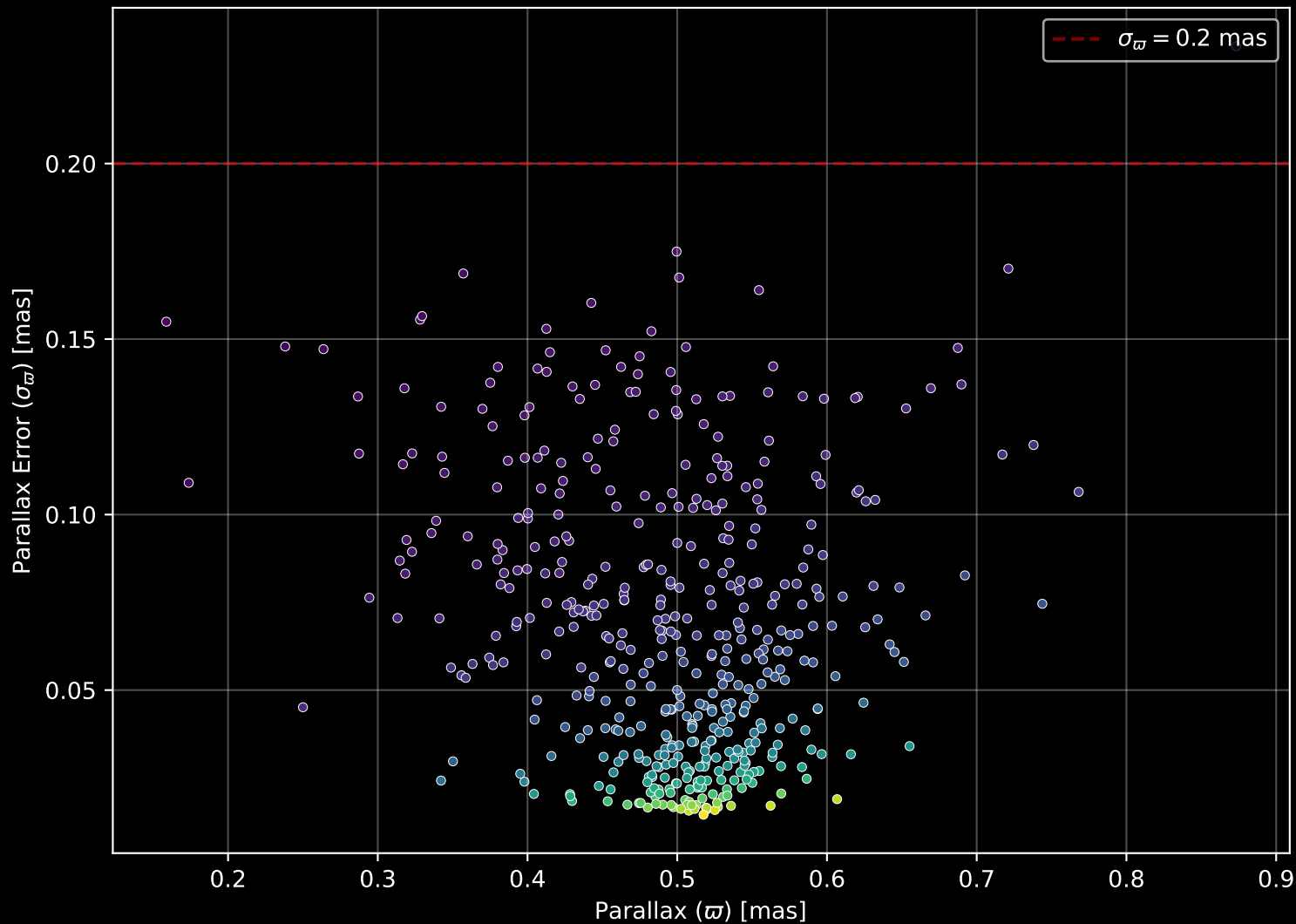
Gaia Cluster: [NGC_6694] Parallax Quality (n= 473)
