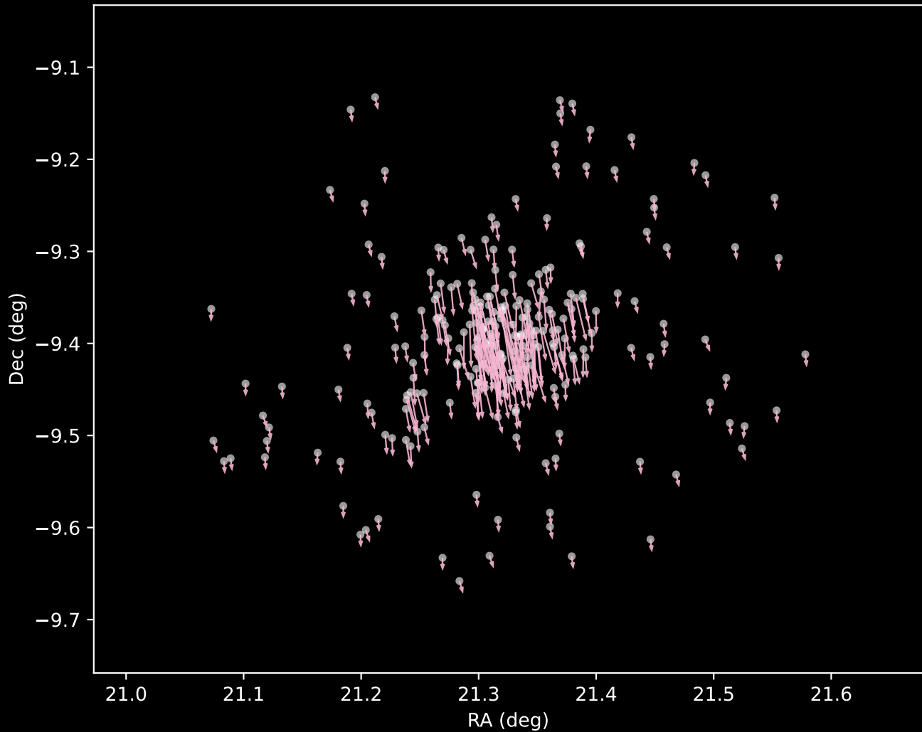
Gaia DR3 Cluster 13 Proper Motion Vectors (n=242)
