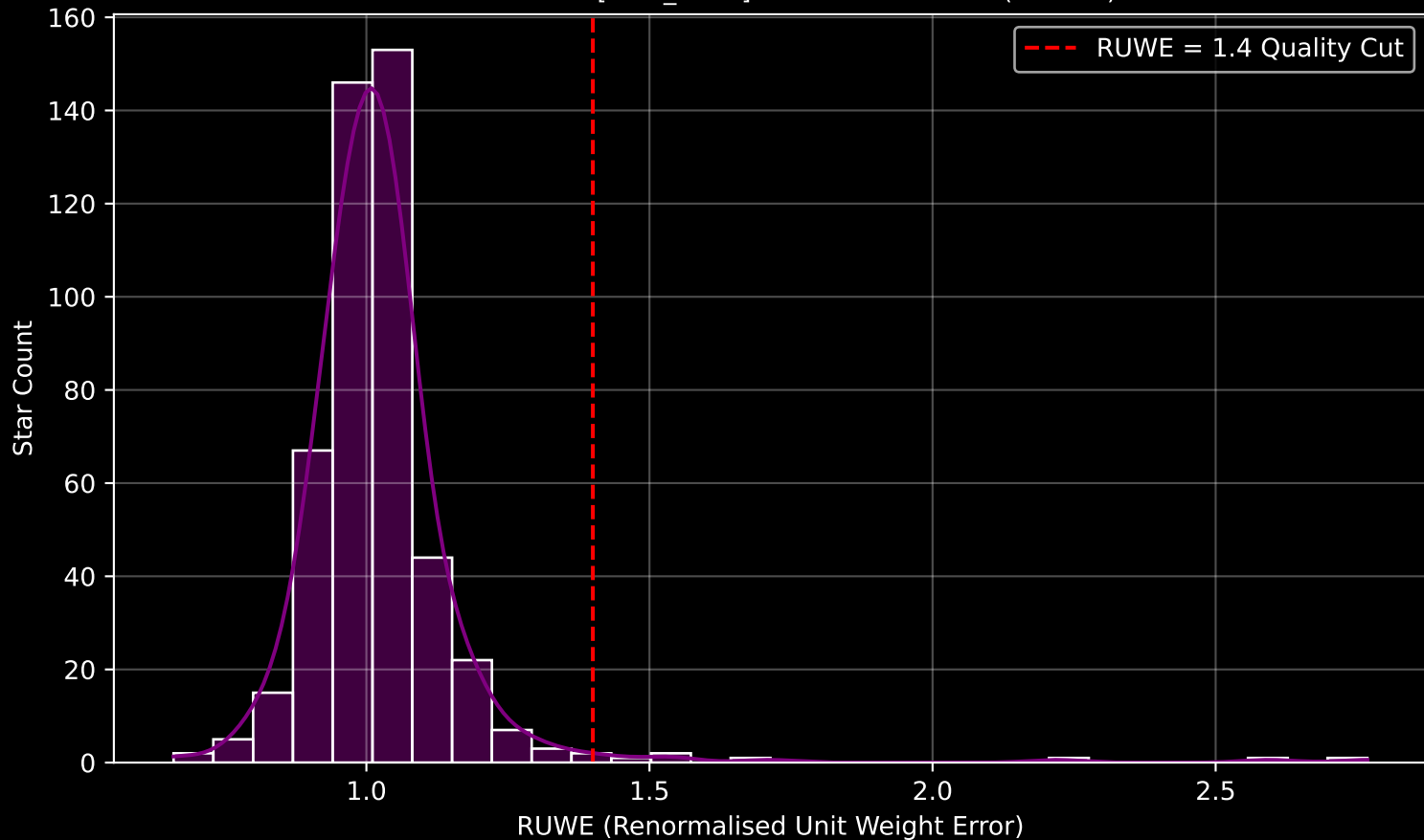
Gaia Cluster: [NGC_6694] RUWE Distribution (n= 473)
