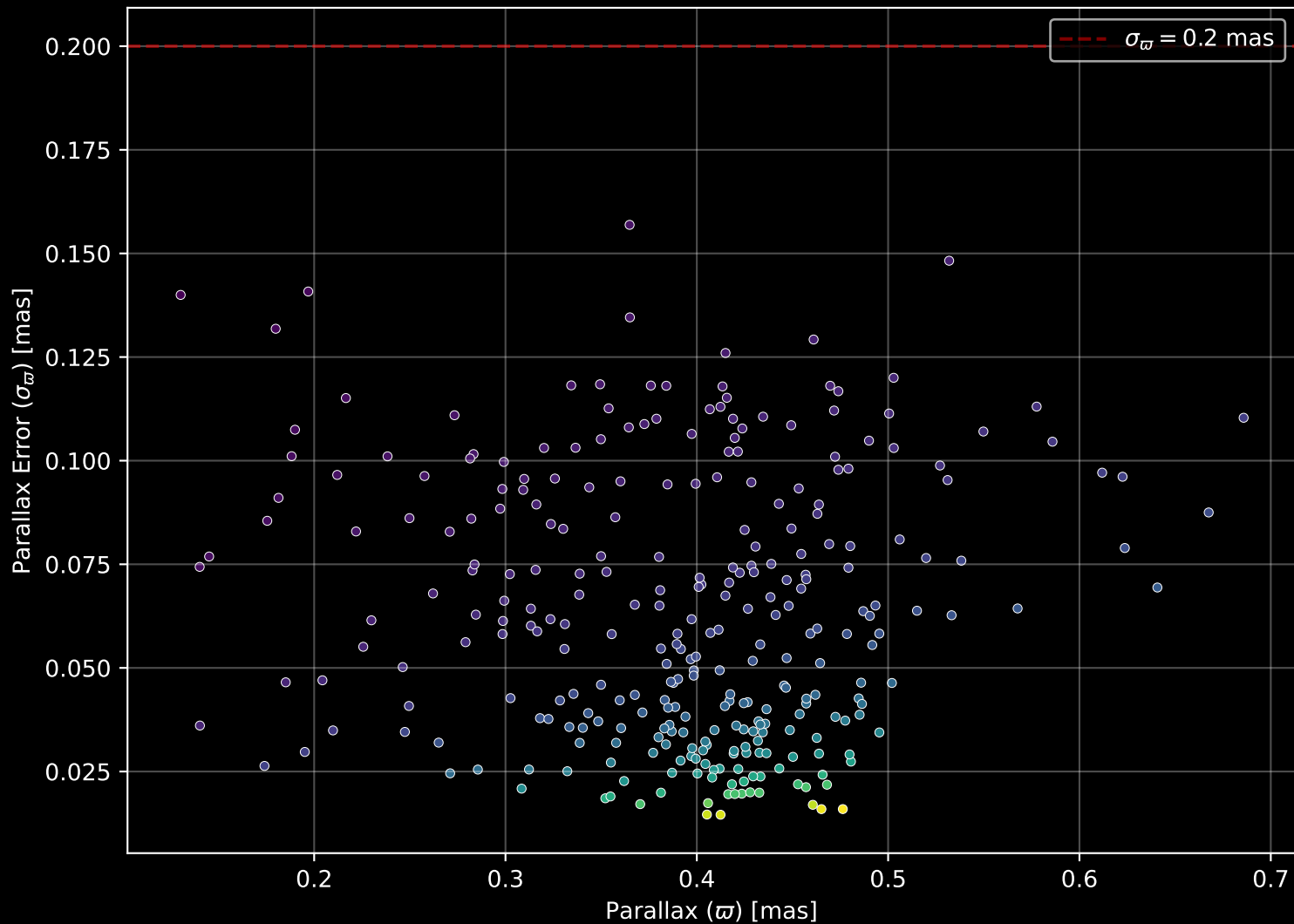
Gaia Cluster: [NGC_6704] Parallax Quality (n= 298)
