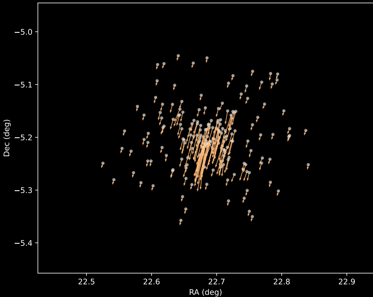
Gaia DR3 Cluster 3 Proper Motion Vectors (n=188)
