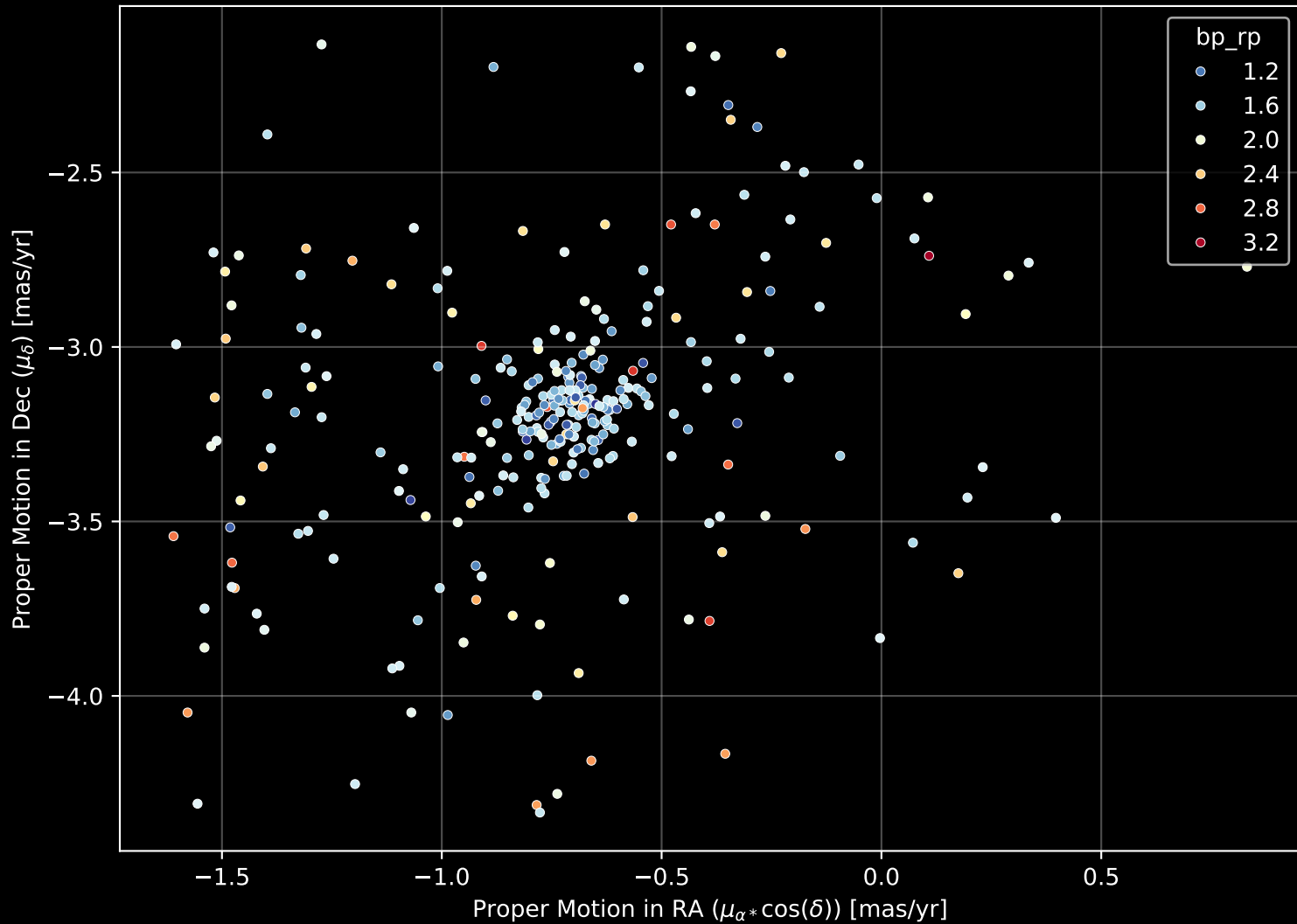
Gaia Cluster: [NGC_6704] Proper Motion Diagram (n= 298)
