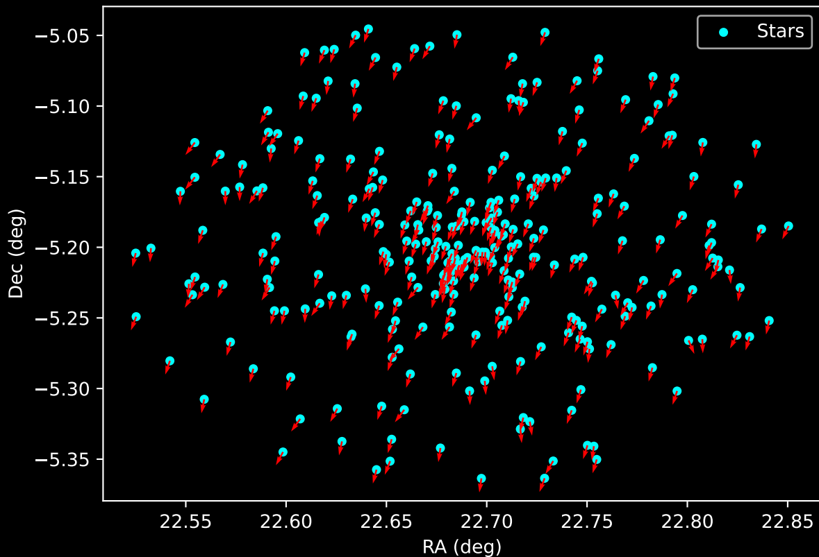
Gaia Cluster: [NGC_6704] Proper Motion Vectors for Gaia Star Field (n= 298)
