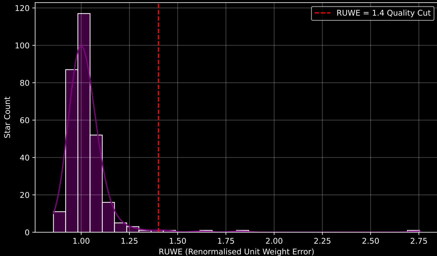
Gaia Cluster: [NGC_6704] RUWE Distribution (n= 297)
