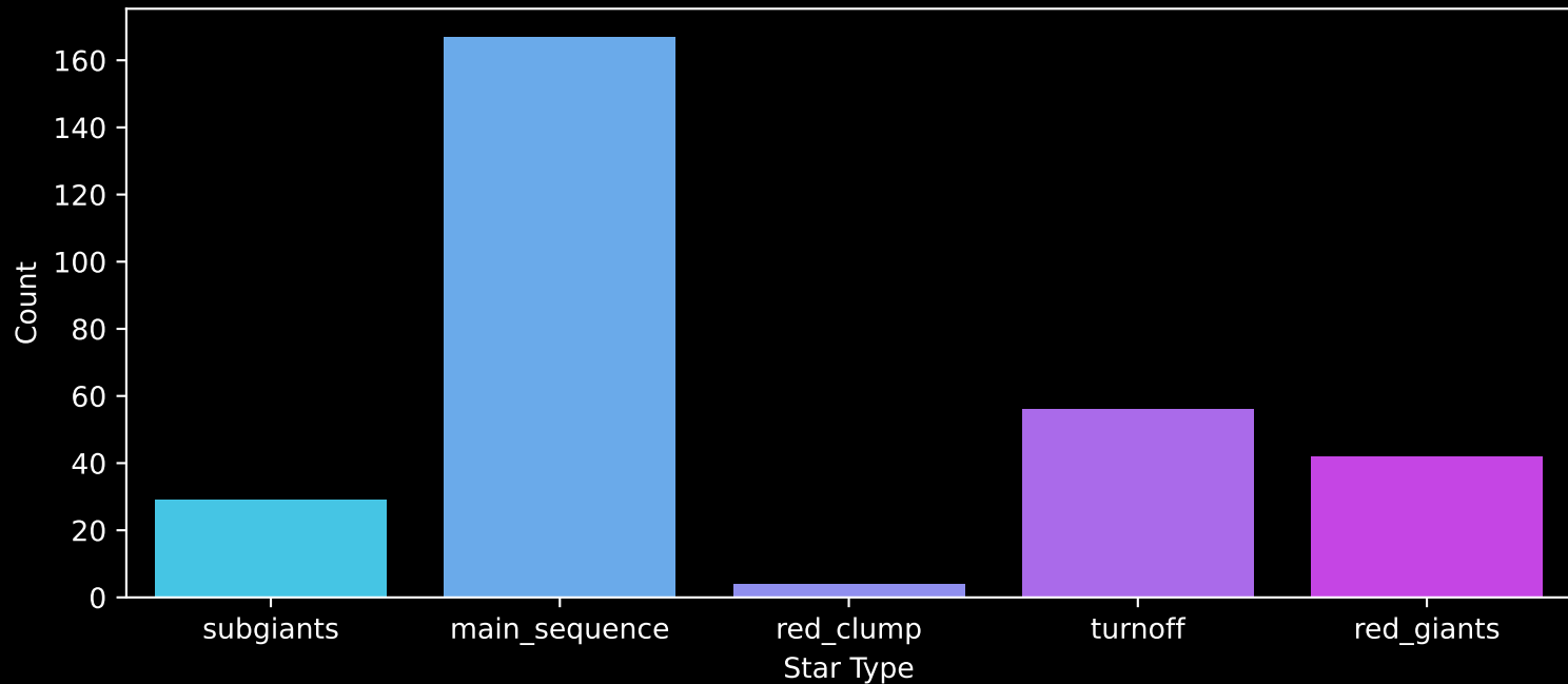
Gaia Cluster: [NGC_6704] Count plot of Star Type
