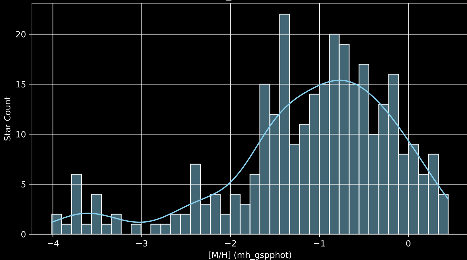
Gaia Cluster: [NGC_6704 [M/H] (mh_gspphot) (n= 296)
