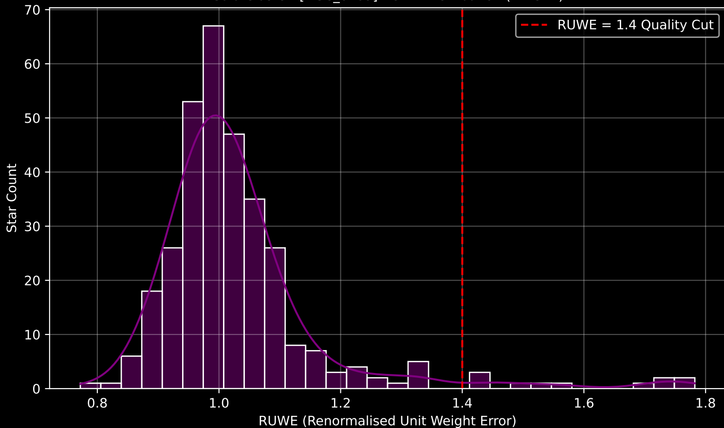
Gaia Cluster: [NGC_6709] RUWE Distribution (n= 321)
