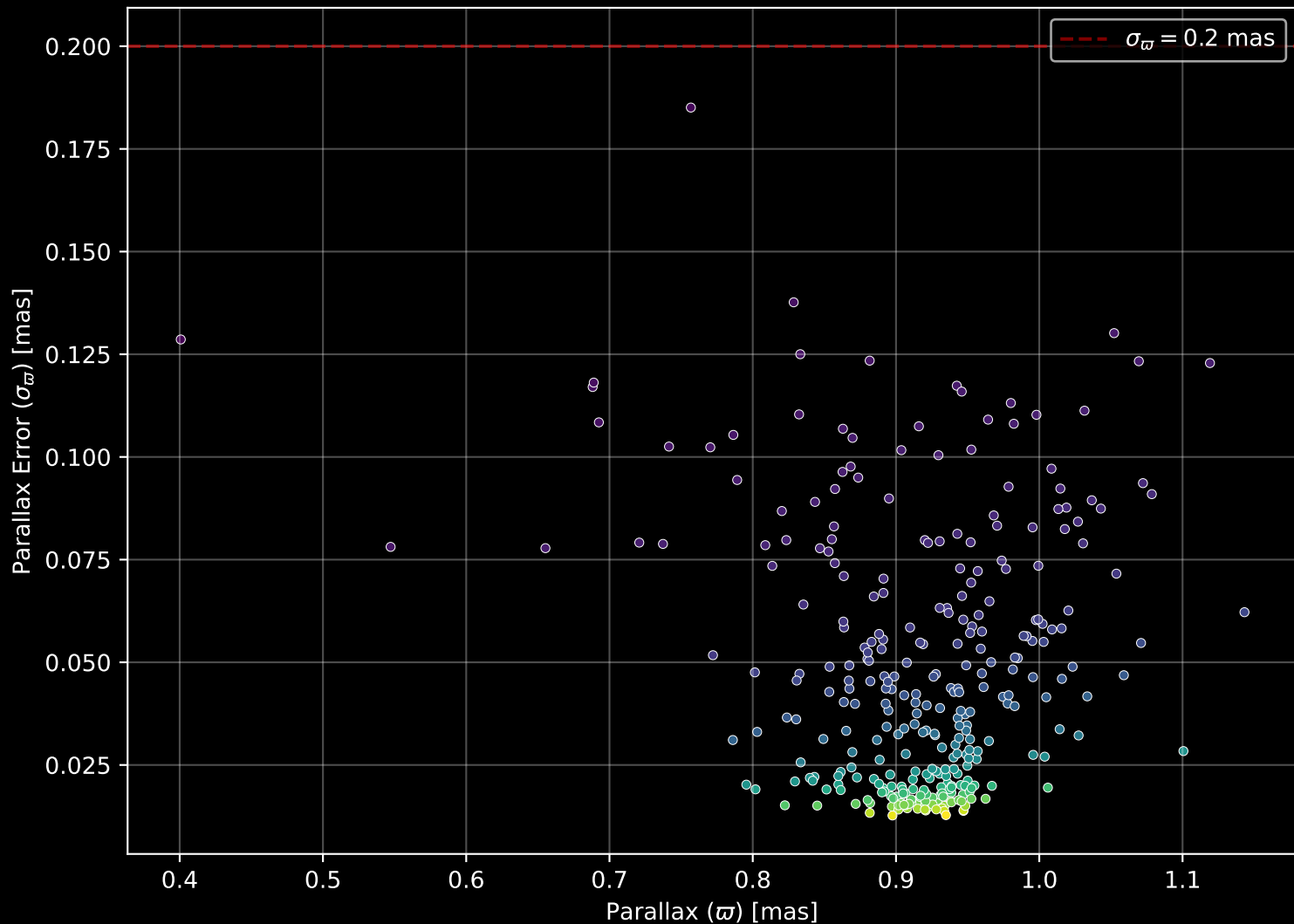
Gaia Cluster: [NGC_6709] Parallax Quality (n= 321)
