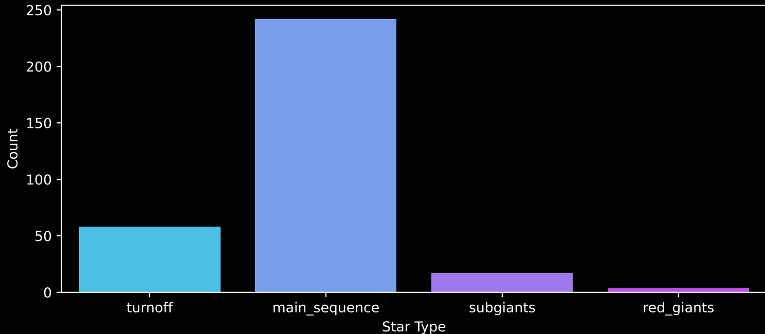
Gaia Cluster: [NGC_6709] Count plot of Star Type
