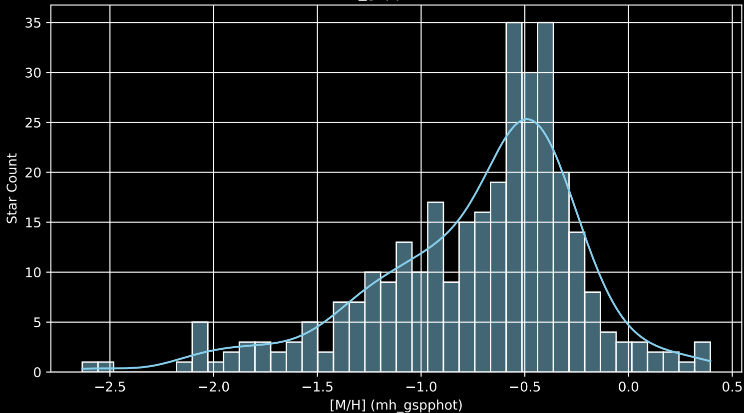
Gaia Cluster: [NGC_6709 [M/H] (mh_gspphot) (n= 321)
