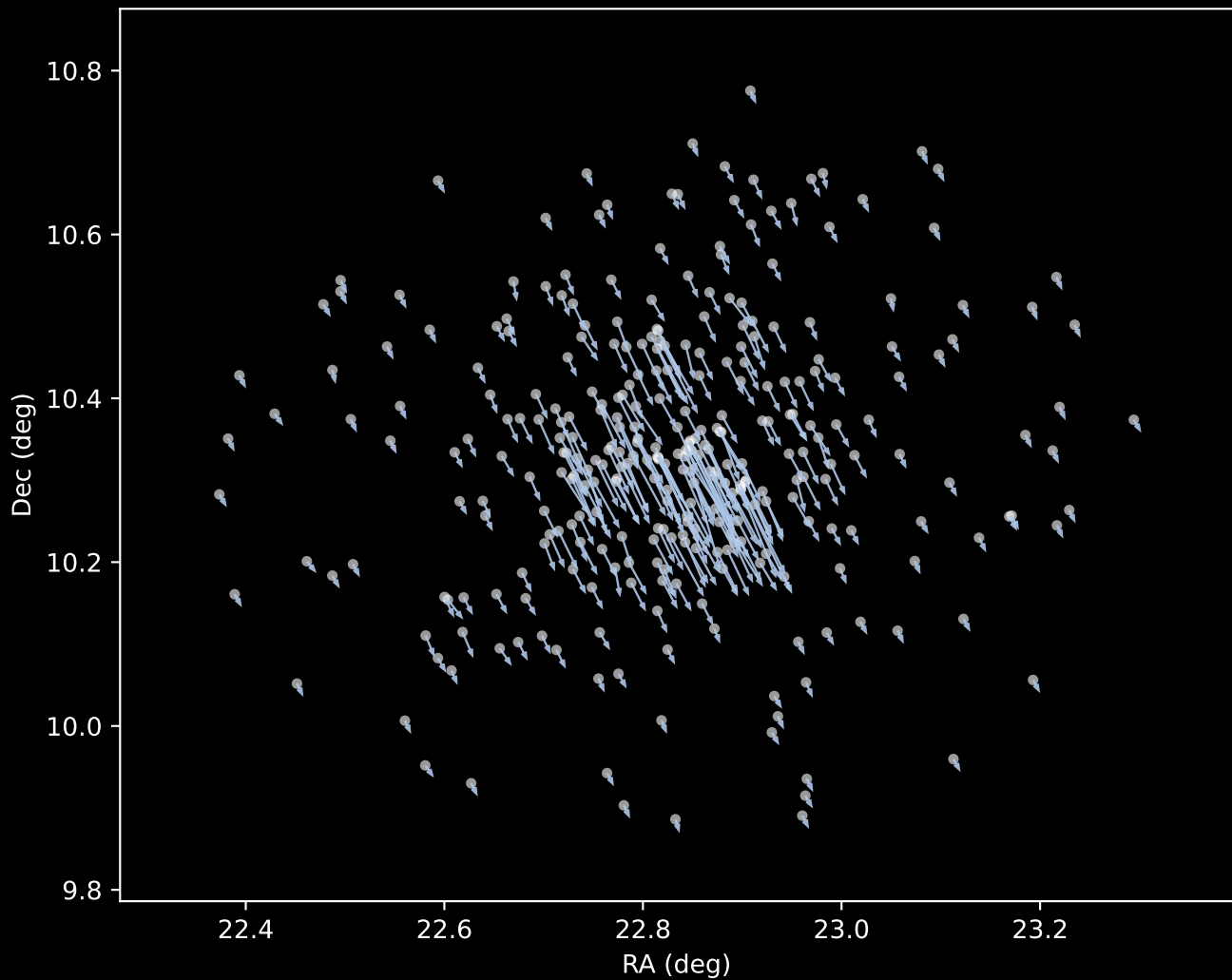
Gaia DR3 Cluster 1 Proper Motion Vectors (n=315)
