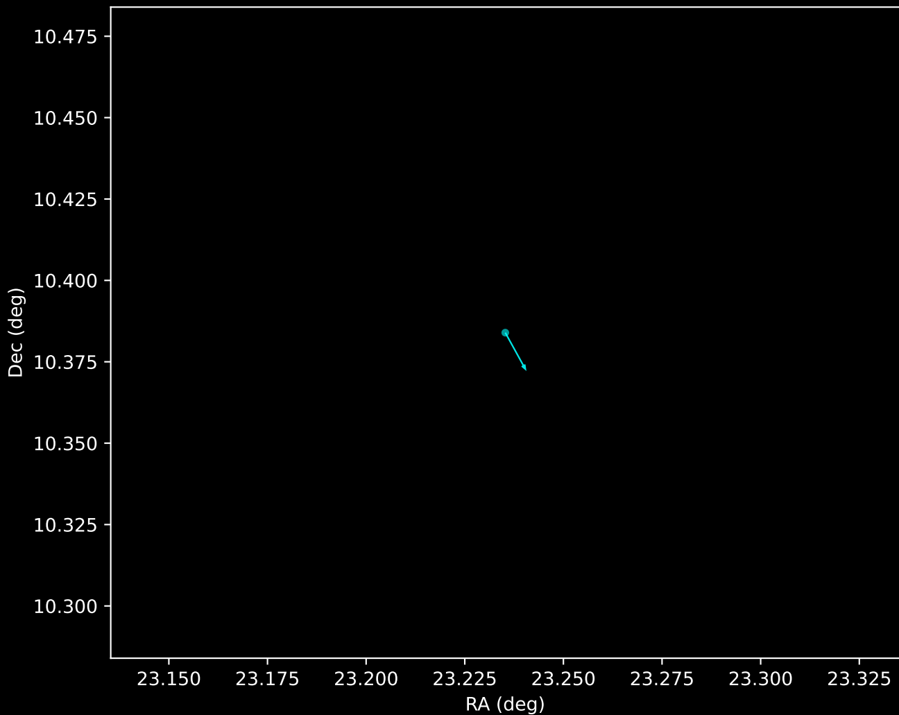
Gaia DR3 Noise Stream Proper Motion Vectors (n=1)
