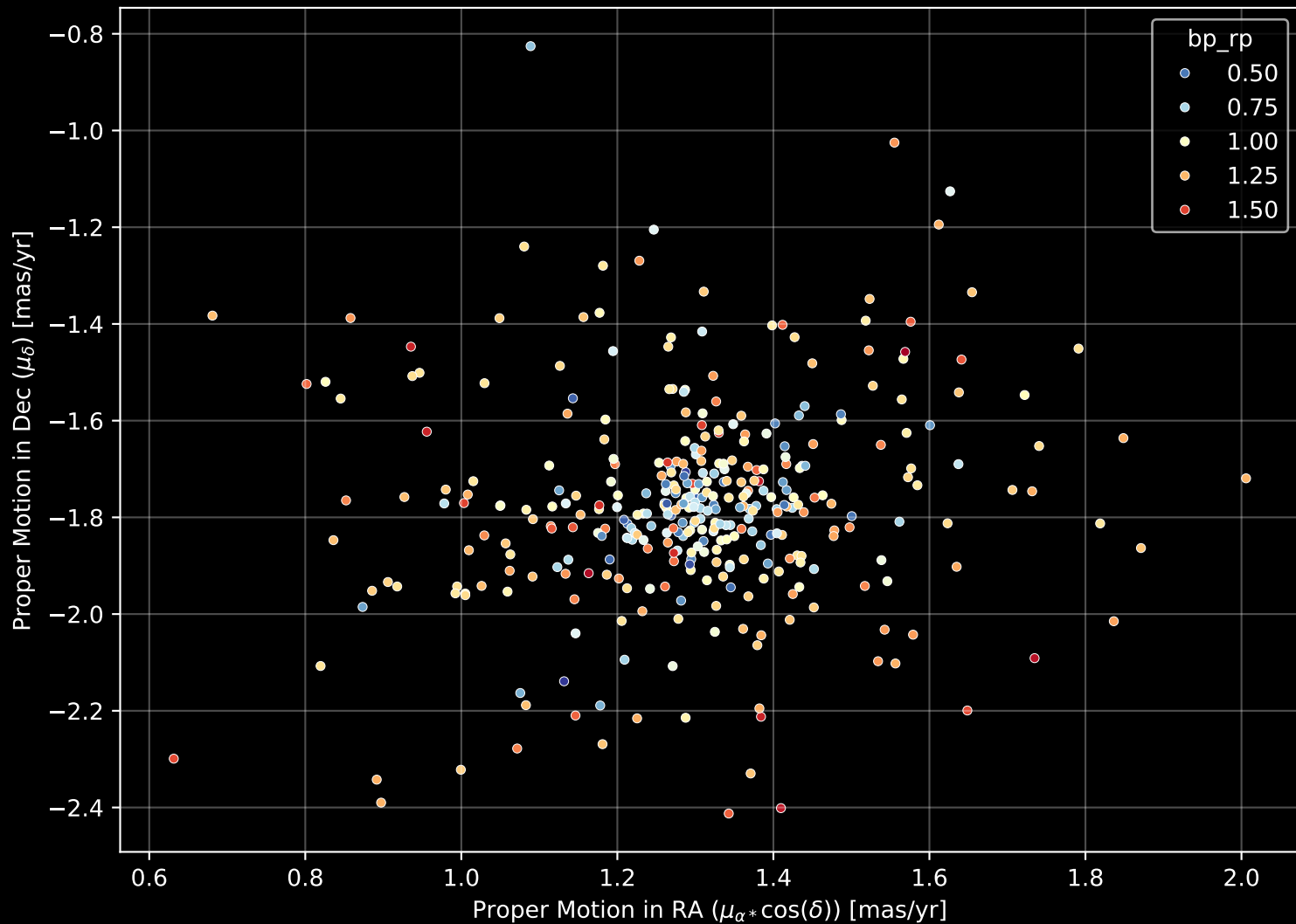
Gaia Cluster: [NGC_6728] Proper Motion Diagram (n= 357)
