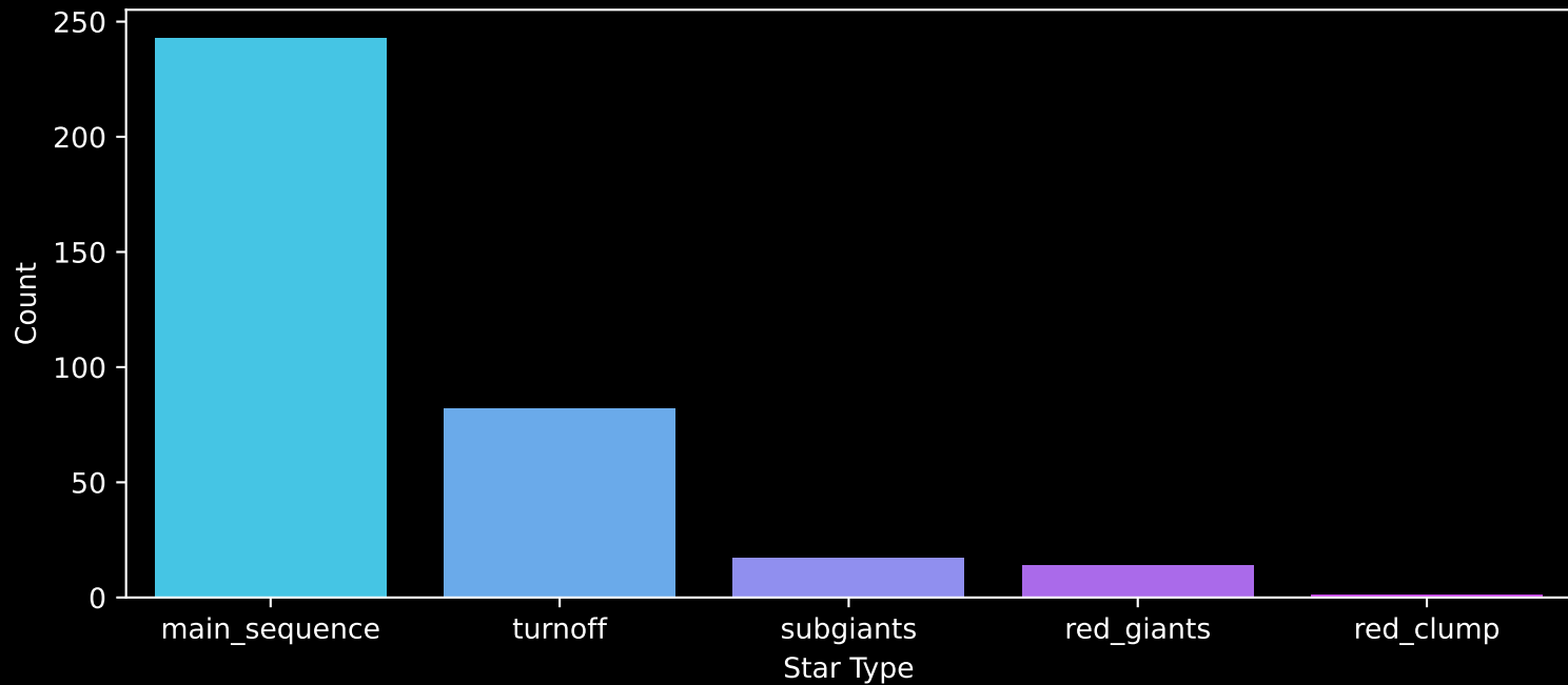
Gaia Cluster: [NGC_6728] Count plot of Star Type
