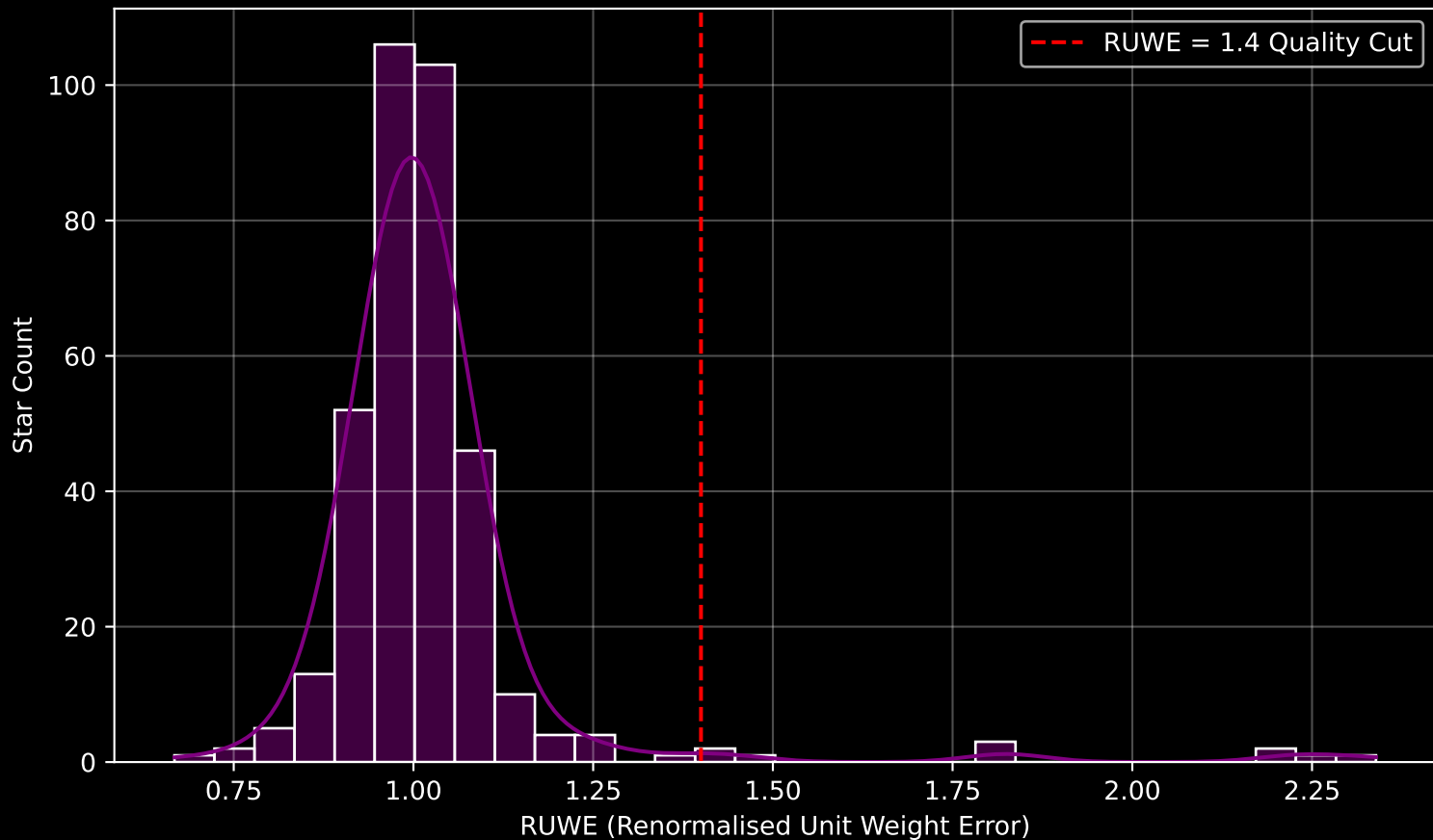
Gaia Cluster: [NGC_6728] RUWE Distribution (n= 357)
