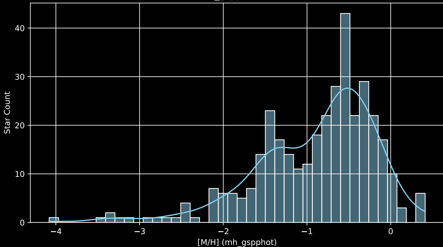
Gaia Cluster: [NGC_6728 [M/H] (mh_gspphot) (n= 357)
