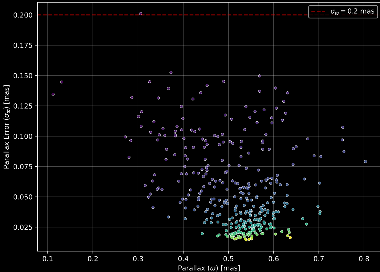
Gaia Cluster: [NGC_6728] Parallax Quality (n= 357)
