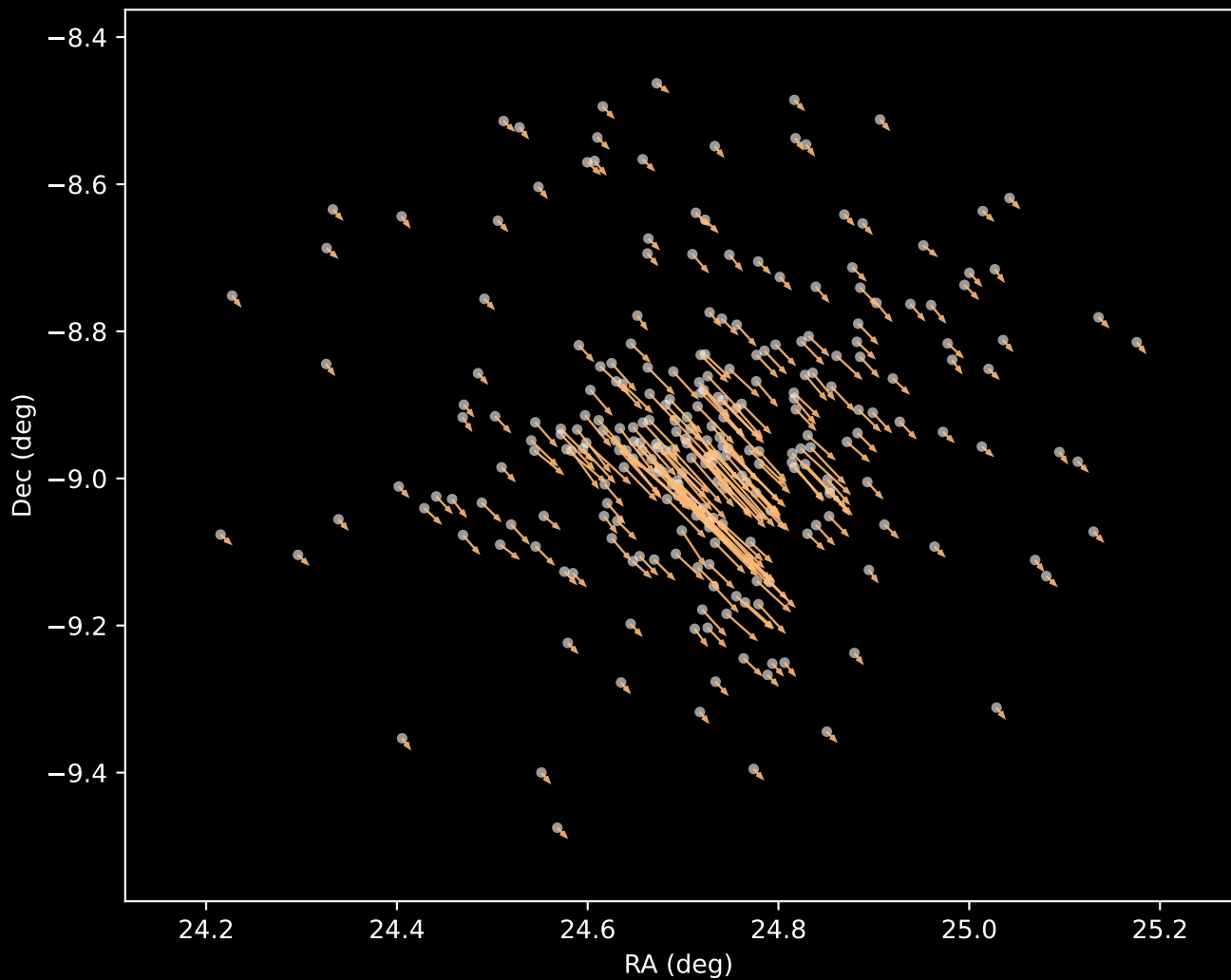
Gaia DR3 Cluster 3 Proper Motion Vectors (n=260)
