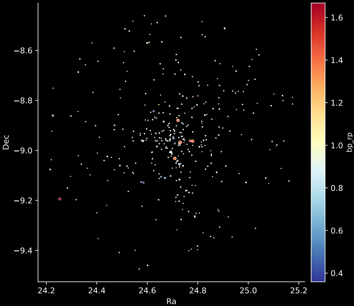
Gaia Cluster: [NGC_6728] Stars: 357
