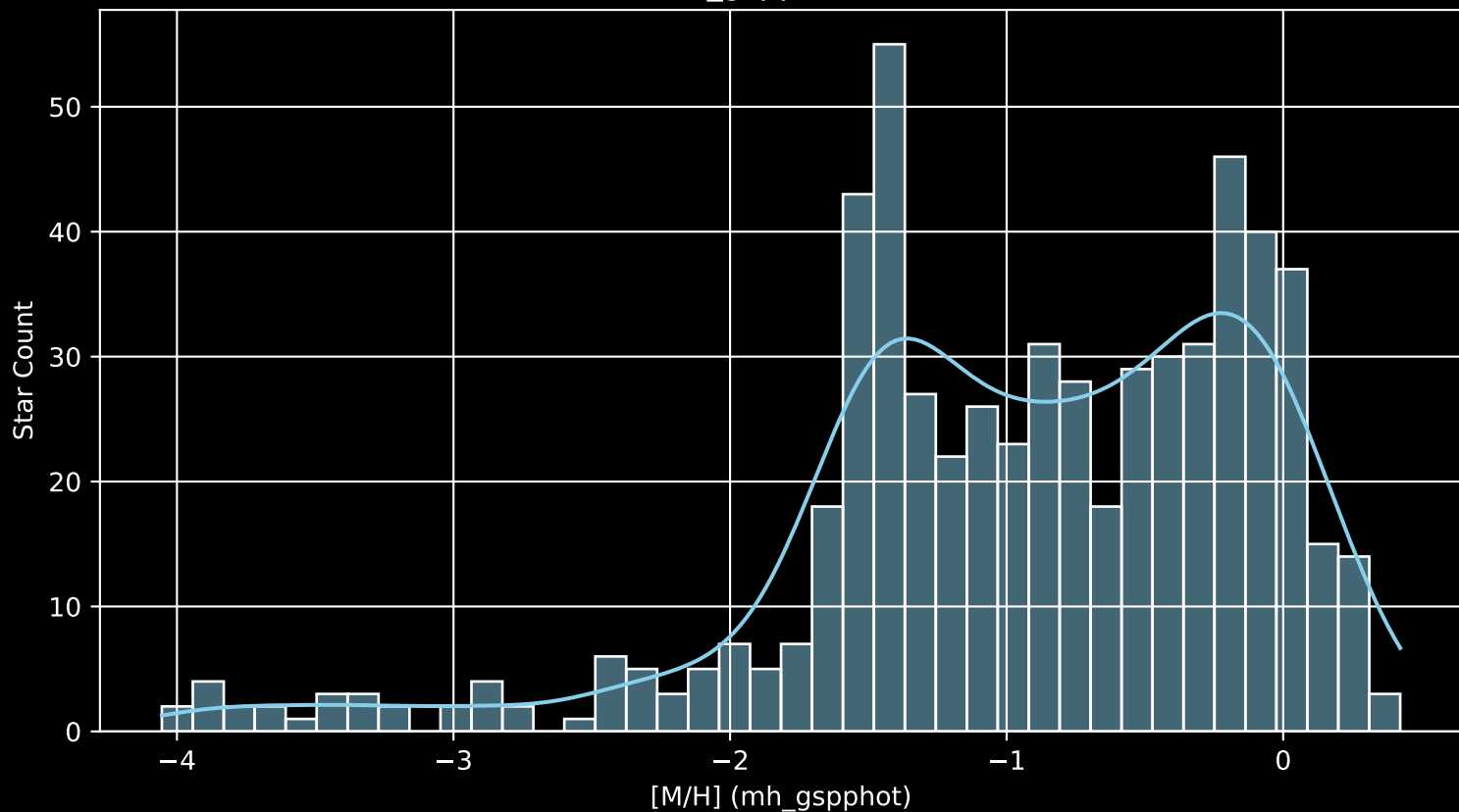
Gaia Cluster: [NGC_6735 [M/H] (mh_gspphot) (n= 602)
