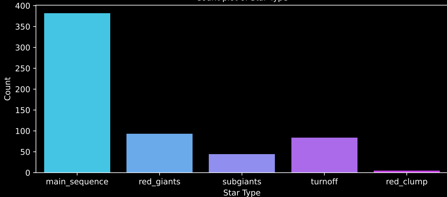
Gaia Cluster: [NGC_6735] Count plot of Star Type
