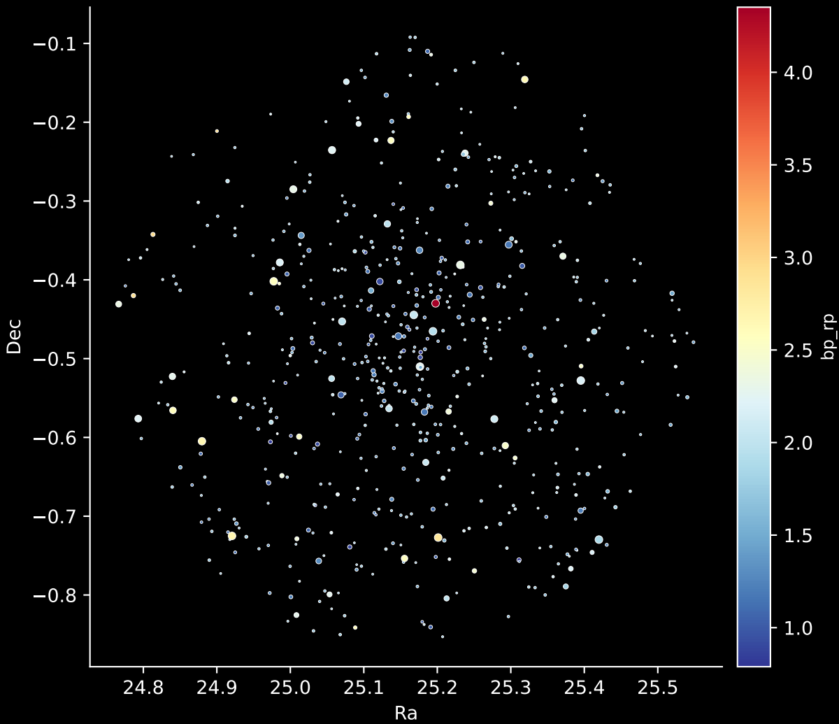
Gaia Cluster: [NGC_6735] Stars: 608
