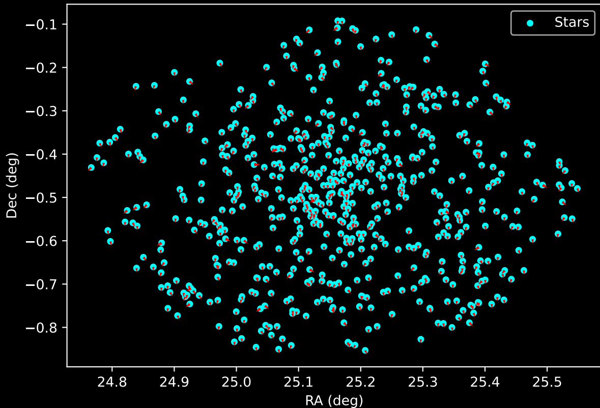
Gaia Cluster: [NGC_6735] Proper Motion Vectors for Gaia Star Field (n= 608)
