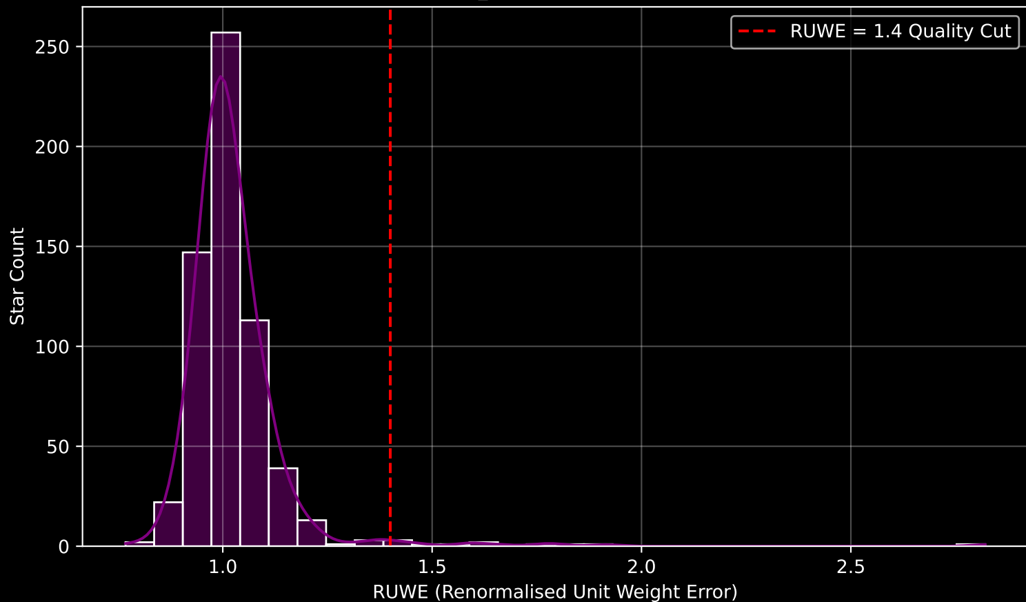
Gaia Cluster: [NGC_6735] RUWE Distribution (n= 608)
