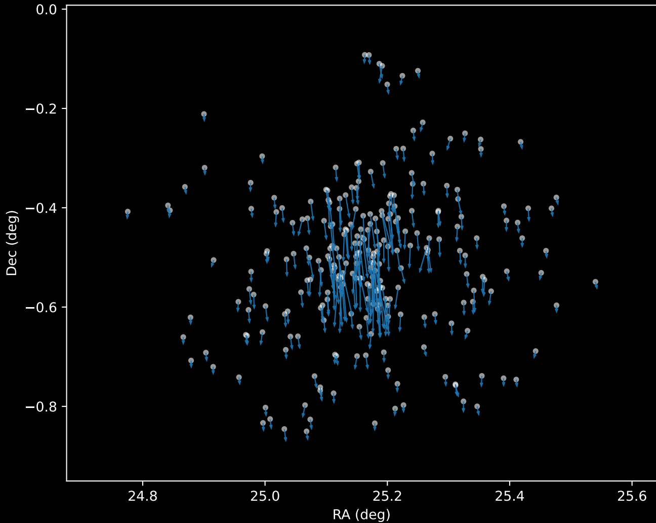
Gaia DR3 Cluster 20 Proper Motion Vectors (n=253)
