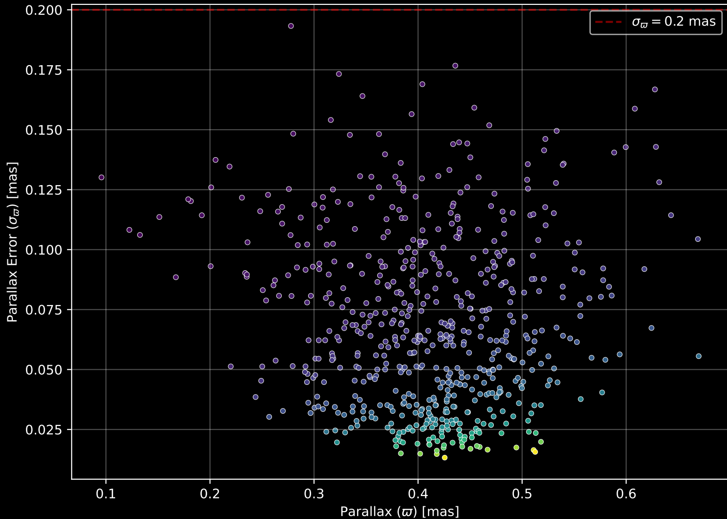
Gaia Cluster: [NGC_6735] Parallax Quality (n= 608)
