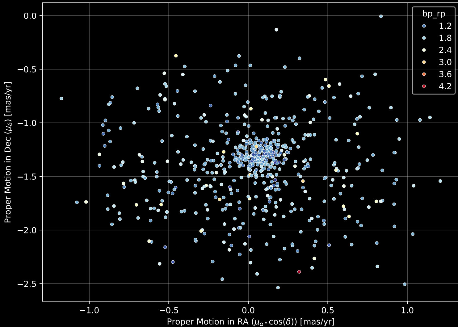
Gaia Cluster: [NGC_6735] Proper Motion Diagram (n= 608)
