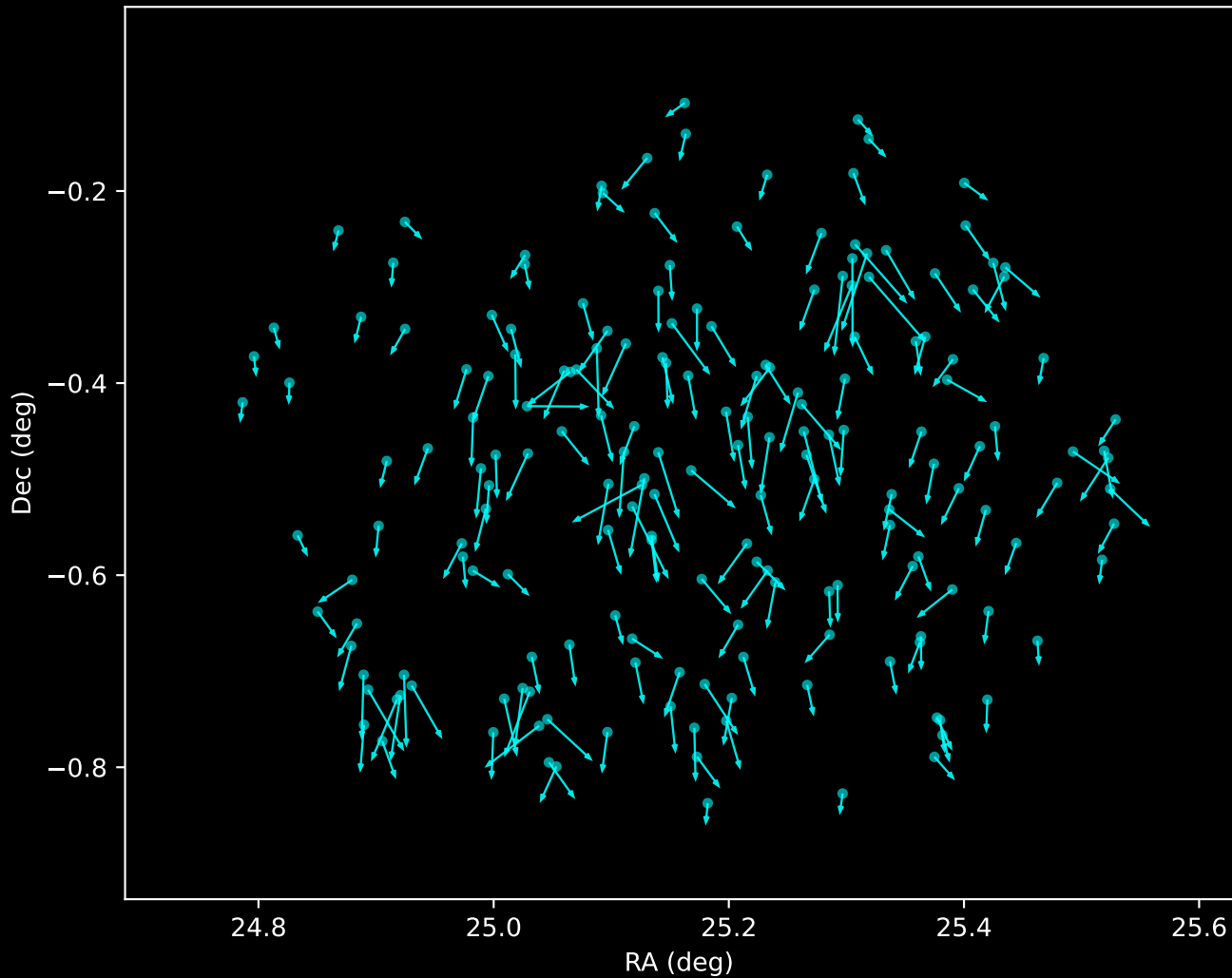
Gaia DR3 Noise Stream Proper Motion Vectors (n=186)
