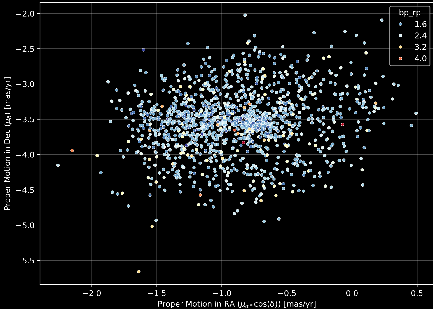
Gaia Cluster: [NGC_6755] Proper Motion Diagram (n= 1379)
