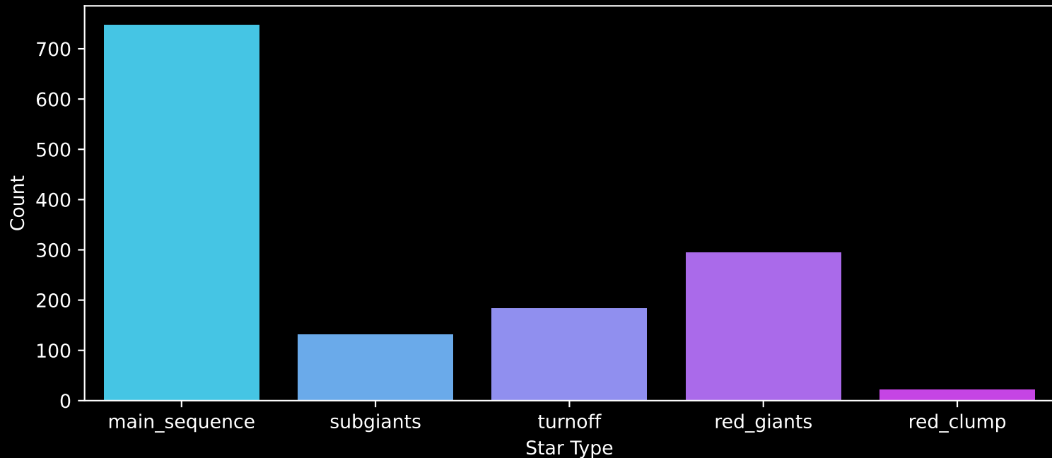
Gaia Cluster: [NGC_6755] Count plot of Star Type
