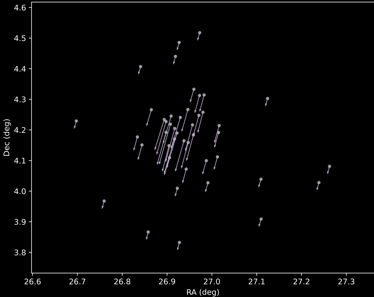
Gaia DR3 Cluster 69 Proper Motion Vectors (n=44)
