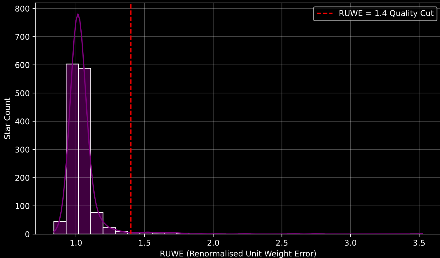
Gaia Cluster: [NGC_6755] RUWE Distribution (n= 1376)
