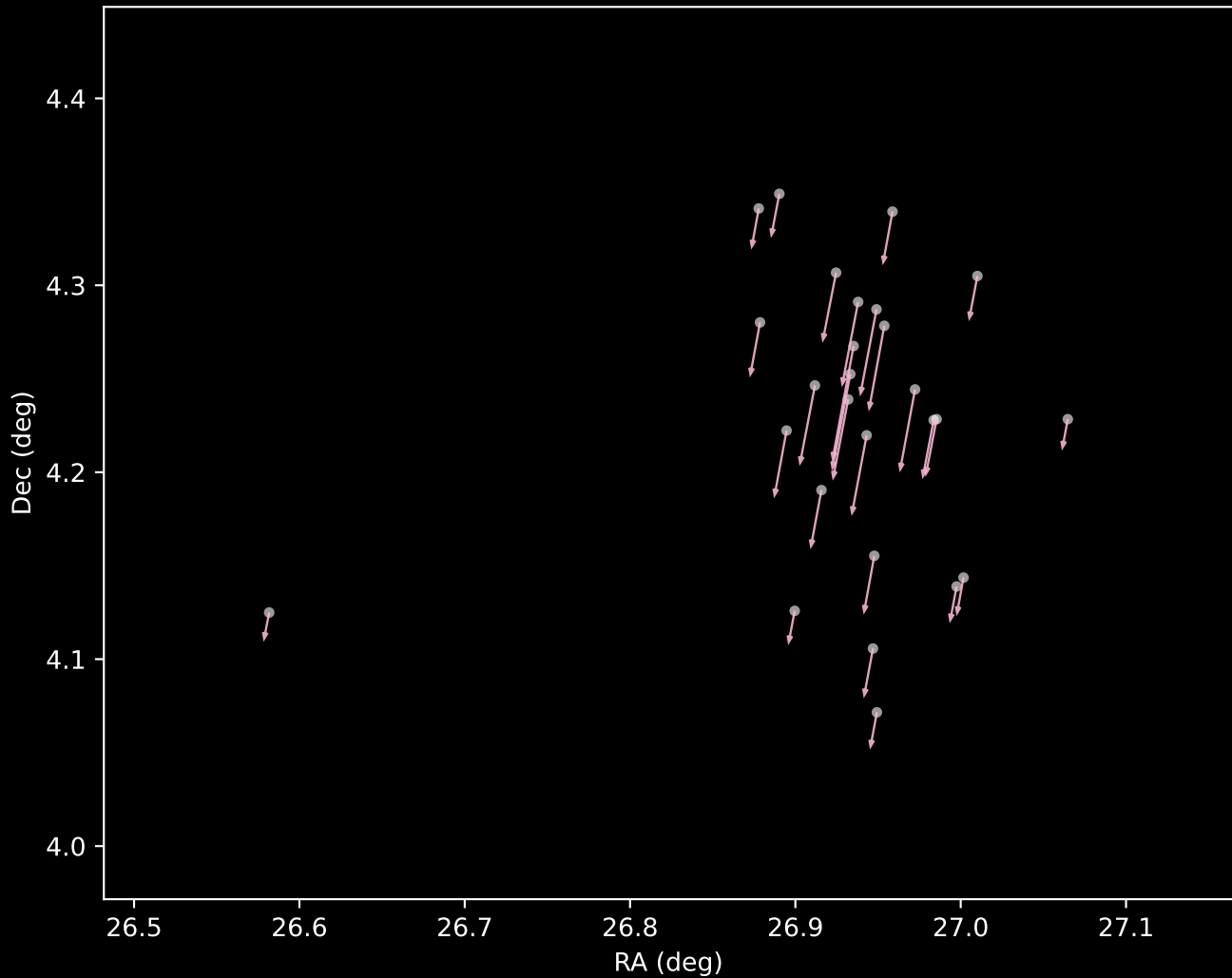
Gaia DR3 Cluster 73 Proper Motion Vectors (n=27)
