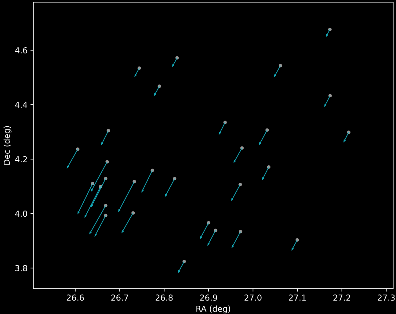
Gaia DR3 Cluster 38 Proper Motion Vectors (n=29)
