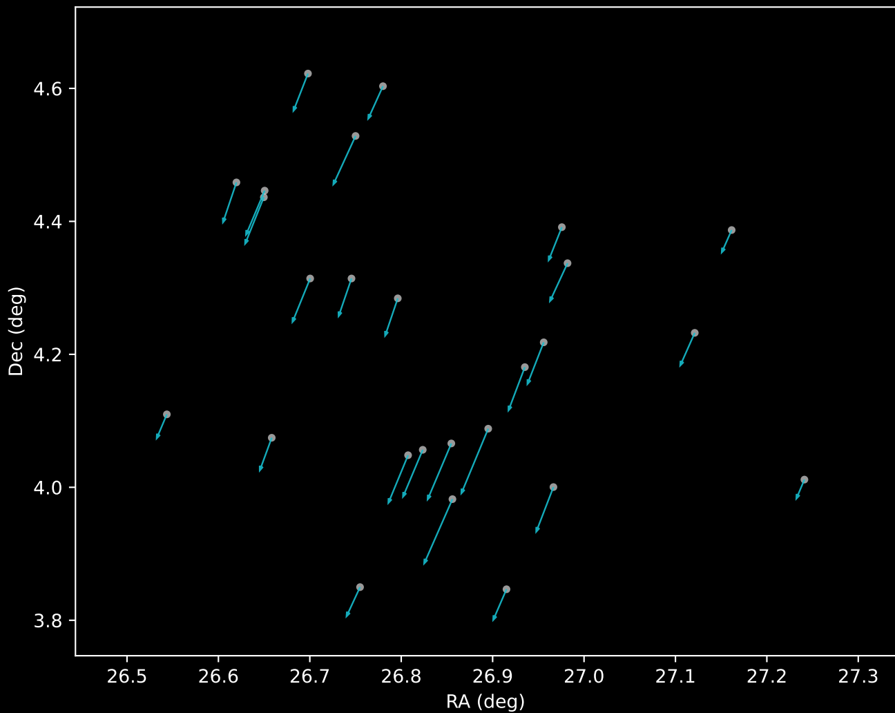
Gaia DR3 Cluster 18 Proper Motion Vectors (n=26)
