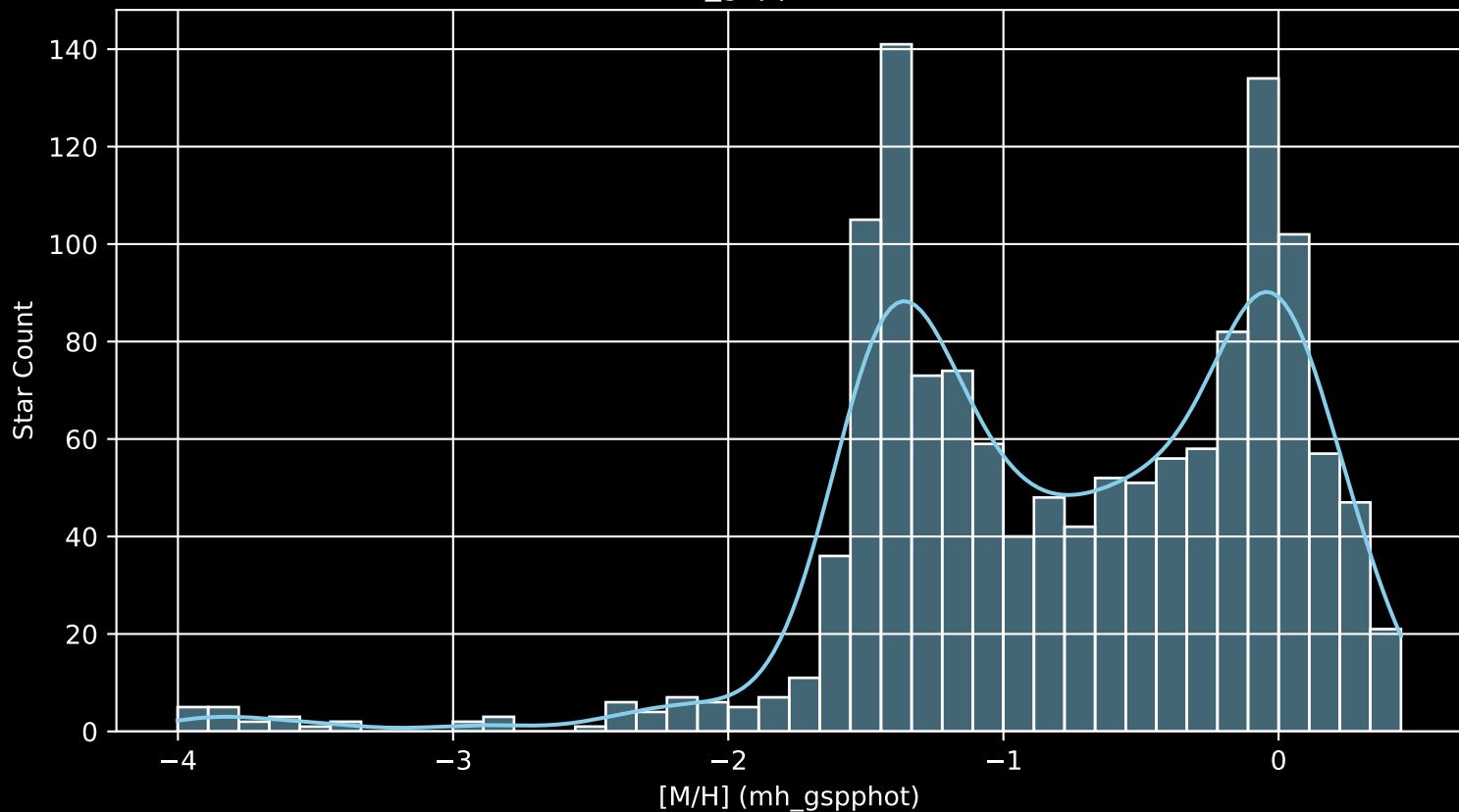
Gaia Cluster: [NGC_6755 [M/H] (mh_gspphot) (n= 1348)
