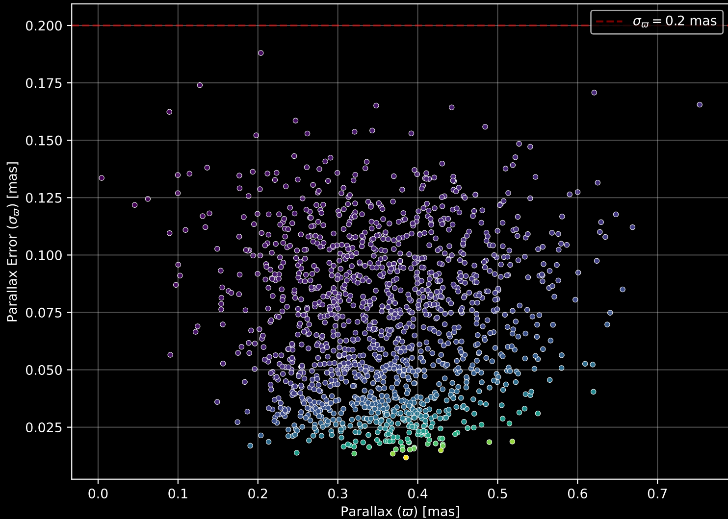
Gaia Cluster: [NGC_6755] Parallax Quality (n= 1379)
