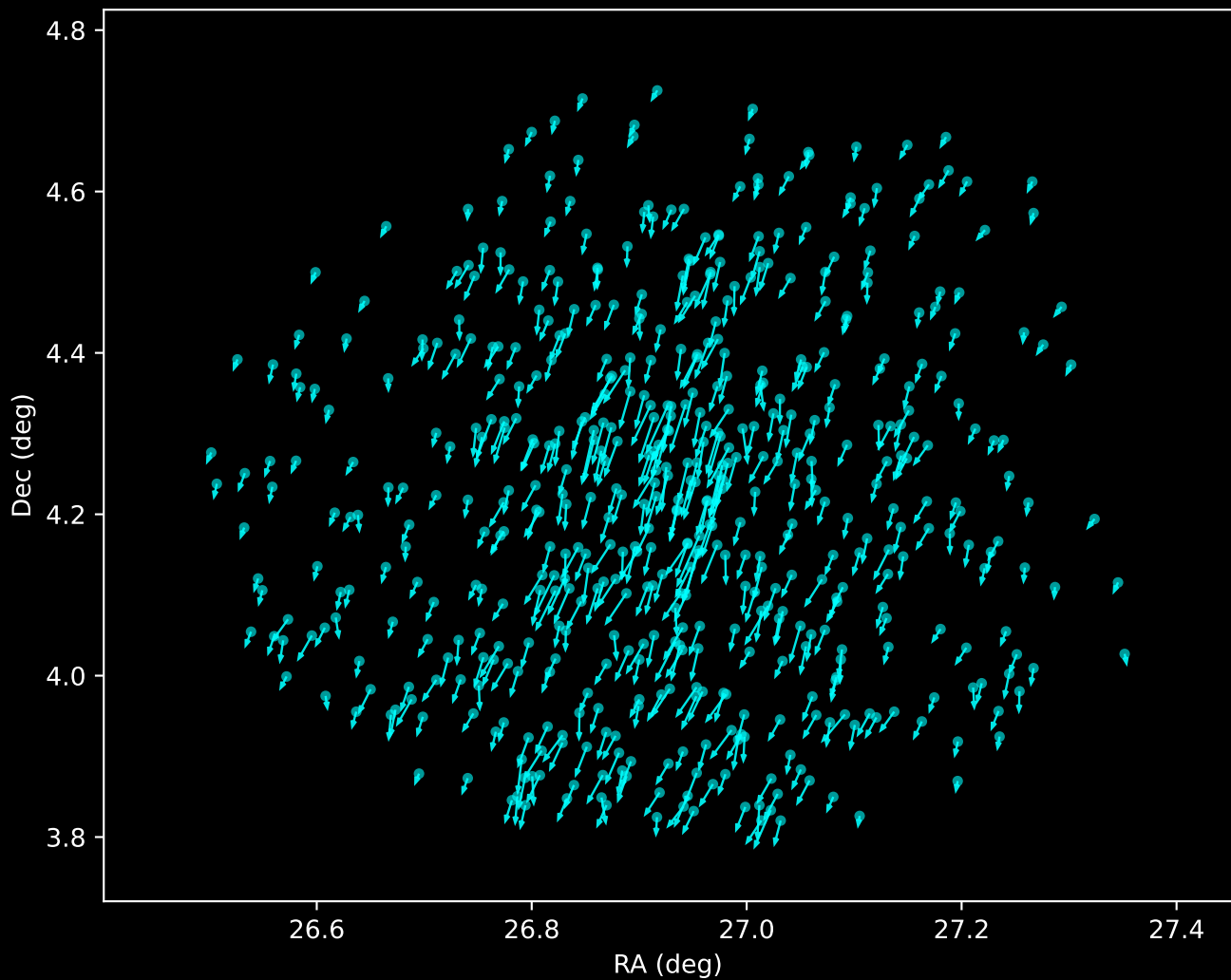
Gaia DR3 Noise Stream Proper Motion Vectors (n=532)
