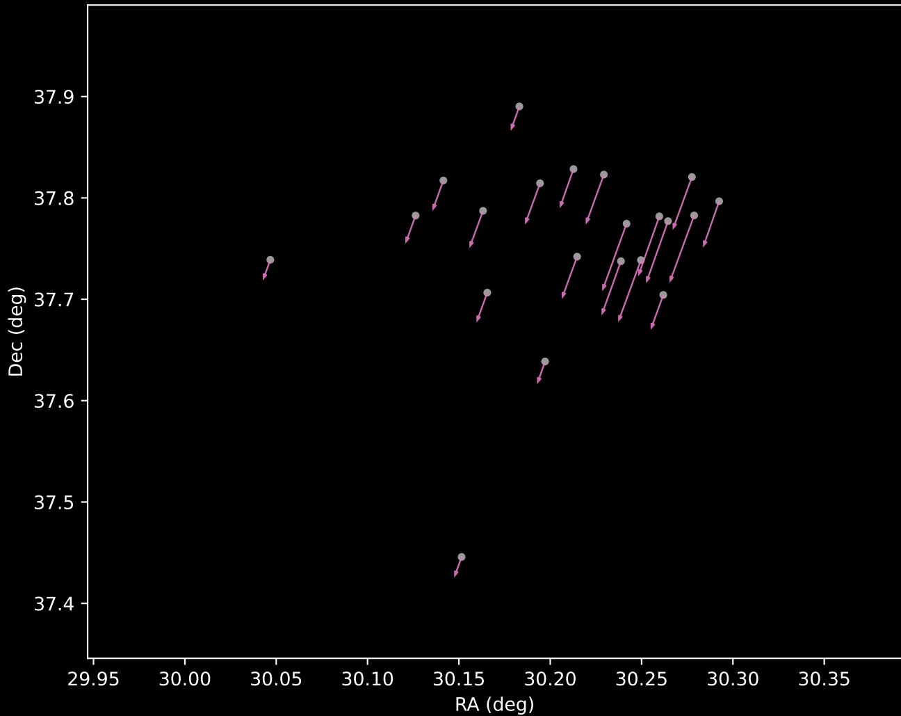
Gaia DR3 Cluster 72 Proper Motion Vectors (n=21)
