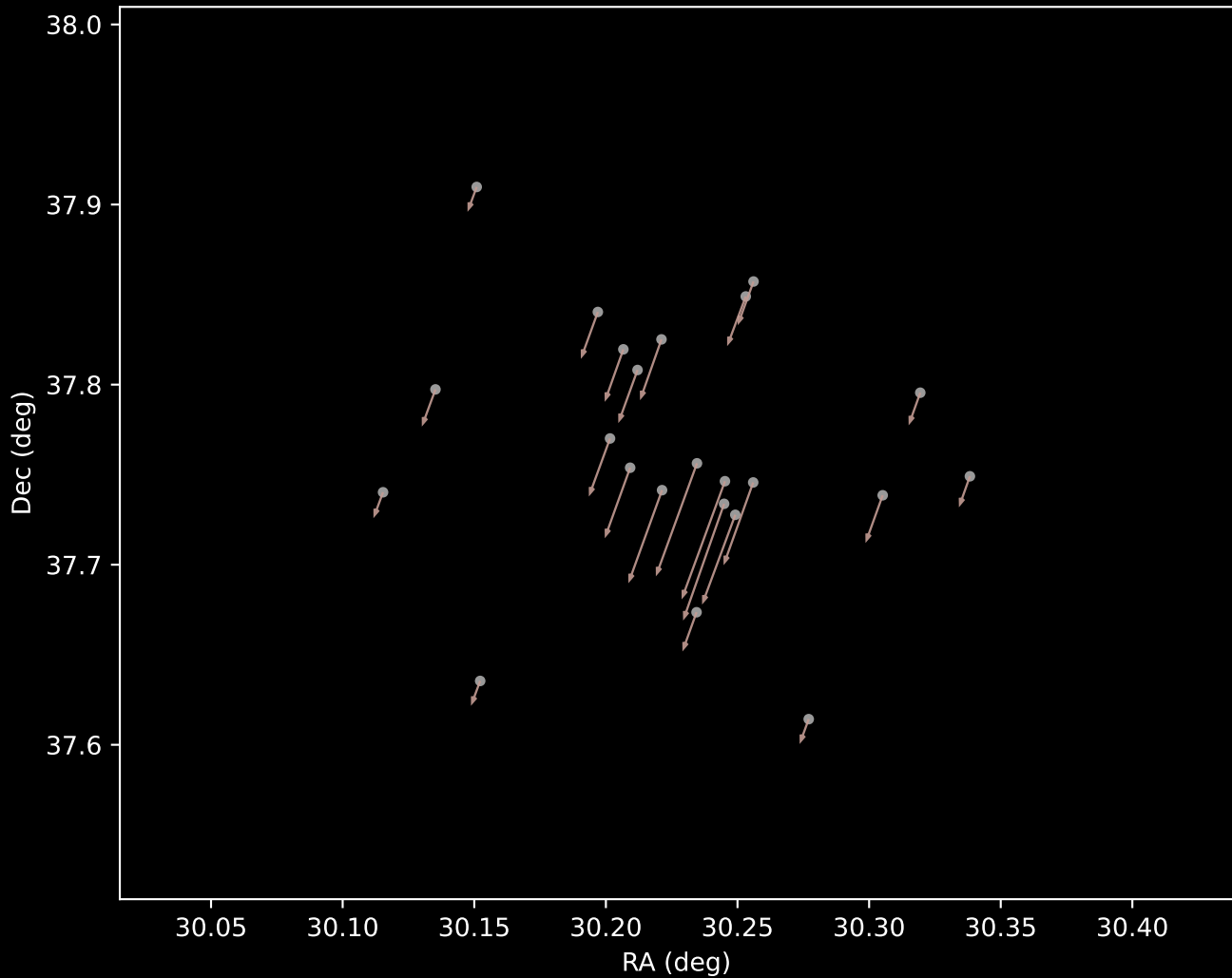
Gaia DR3 Cluster 31 Proper Motion Vectors (n=23)
