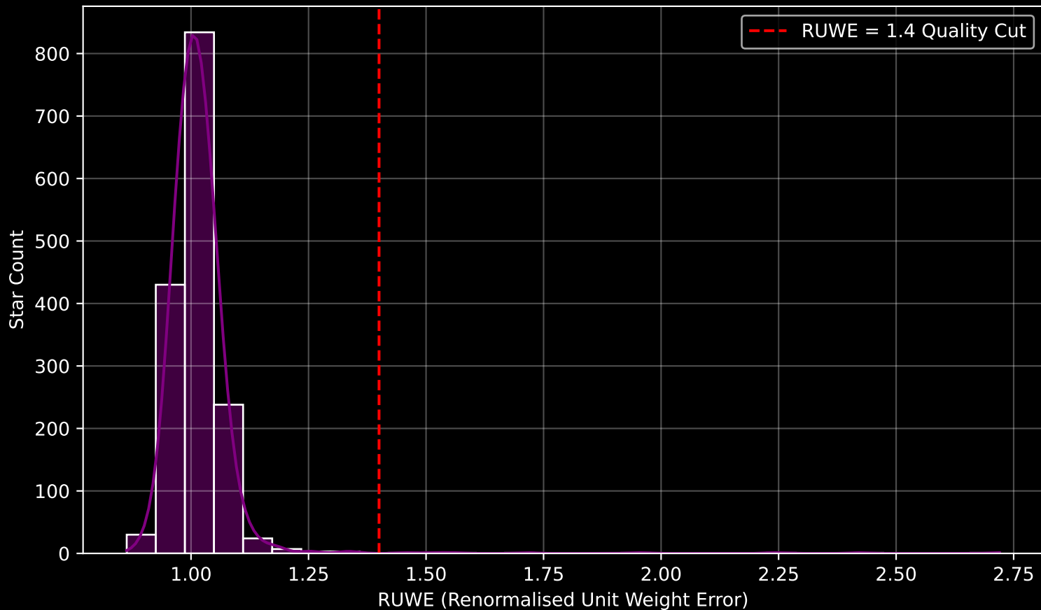
Gaia Cluster: [NGC_6791] RUWE Distribution (n= 1577)
