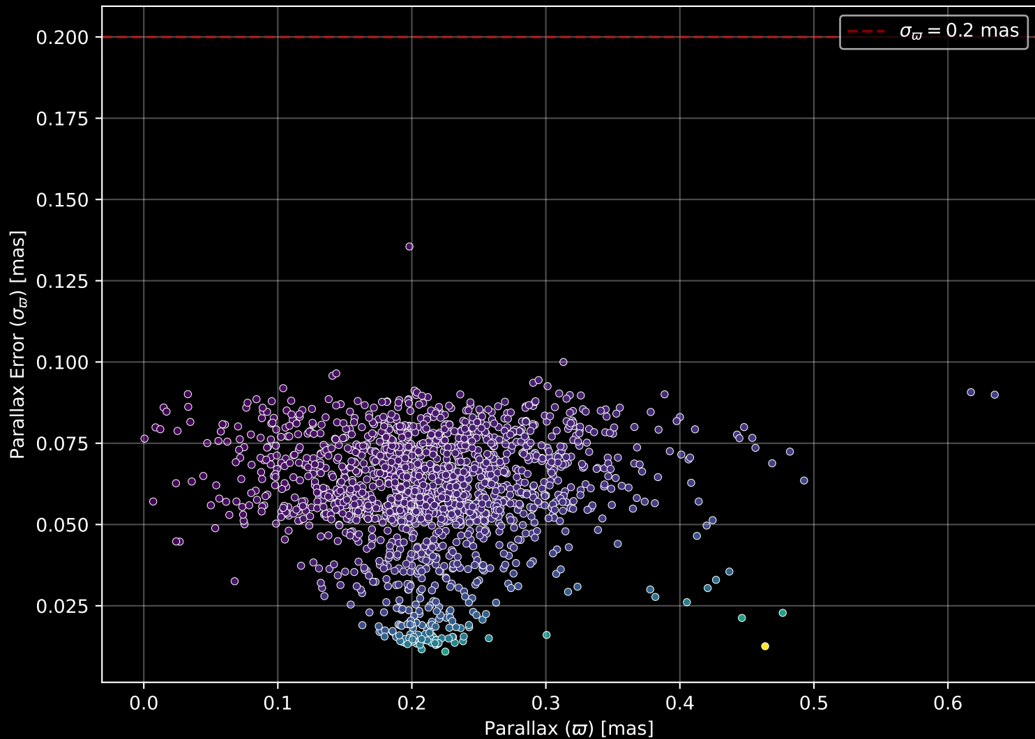
Gaia Cluster: [NGC_6791] Parallax Quality (n= 1577)
