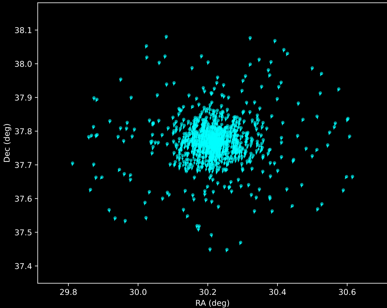
Gaia DR3 Noise Stream Proper Motion Vectors (n=698)
