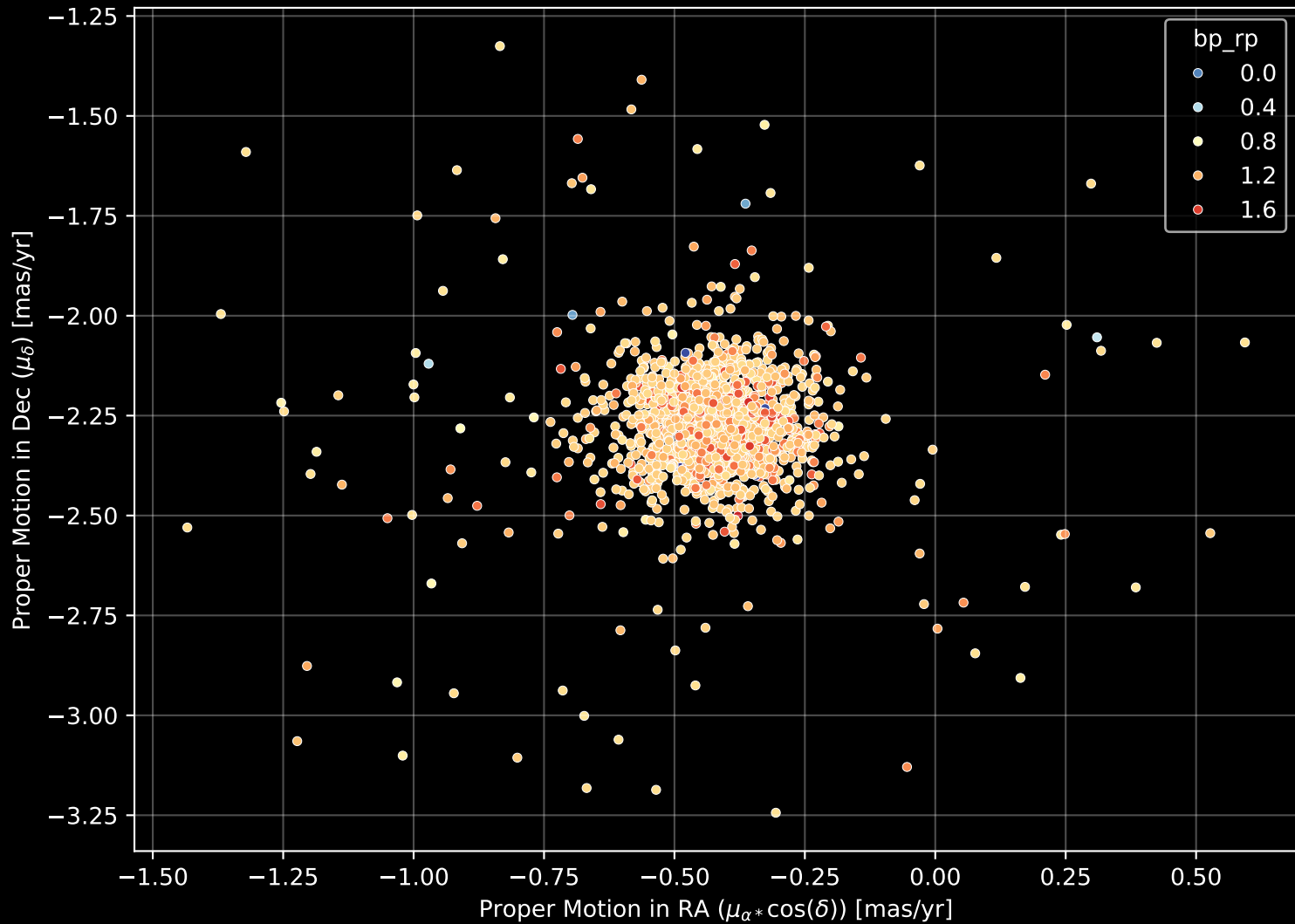
Gaia Cluster: [NGC_6791] Proper Motion Diagram (n= 1577)
