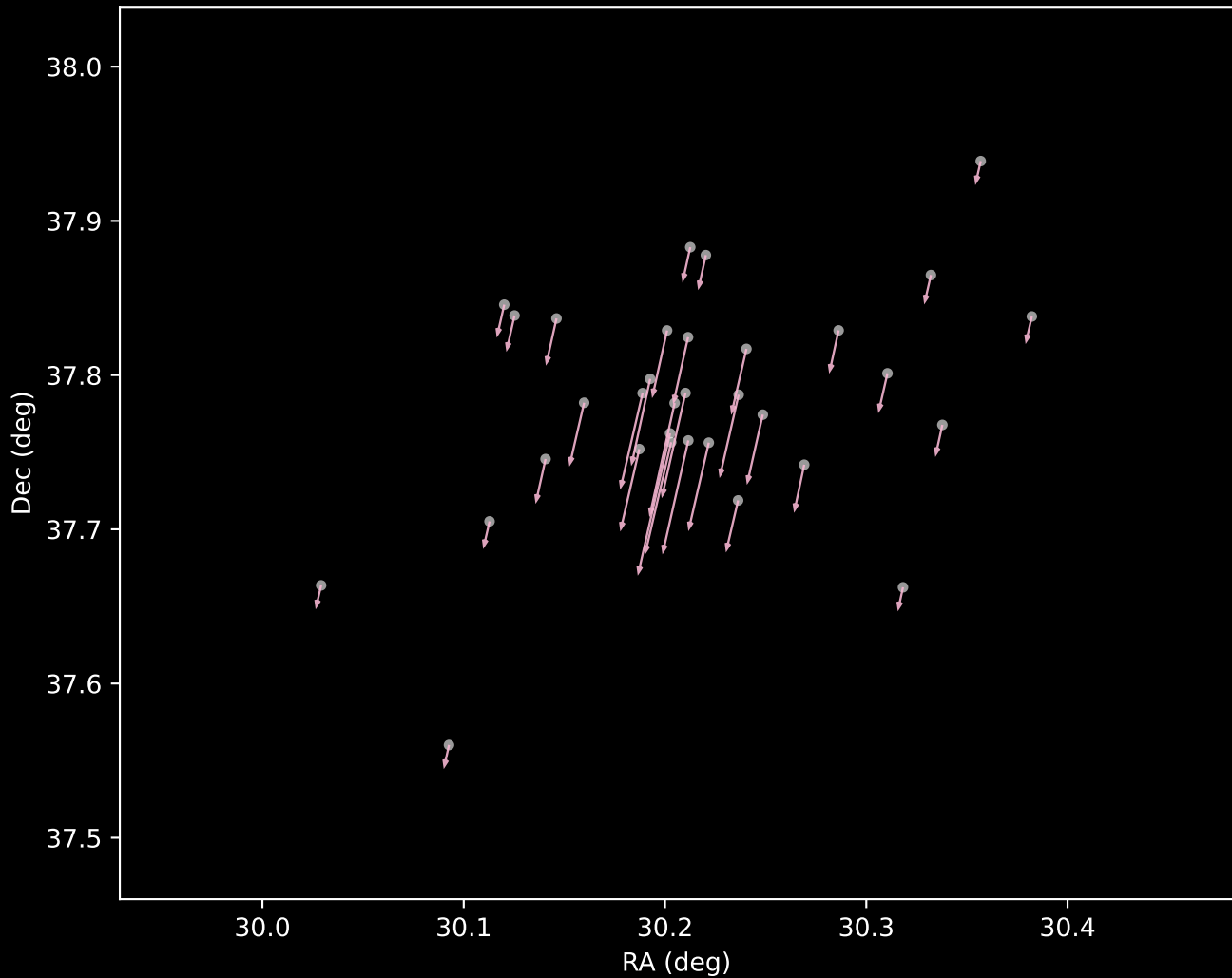
Gaia DR3 Cluster 53 Proper Motion Vectors (n=33)
