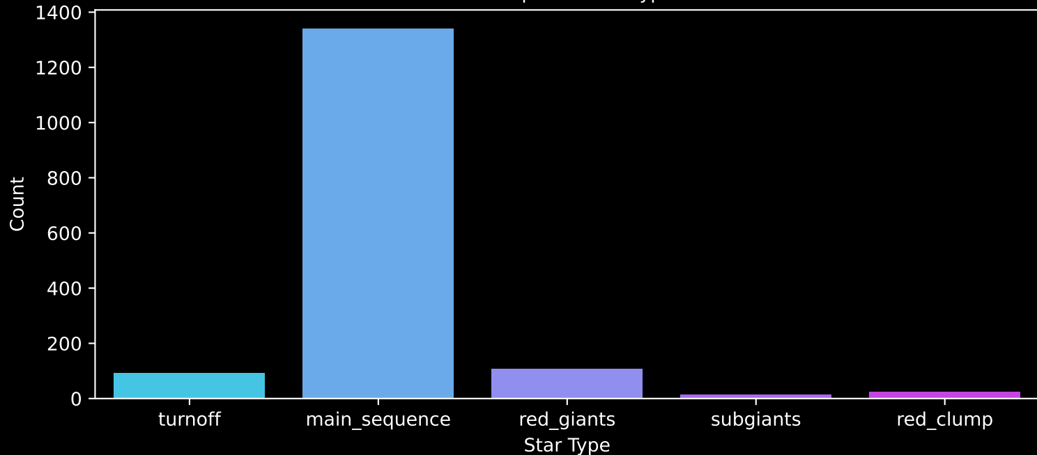
Gaia Cluster: [NGC_6791] Count plot of Star Type
