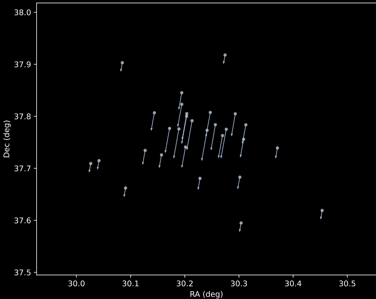
Gaia DR3 Cluster 61 Proper Motion Vectors (n=29)
