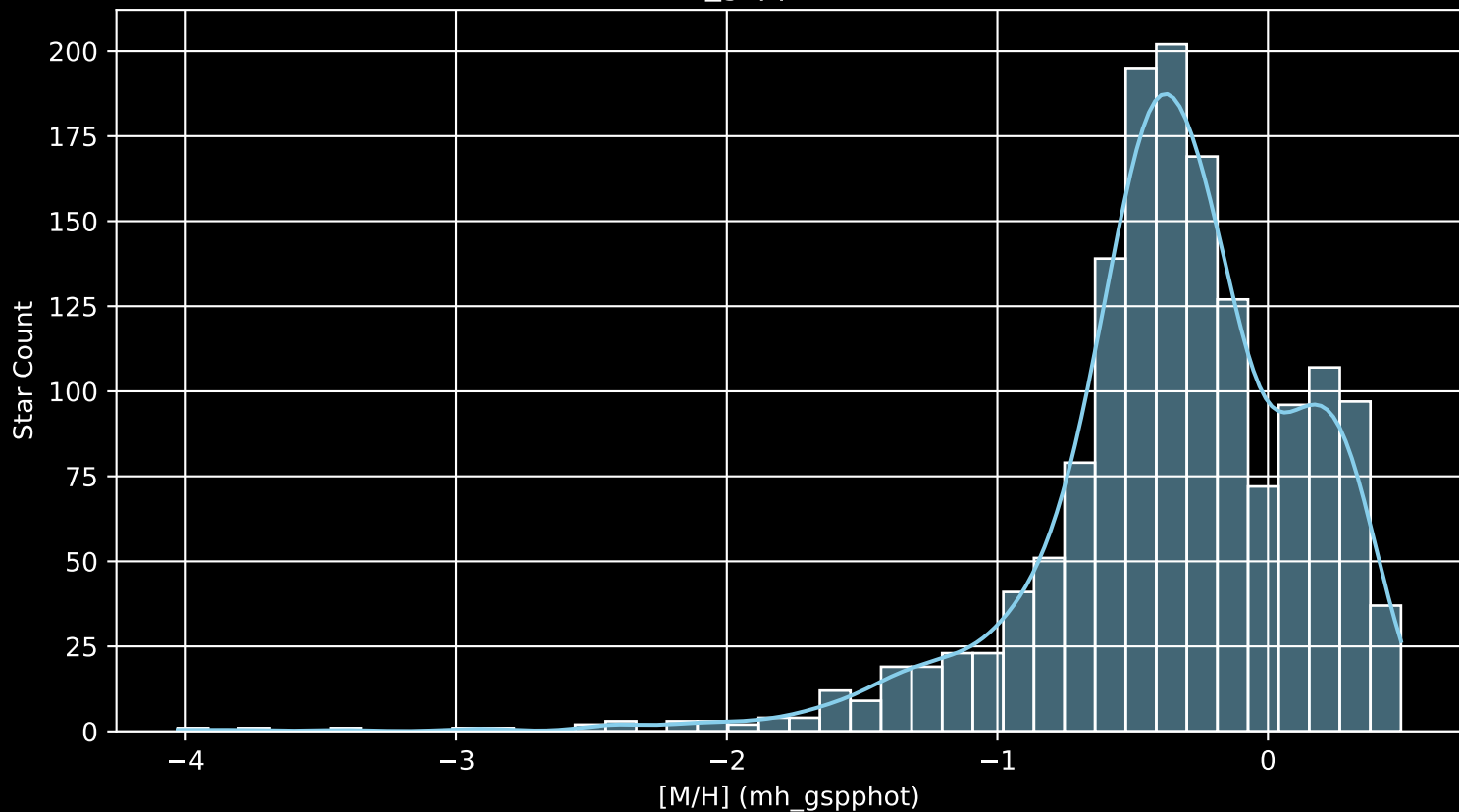
Gaia Cluster: [NGC_6791 [M/H] (mh_gspphot) (n= 1543)
