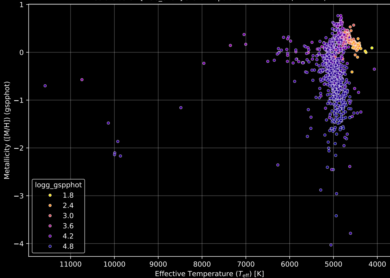
Gaia Cluster: [NGC_6791] Stellar Population Parameters (n= 1577)
