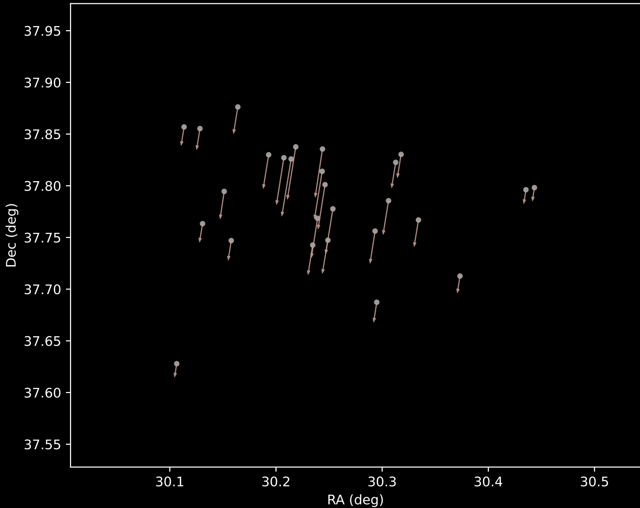
Gaia DR3 Cluster 51 Proper Motion Vectors (n=27)
