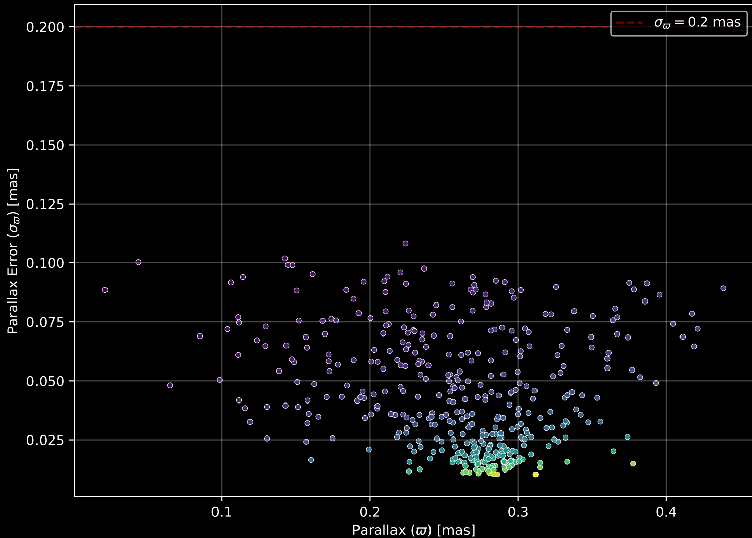
Gaia Cluster: [NGC_6834] Parallax Quality (n= 406)
