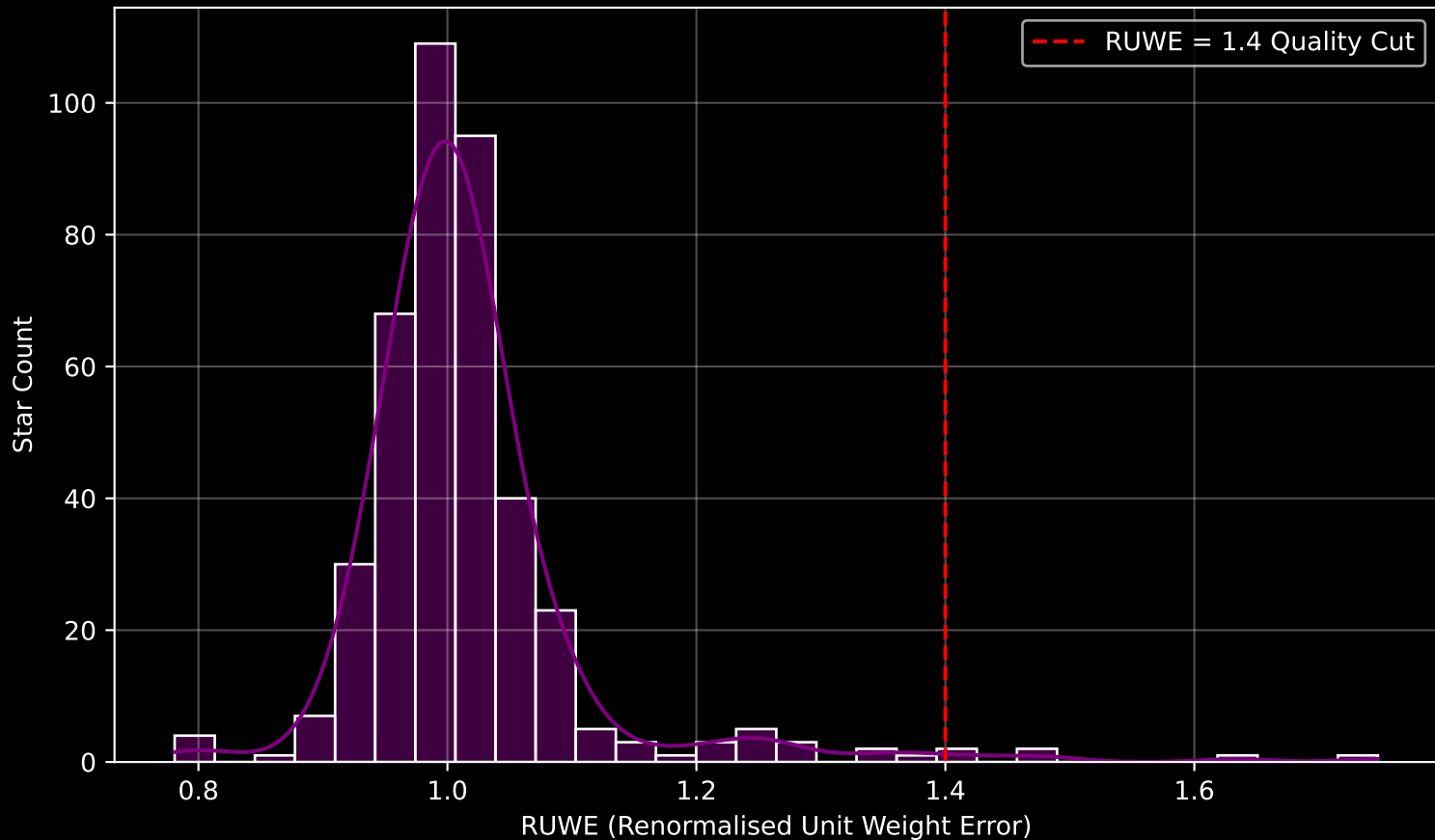
Gaia Cluster: [NGC_6834] RUWE Distribution (n= 406)
