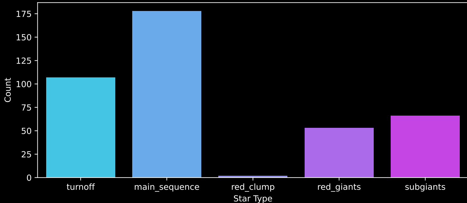
Gaia Cluster: [NGC_6834] Count plot of Star Type
