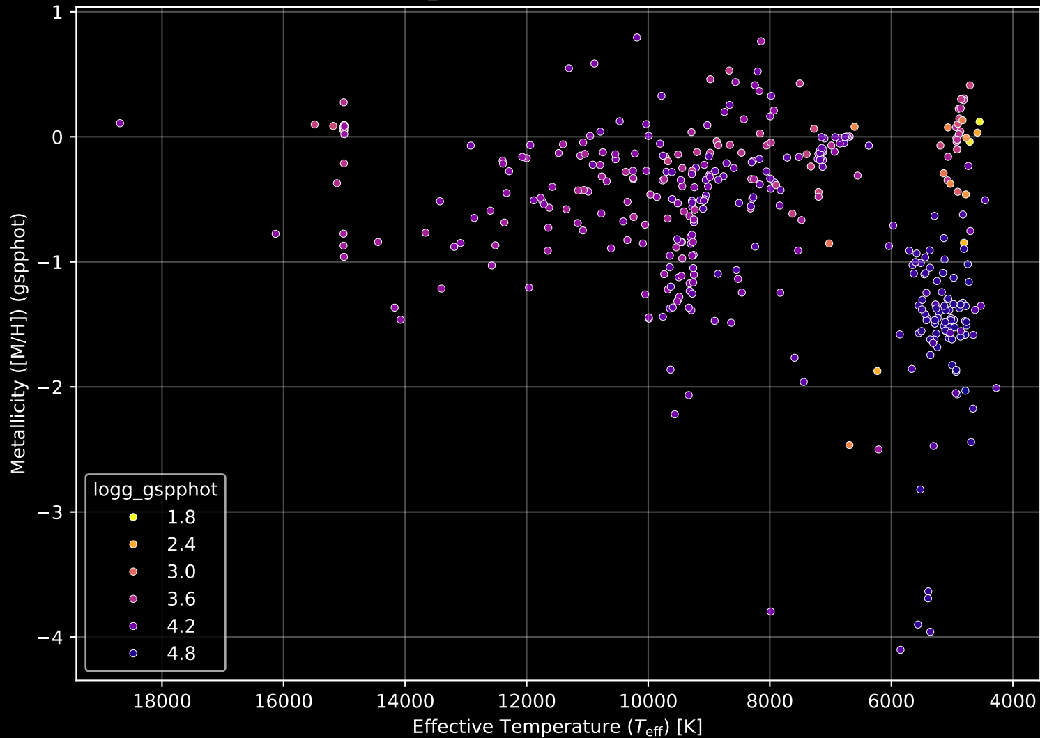
Gaia Cluster: [NGC_6834] Stellar Population Parameters (n= 406)
