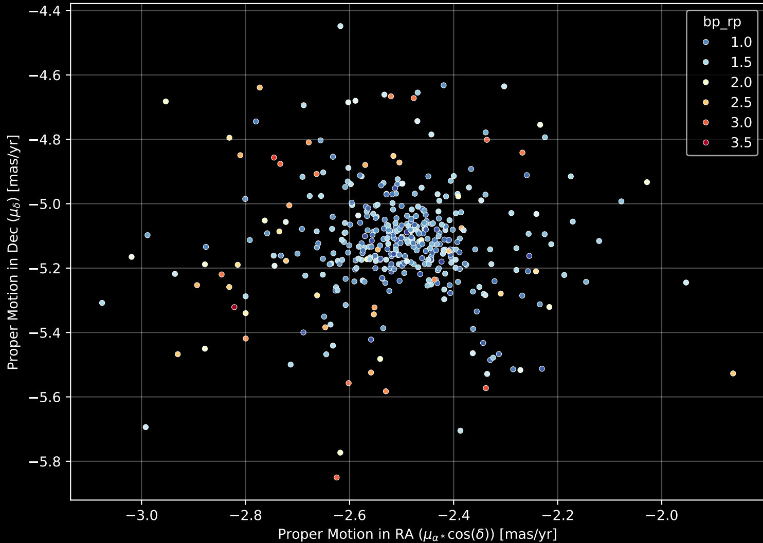
Gaia Cluster: [NGC_6834] Proper Motion Diagram (n= 406)
