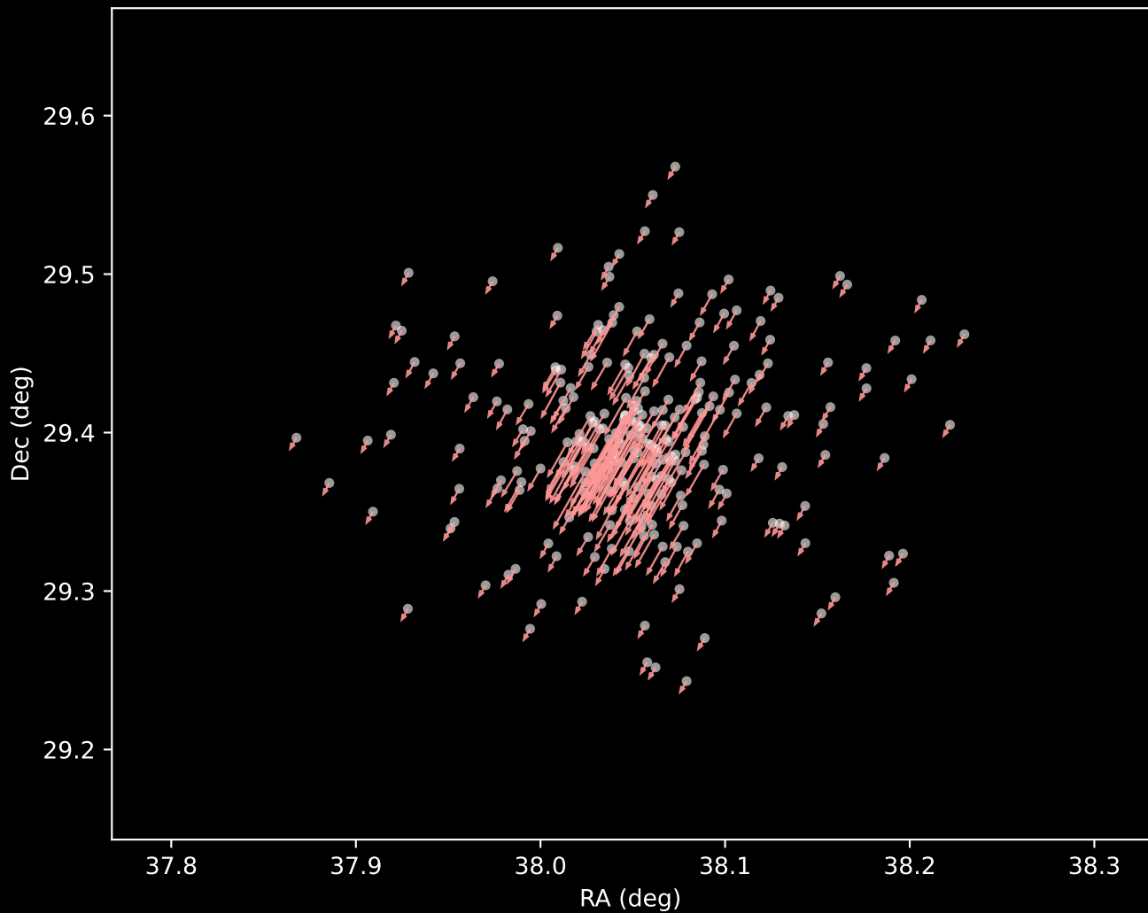
Gaia DR3 Cluster 7 Proper Motion Vectors (n=262)
