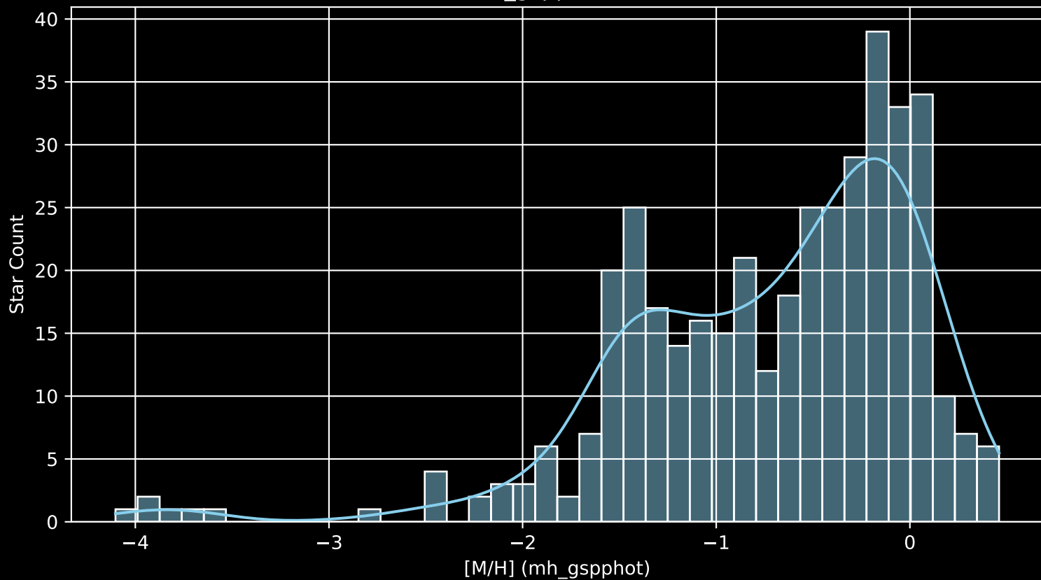
Gaia Cluster: [NGC_6834 [M/H] (mh_gspphot) (n= 400)
