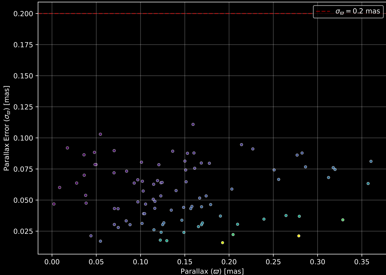
Gaia Cluster: [NGC_6846] Parallax Quality (n= 94)
