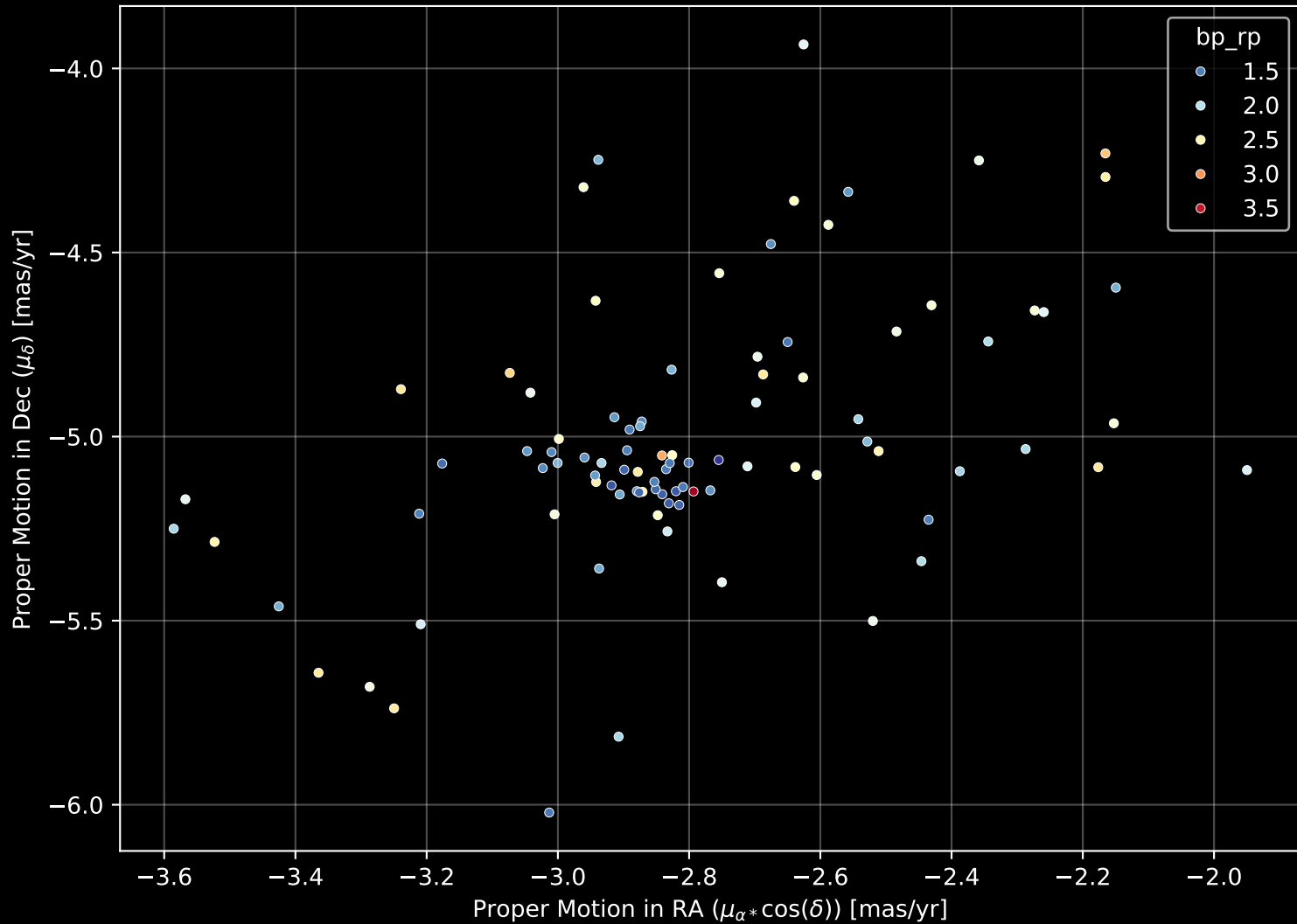
Gaia Cluster: [NGC_6846] Proper Motion Diagram (n= 94)
