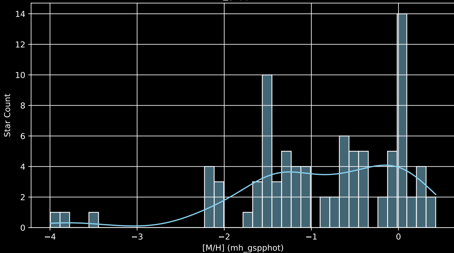
Gaia Cluster: [NGC_6846 [M/H] (mh_gspphot) (n= 89)
