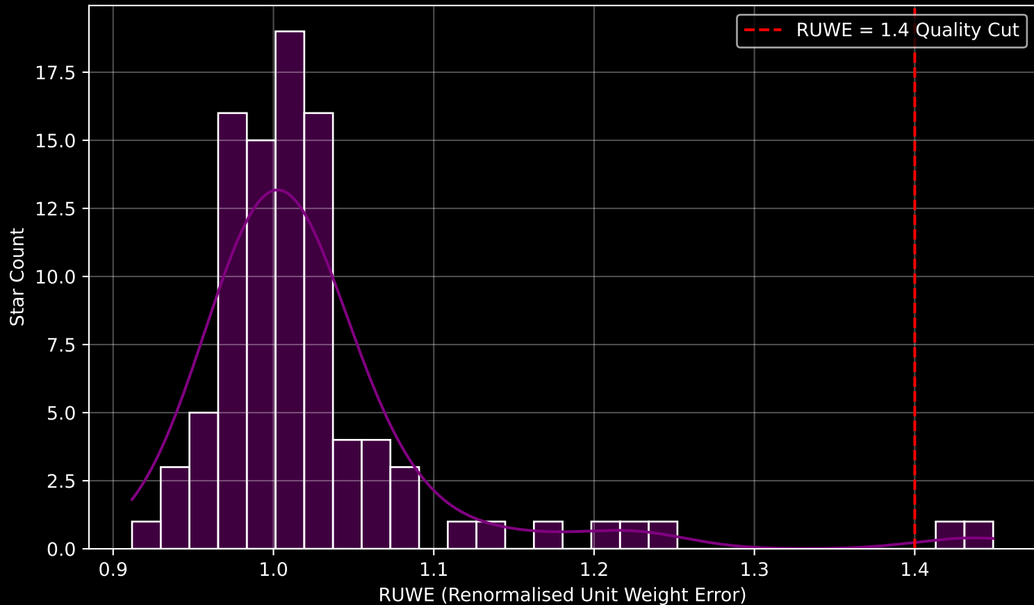
Gaia Cluster: [NGC_6846] RUWE Distribution (n= 94)
