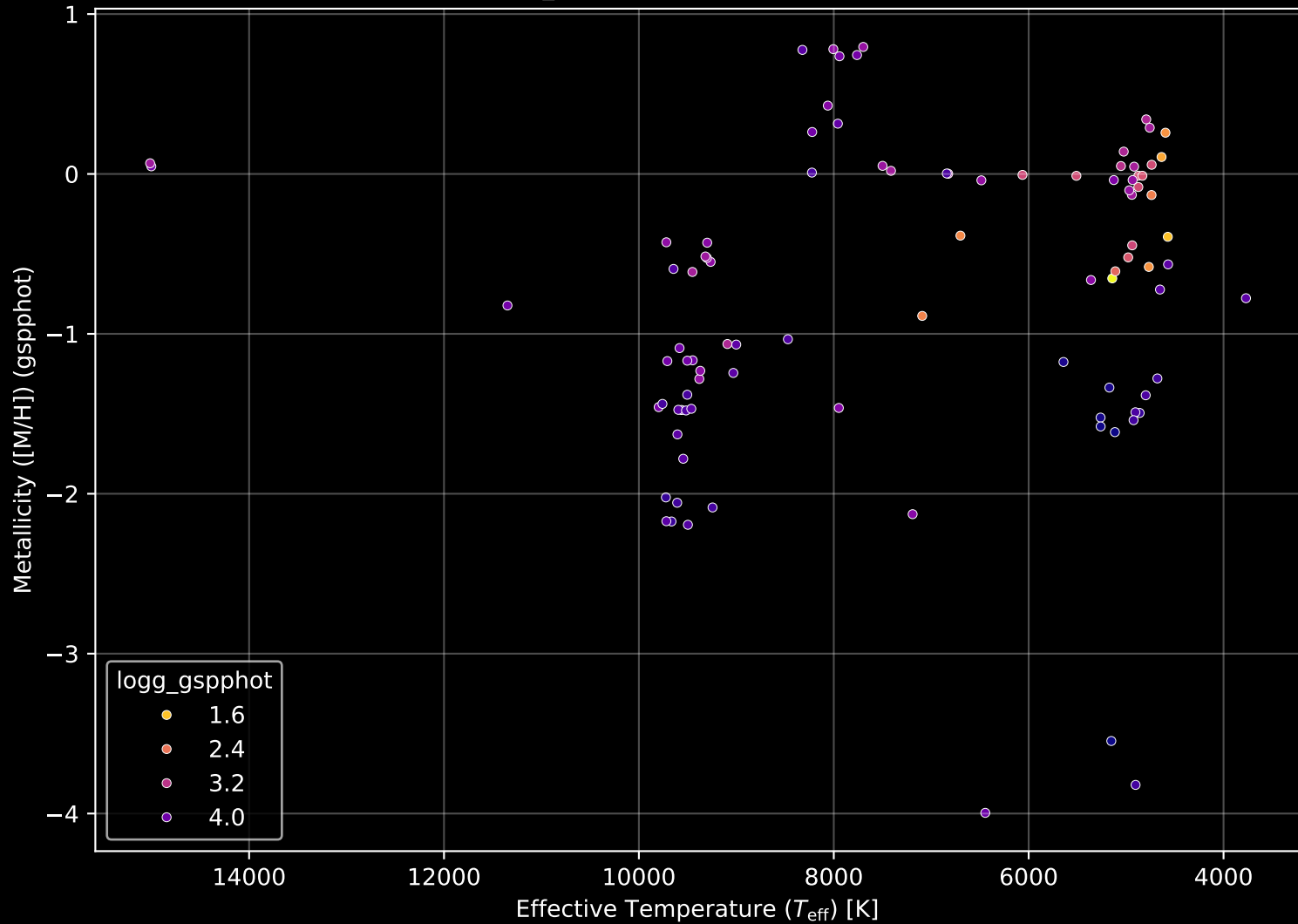
Gaia Cluster: [NGC_6846] Stellar Population Parameters (n= 94)
