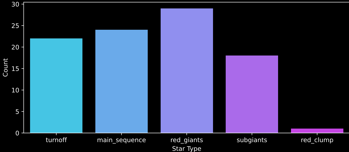
Gaia Cluster: [NGC_6846] Count plot of Star Type
