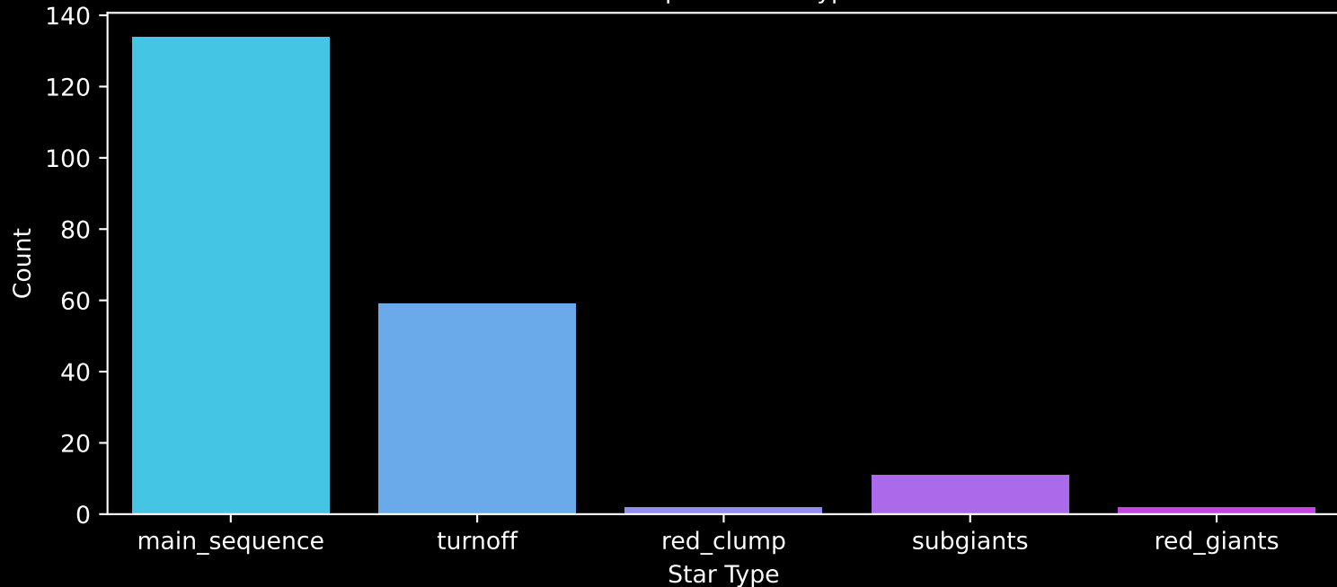
Gaia Cluster: [NGC_6866] Count plot of Star Type
