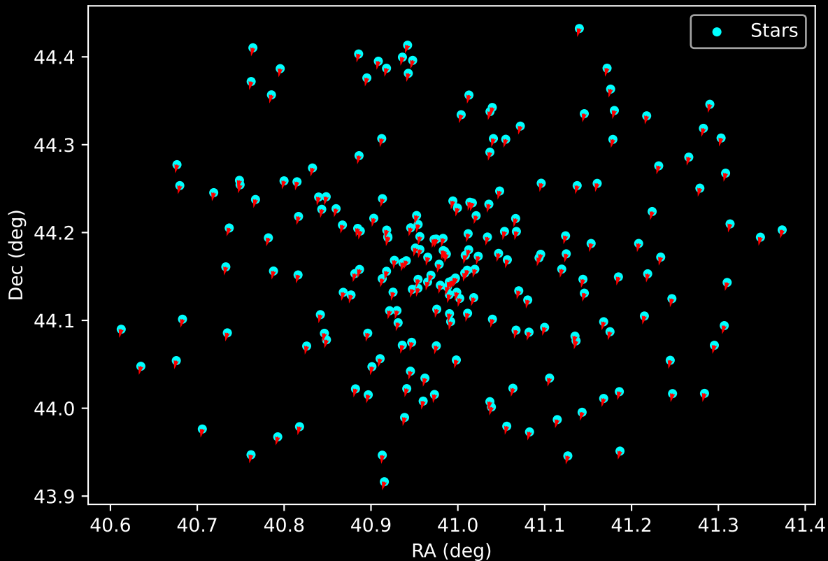
Gaia Cluster: [NGC_6866] Proper Motion Vectors for Gaia Star Field (n= 208)
