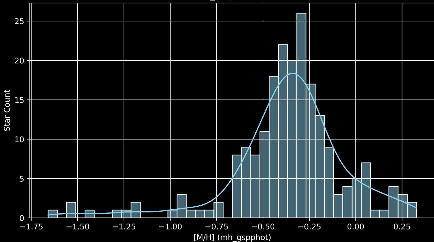
Gaia Cluster: [NGC_6866 [M/H] (mh_gspphot) (n= 208)
