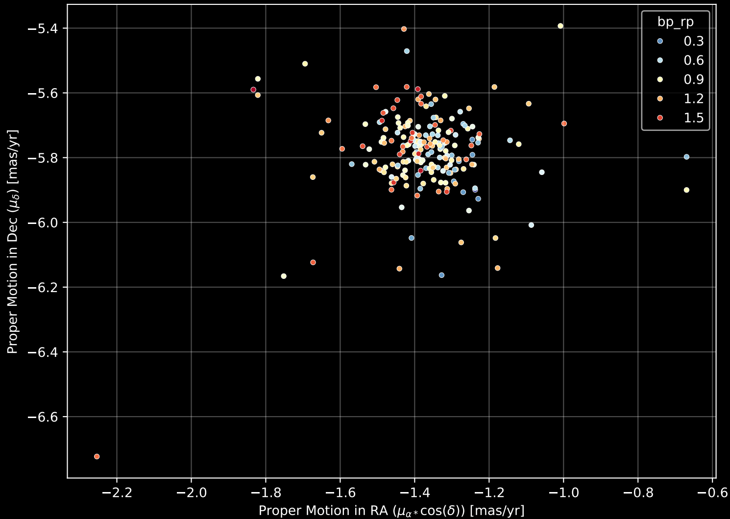
Gaia Cluster: [NGC_6866] Proper Motion Diagram (n= 208)
