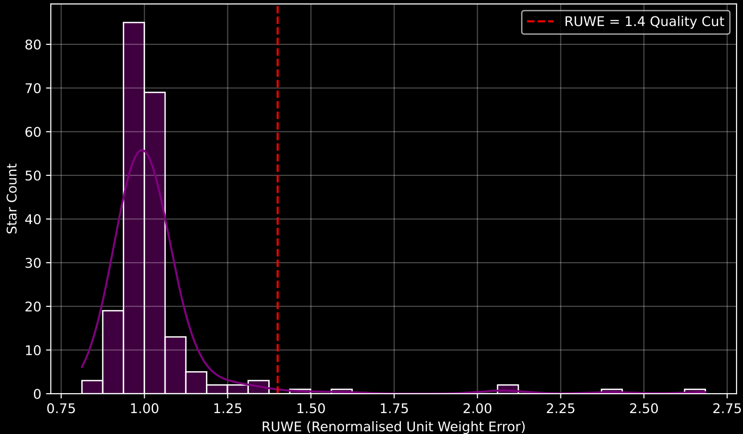
Gaia Cluster: [NGC_6866] RUWE Distribution (n= 207)
