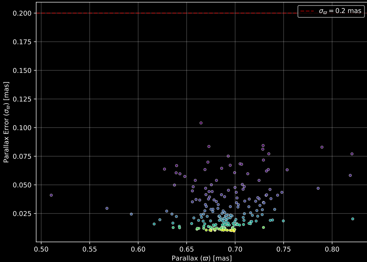
Gaia Cluster: [NGC_6866] Parallax Quality (n= 208)
