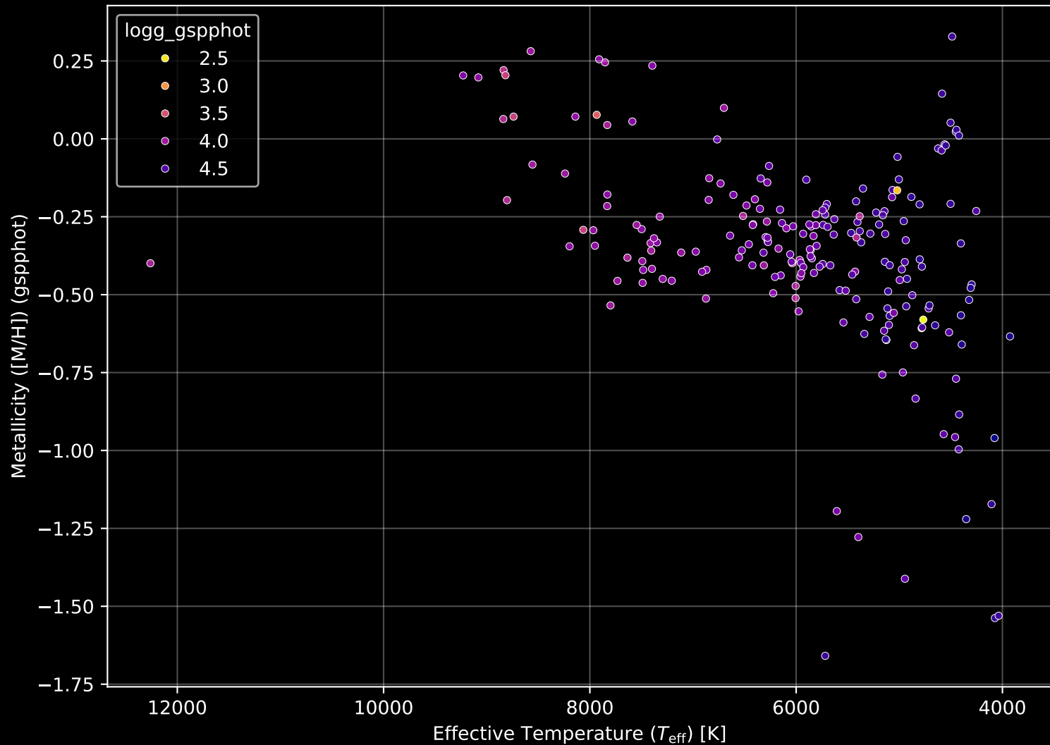
Gaia Cluster: [NGC_6866] Stellar Population Parameters (n= 208)
