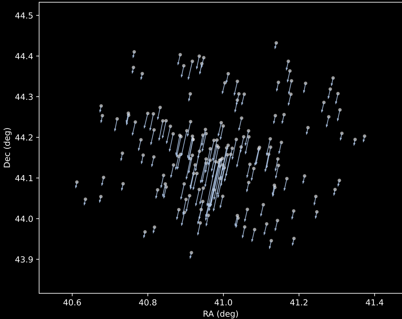
Gaia DR3 Cluster 1 Proper Motion Vectors (n=158)
