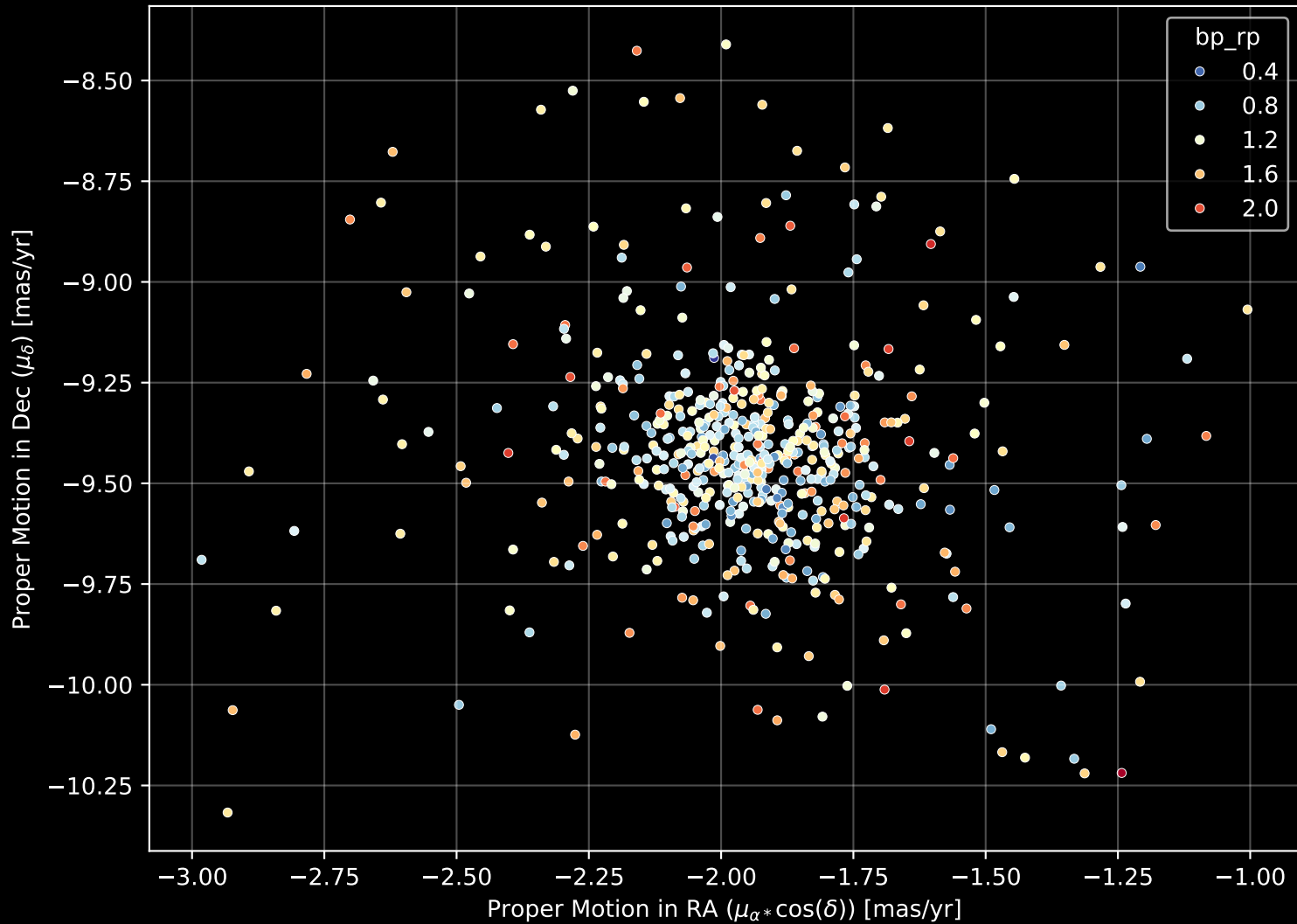
Gaia Cluster: [NGC_6940] Proper Motion Diagram (n= 559)
