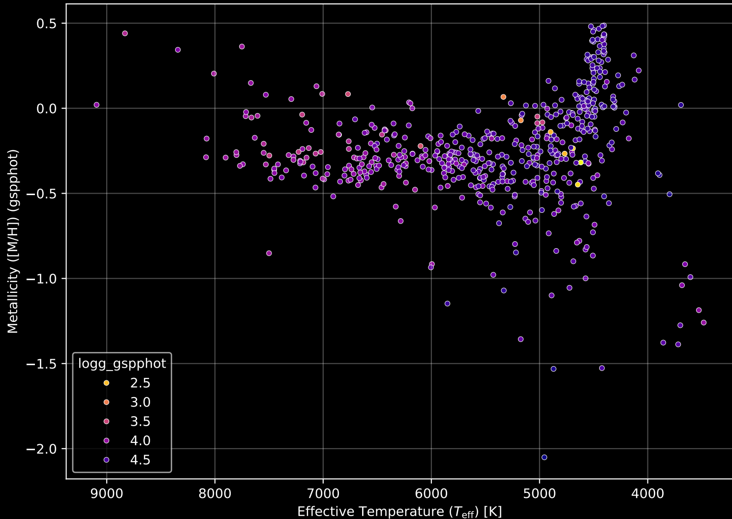
Gaia Cluster: [NGC_6940] Stellar Population Parameters (n= 559)
