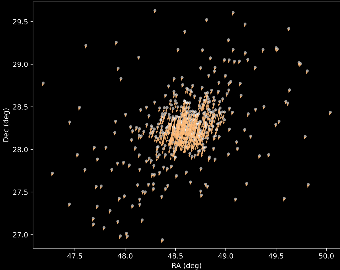
Gaia DR3 Cluster 3 Proper Motion Vectors (n=486)
