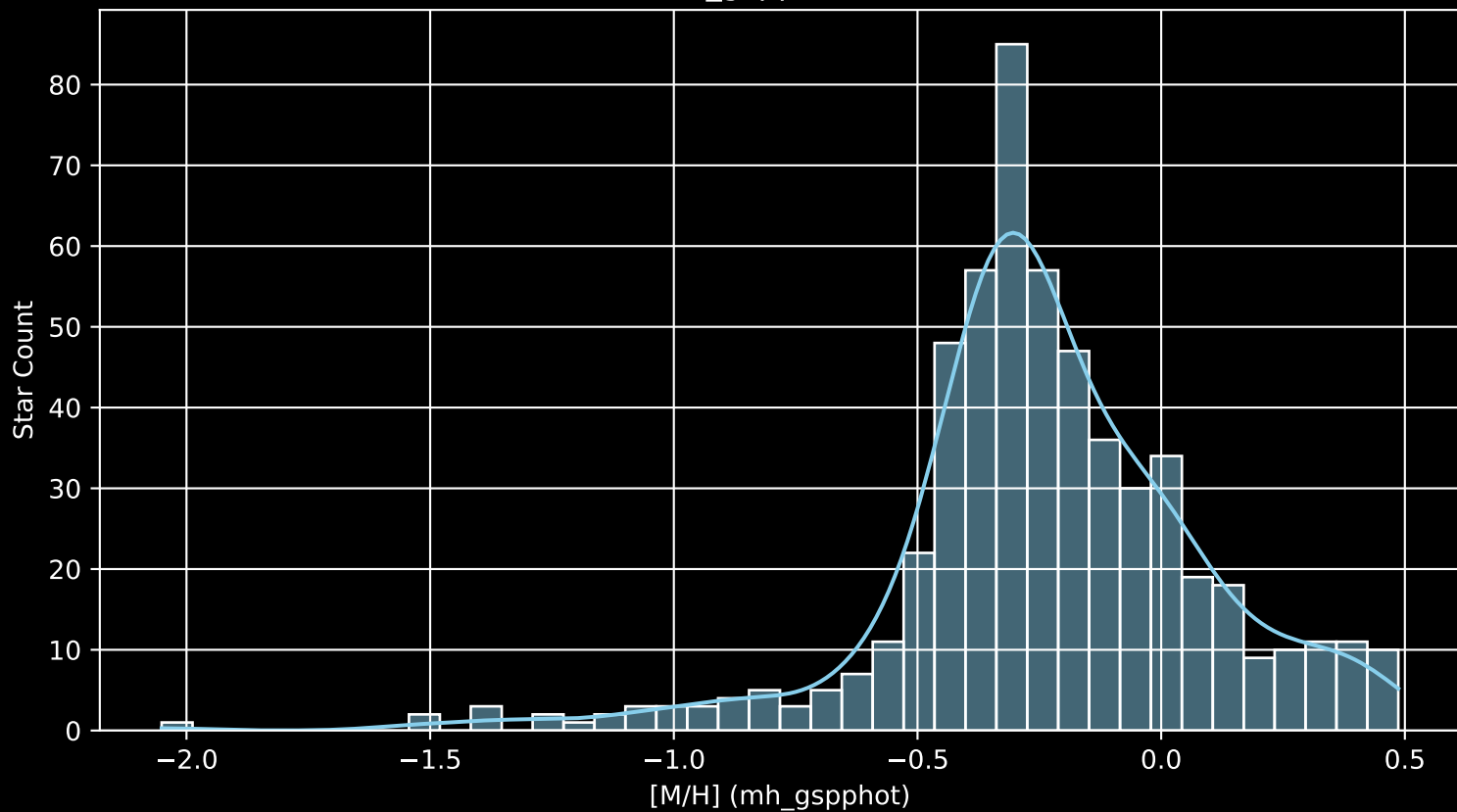
Gaia Cluster: [NGC_6940 [M/H] (mh_gspphot) (n= 559)
