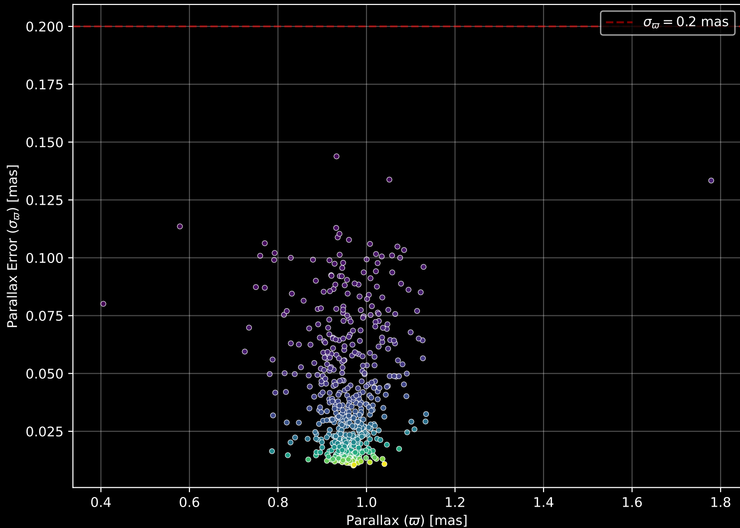
Gaia Cluster: [NGC_6940] Parallax Quality (n= 559)
