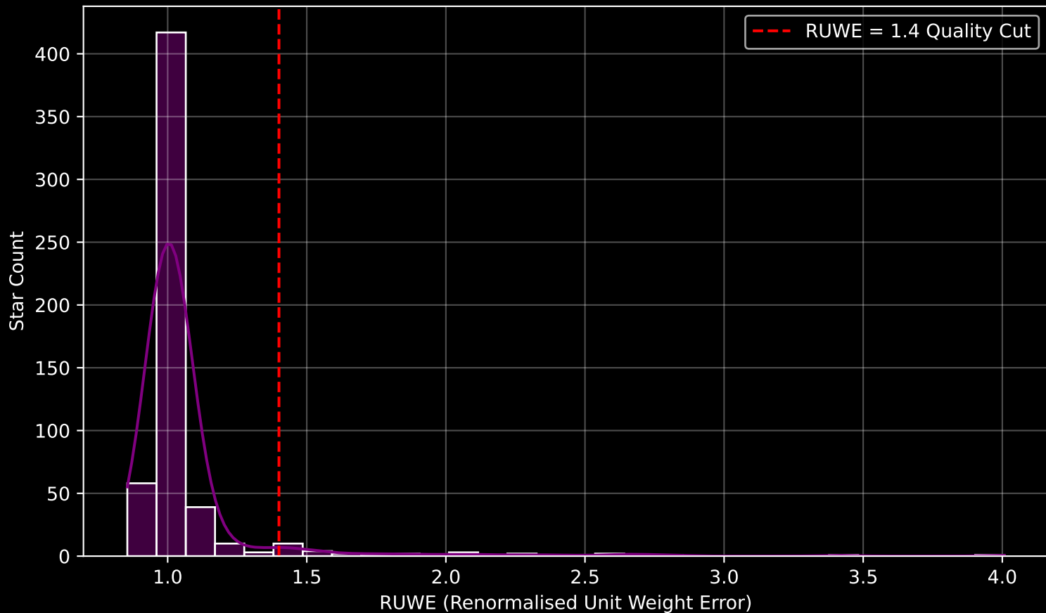
Gaia Cluster: [NGC_6940] RUWE Distribution (n= 559)
