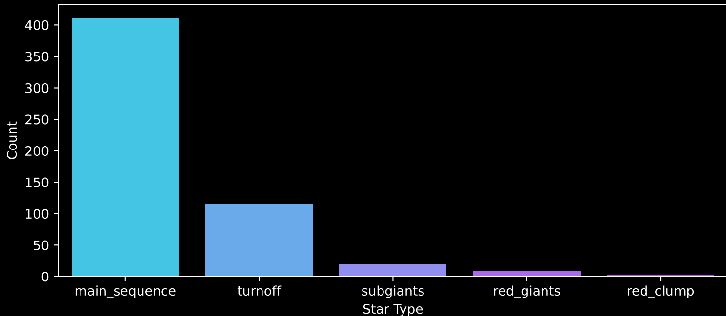
Gaia Cluster: [NGC_6940] Count plot of Star Type
