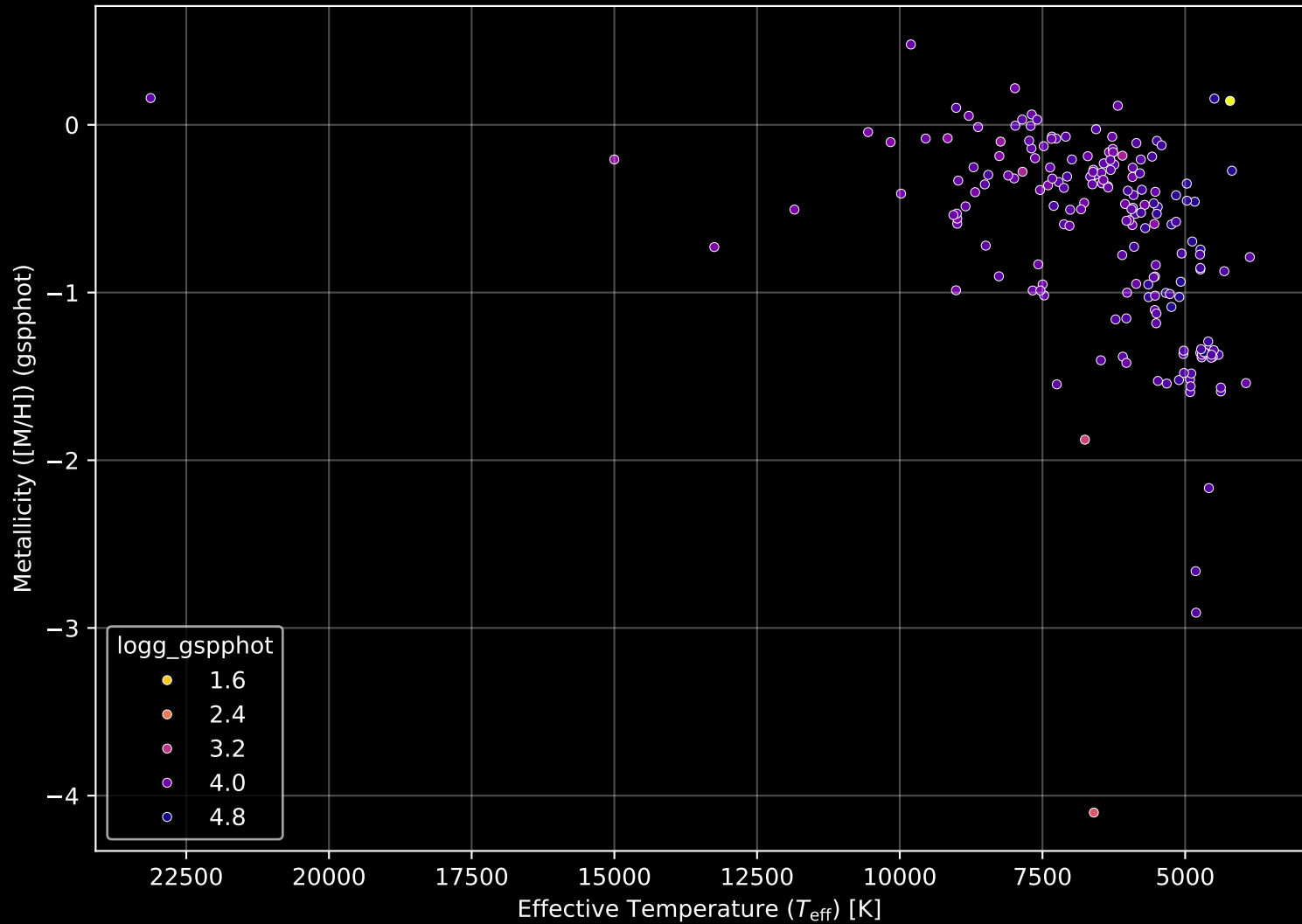
Gaia Cluster: [NGC_7031] Stellar Population Parameters (n= 187)
