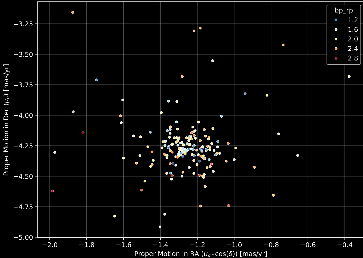
Gaia Cluster: [NGC_7031] Proper Motion Diagram (n= 187)
