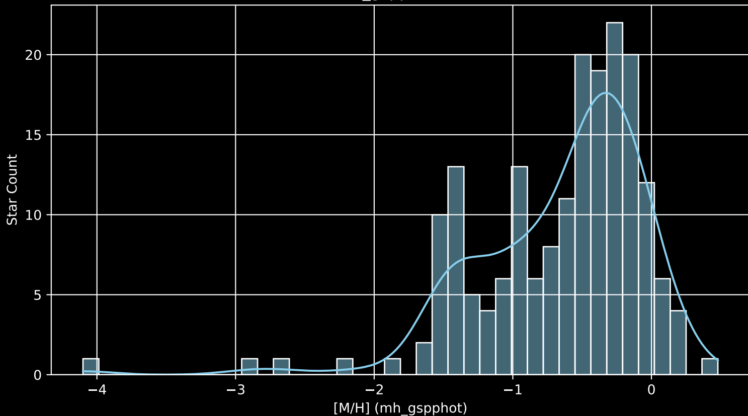
Gaia Cluster: [NGC_7031 [M/H] (mh_gspphot) (n= 187)
