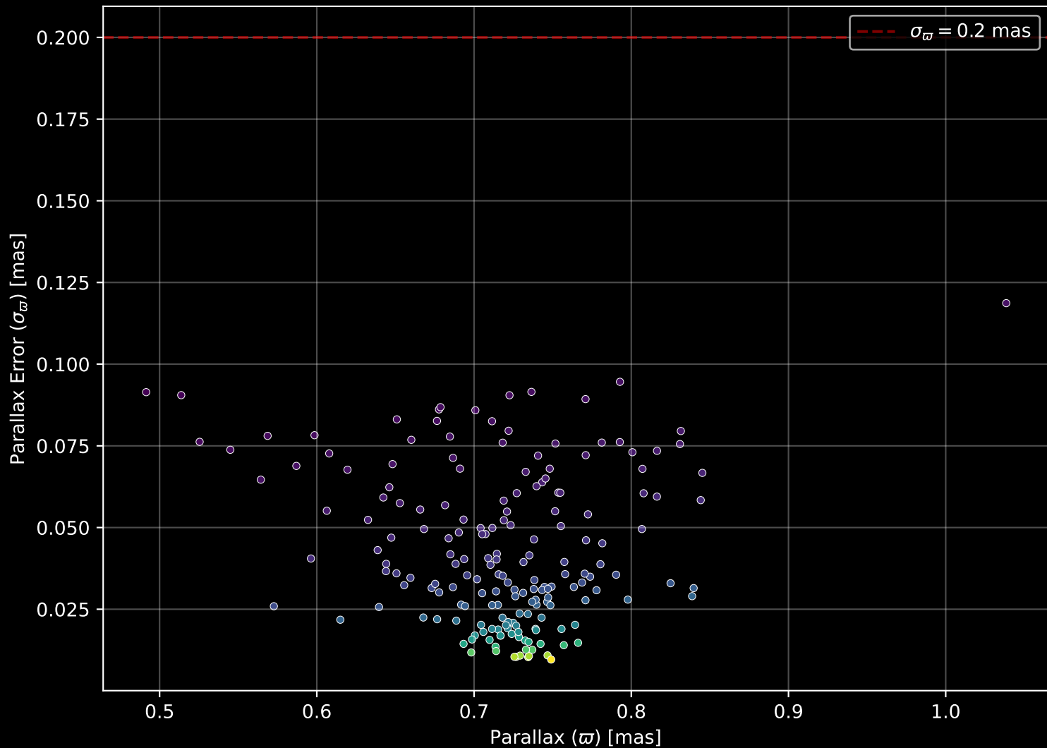
Gaia Cluster: [NGC_7031] Parallax Quality (n= 187)
