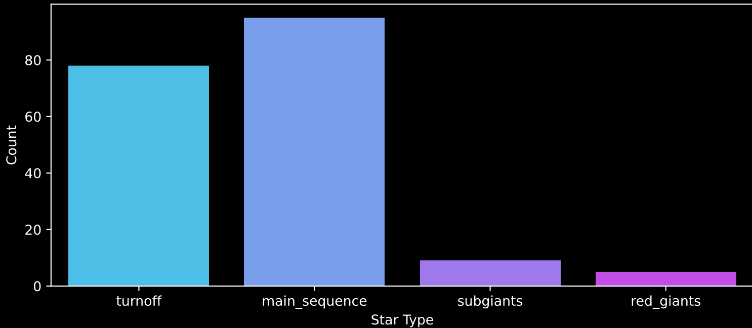
Gaia Cluster: [NGC_7031] Count plot of Star Type
