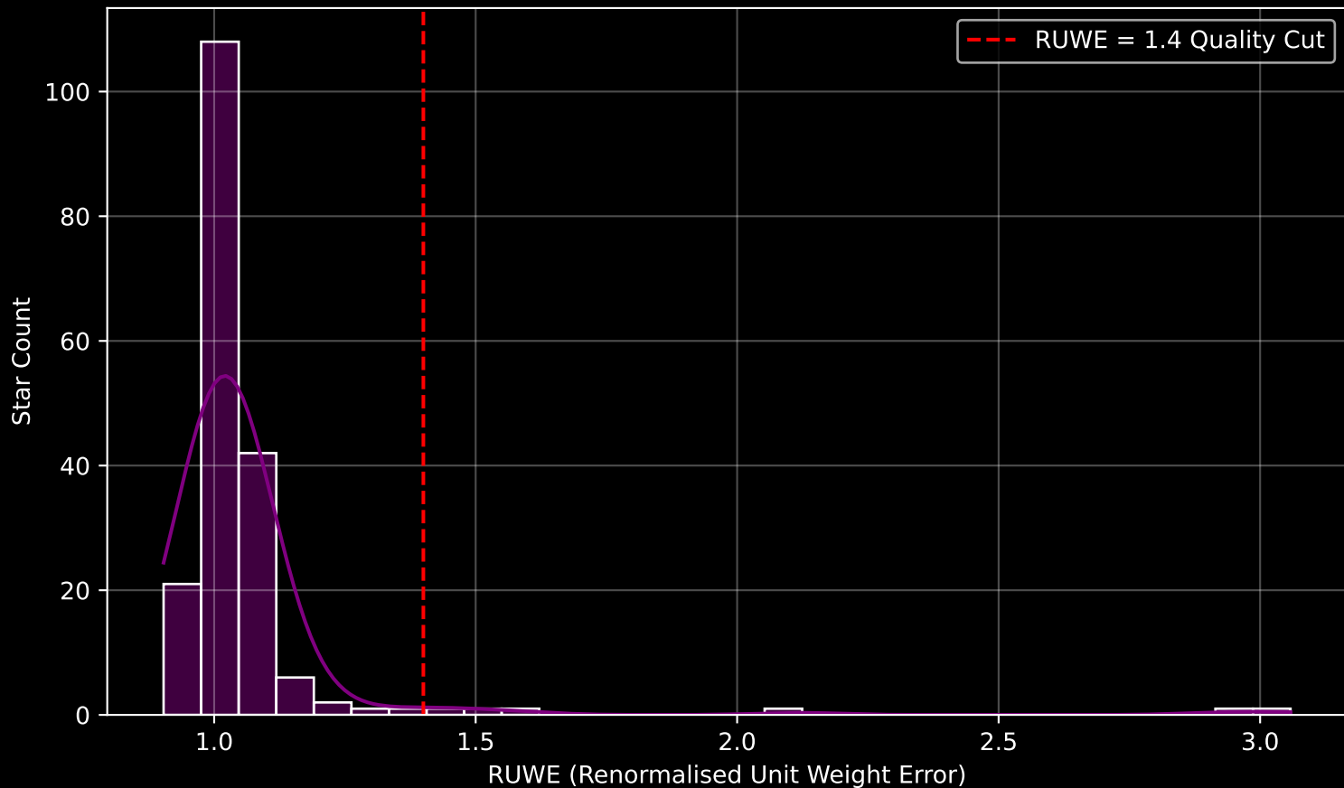
Gaia Cluster: [NGC_7031] RUWE Distribution (n= 187)
