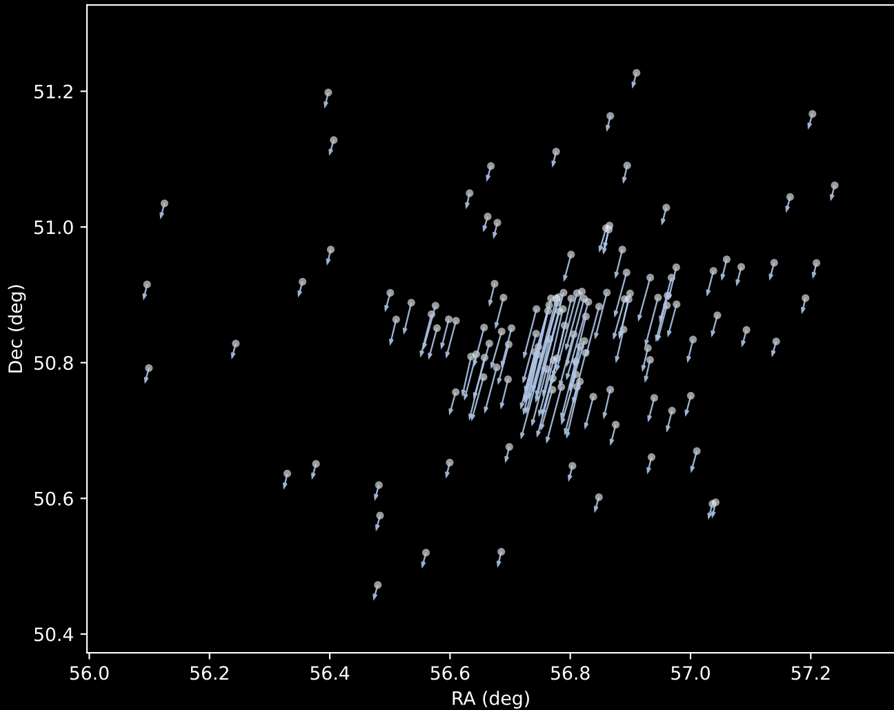
Gaia DR3 Cluster 1 Proper Motion Vectors (n=130)
