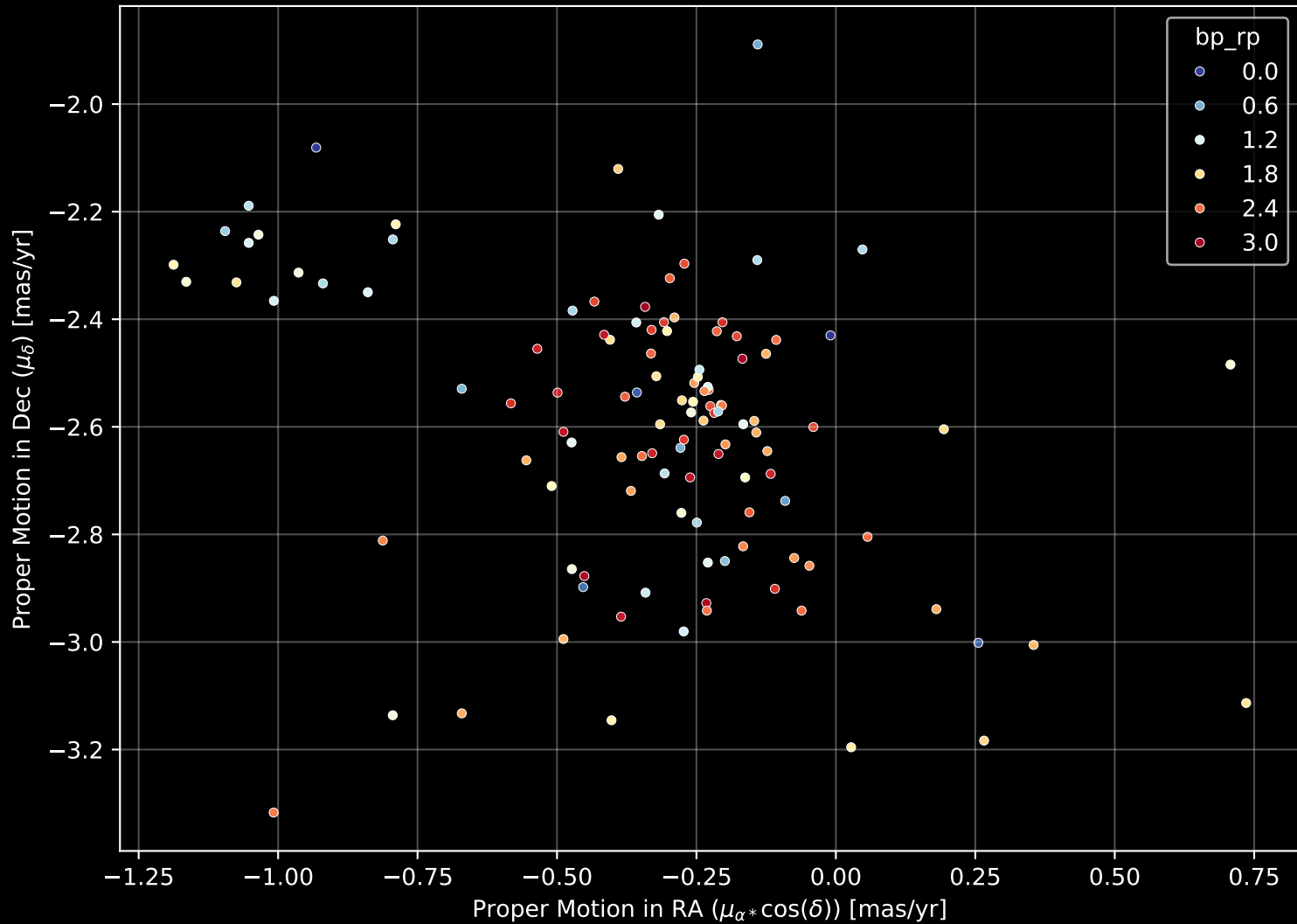
Gaia Cluster: [NGC_7039] Proper Motion Diagram (n= 117)
