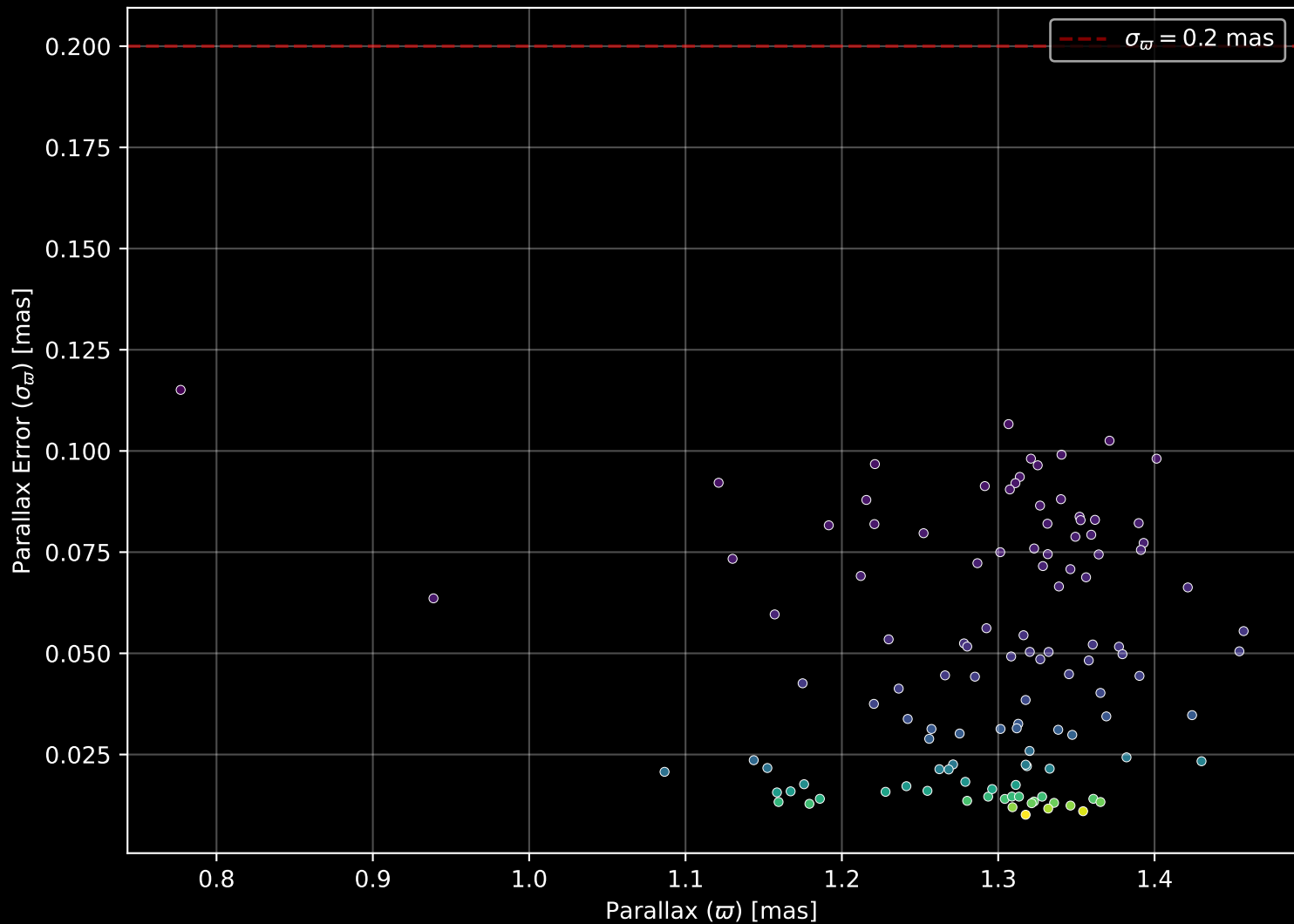
Gaia Cluster: [NGC_7039] Parallax Quality (n= 117)
