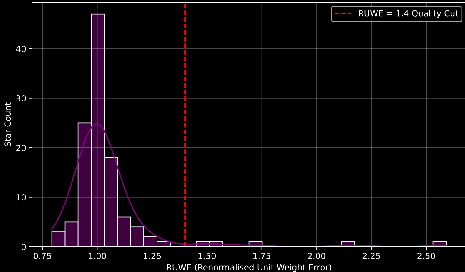
Gaia Cluster: [NGC_7039] RUWE Distribution (n= 116)
