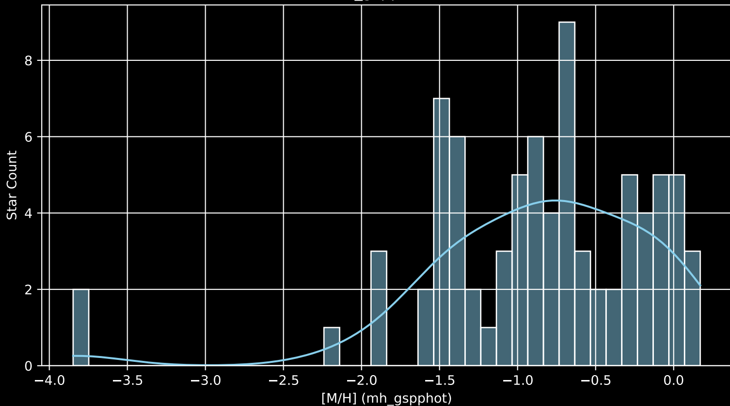
Gaia Cluster: [NGC_7067 [M/H] (mh_gspphot) (n= 80)
