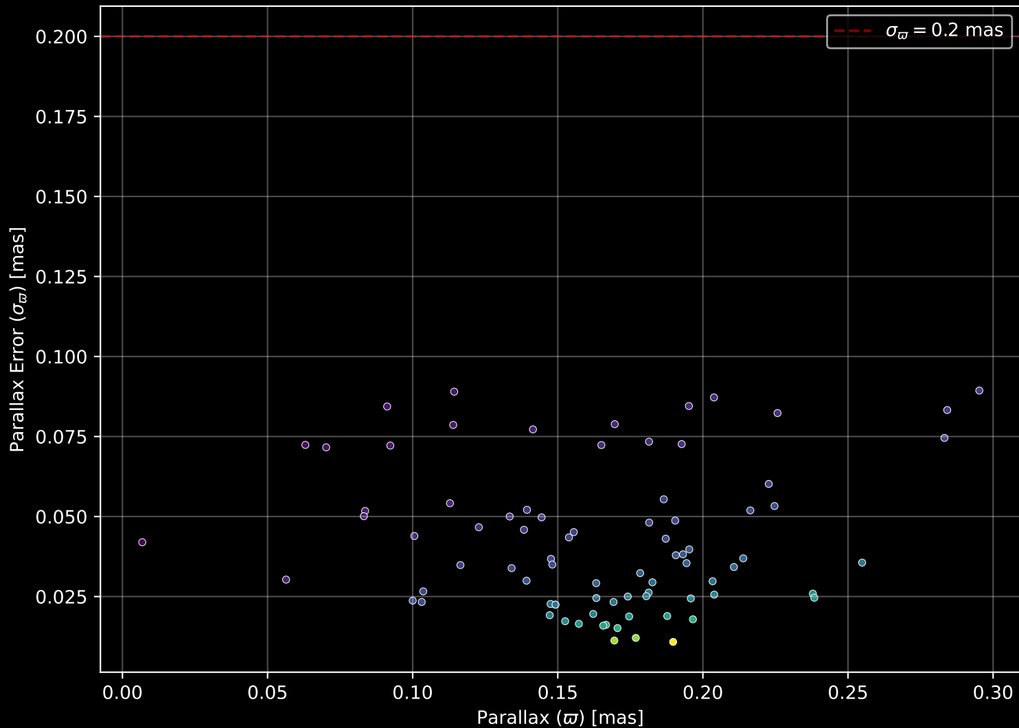
Gaia Cluster: [NGC_7067] Parallax Quality (n= 81)
