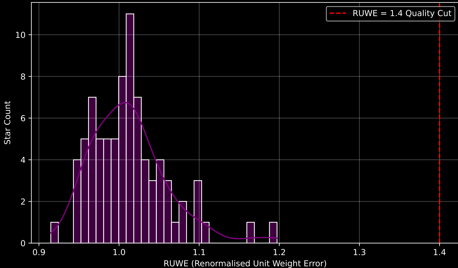
Gaia Cluster: [NGC_7067] RUWE Distribution (n= 81)
