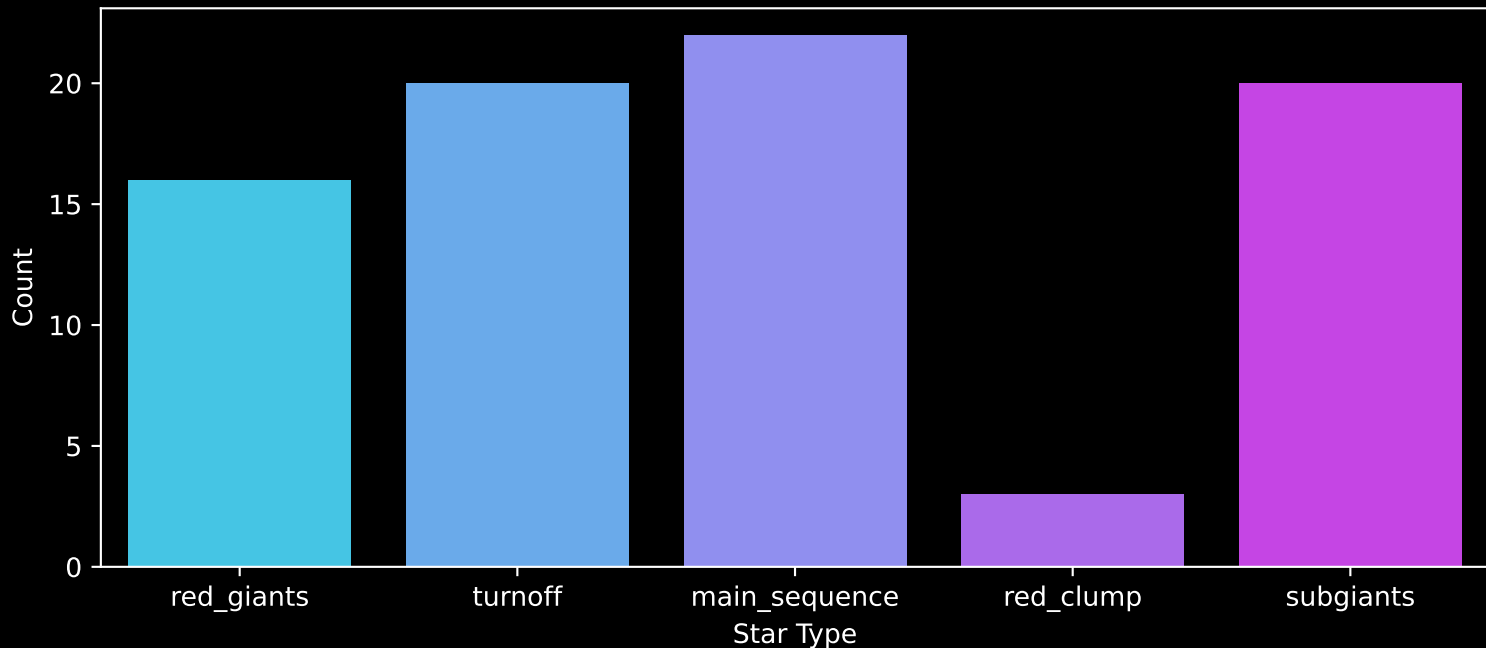
Gaia Cluster: [NGC_7067] Count plot of Star Type
