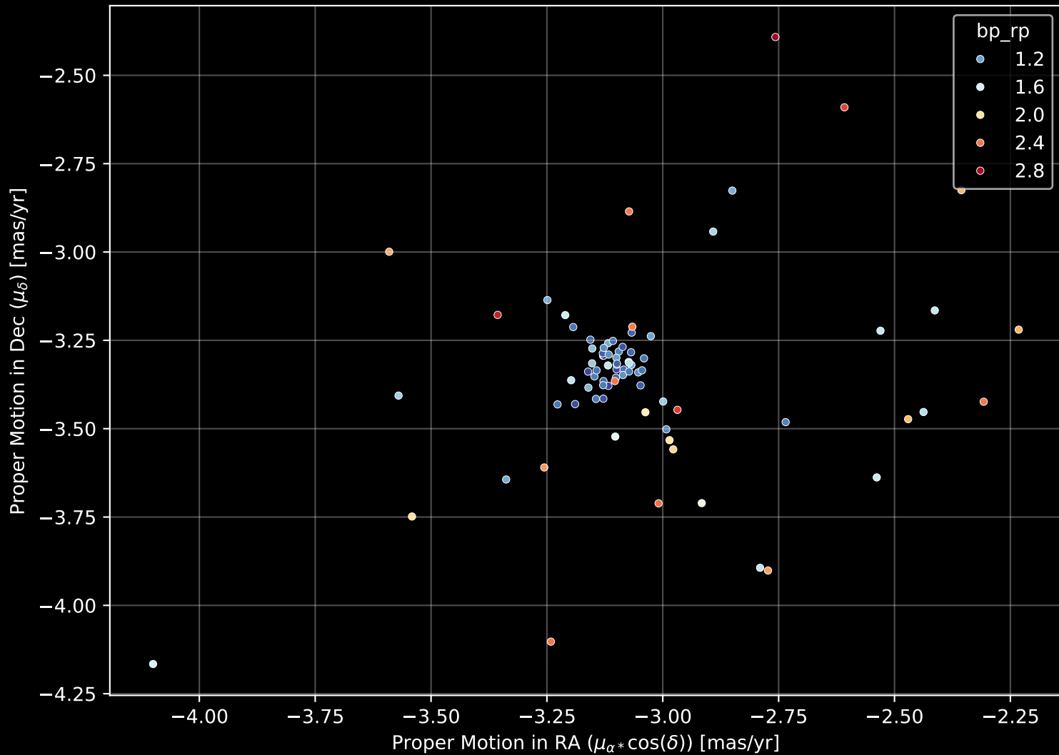
Gaia Cluster: [NGC_7067] Proper Motion Diagram (n= 81)
