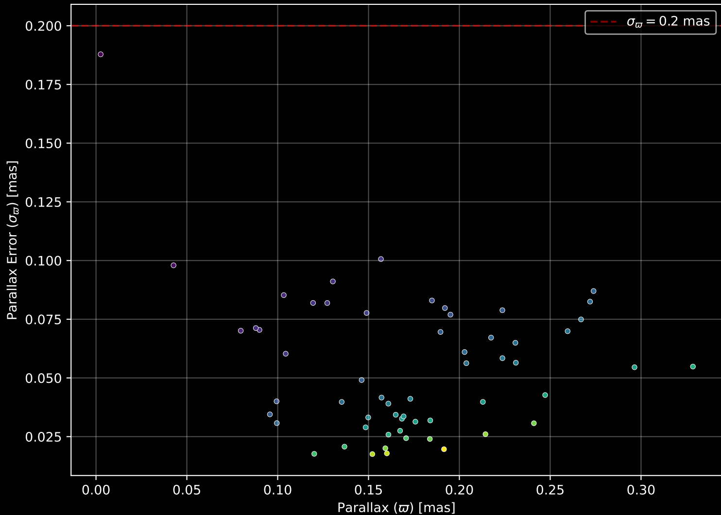
Gaia Cluster: [NGC_7226] Parallax Quality (n= 58)
