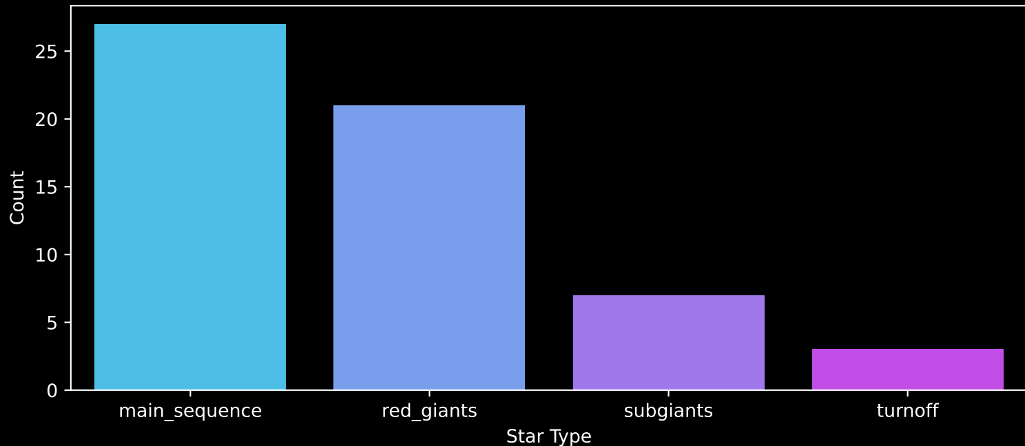
Gaia Cluster: [NGC_7226] Count plot of Star Type
