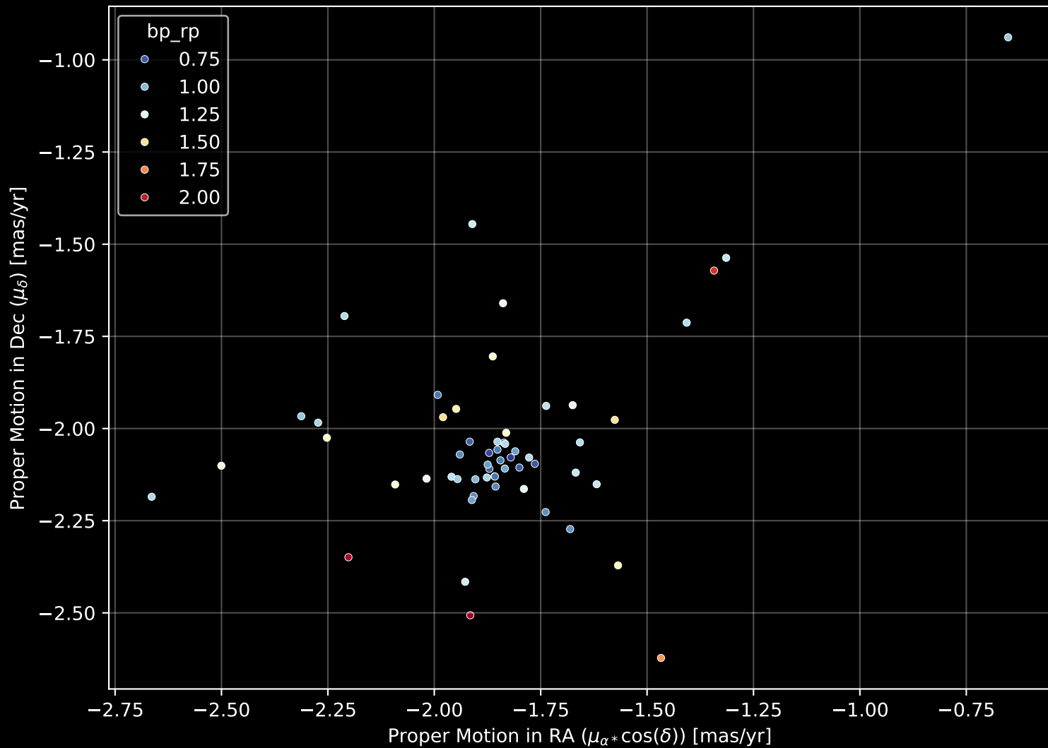
Gaia Cluster: [NGC_7226] Proper Motion Diagram (n= 58)
