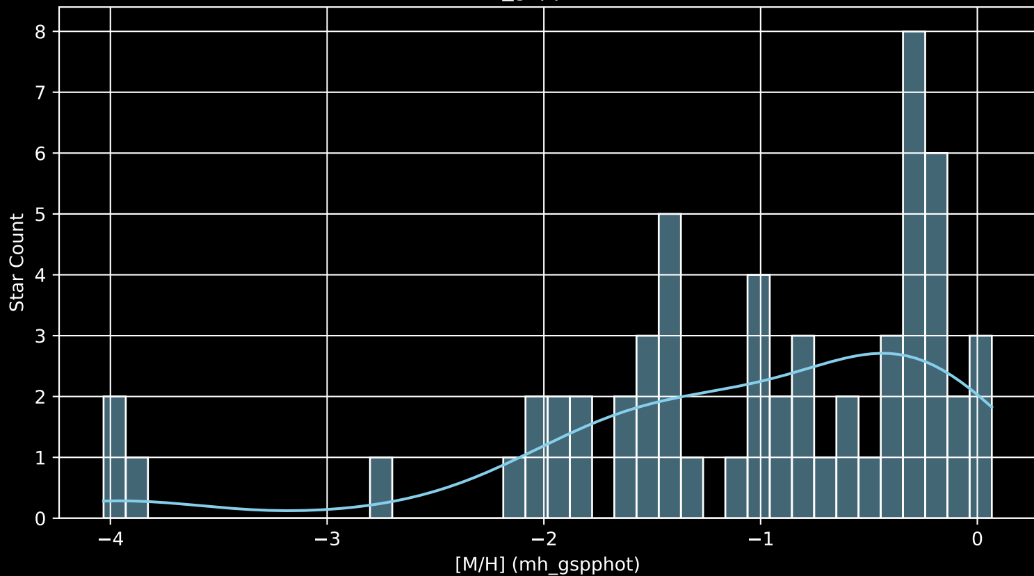
Gaia Cluster: [NGC_7226 [M/H] (mh_gspphot) (n= 58)
