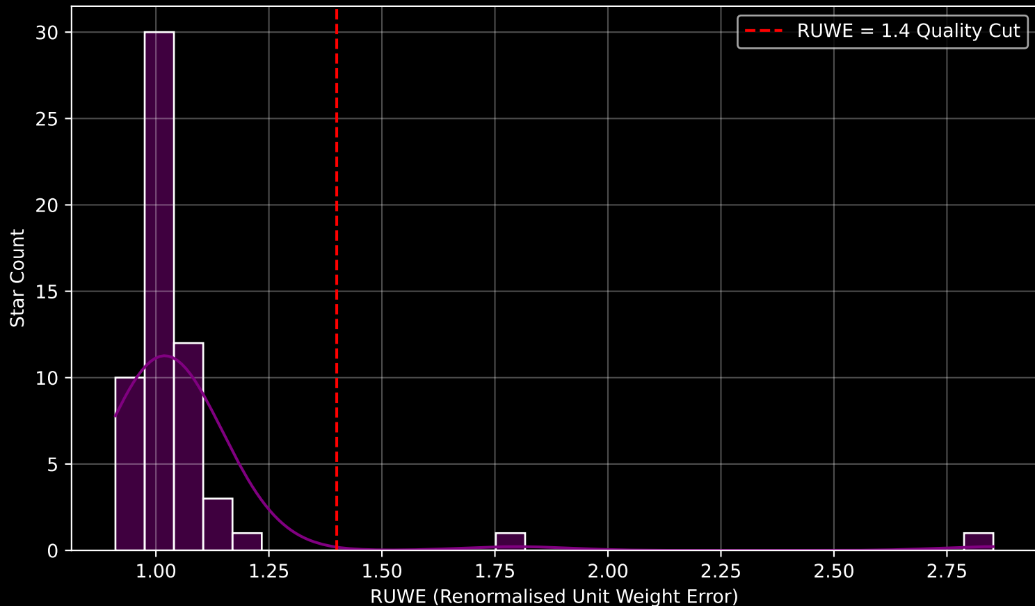
Gaia Cluster: [NGC_7226] RUWE Distribution (n= 58)
