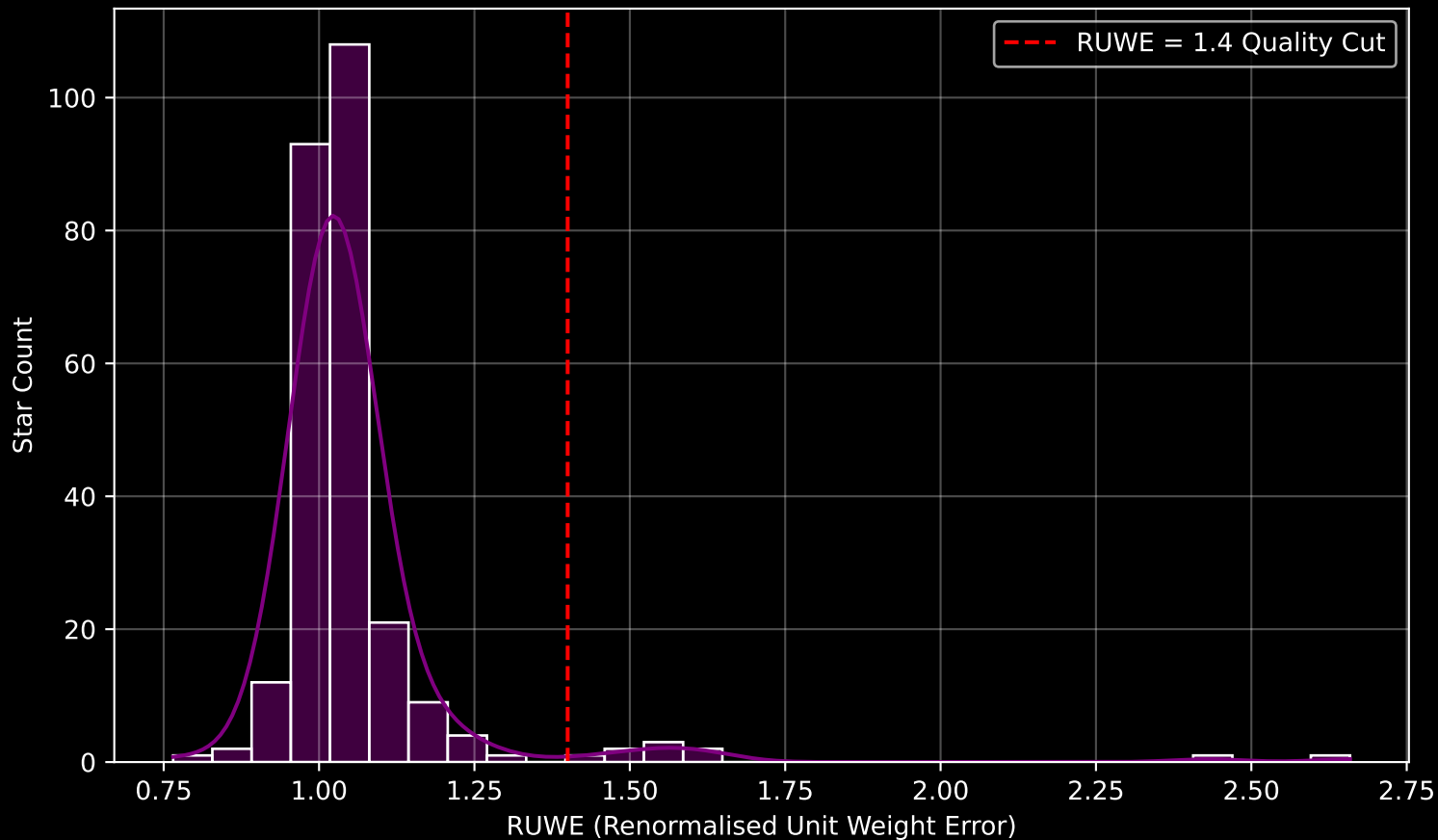
Gaia Cluster: [NGC_7235] RUWE Distribution (n= 261)
