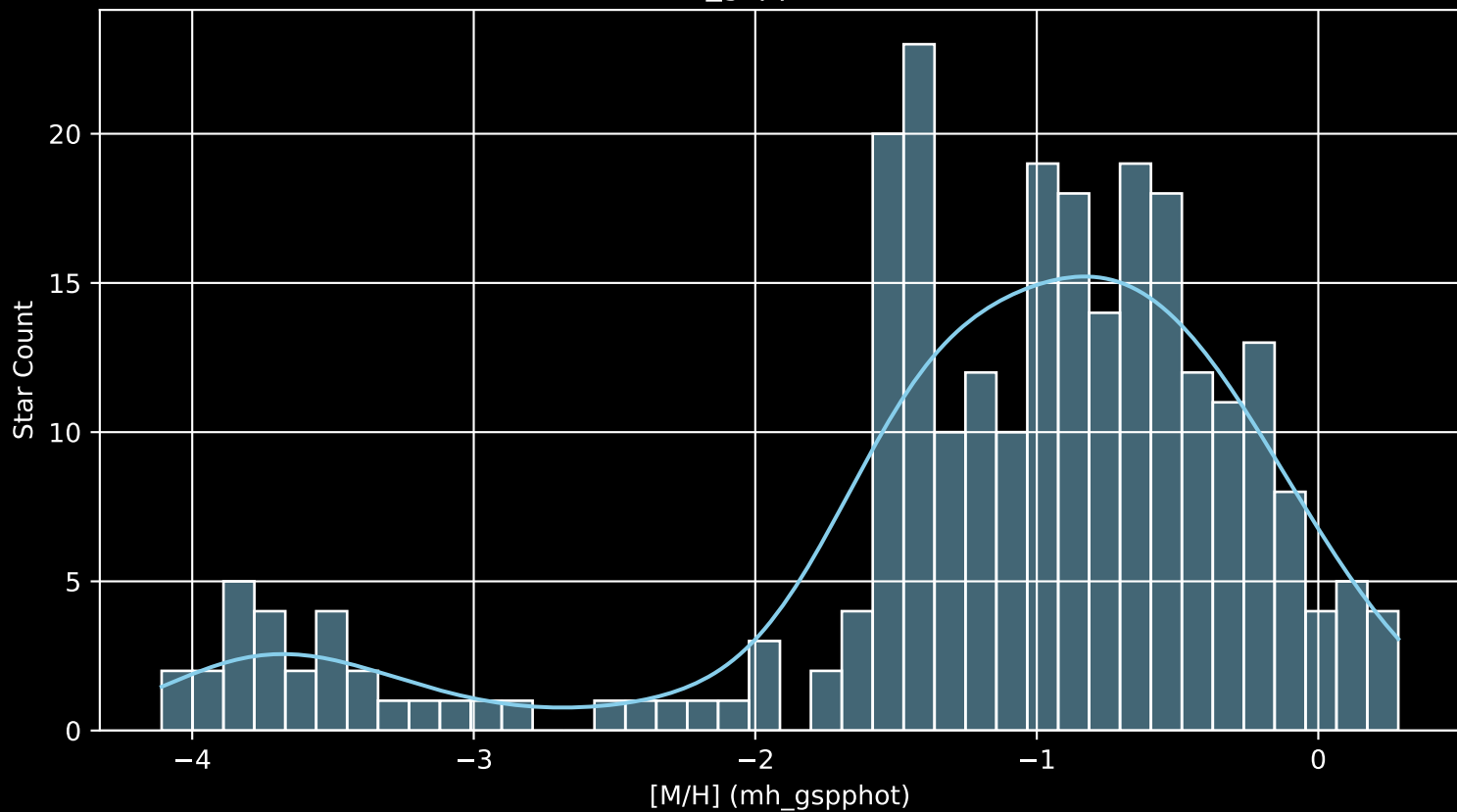
Gaia Cluster: [NGC_7235 [M/H] (mh_gspphot) (n= 260)
