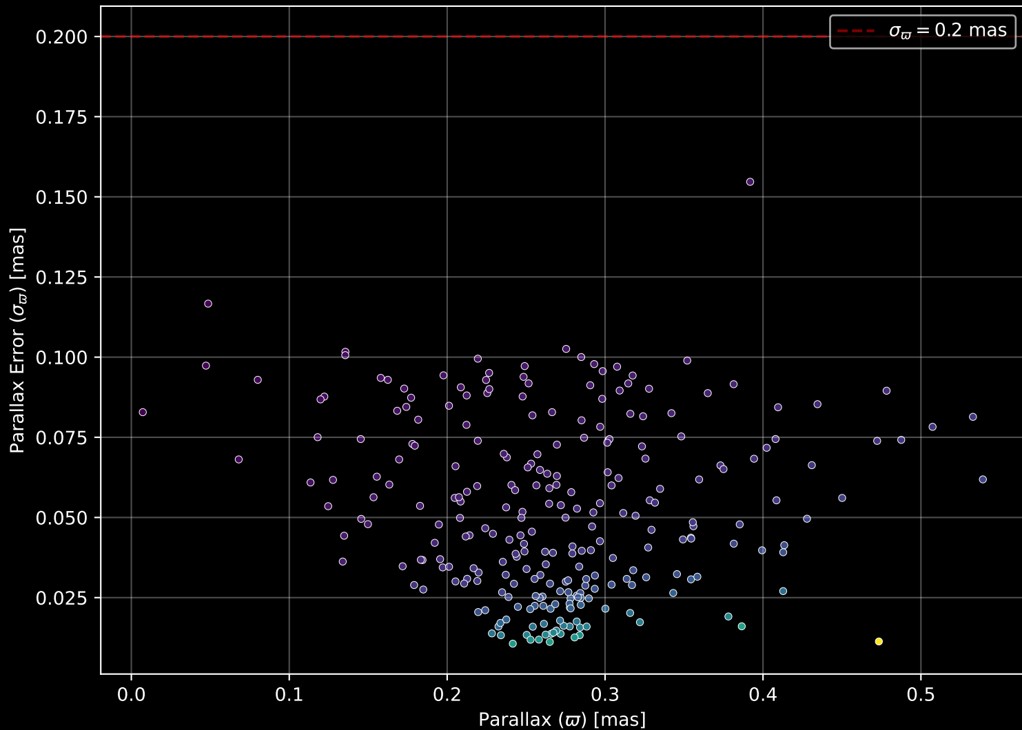
Gaia Cluster: [NGC_7235] Parallax Quality (n= 262)
