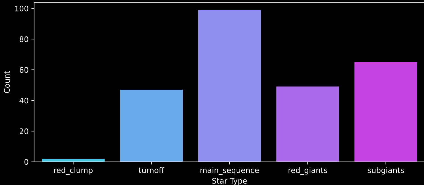
Gaia Cluster: [NGC_7235] Count plot of Star Type
