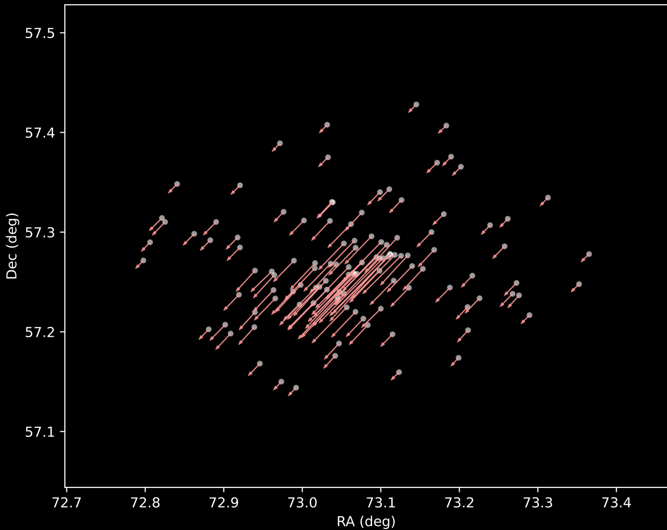
Gaia DR3 Cluster 7 Proper Motion Vectors (n=115)
