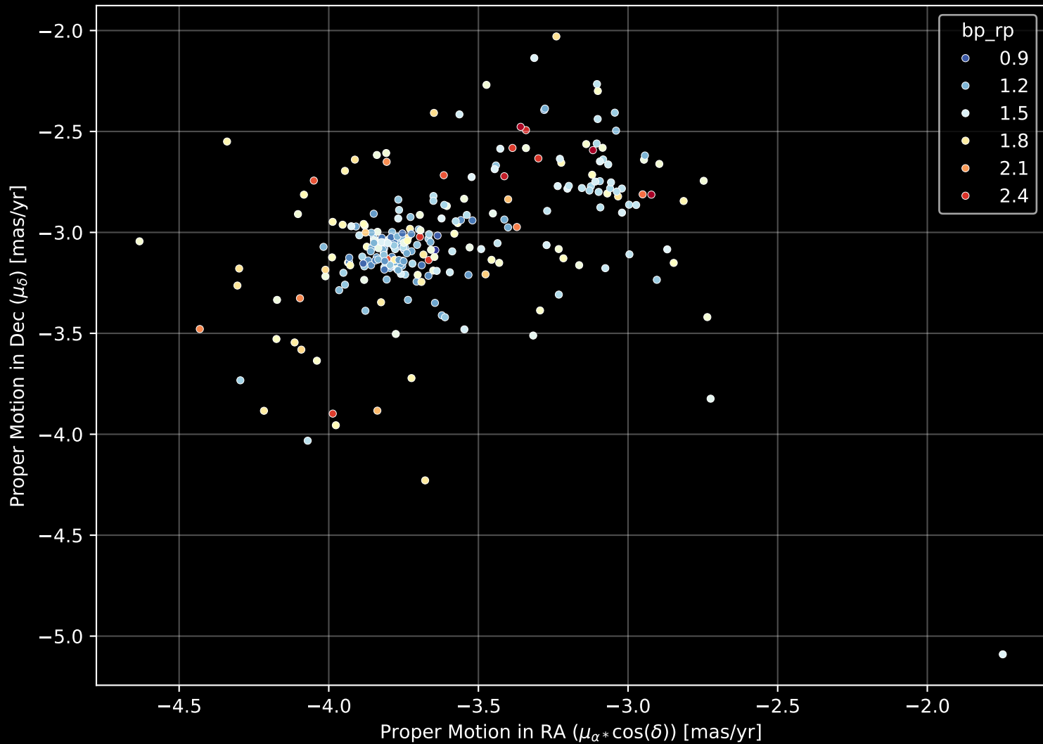
Gaia Cluster: [NGC_7235] Proper Motion Diagram (n= 262)
