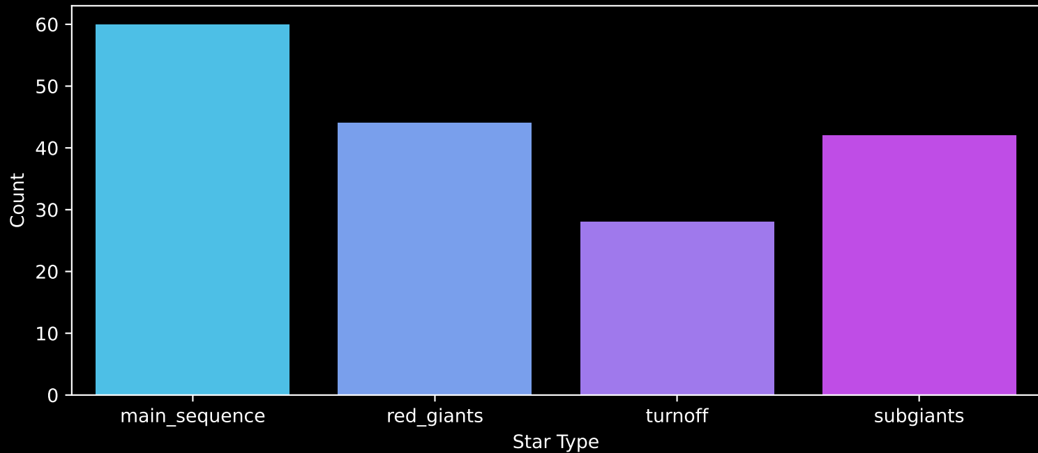
Gaia Cluster: [NGC_7261] Count plot of Star Type
