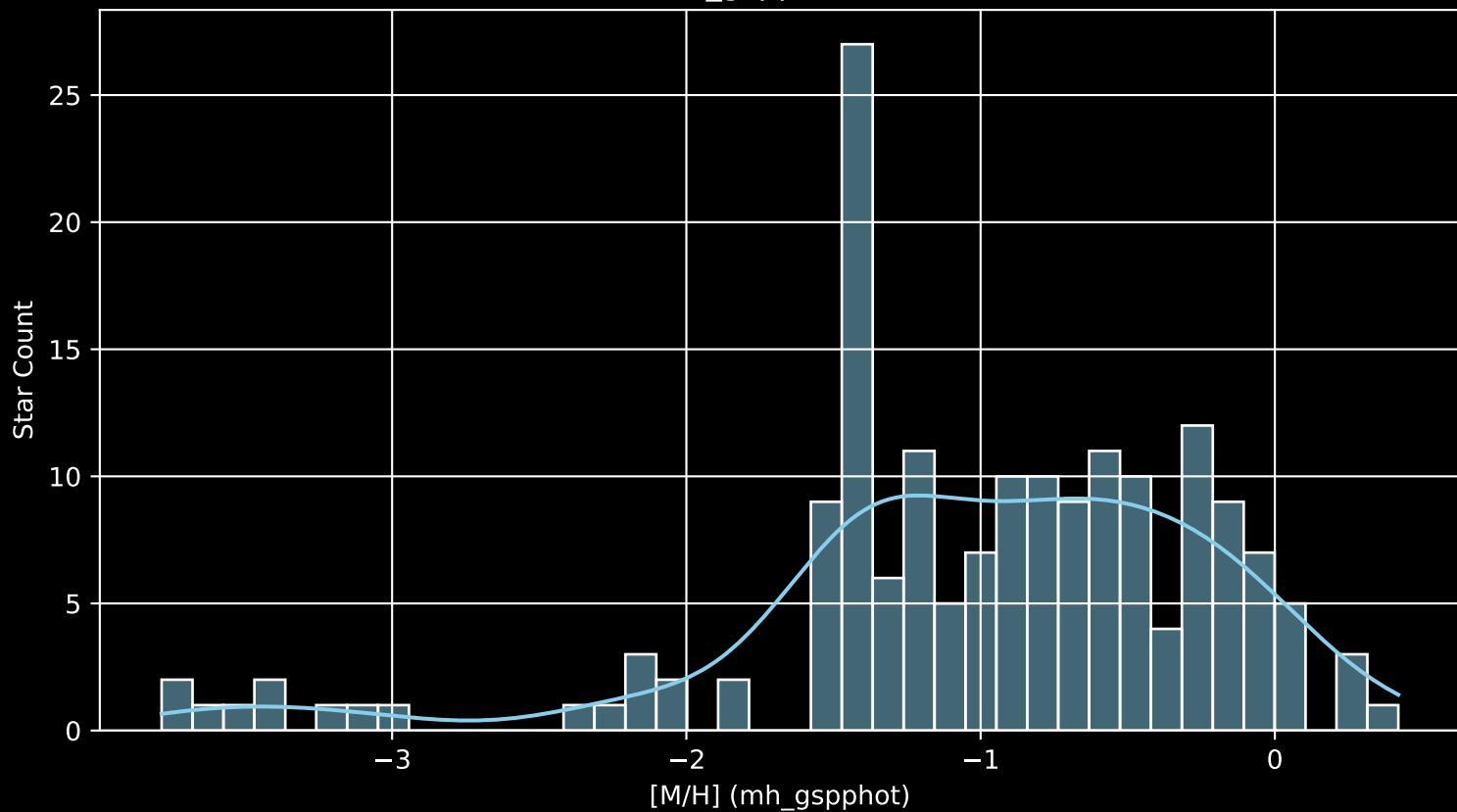
Gaia Cluster: [NGC_7261 [M/H] (mh_gspphot) (n= 174)
