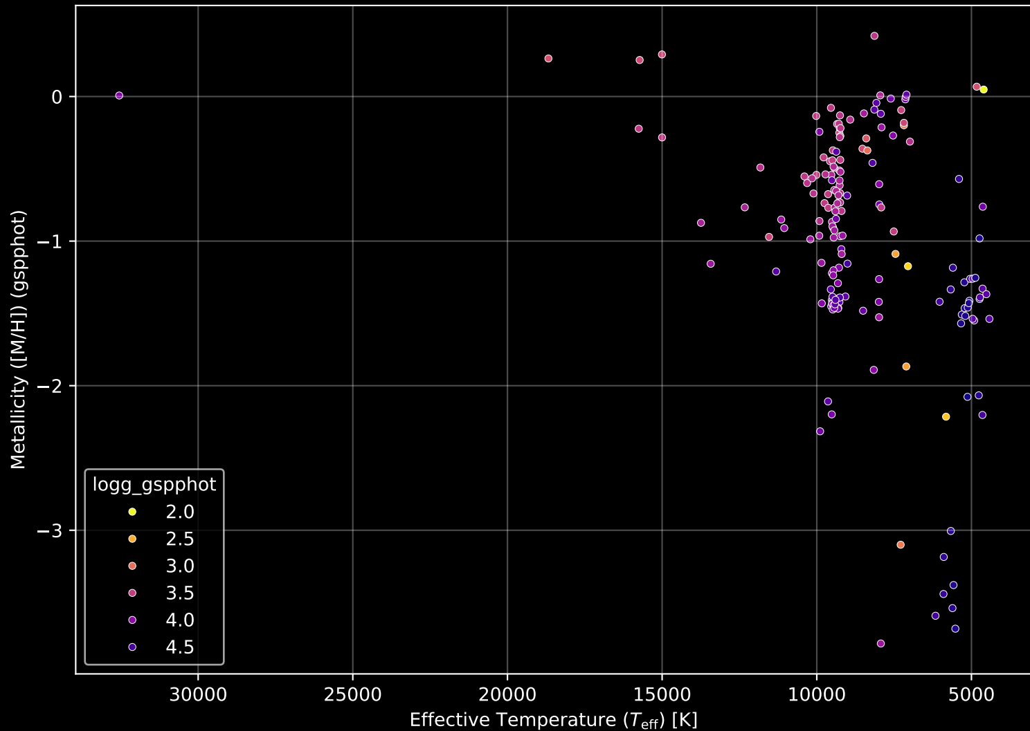
Gaia Cluster: [NGC_7261] Stellar Population Parameters (n= 174)
