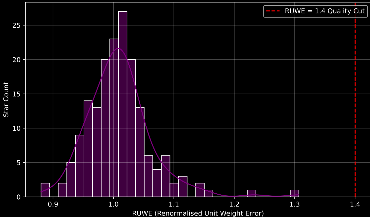
Gaia Cluster: [NGC_7261] RUWE Distribution (n= 174)
