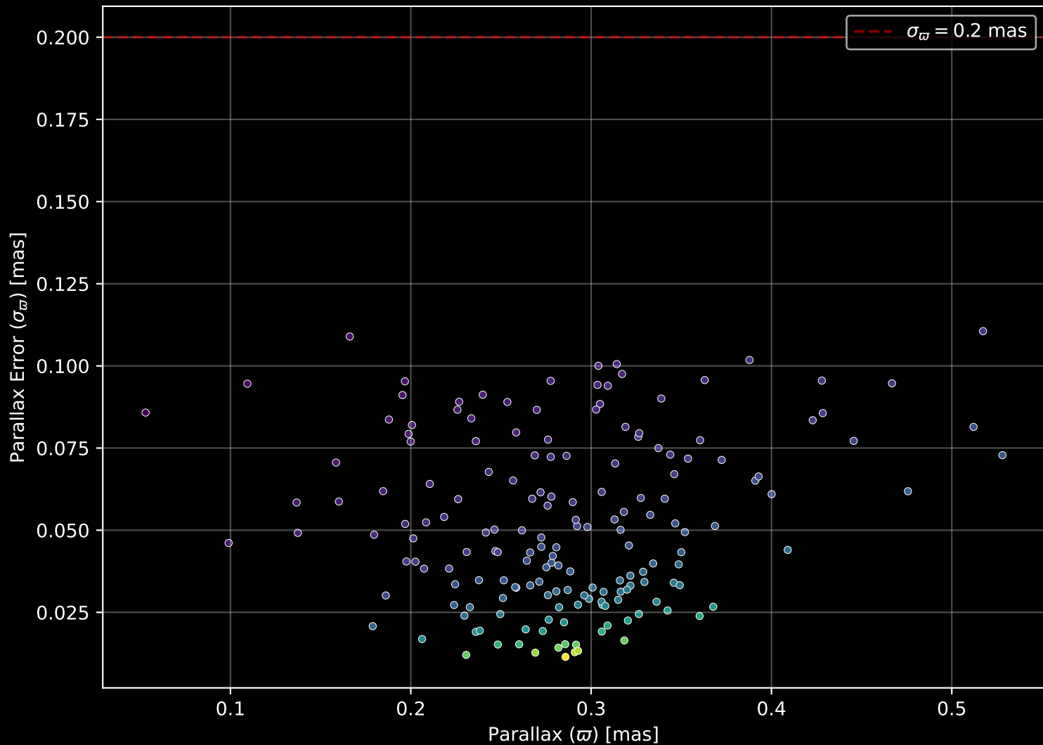
Gaia Cluster: [NGC_7261] Parallax Quality (n= 174)
