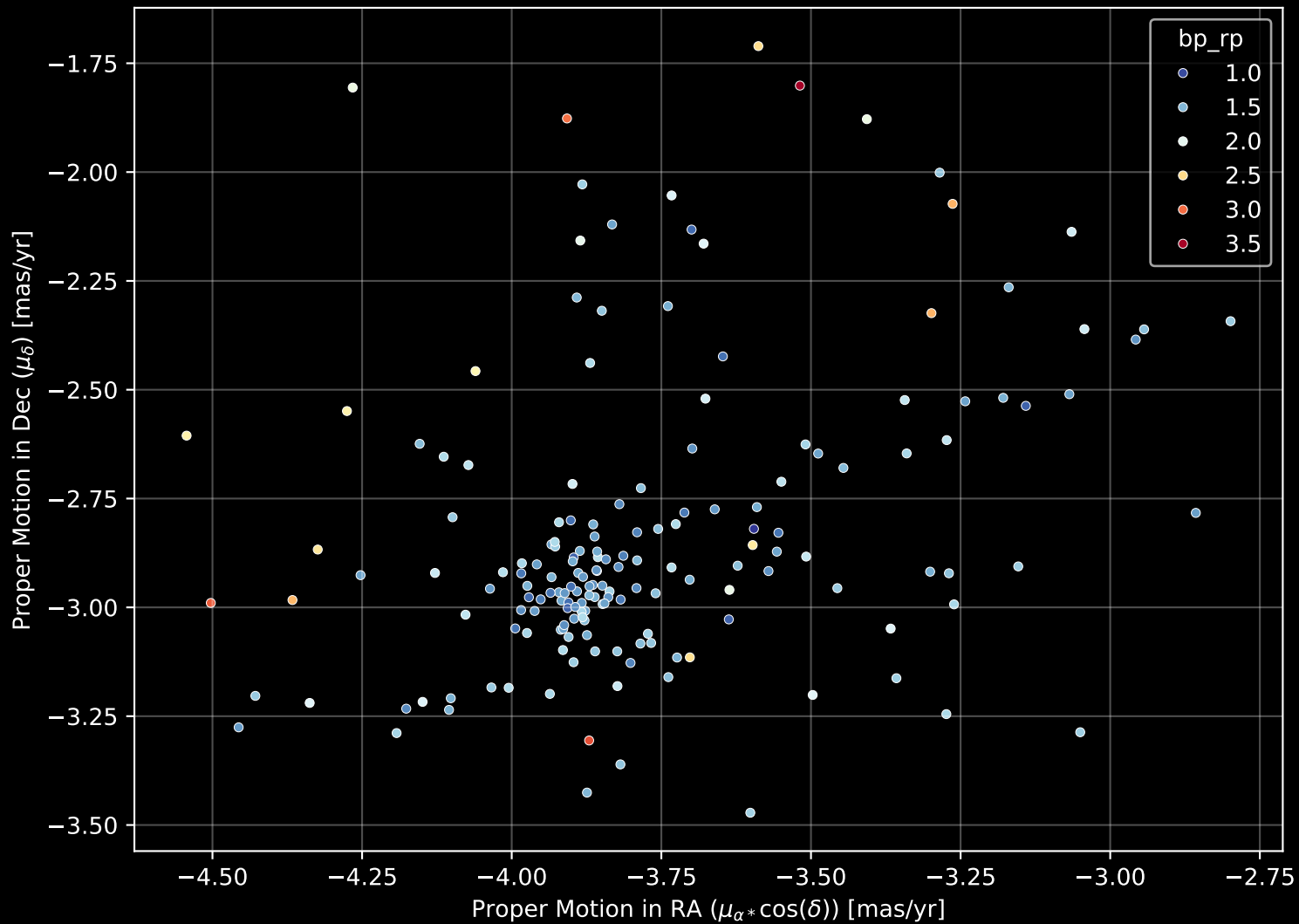
Gaia Cluster: [NGC_7261] Proper Motion Diagram (n= 174)
