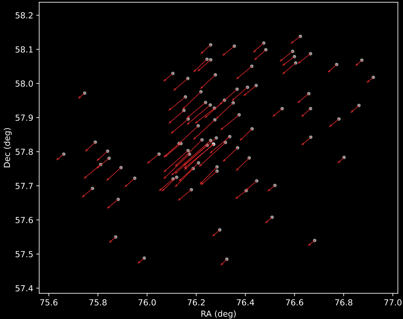
Gaia DR3 Cluster 6 Proper Motion Vectors (n=82)
