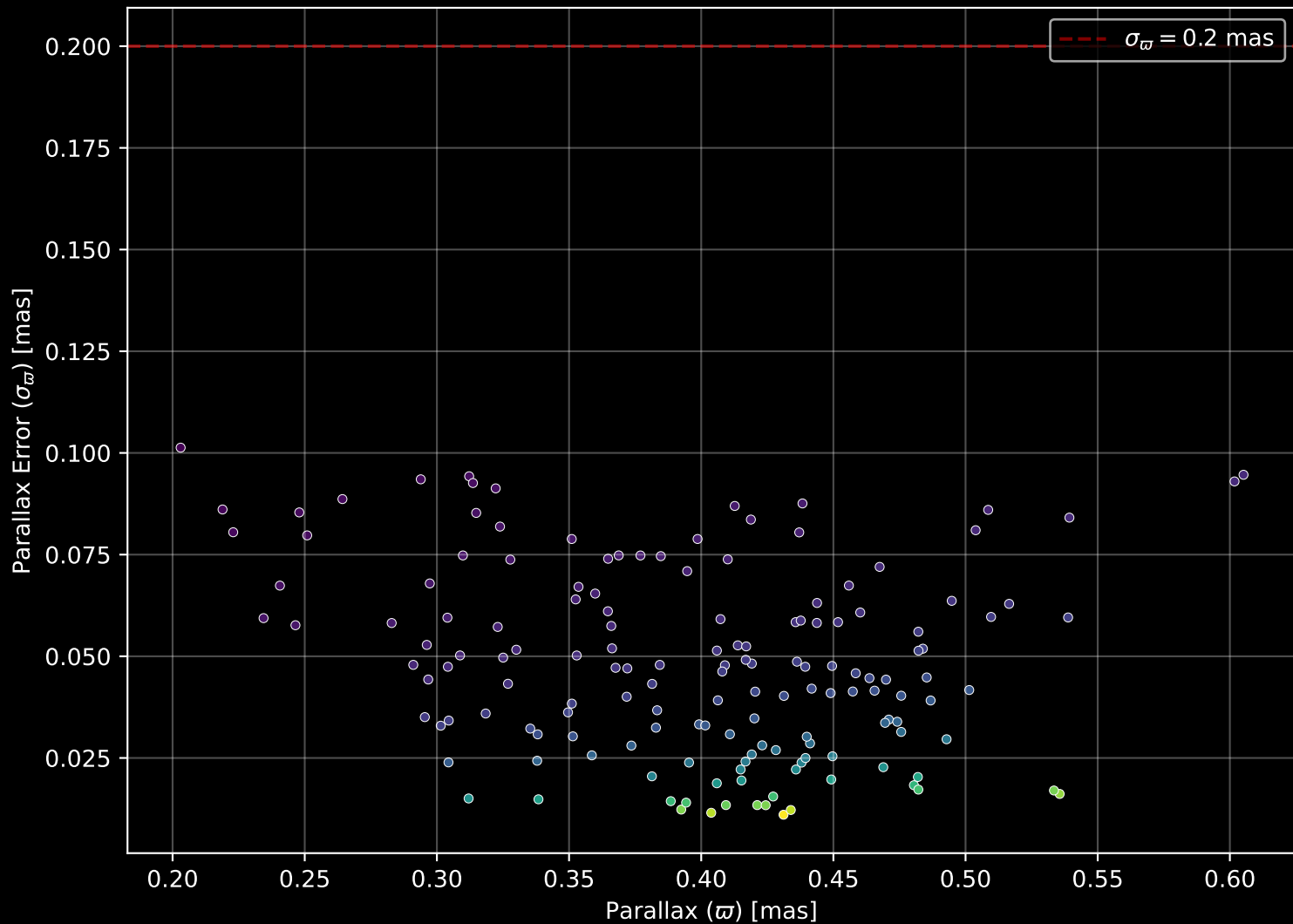
Gaia Cluster: [NGC_7281] Parallax Quality (n= 156)
