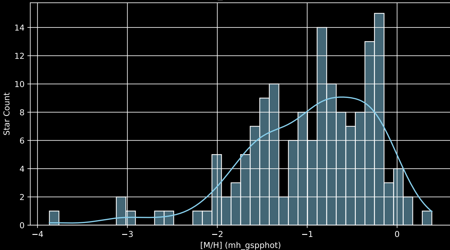
Gaia Cluster: [NGC_7281 [M/H] (mh_gspphot) (n= 156)
