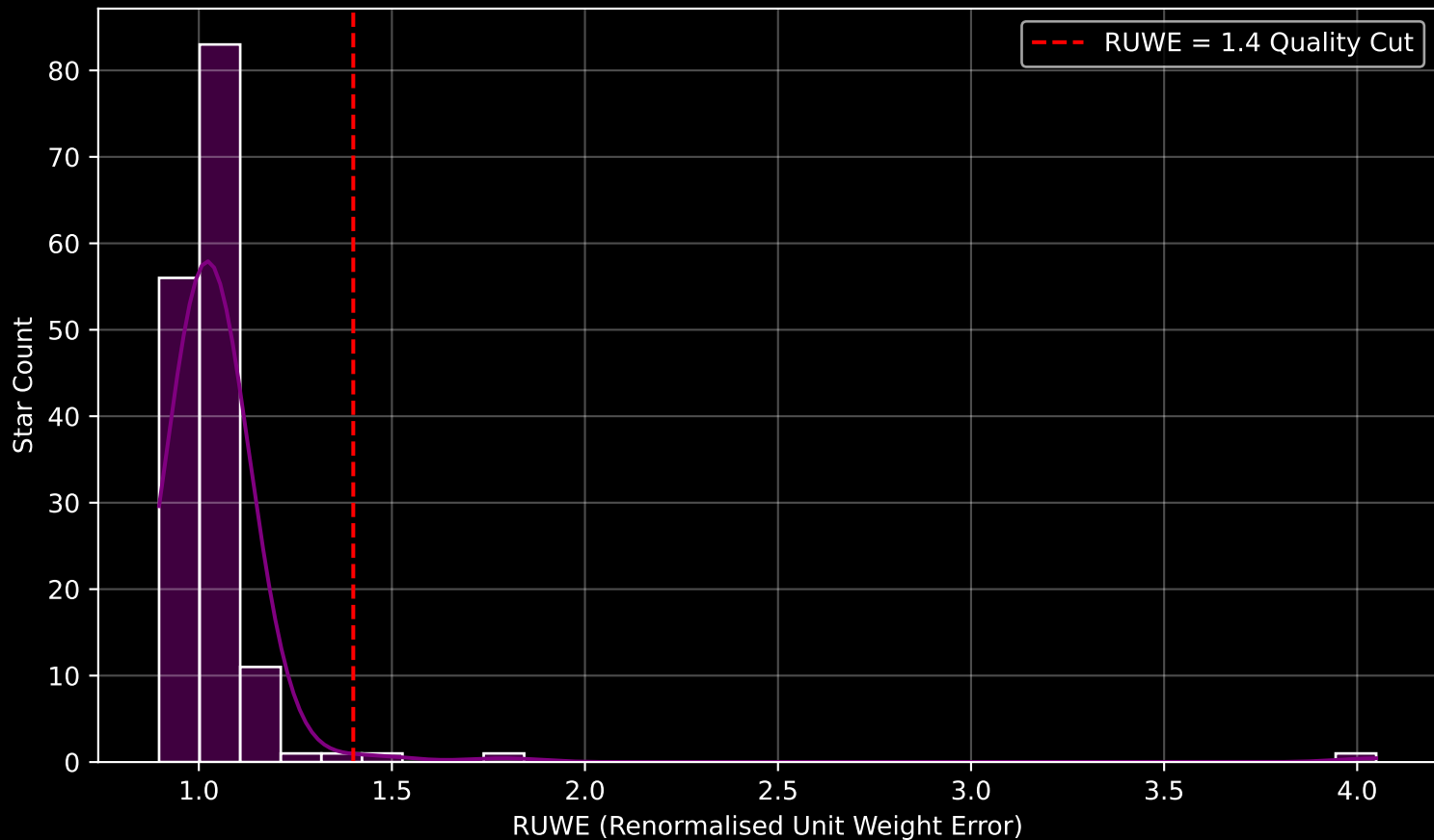
Gaia Cluster: [NGC_7281] RUWE Distribution (n= 155)
