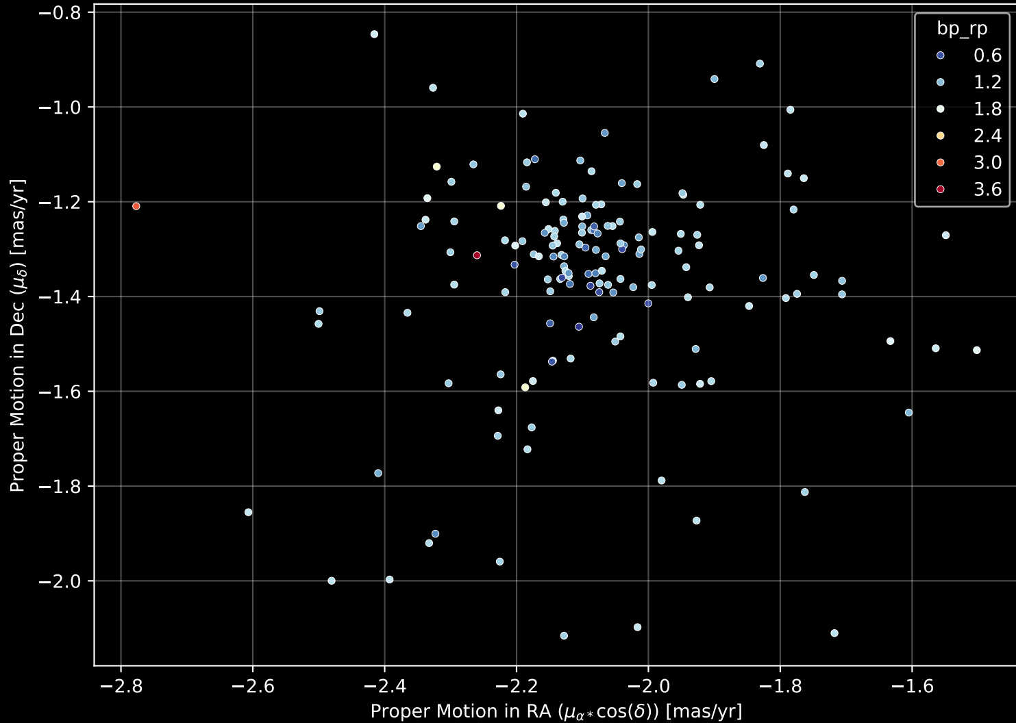
Gaia Cluster: [NGC_7281] Proper Motion Diagram (n= 156)
