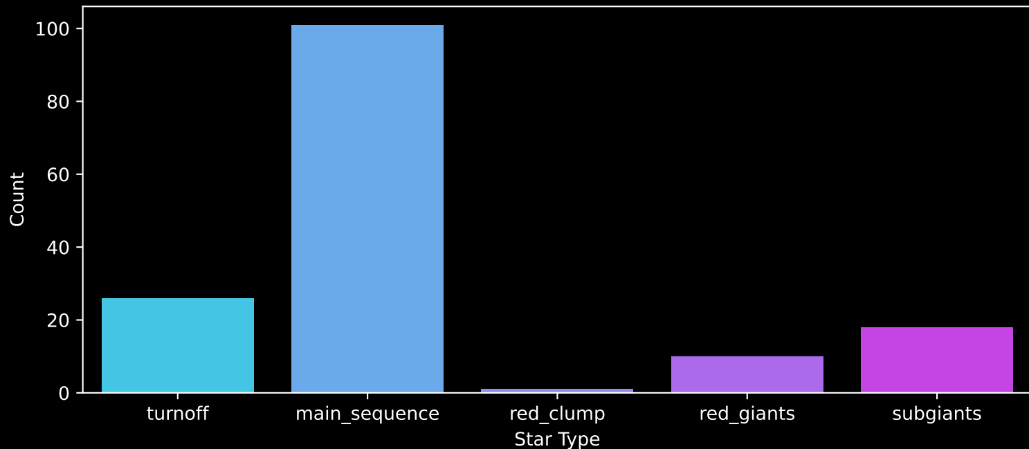
Gaia Cluster: [NGC_7281] Count plot of Star Type
