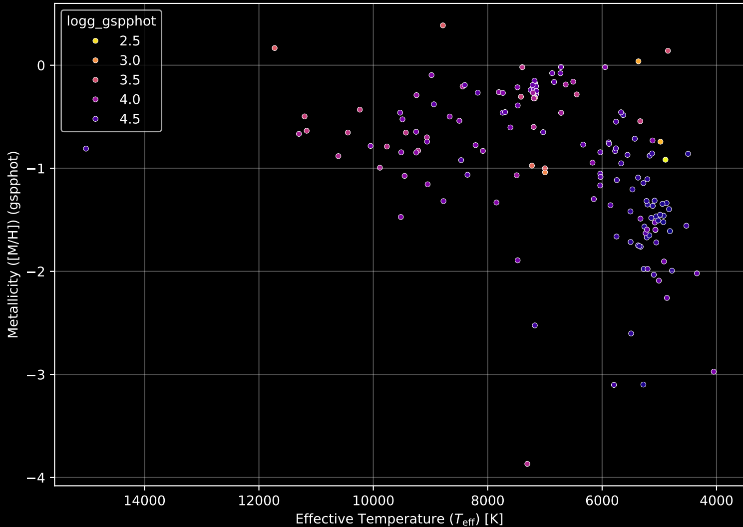
Gaia Cluster: [NGC_7281] Stellar Population Parameters (n= 156)
