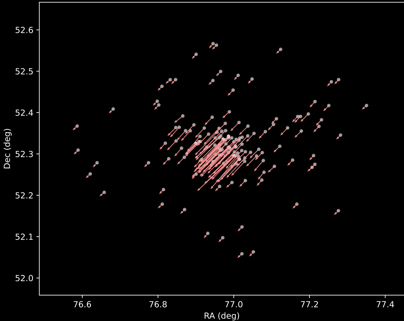
Gaia DR3 Cluster 7 Proper Motion Vectors (n=142)
