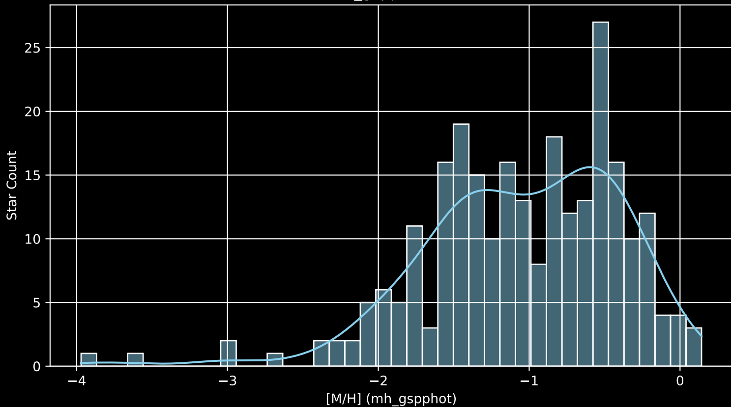
Gaia Cluster: [NGC_7296 [M/H] (mh_gspphot) (n= 257)
