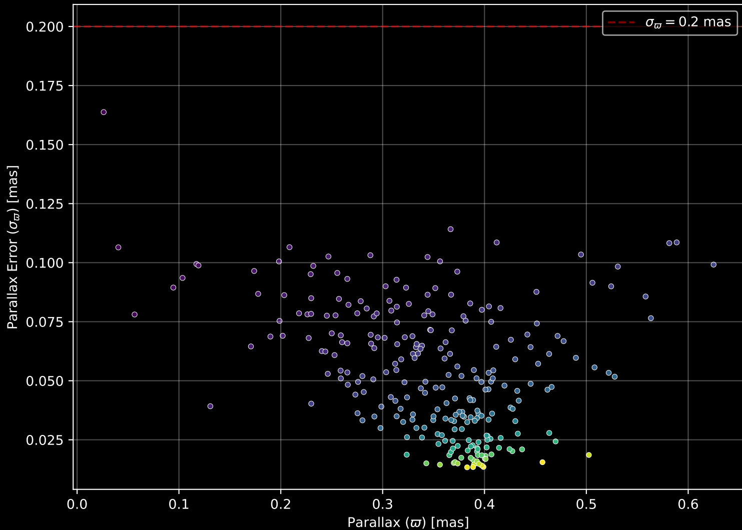
Gaia Cluster: [NGC_7296] Parallax Quality (n= 257)
