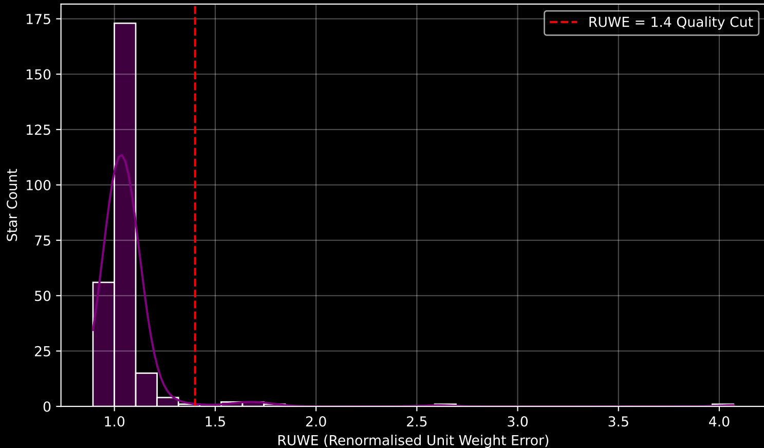
Gaia Cluster: [NGC_7296] RUWE Distribution (n= 256)
