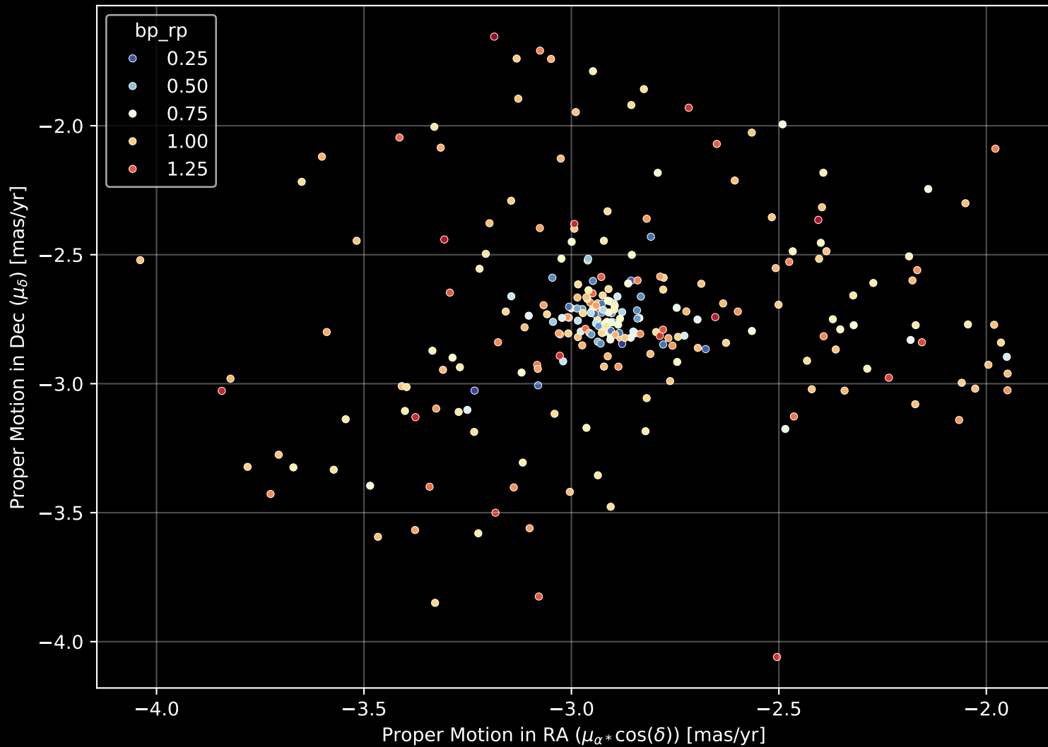
Gaia Cluster: [NGC_7296] Proper Motion Diagram (n= 257)
