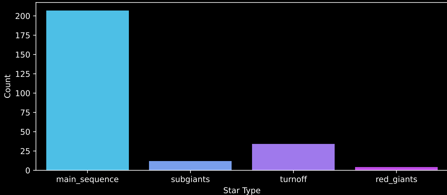
Gaia Cluster: [NGC_7296] Count plot of Star Type
