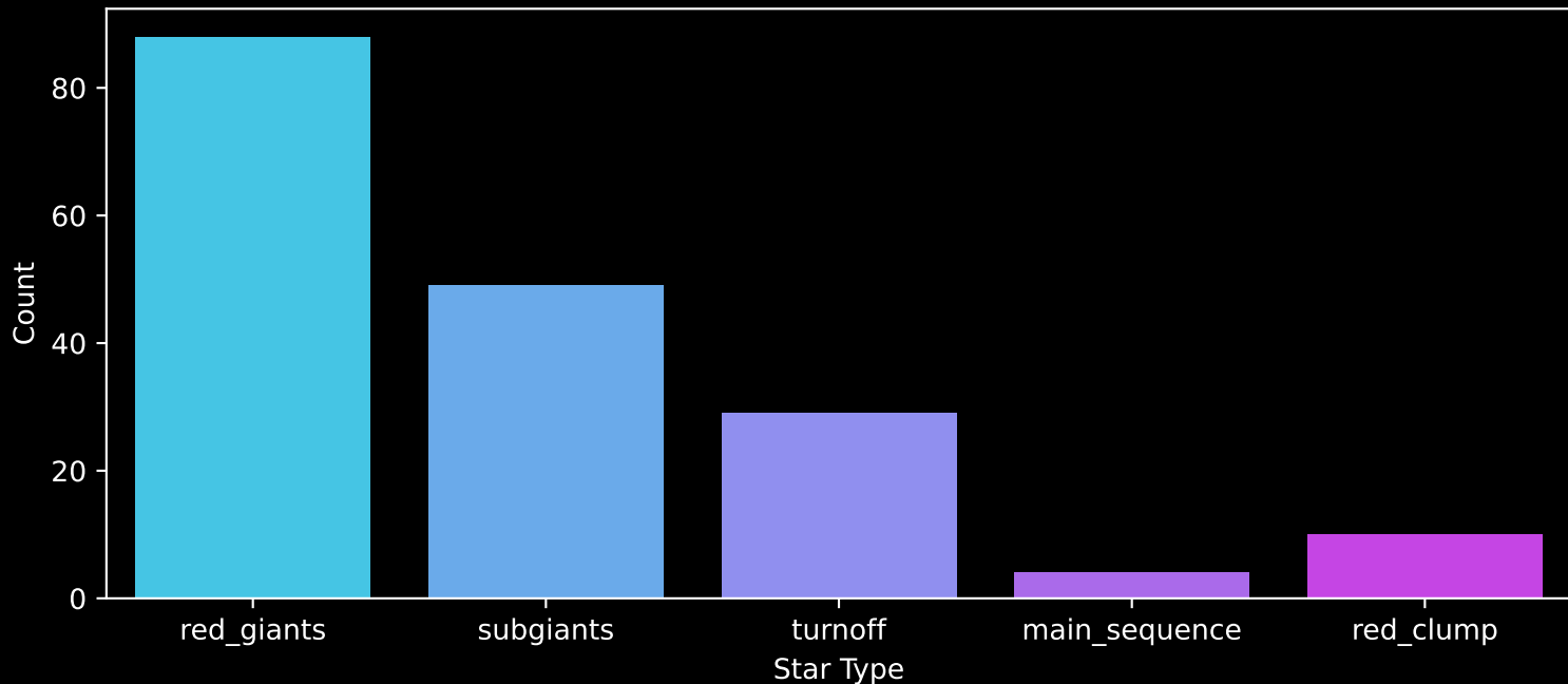
Gaia Cluster: [NGC_7419] Count plot of Star Type
