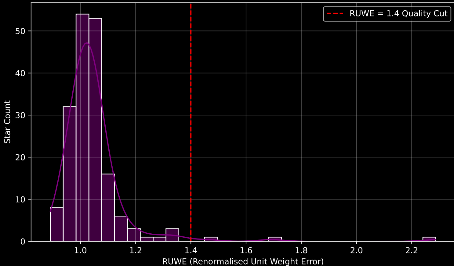
Gaia Cluster: [NGC_7419] RUWE Distribution (n= 180)
