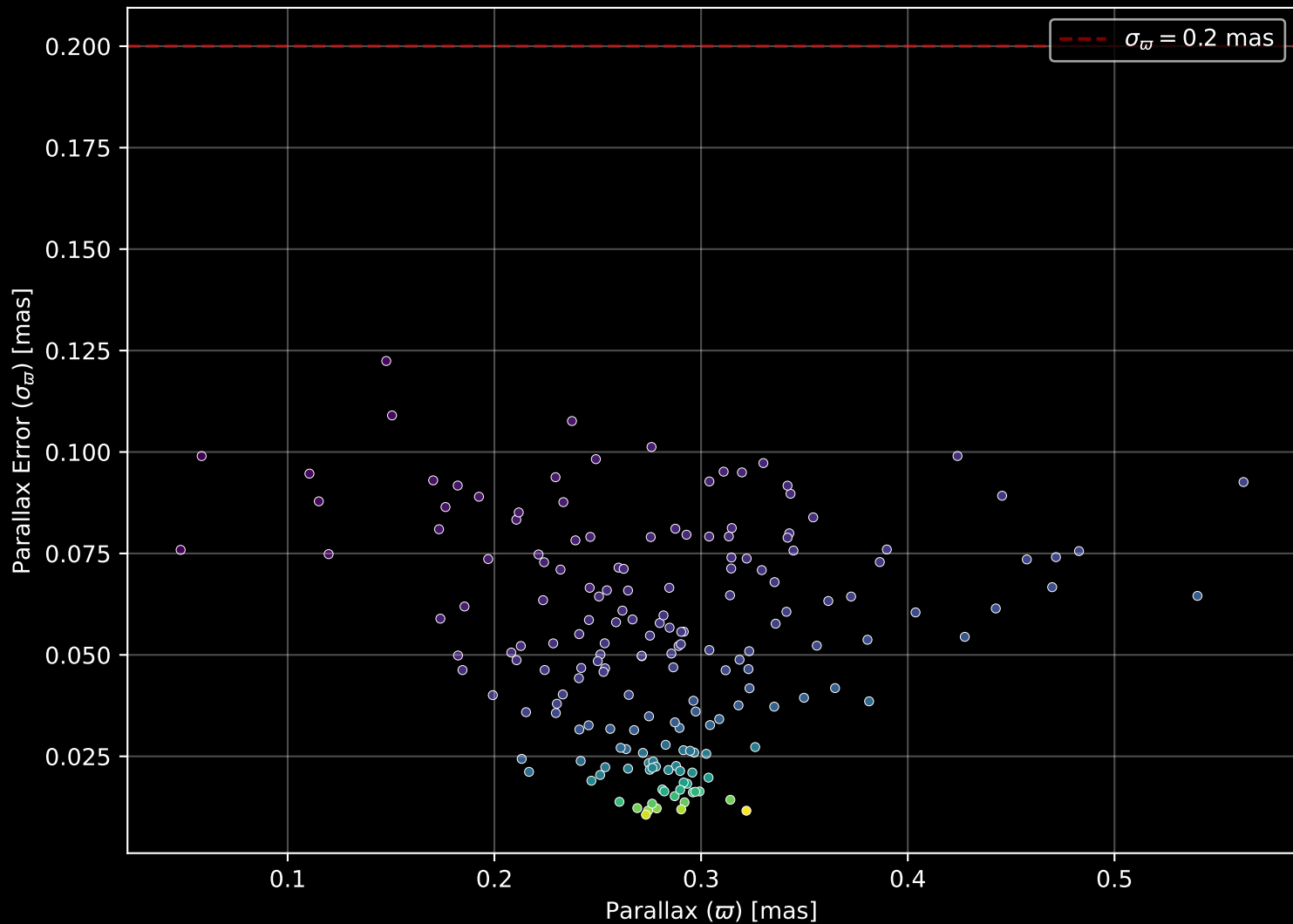
Gaia Cluster: [NGC_7419] Parallax Quality (n= 180)
