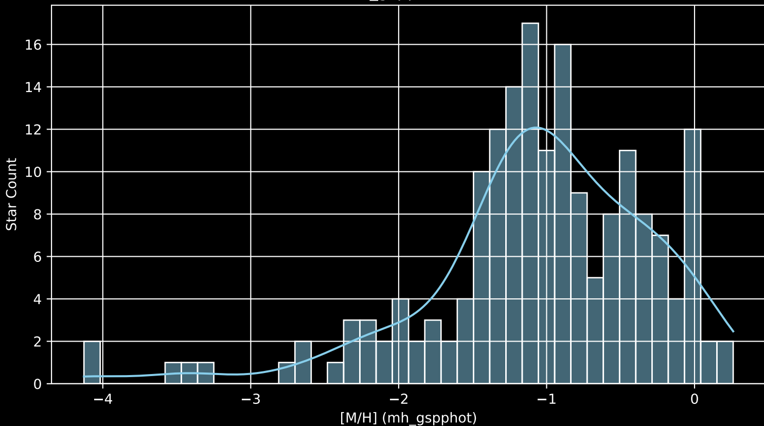
Gaia Cluster: [NGC_7419 [M/H] (mh_gspphot) (n= 180)
