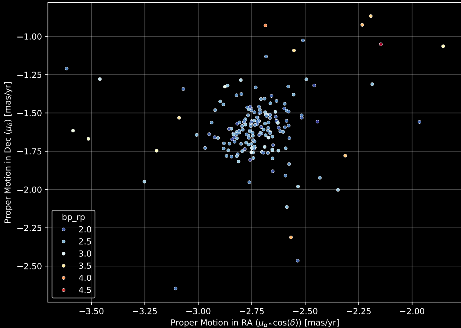
Gaia Cluster: [NGC_7419] Proper Motion Diagram (n= 180)
