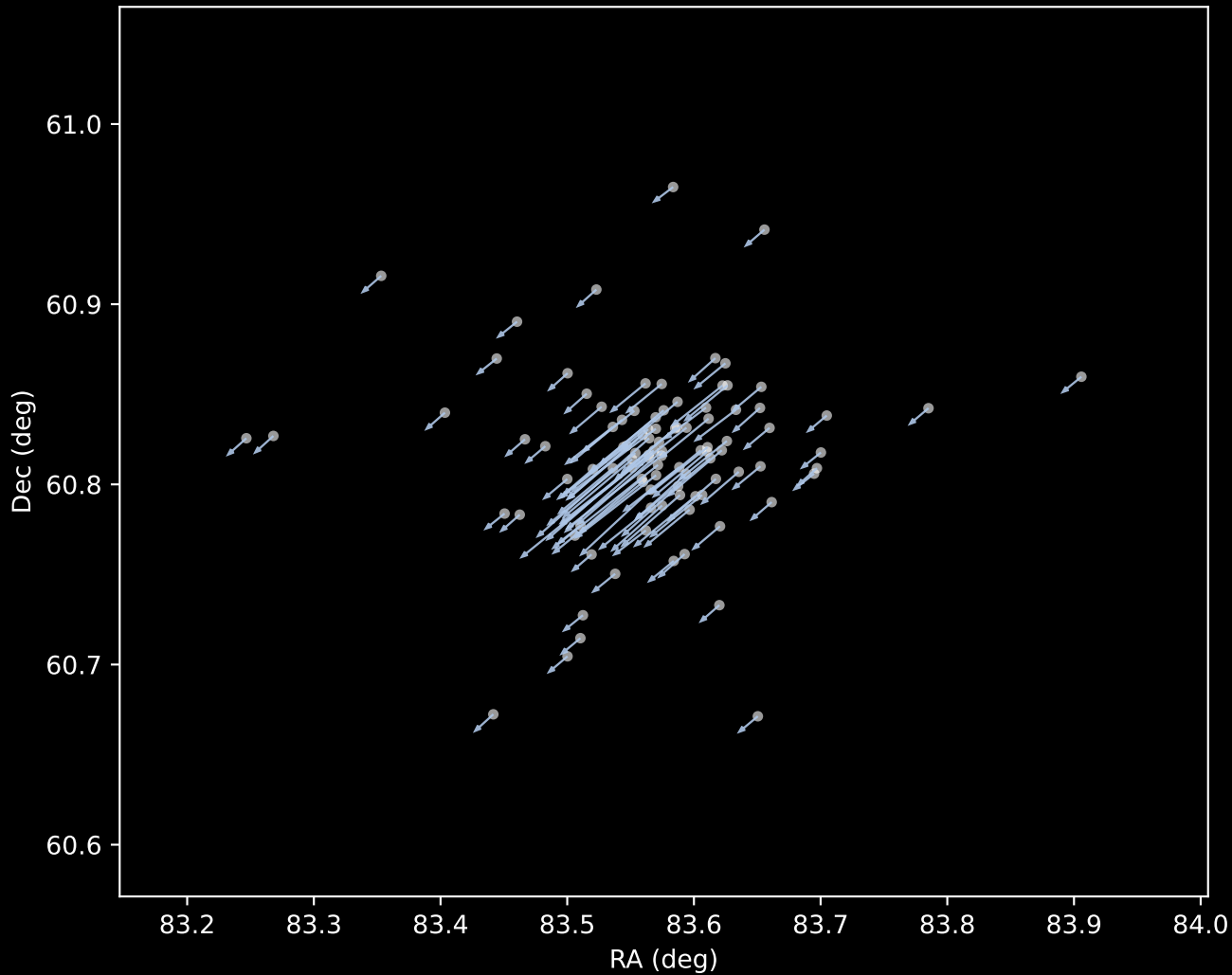
Gaia DR3 Cluster 1 Proper Motion Vectors (n=99)
