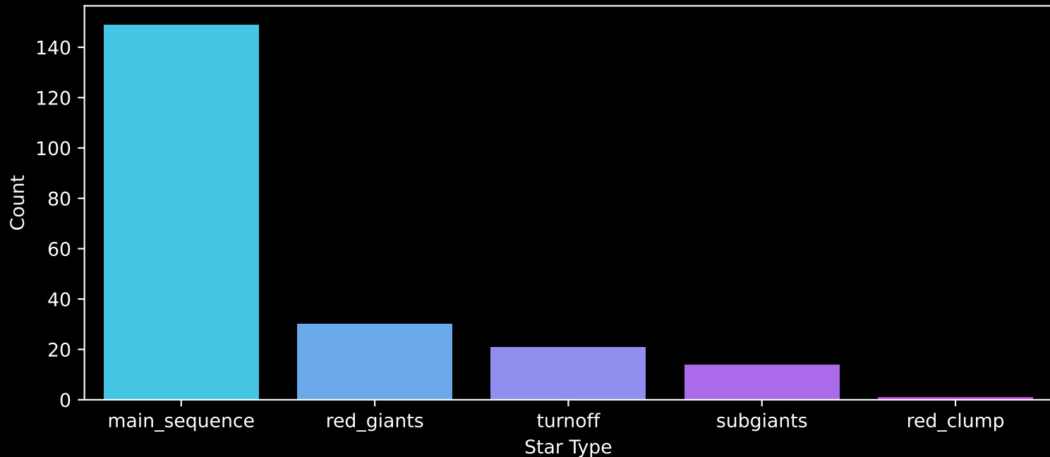
Gaia Cluster: [NGC_7423] Count plot of Star Type
