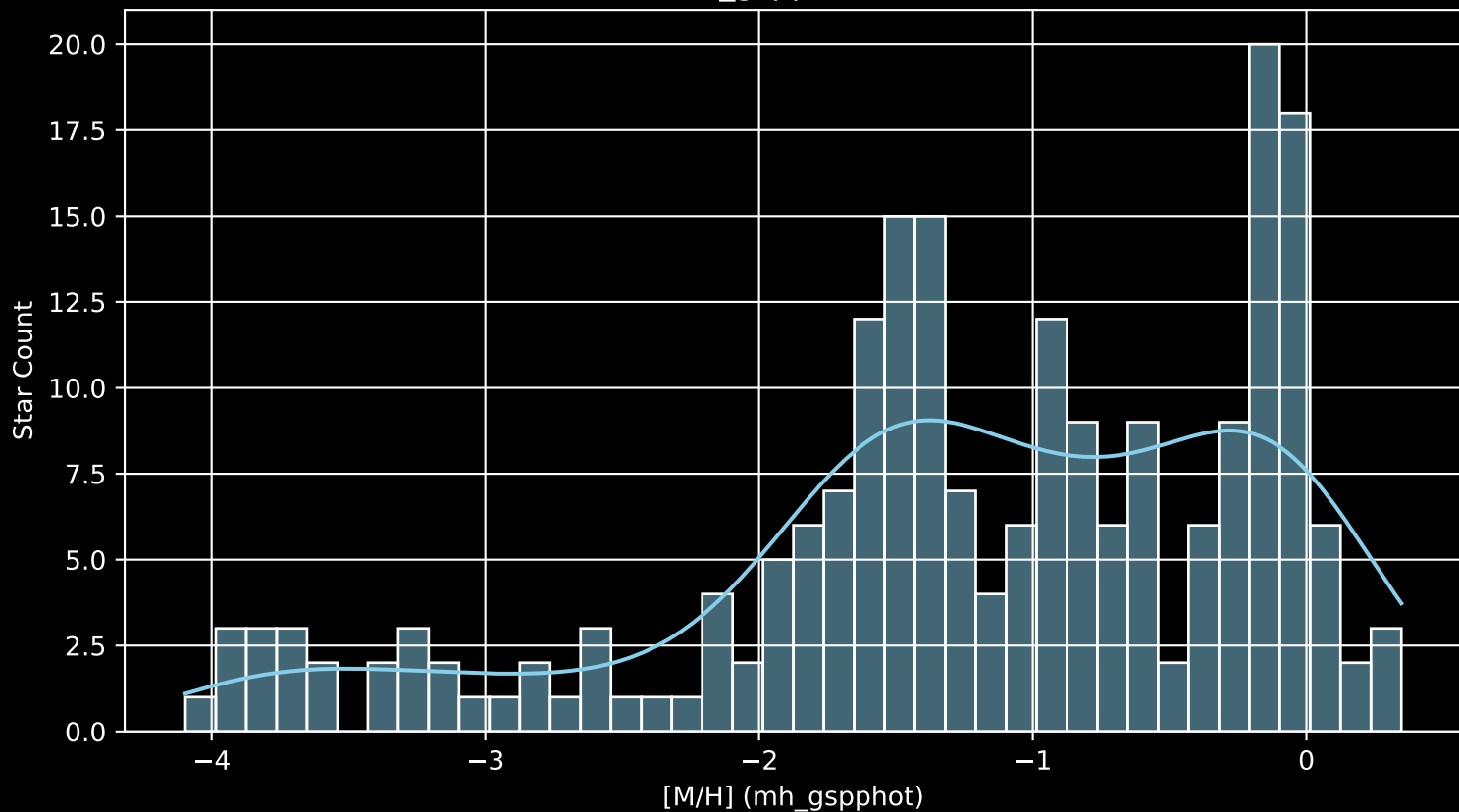
Gaia Cluster: [NGC_7423 [M/H] (mh_gspphot) (n= 215)
