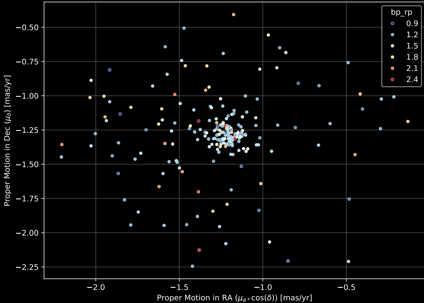
Gaia Cluster: [NGC_7423] Proper Motion Diagram (n= 215)
