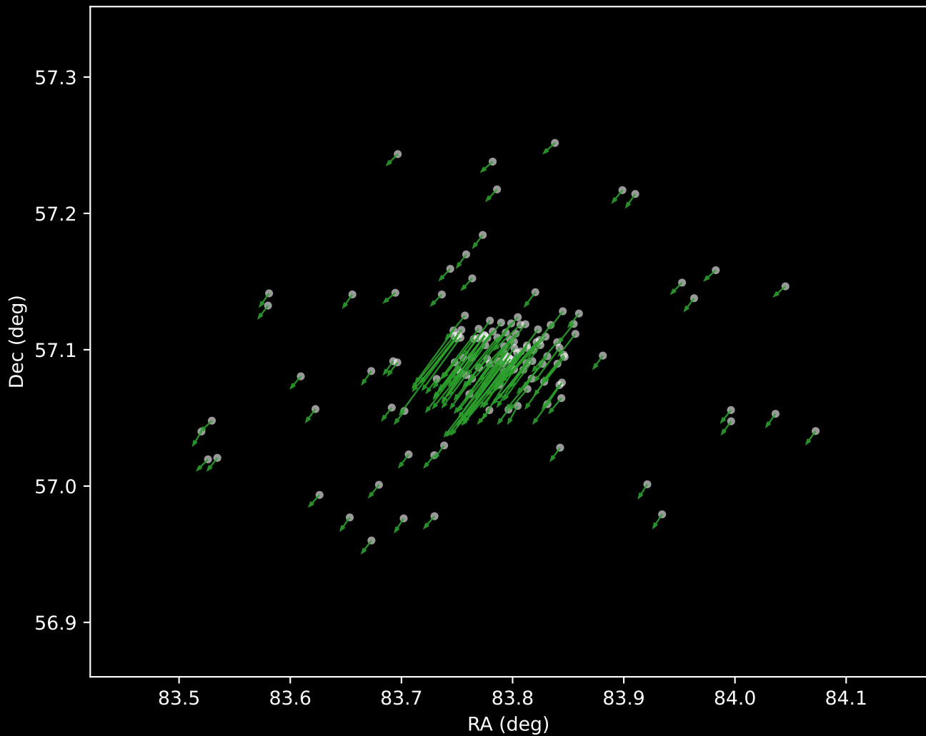
Gaia DR3 Cluster 4 Proper Motion Vectors (n=136)
