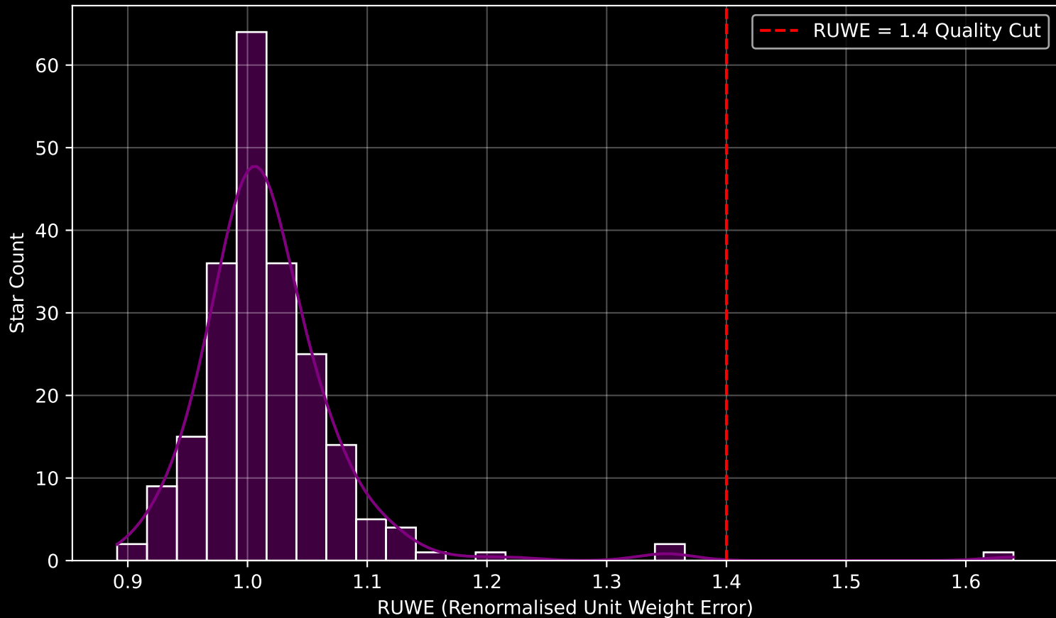
Gaia Cluster: [NGC_7423] RUWE Distribution (n= 215)
