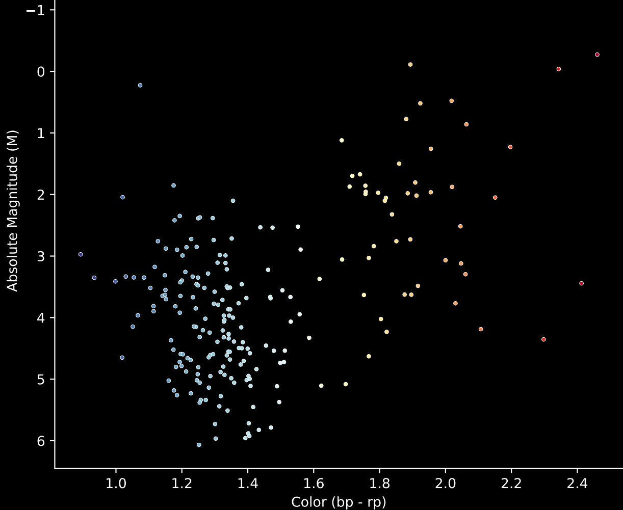
Gaia Cluster: [NGC_7423] Stars (n= 215) Hertzsprung-Russel Diagram
