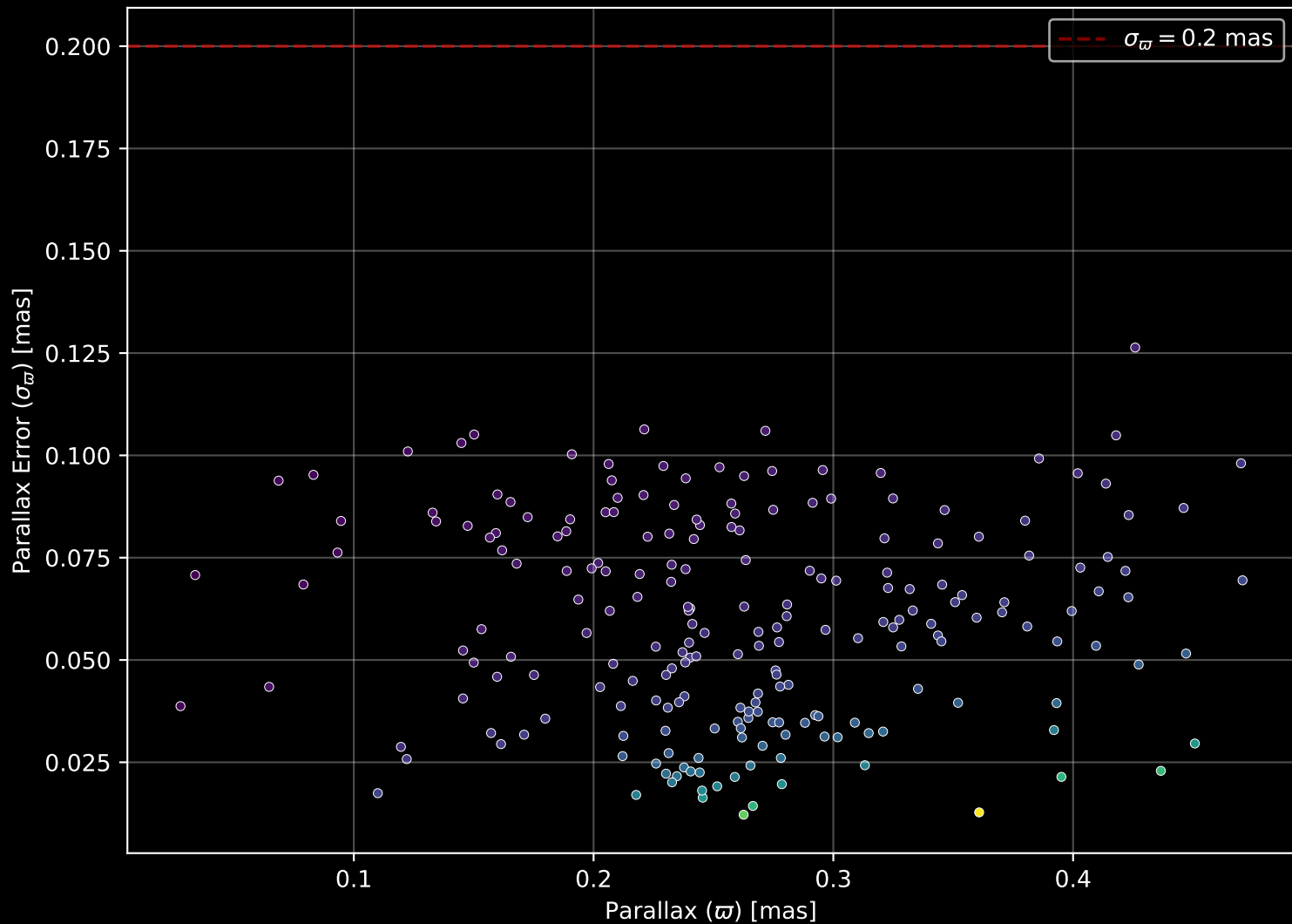
Gaia Cluster: [NGC_7423] Parallax Quality (n= 215)
