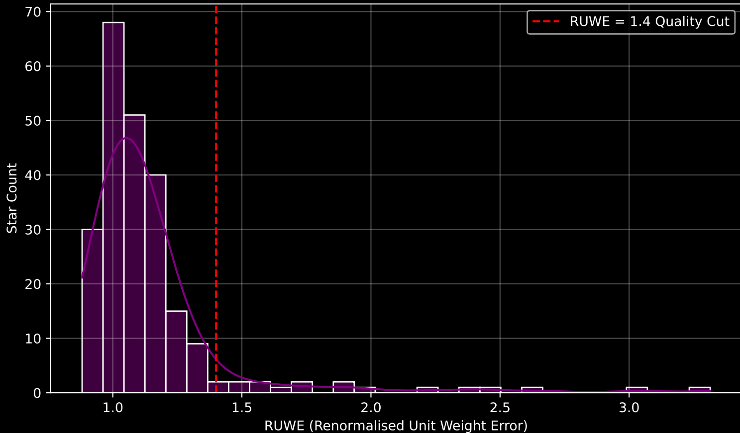
Gaia Cluster: [NGC_752] RUWE Distribution (n= 231)
