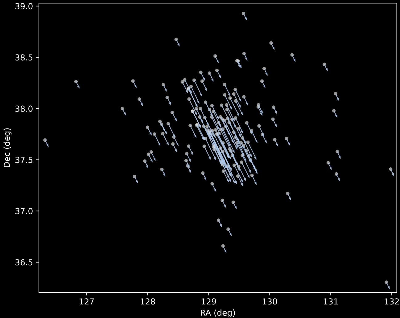
Gaia DR3 Cluster 1 Proper Motion Vectors (n=152)
