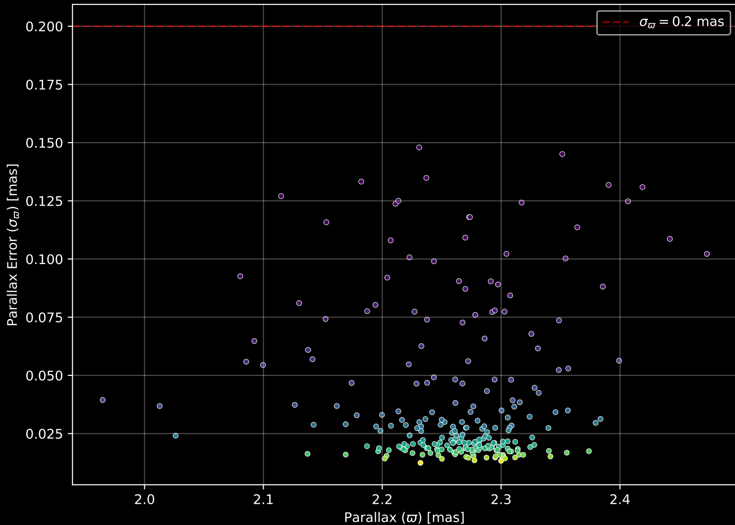
Gaia Cluster: [NGC_752] Parallax Quality (n= 232)
