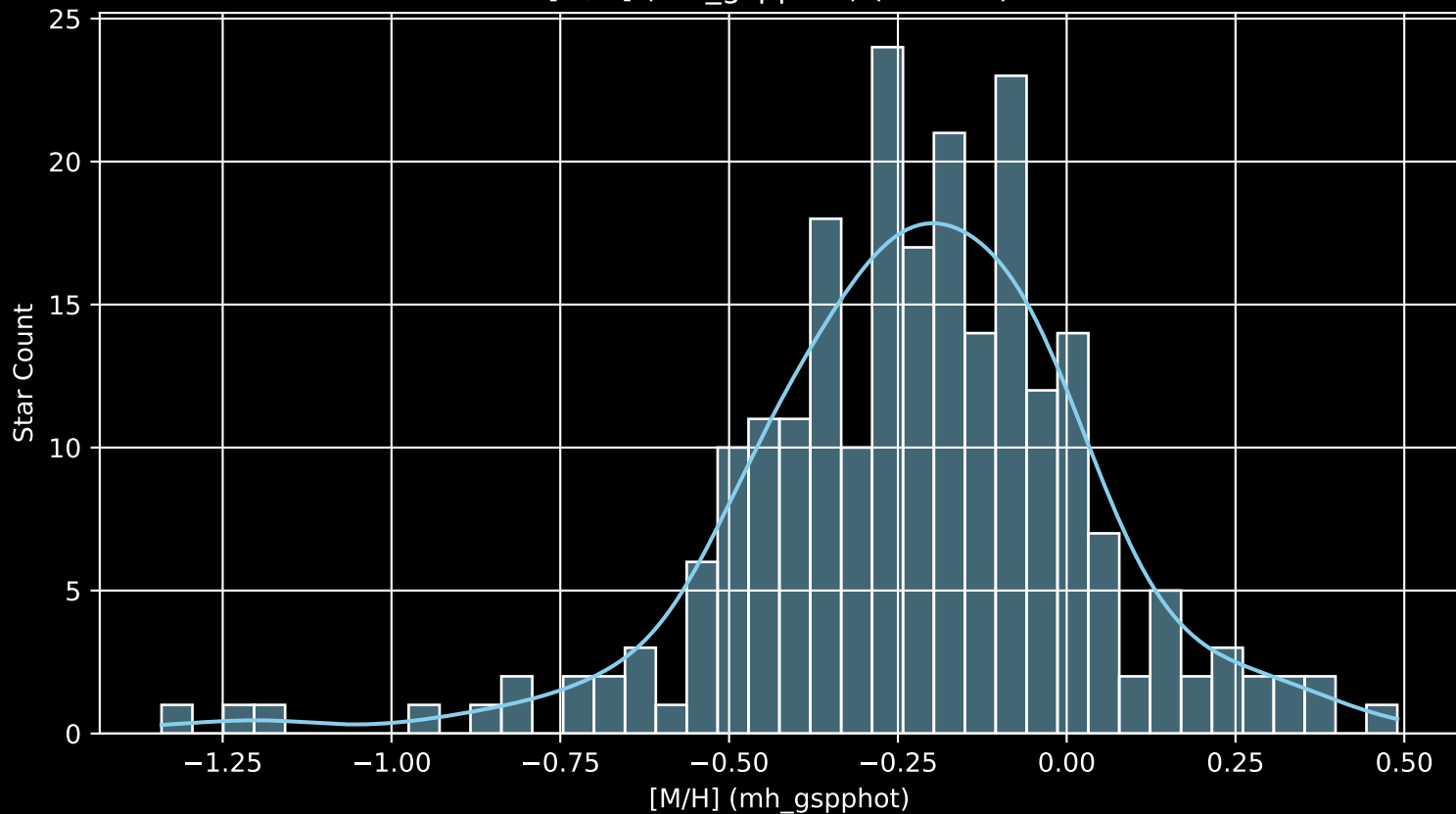
Gaia Cluster: [NGC_752 [M/H] (mh_gspphot) (n= 232)
