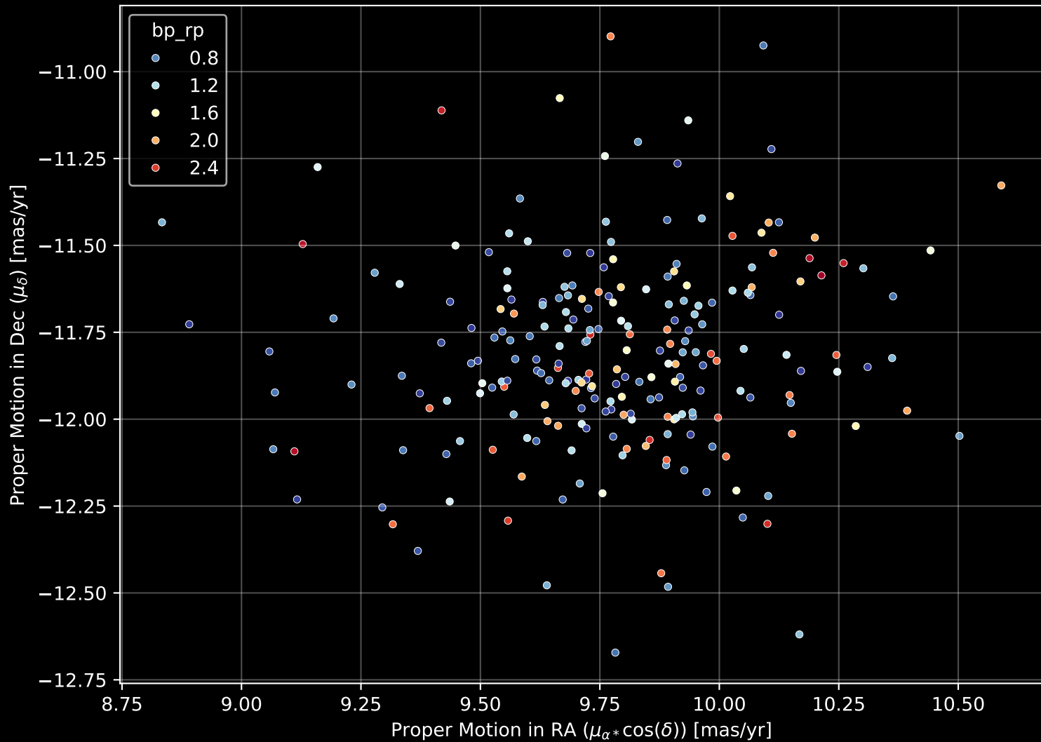
Gaia Cluster: [NGC_752] Proper Motion Diagram (n= 232)
