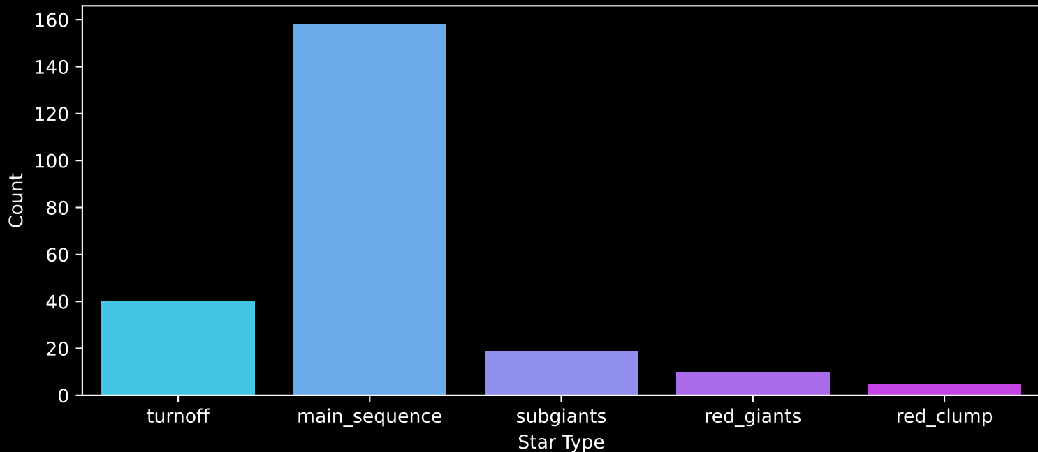
Gaia Cluster: [NGC_752] Count plot of Star Type
