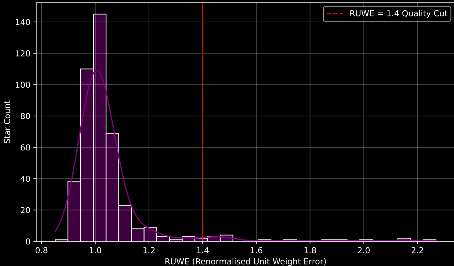
Gaia Cluster: [NGC_7762] RUWE Distribution (n= 427)
