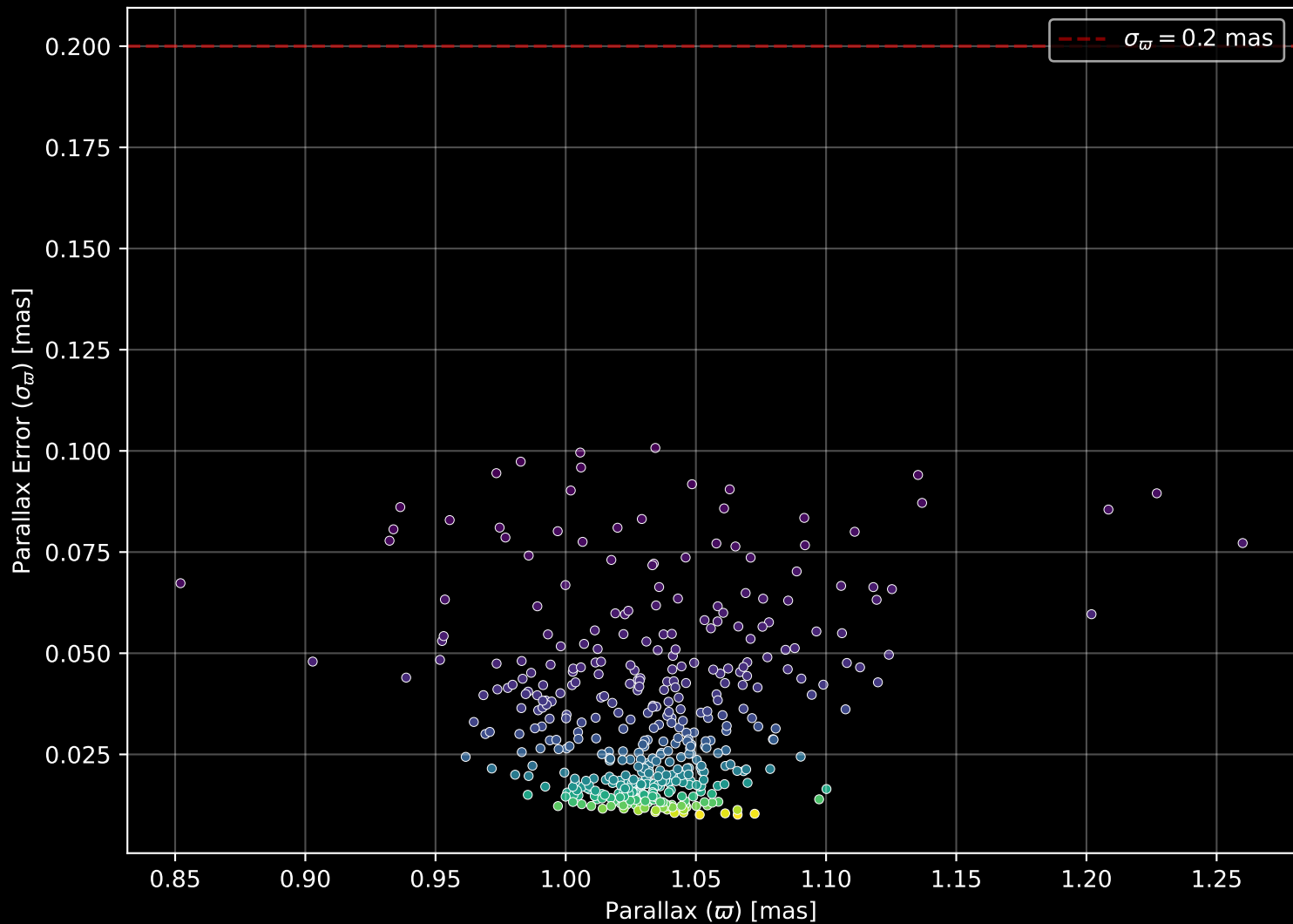
Gaia Cluster: [NGC_7762] Parallax Quality (n= 427)
