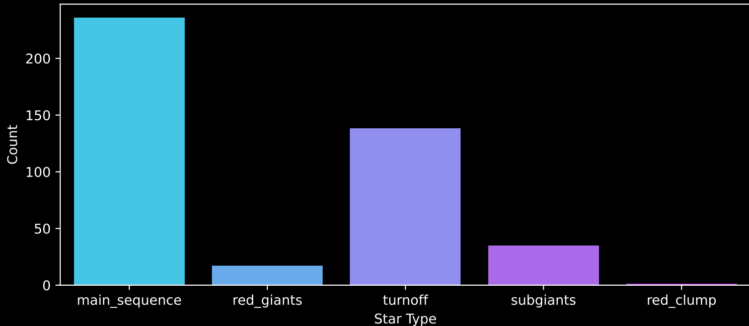
Gaia Cluster: [NGC_7762] Count plot of Star Type
