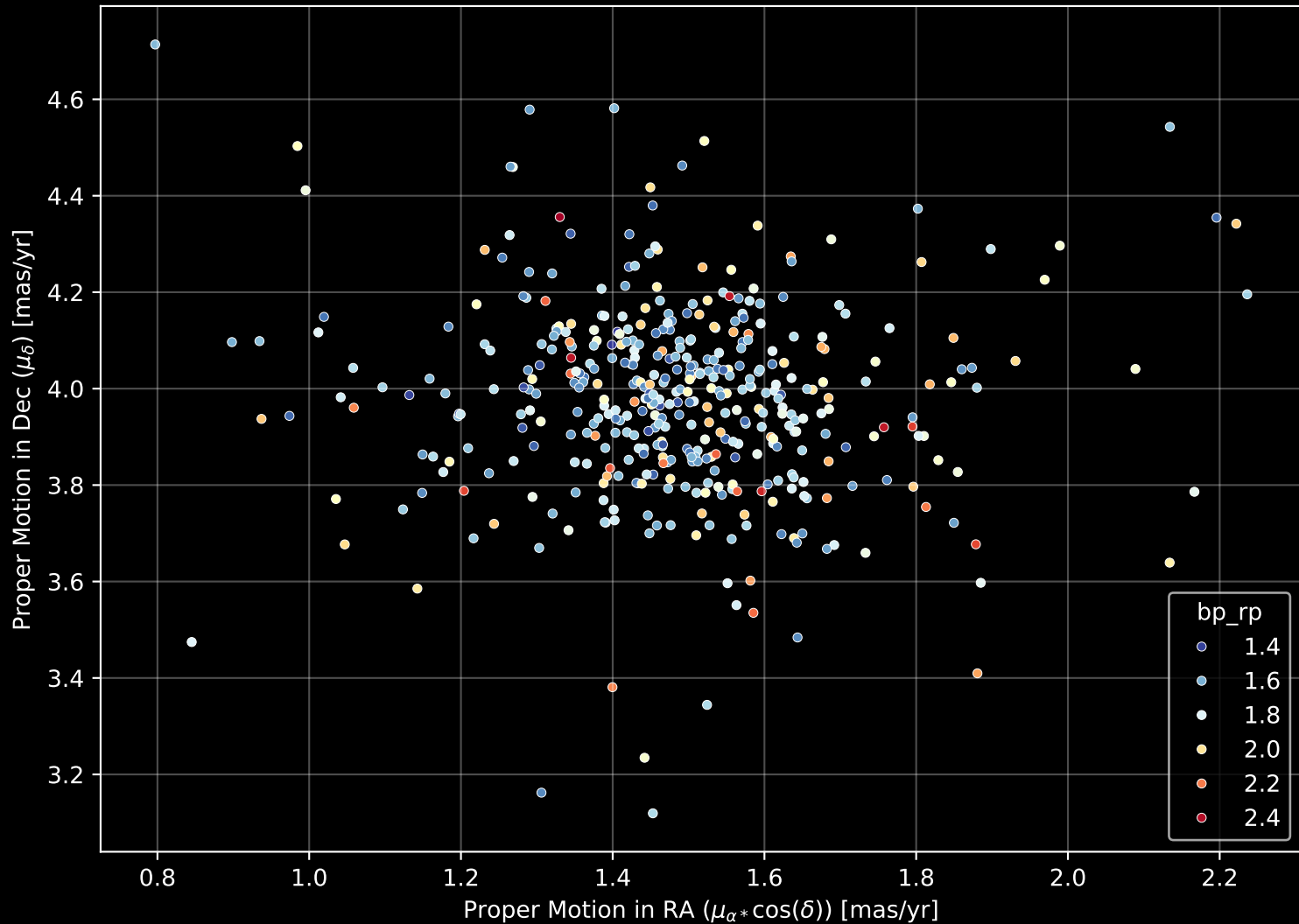
Gaia Cluster: [NGC_7762] Proper Motion Diagram (n= 427)
