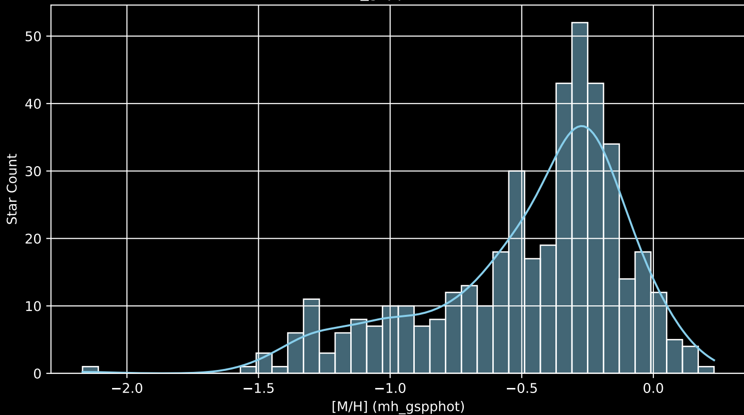
Gaia Cluster: [NGC_7762 [M/H] (mh_gspphot) (n= 427)
