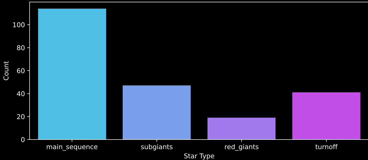
Gaia Cluster: [NGC_7788] Count plot of Star Type
