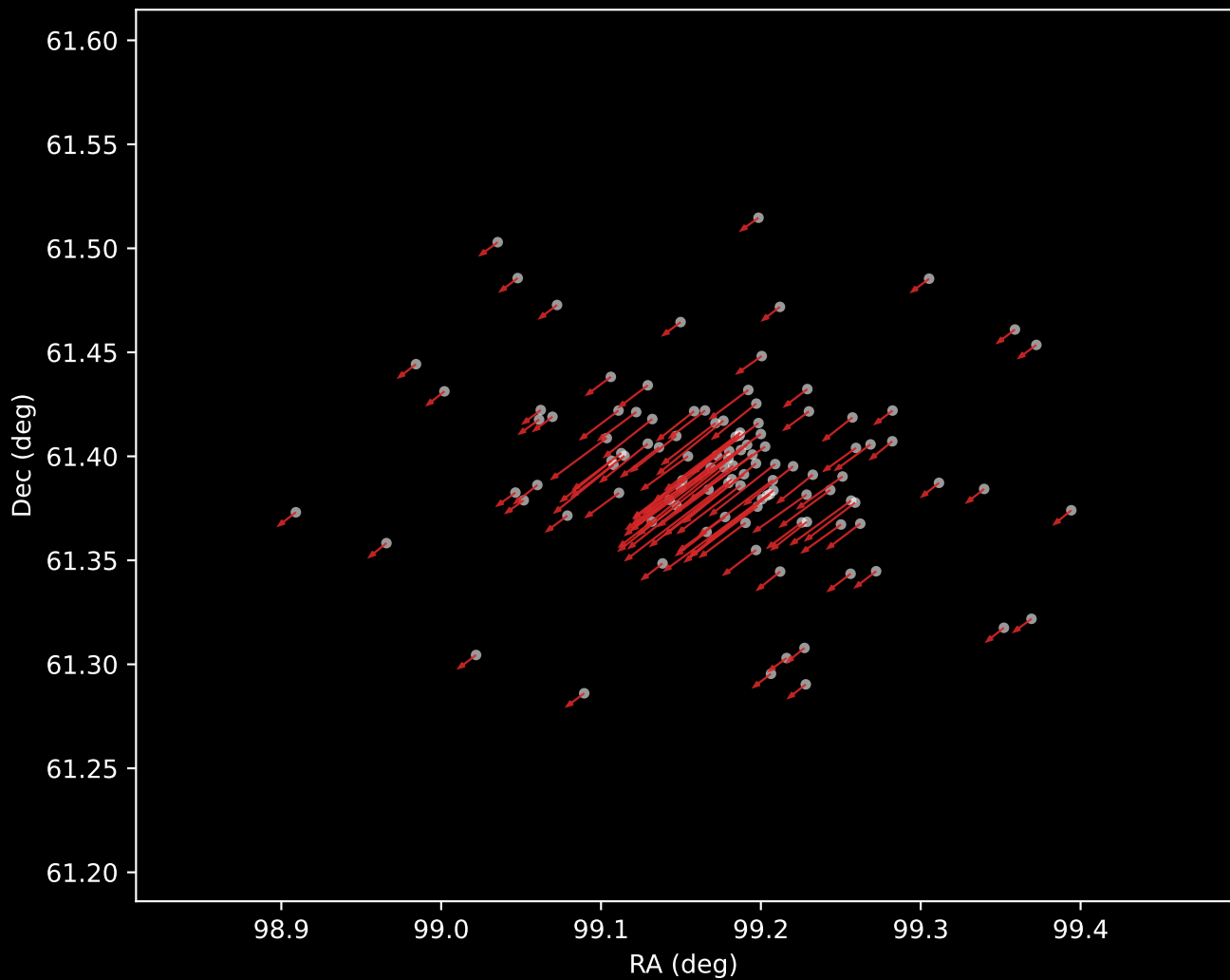
Gaia DR3 Cluster 6 Proper Motion Vectors (n=112)
