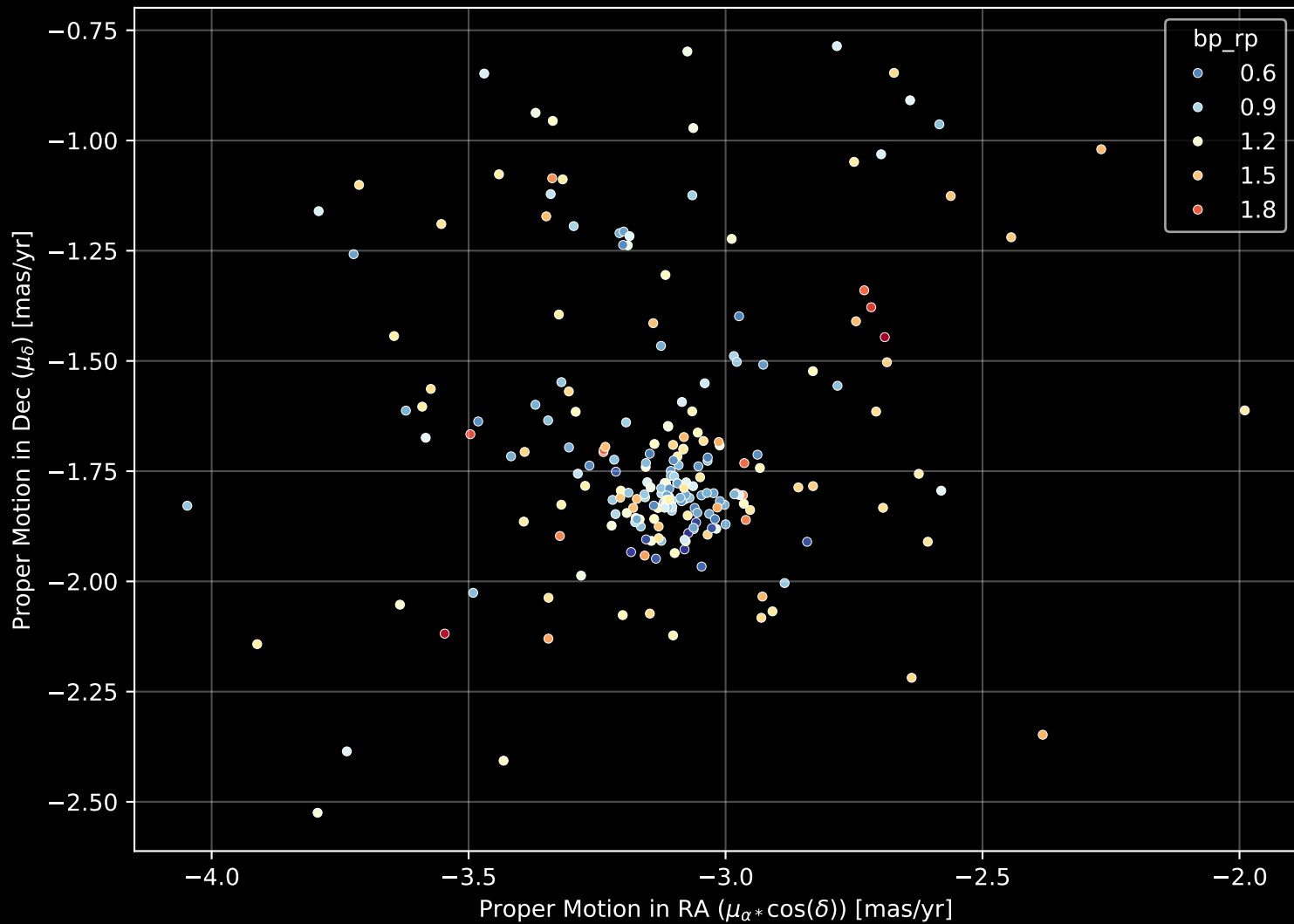
Gaia Cluster: [NGC_7788] Proper Motion Diagram (n= 221)
