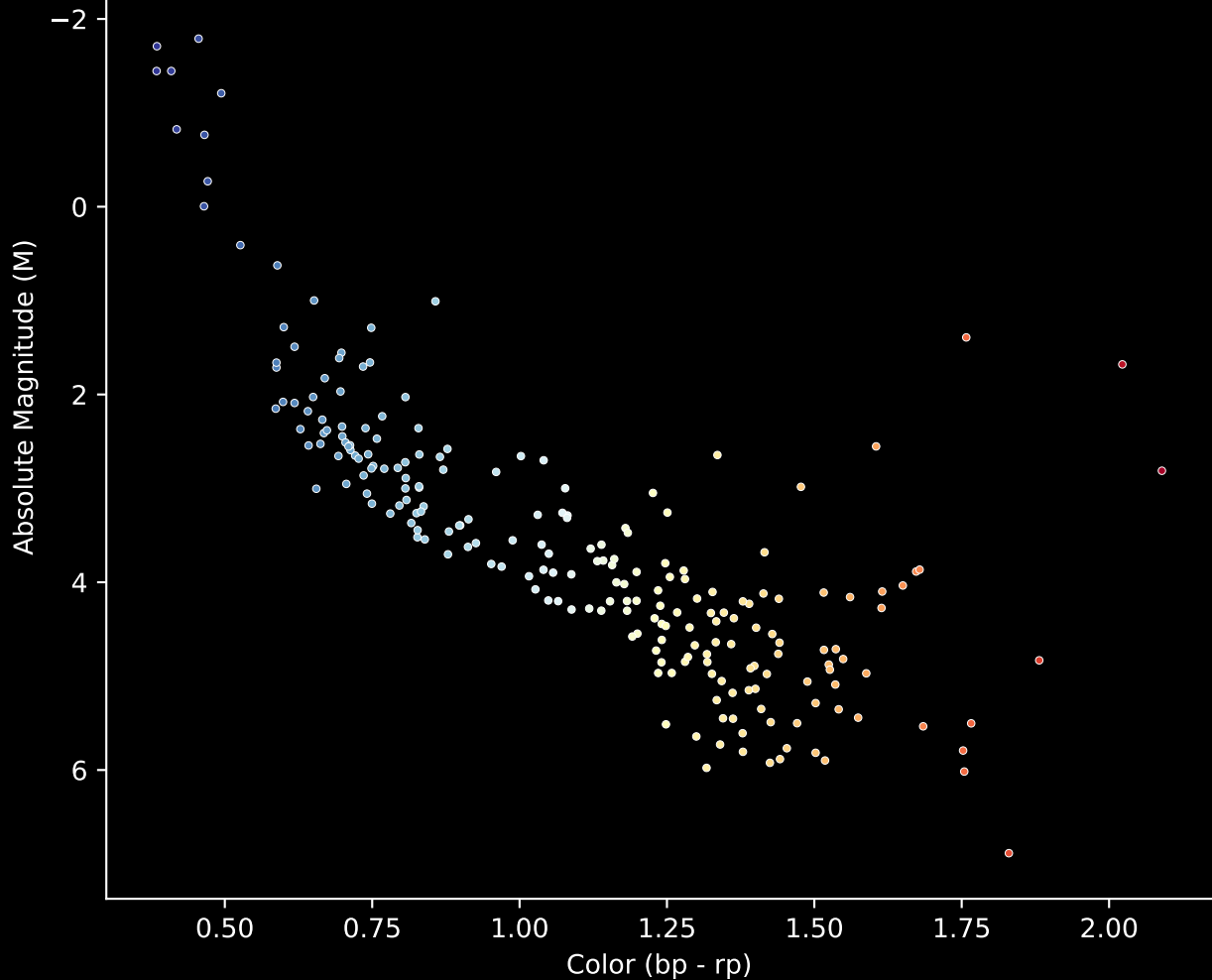
Gaia Cluster: [NGC_7788] Stars (n= 221) Hertzsprung-Russel Diagram
