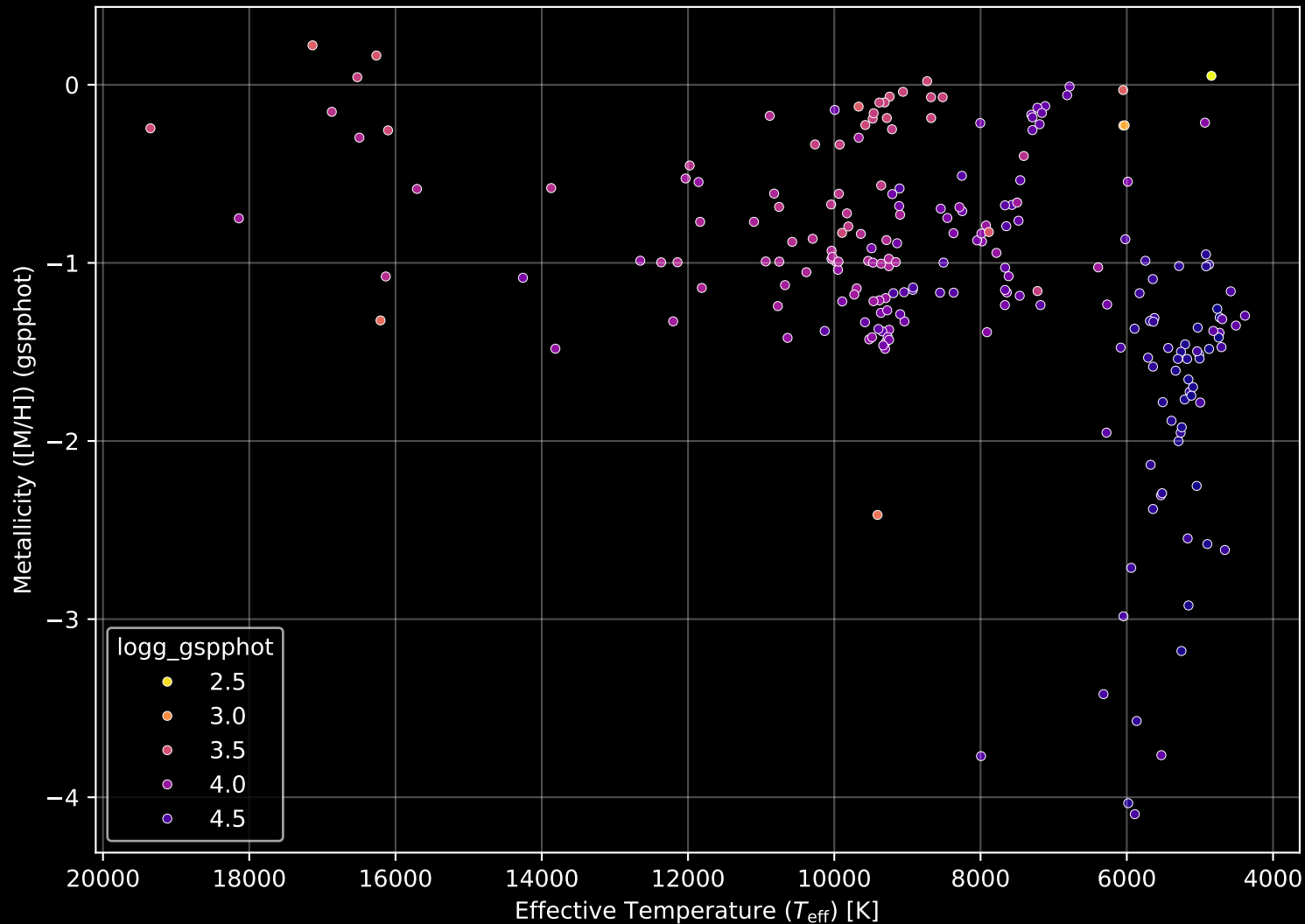
Gaia Cluster: [NGC_7788] Stellar Population Parameters (n= 221)
