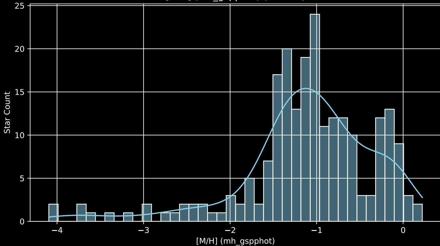
Gaia Cluster: [NGC_7788 [M/H] (mh_gspphot) (n= 221)
