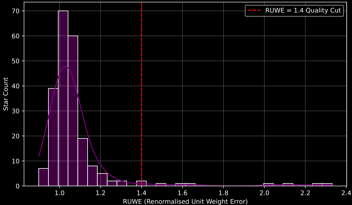
Gaia Cluster: [NGC_7788] RUWE Distribution (n= 221)
