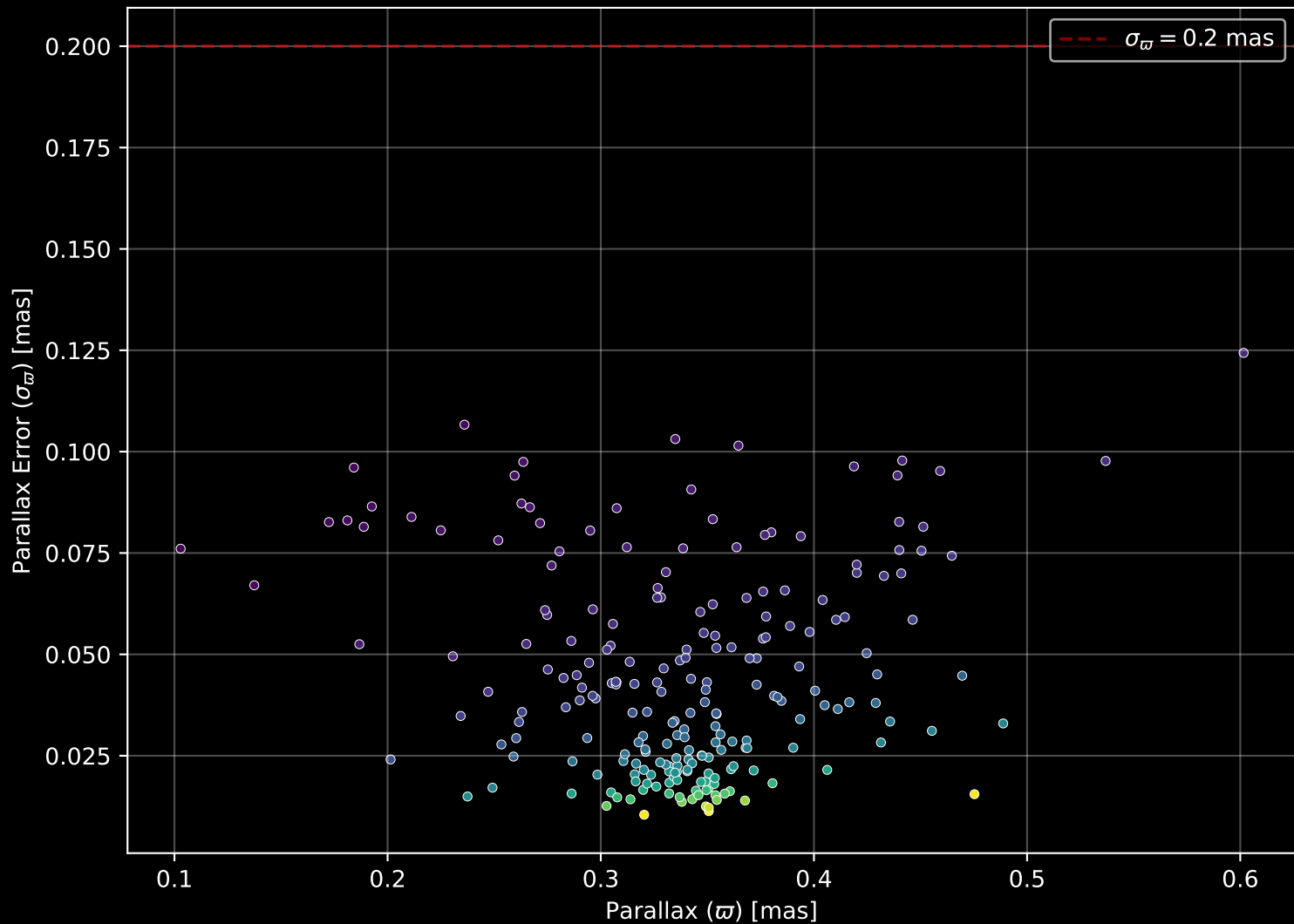
Gaia Cluster: [NGC_7788] Parallax Quality (n= 221)
