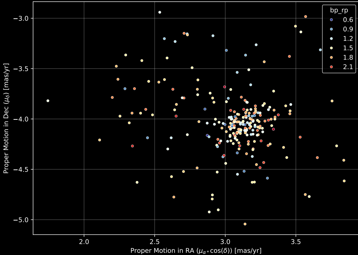
Gaia Cluster: [NGC_886] Proper Motion Diagram (n= 251)
