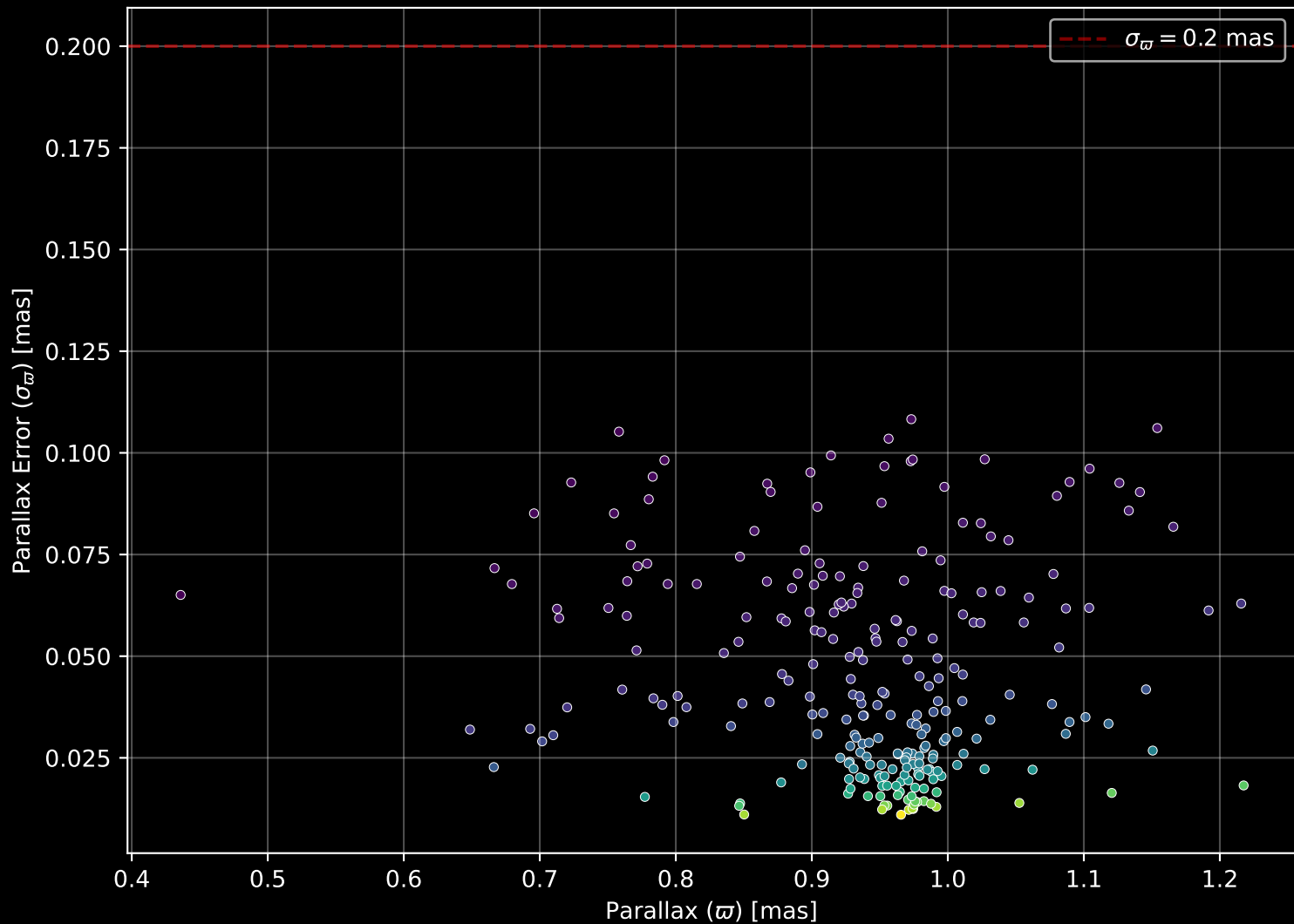
Gaia Cluster: [NGC_886] Parallax Quality (n= 251)
