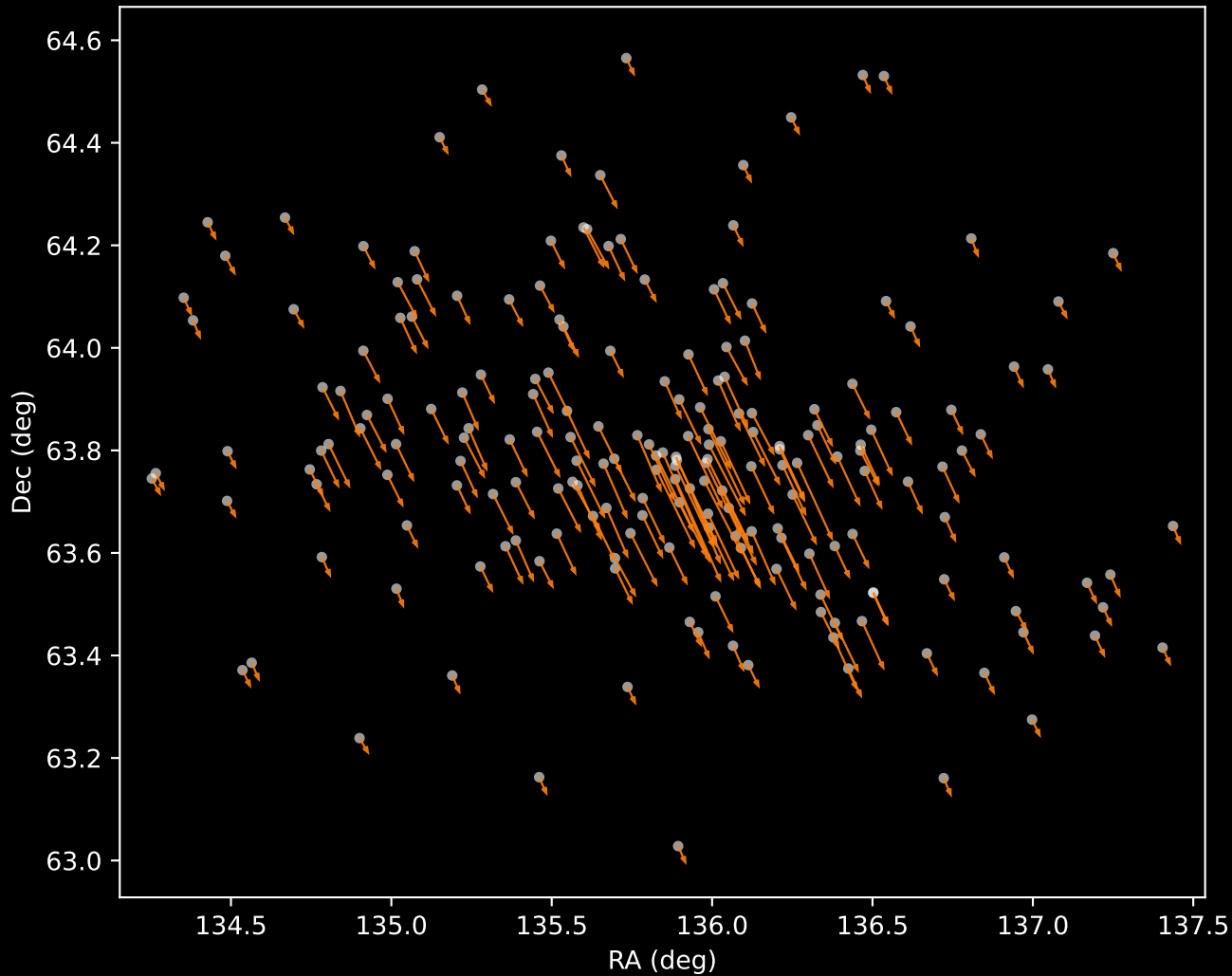
Gaia DR3 Cluster 2 Proper Motion Vectors (n=197)
