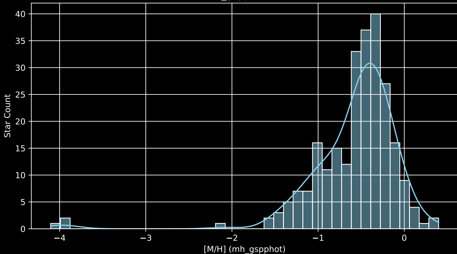
Gaia Cluster: [NGC_886 [M/H] (mh_gspphot) (n= 251)
