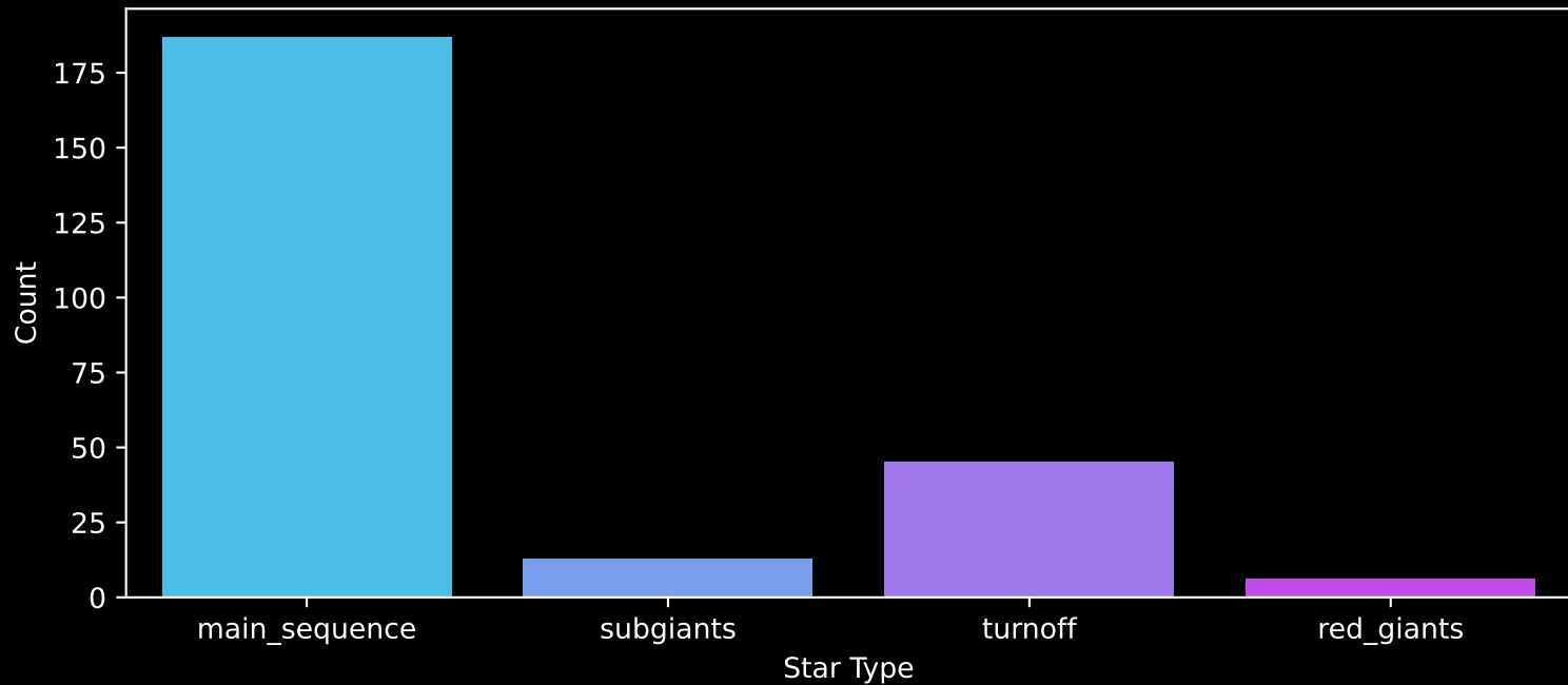
Gaia Cluster: [NGC_886] Count plot of Star Type
