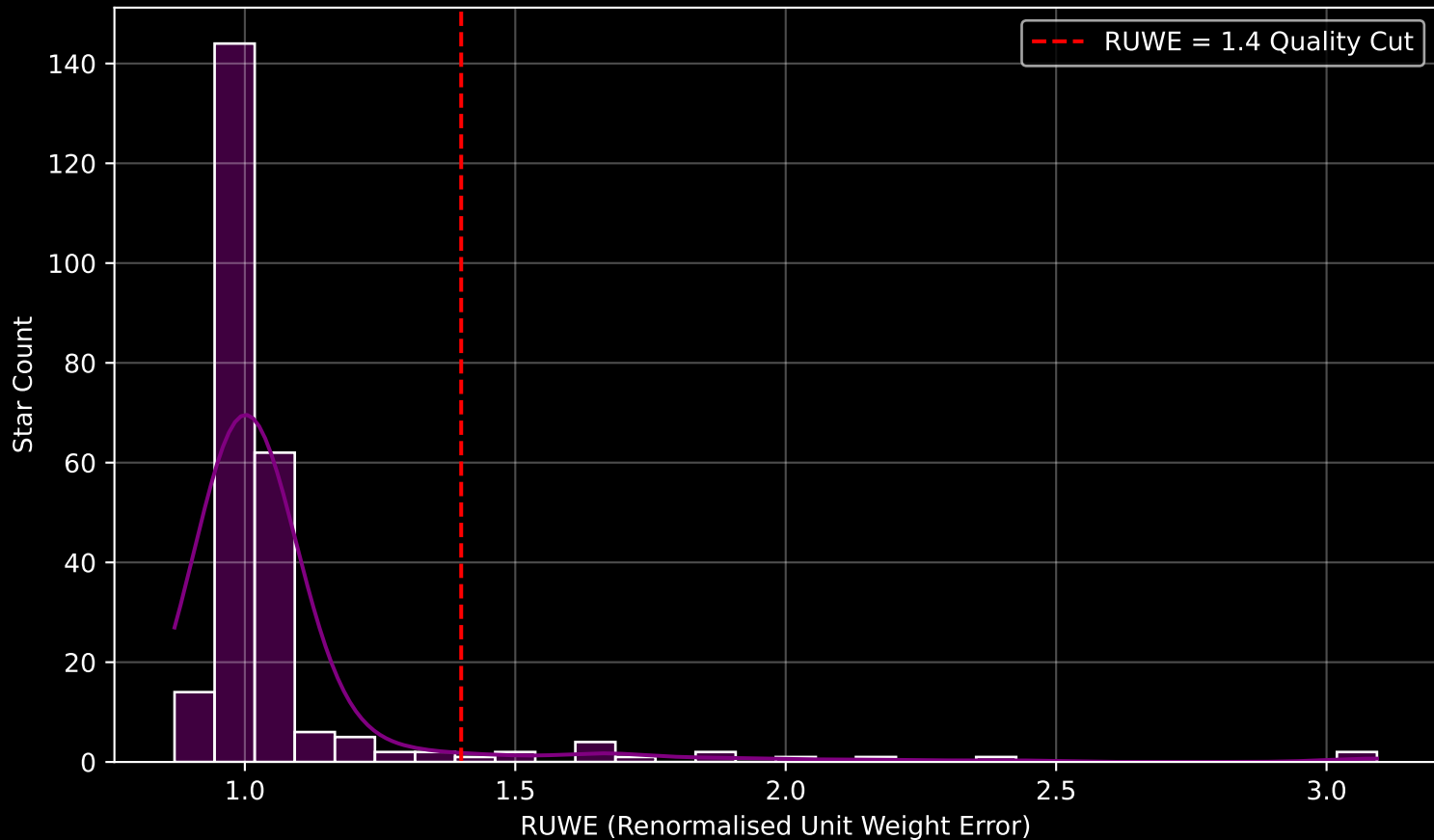
Gaia Cluster: [NGC_886] RUWE Distribution (n= 250)
