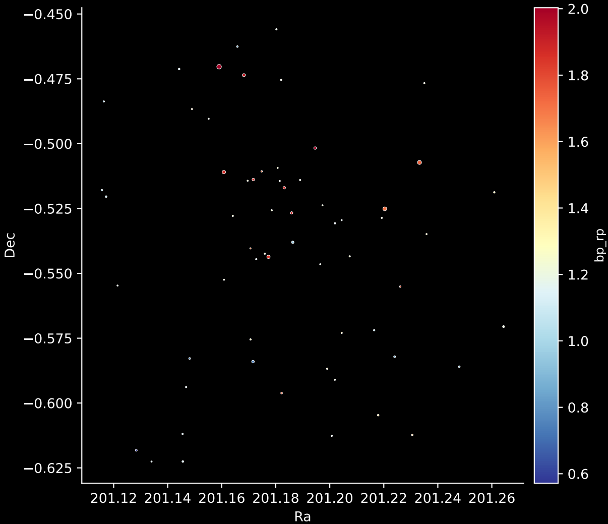
Gaia Cluster: [Patchick_90] Stars: 61
