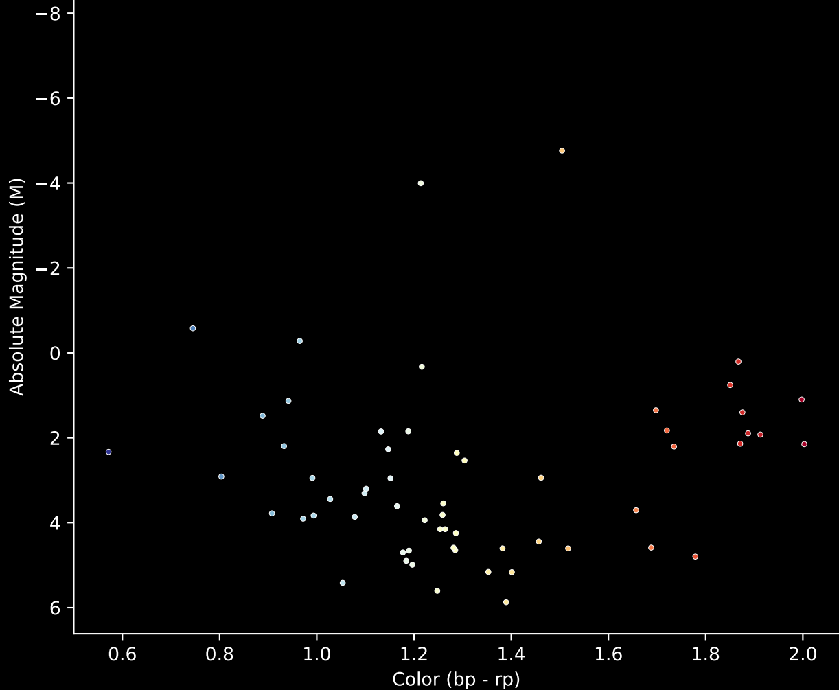
Gaia Cluster: [Patchick_90] Stars (n= 61) Hertzsprung-Russel Diagram
