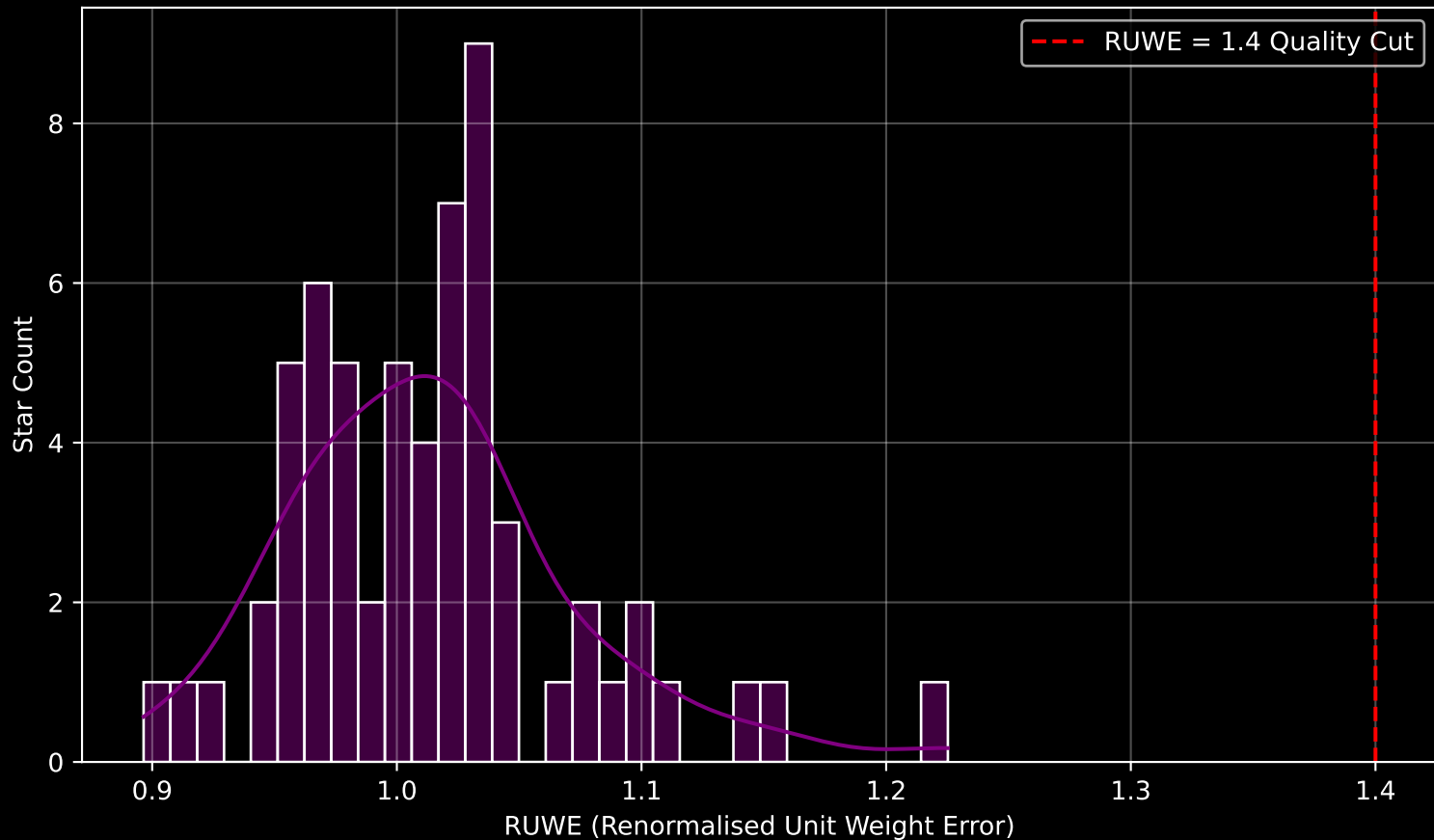
Gaia Cluster: [Patchick_90] RUWE Distribution (n= 61)
