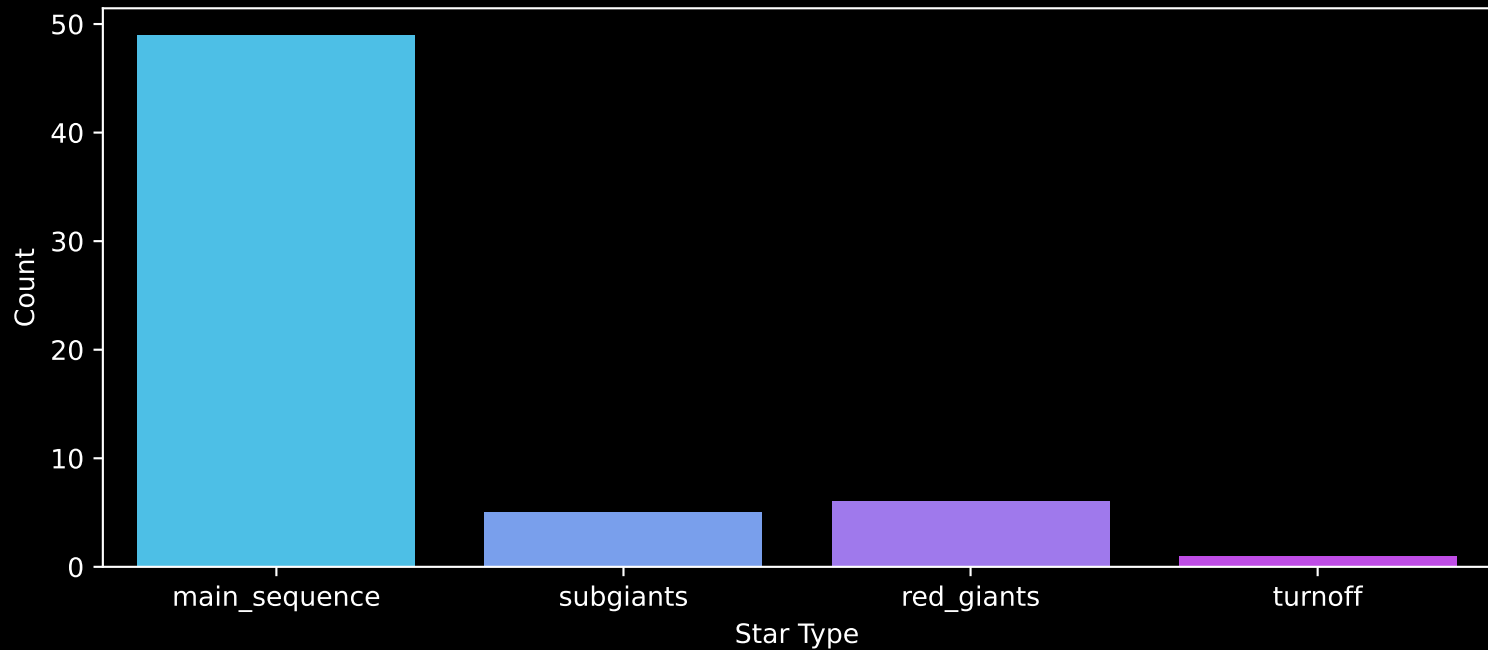
Gaia Cluster: [Patchick_90] Count plot of Star Type
