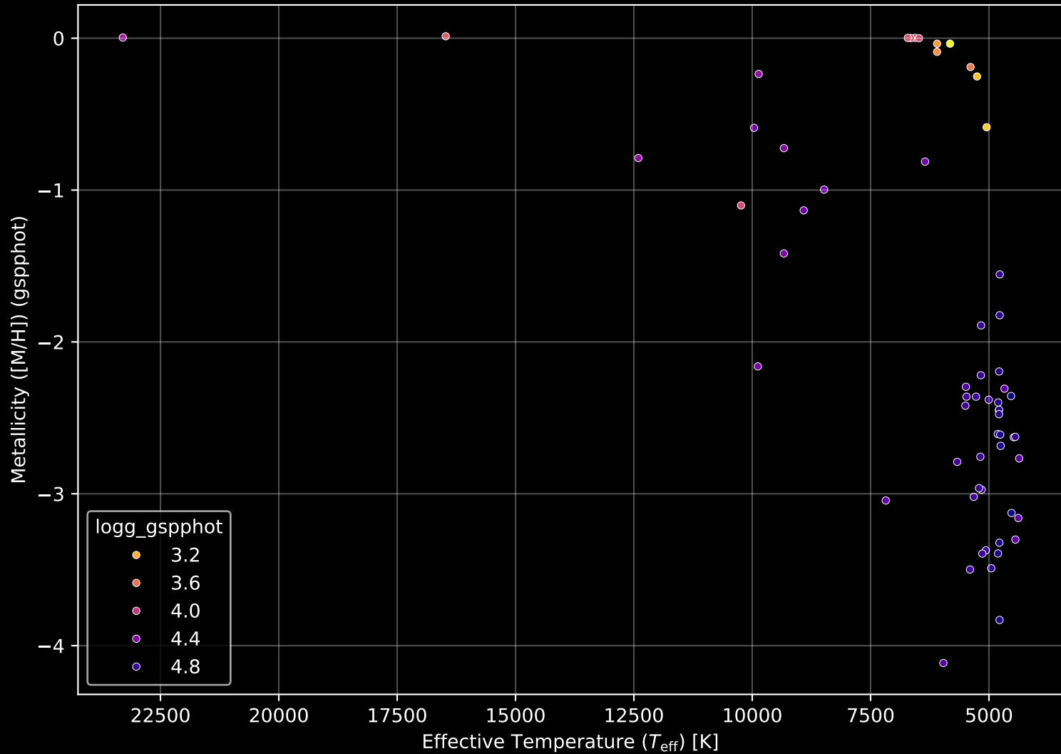
Gaia Cluster: [Patchick_90] Stellar Population Parameters (n= 61)
