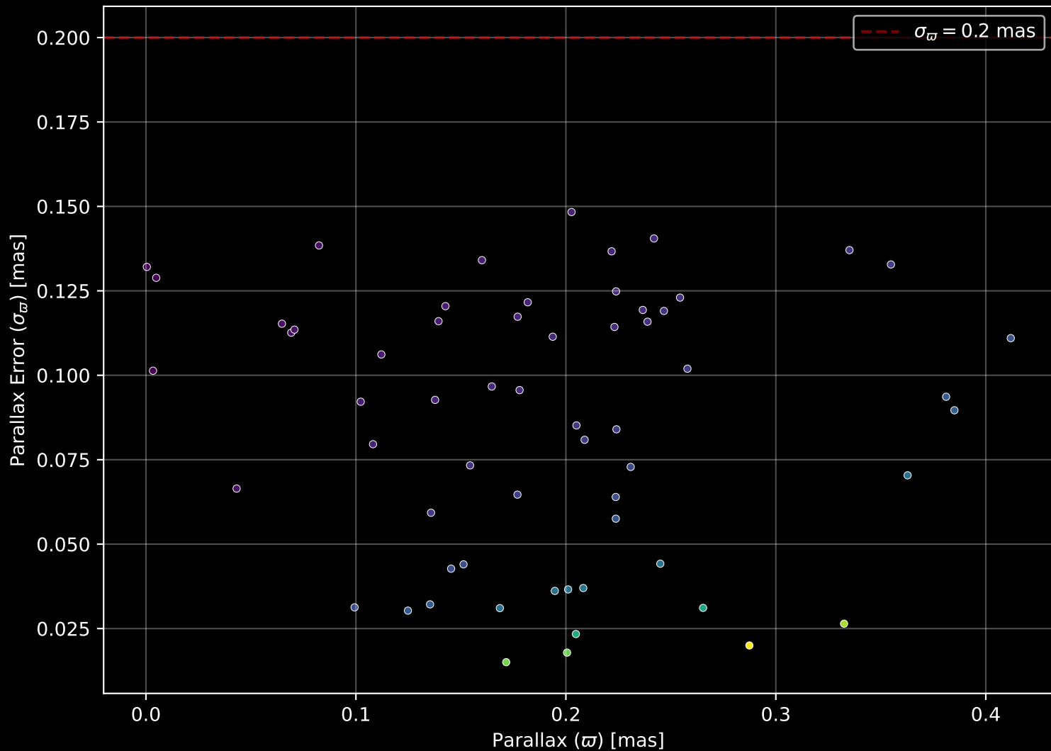
Gaia Cluster: [Patchick_90] Parallax Quality (n= 61)
