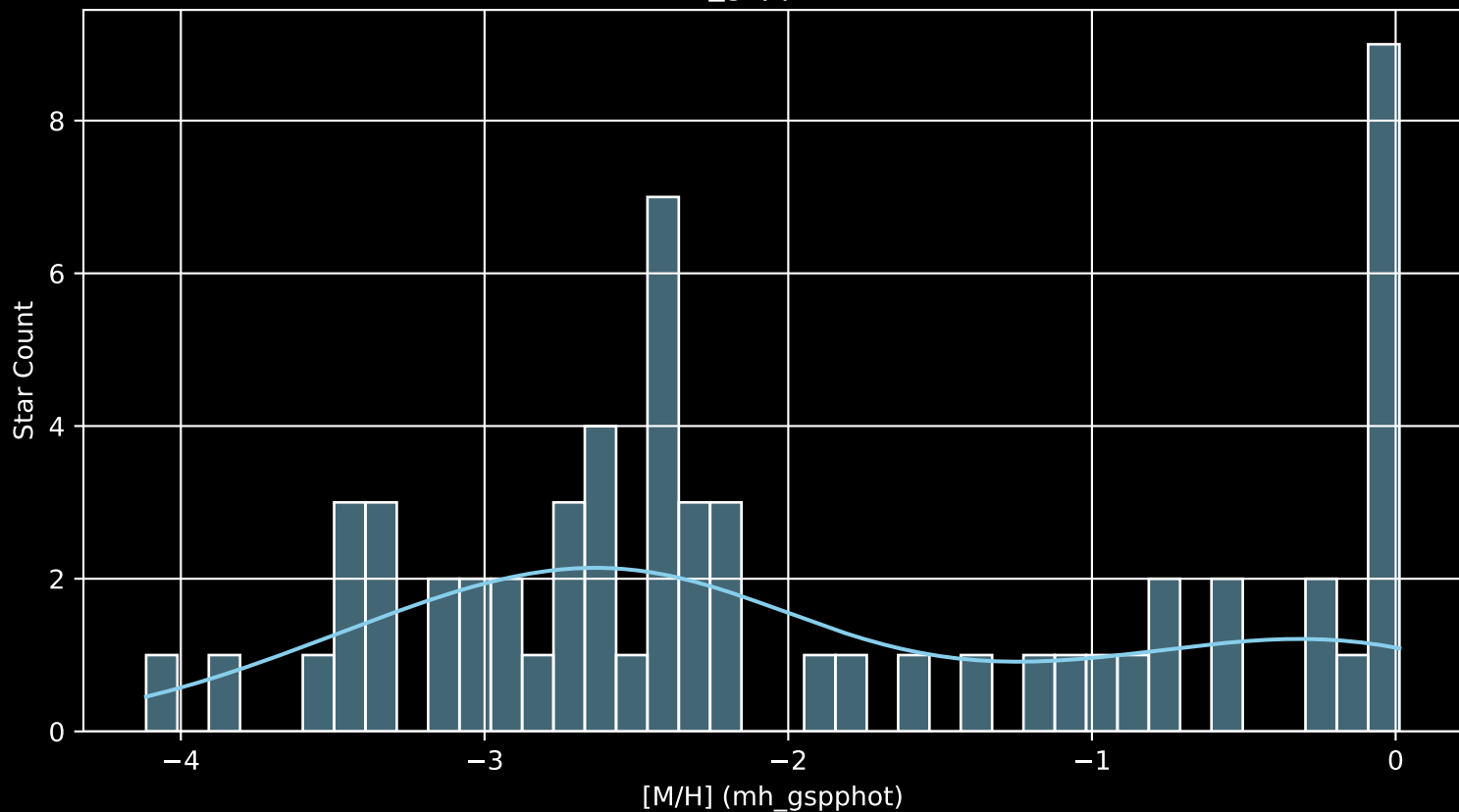
Gaia Cluster: [Patchick_90 [M/H] (mh_gspphot) (n= 61)
