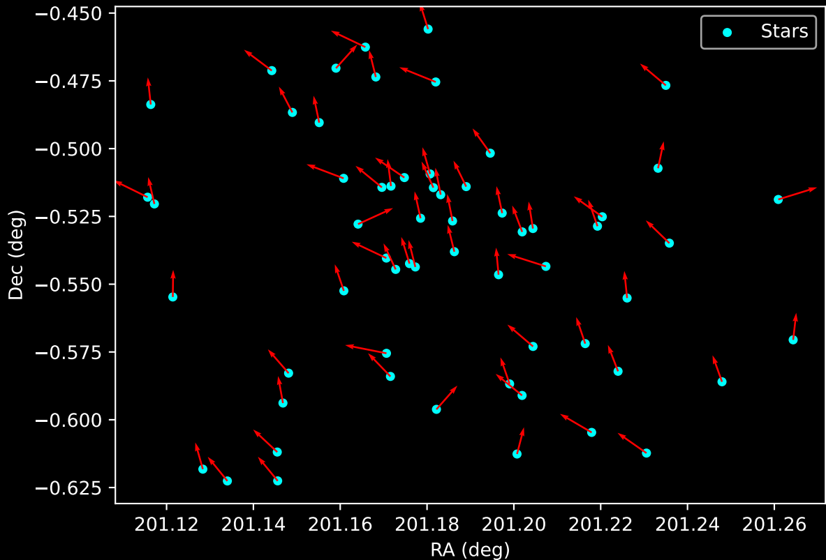
Gaia Cluster: [Patchick_90] Proper Motion Vectors for Gaia Star Field (n= 61)
