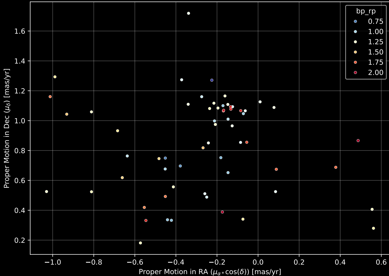
Gaia Cluster: [Patchick_90] Proper Motion Diagram (n= 61)
