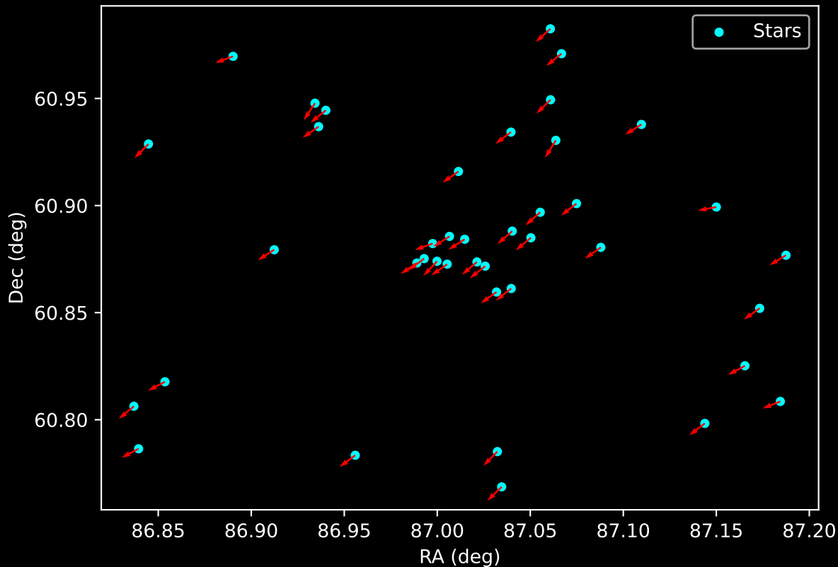
Gaia Cluster: [Pfleiderer_3] Proper Motion Vectors for Gaia Star Field (n= 41)
