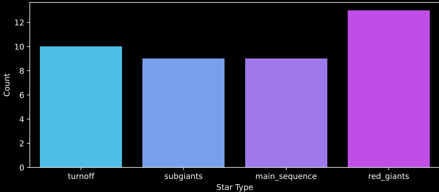
Gaia Cluster: [Pfleiderer_3] Count plot of Star Type
