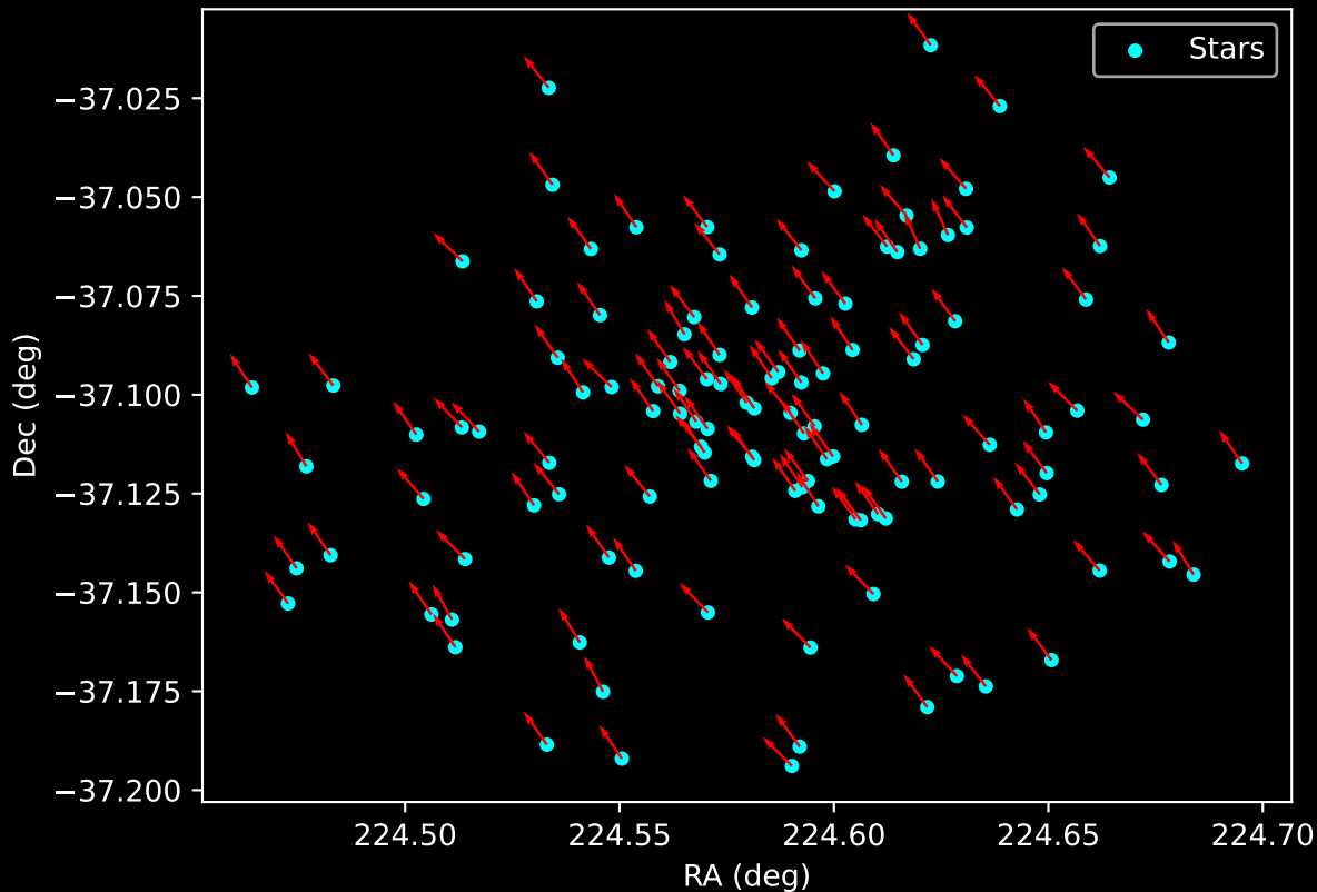
Gaia Cluster: [Pismis_1] Proper Motion Vectors for Gaia Star Field (n= 120)
