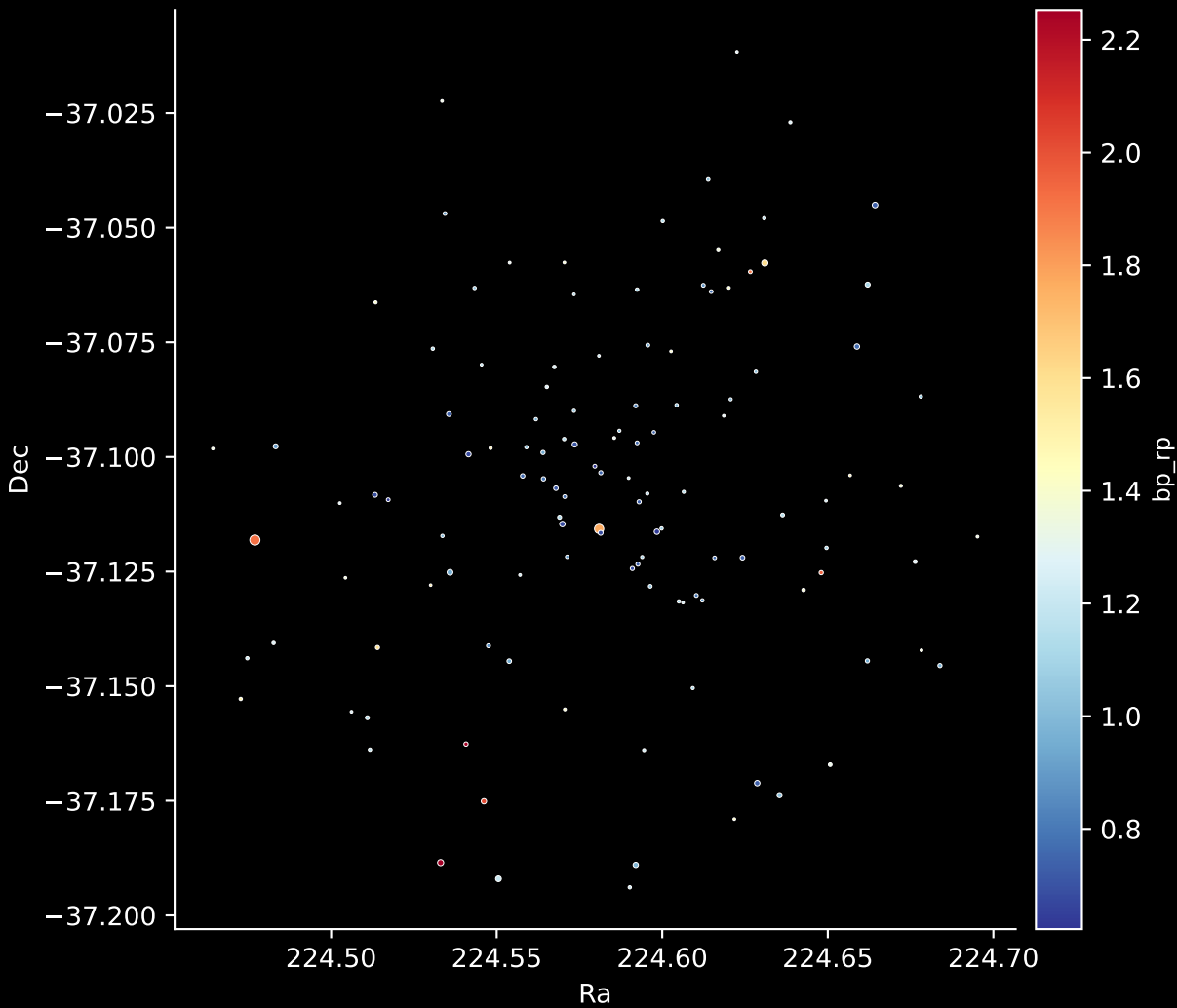
Gaia Cluster: [Pismis_1] Stars: 120
