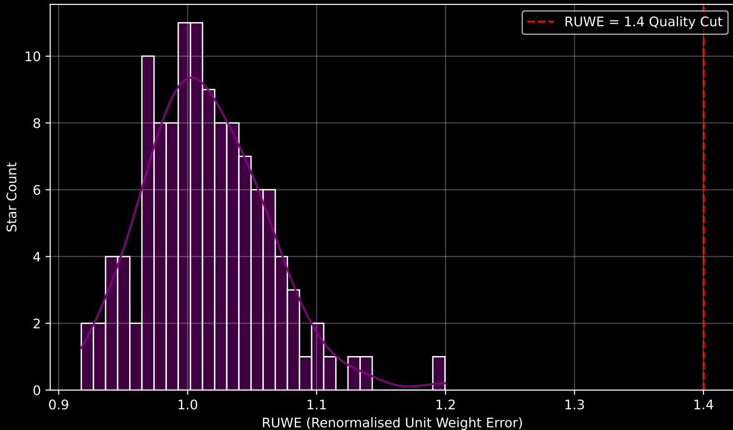
Gaia Cluster: [Pismis_1] RUWE Distribution (n= 120)
