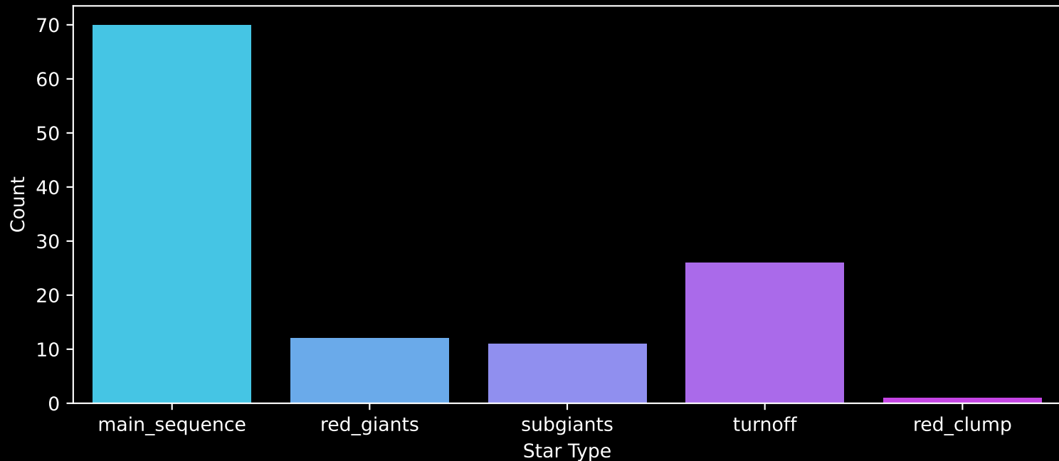
Gaia Cluster: [Pismis_1] Count plot of Star Type
