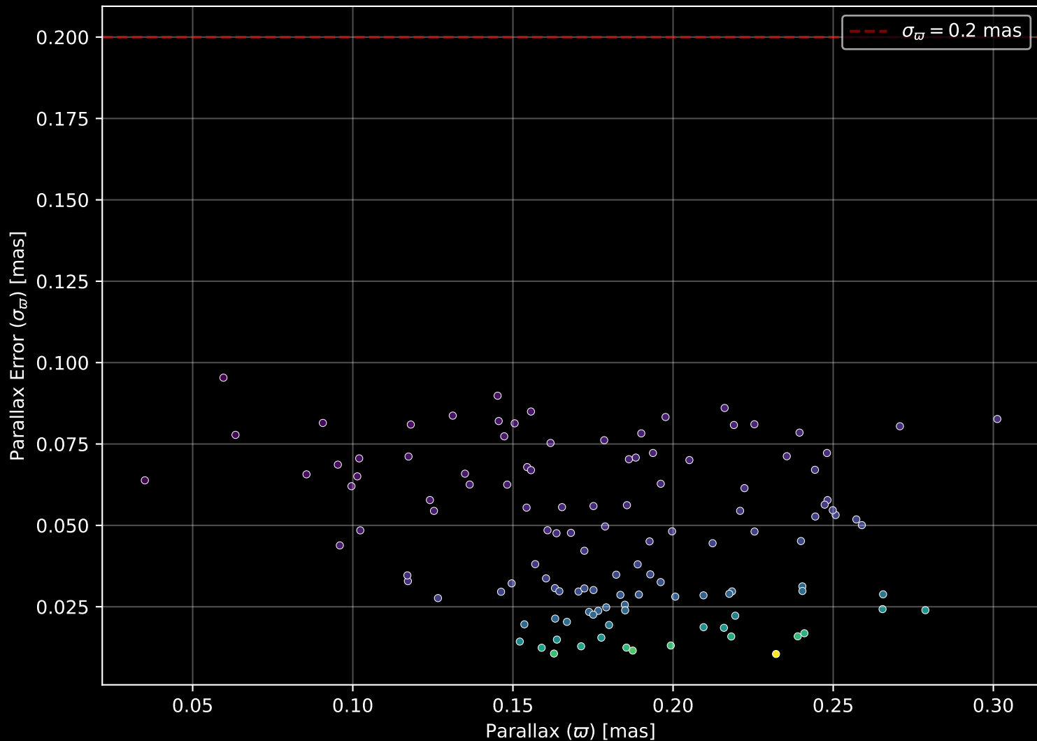
Gaia Cluster: [Pismis_1] Parallax Quality (n= 120)
