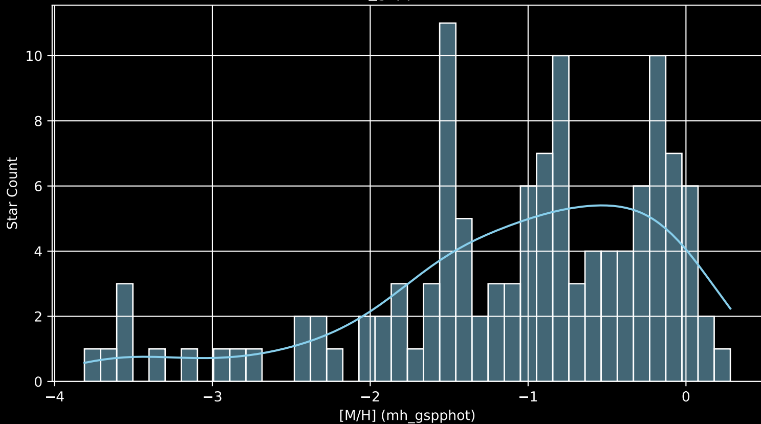
Gaia Cluster: [Pismis_1 [M/H] (mh_gspphot) (n= 120)
