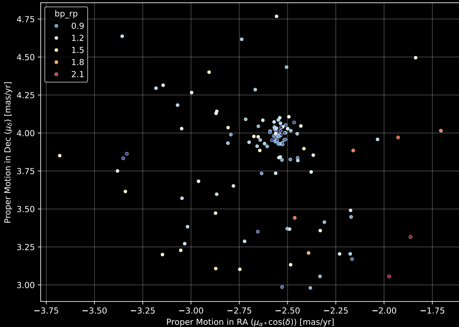
Gaia Cluster: [Pismis_1] Proper Motion Diagram (n= 120)
