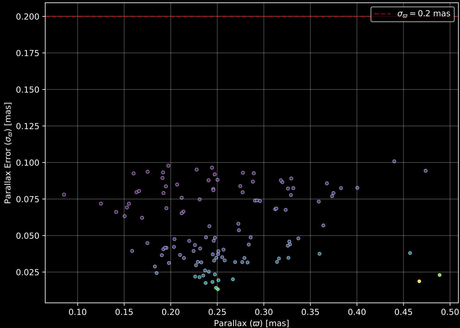
Gaia Cluster: [Pismis_2] Parallax Quality (n= 118)
