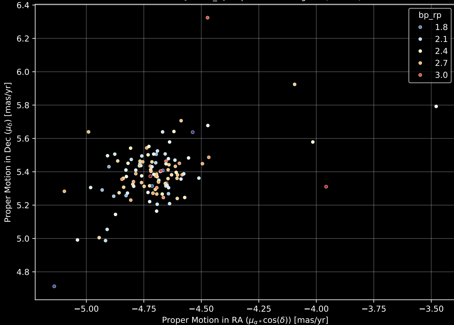
Gaia Cluster: [Pismis_2] Proper Motion Diagram (n= 118)
