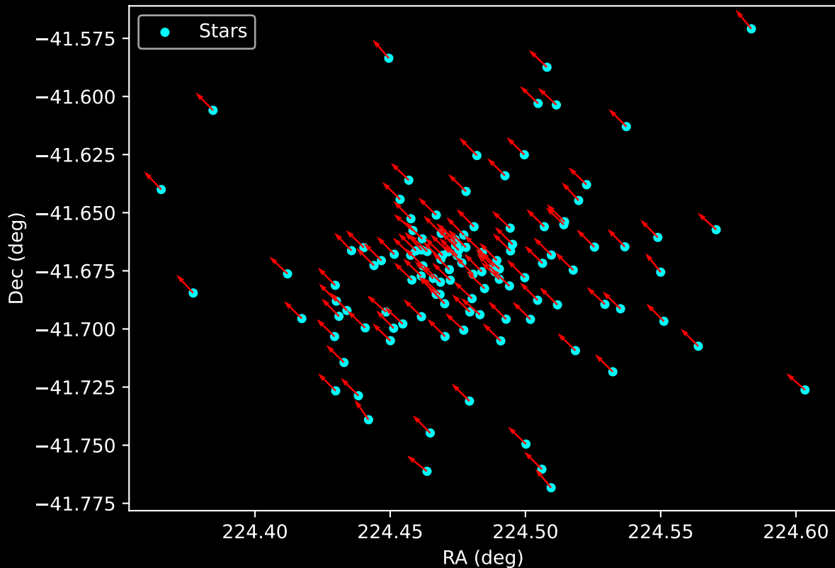
Gaia Cluster: [Pismis_2] Proper Motion Vectors for Gaia Star Field (n= 118)
