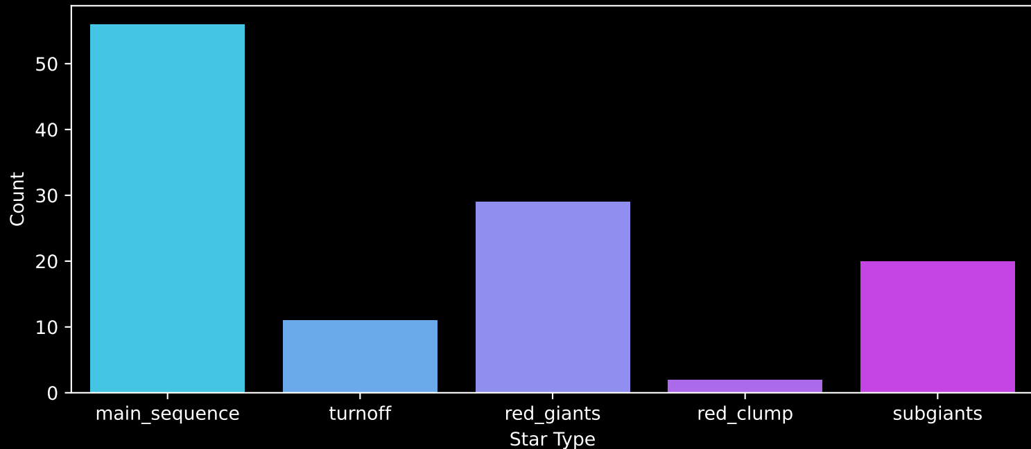
Gaia Cluster: [Pismis_2] Count plot of Star Type
