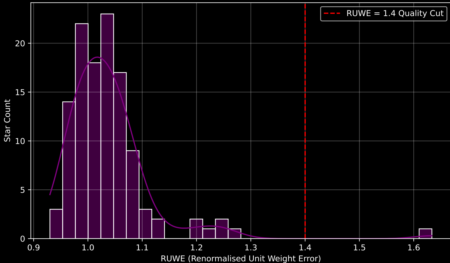
Gaia Cluster: [Pismis_2] RUWE Distribution (n= 118)
