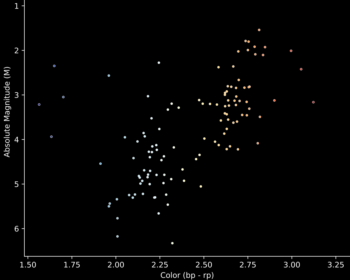
Gaia Cluster: [Pismis_2] Stars (n= 118) Hertzsprung-Russel Diagram
