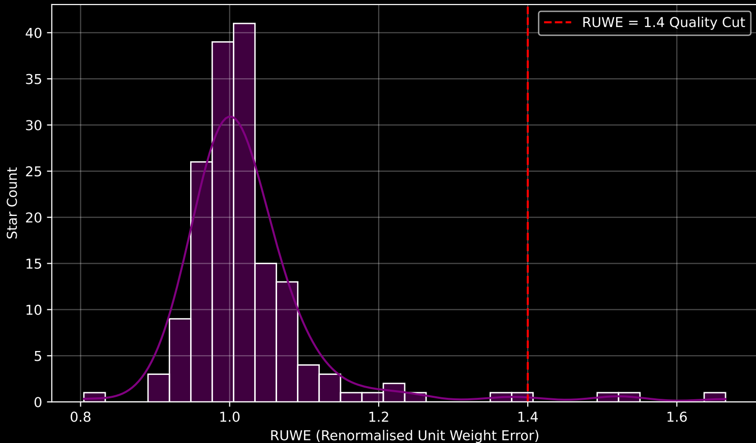
Gaia Cluster: [Pismis_21] RUWE Distribution (n= 164)
