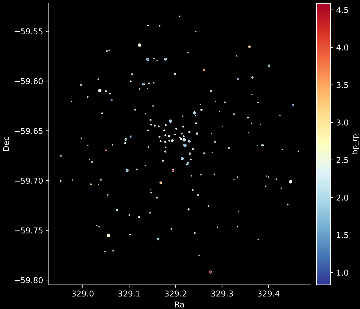
Gaia Cluster: [Pismis_21] Stars: 164
