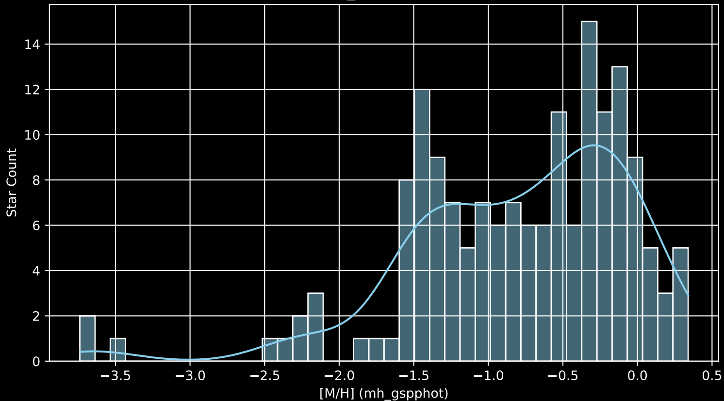
Gaia Cluster: [Pismis_21 [M/H] (mh_gspphot) (n= 164)
