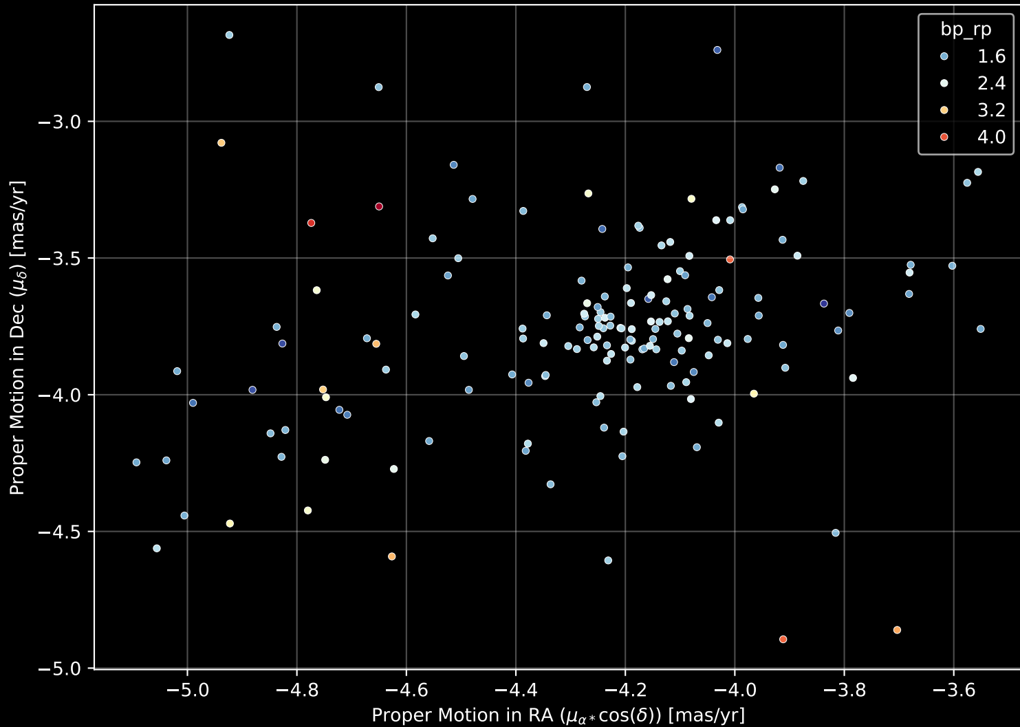
Gaia Cluster: [Pismis_21] Proper Motion Diagram (n= 164)
