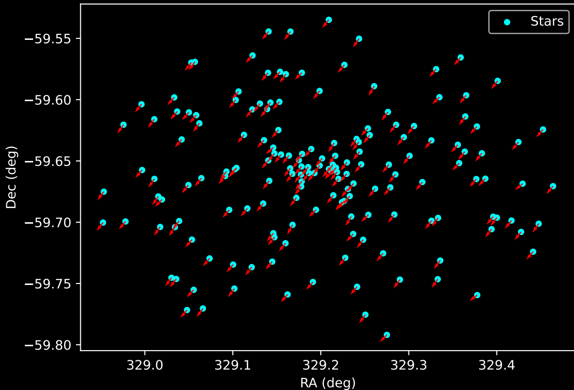
Gaia Cluster: [Pismis_21] Proper Motion Vectors for Gaia Star Field (n= 164)
