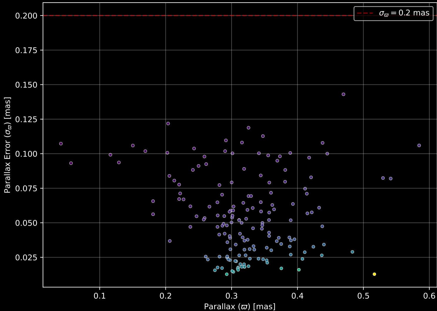
Gaia Cluster: [Pismis_21] Parallax Quality (n= 164)
