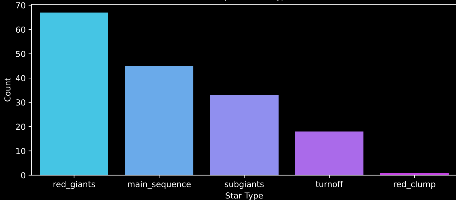
Gaia Cluster: [Pismis_21] Count plot of Star Type
