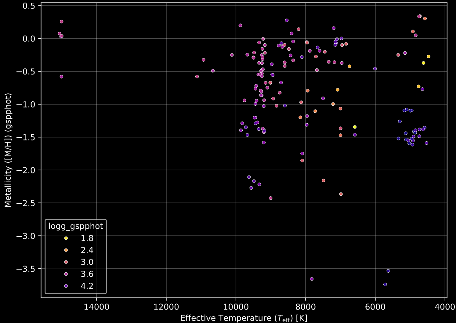
Gaia Cluster: [Pismis_21] Stellar Population Parameters (n= 164)
