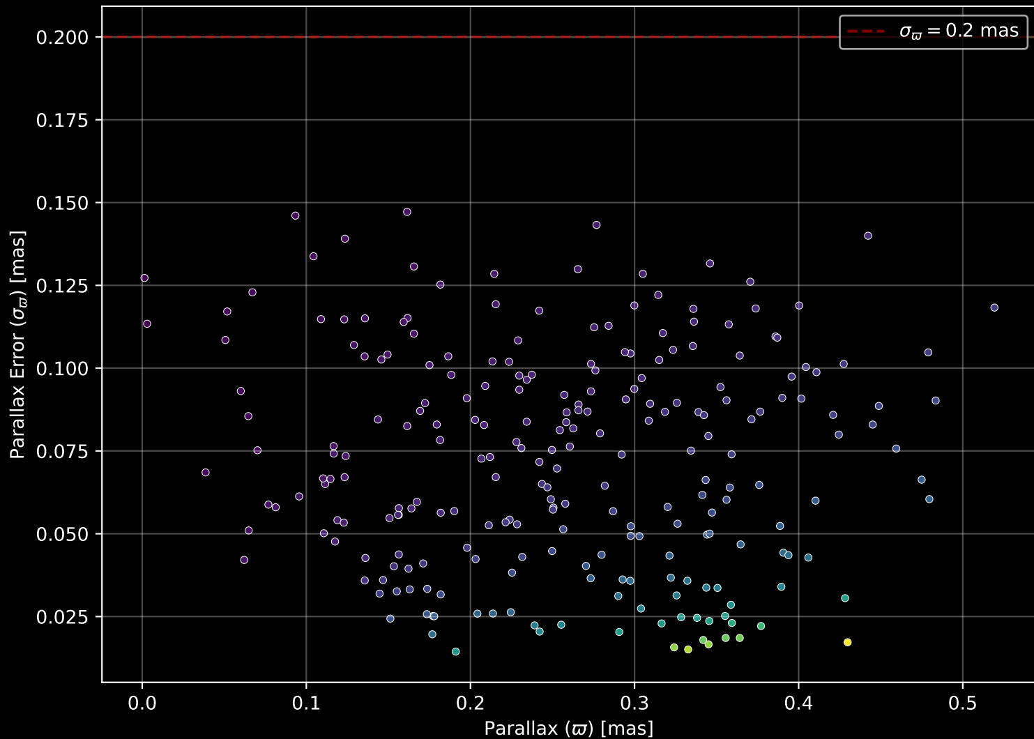
Gaia Cluster: [Pismis_22] Parallax Quality (n= 243)
