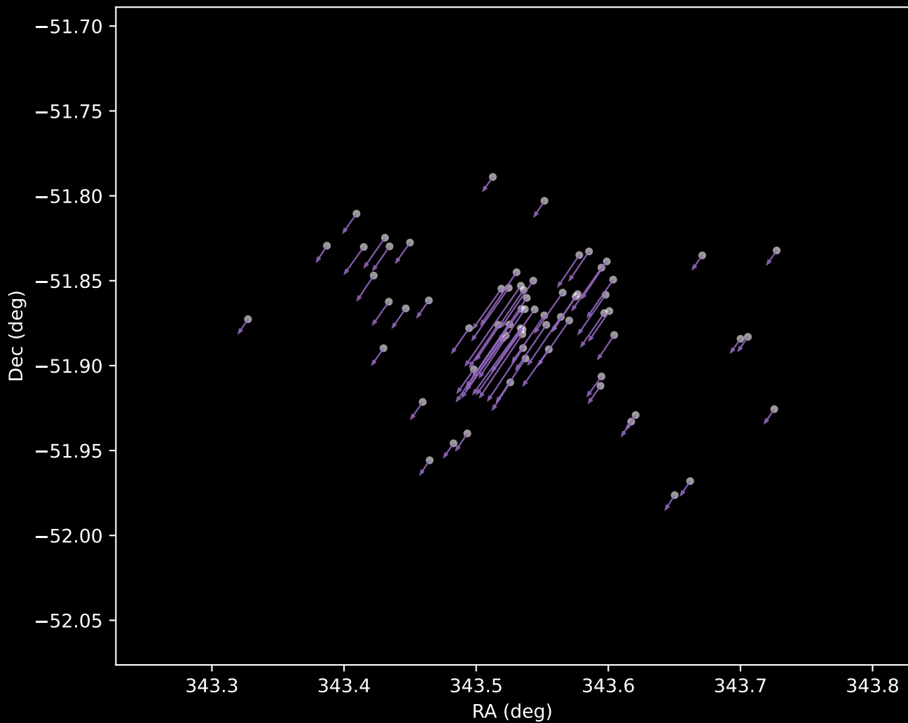
Gaia DR3 Cluster 8 Proper Motion Vectors (n=68)
