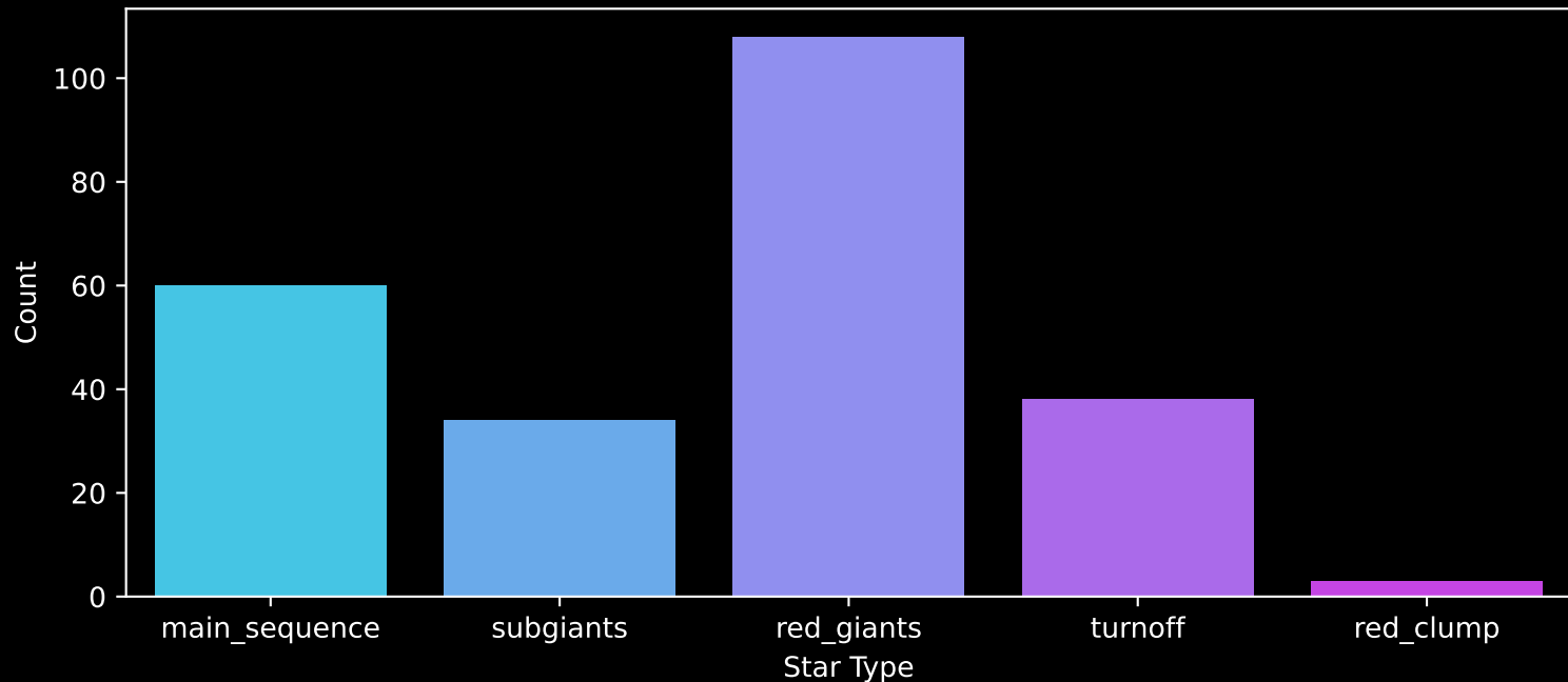
Gaia Cluster: [Pismis_22] Count plot of Star Type
