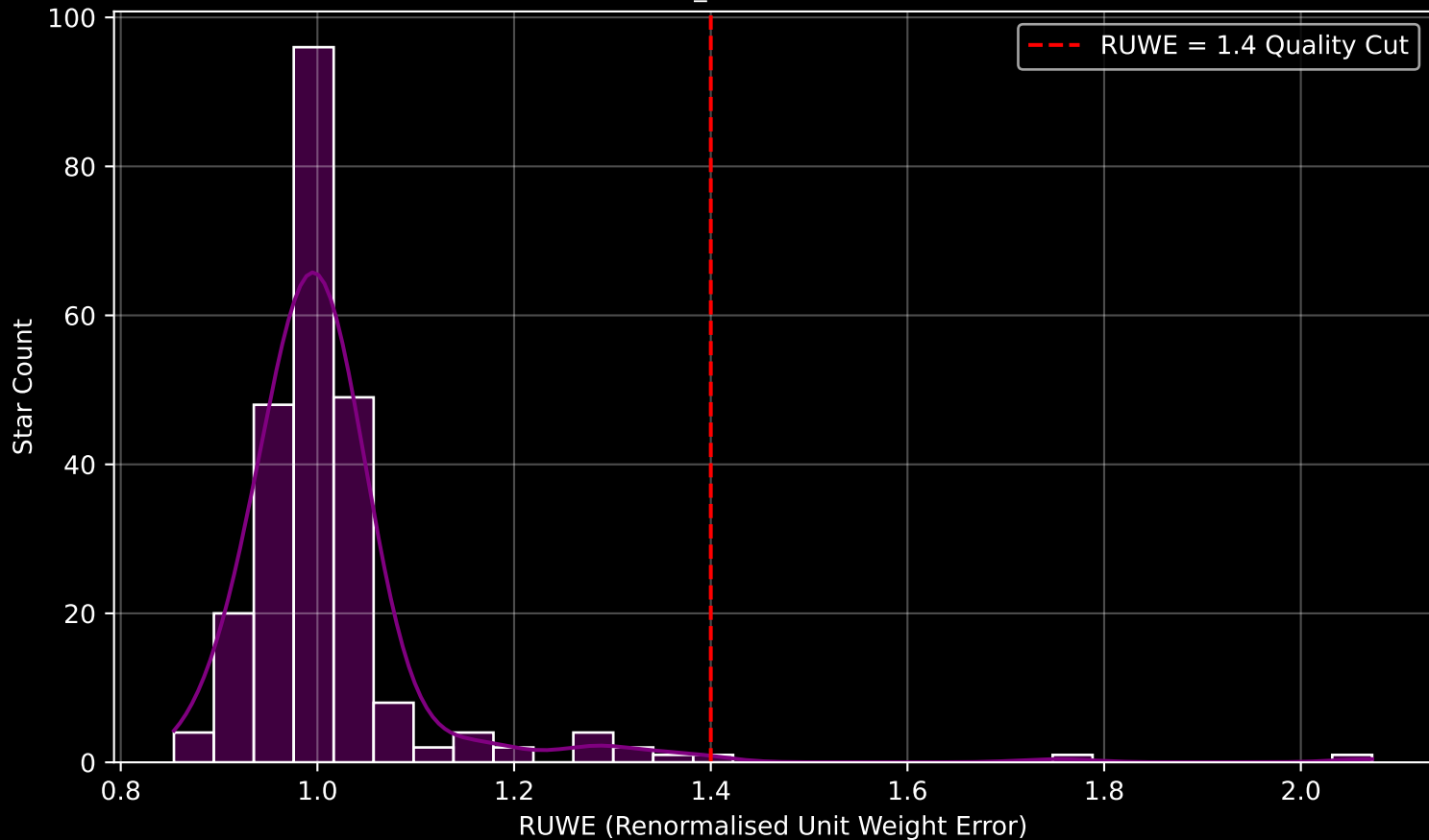
Gaia Cluster: [Pismis_22] RUWE Distribution (n= 243)
