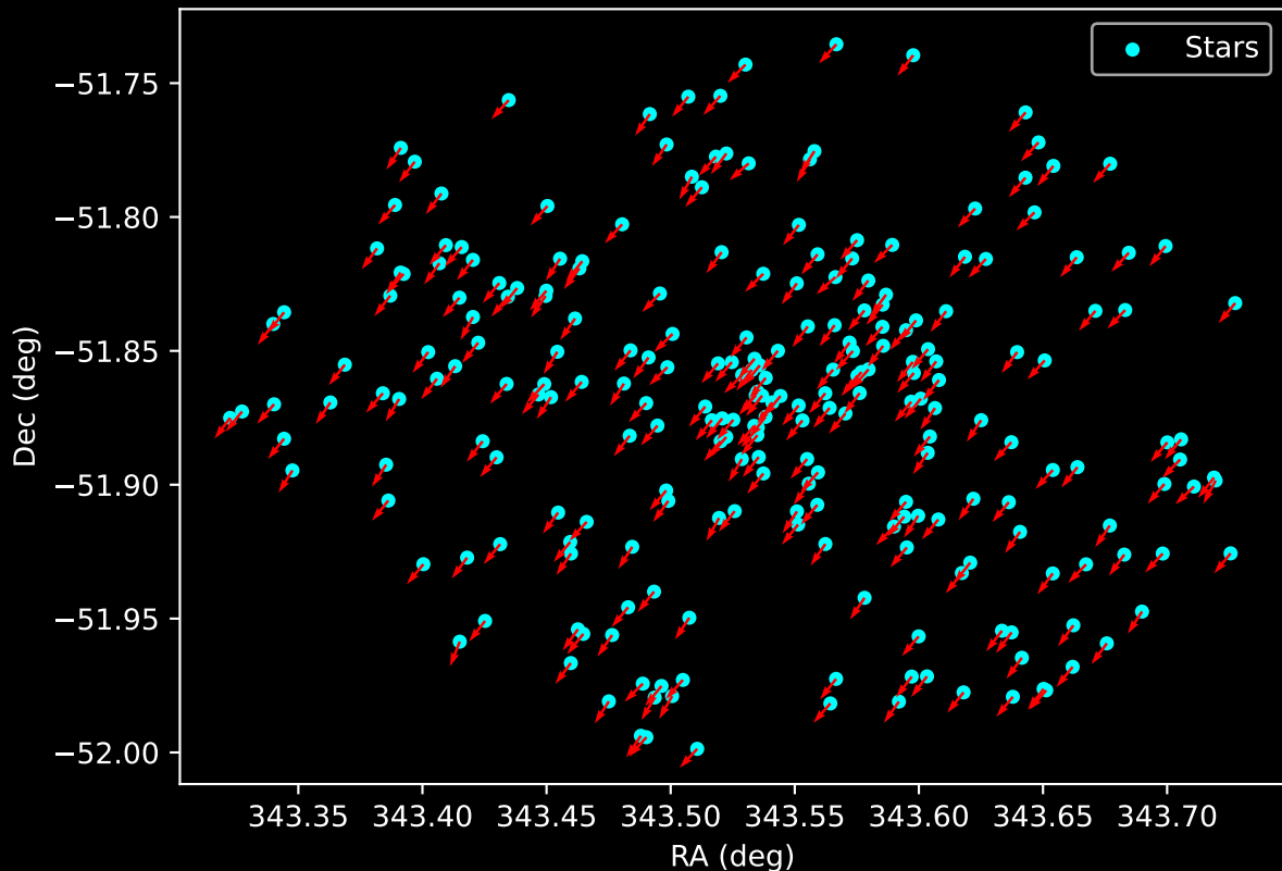
Gaia Cluster: [Pismis_22] Proper Motion Vectors for Gaia Star Field (n= 243)
