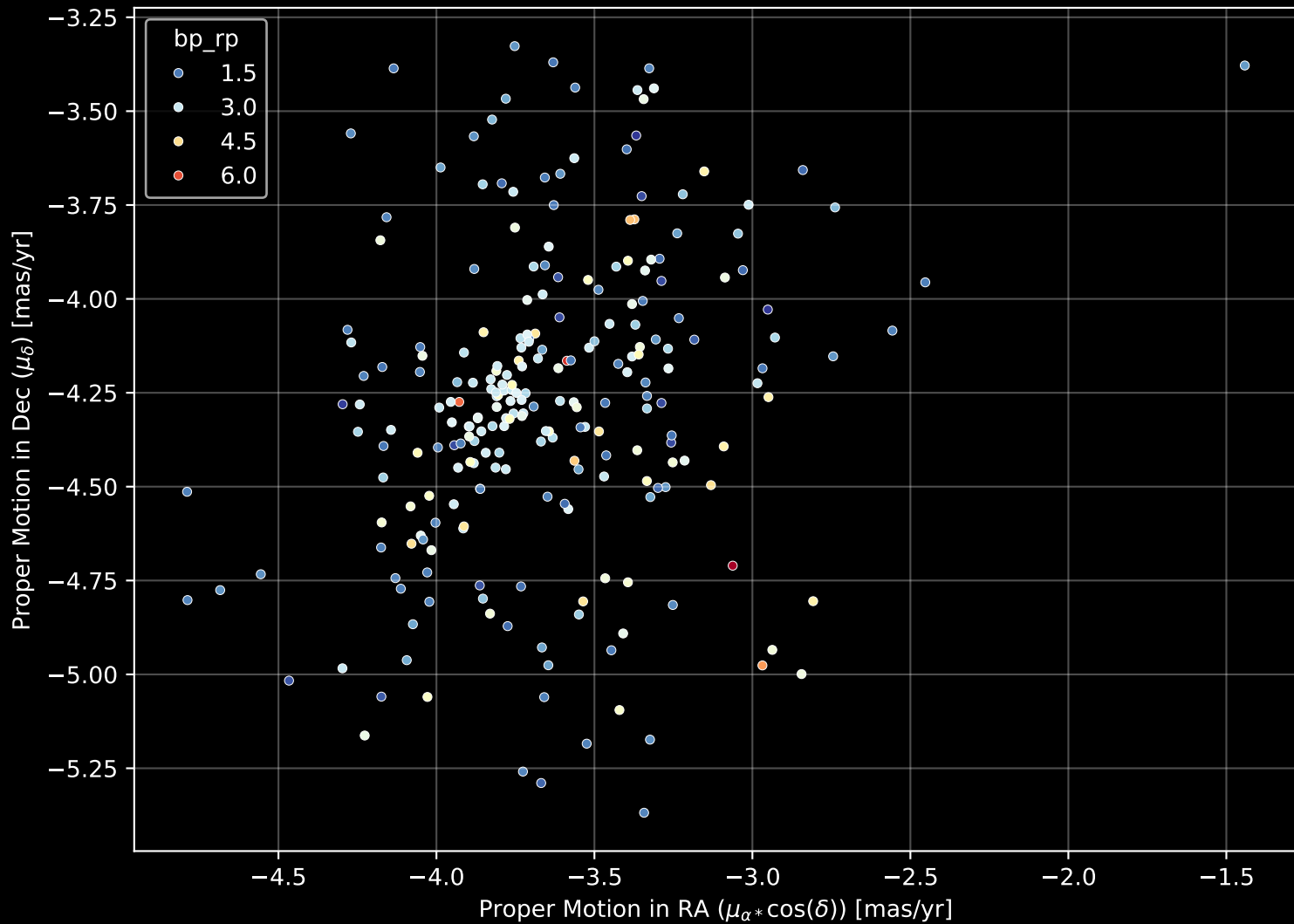
Gaia Cluster: [Pismis_22] Proper Motion Diagram (n= 243)
