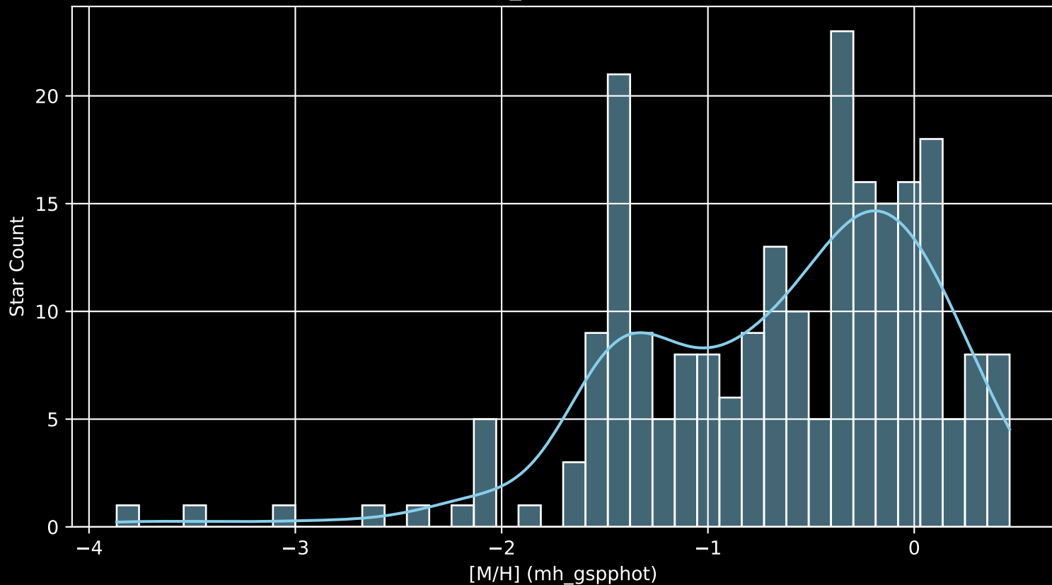
Gaia Cluster: [Pismis_22 [M/H] (mh_gspphot) (n= 227)
