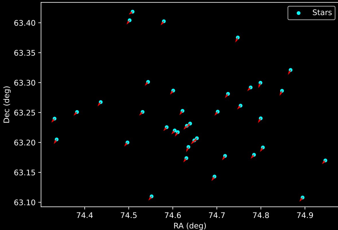
Gaia Cluster: [Pismis_Moreno_1] Proper Motion Vectors for Gaia Star Field (n= 37)
