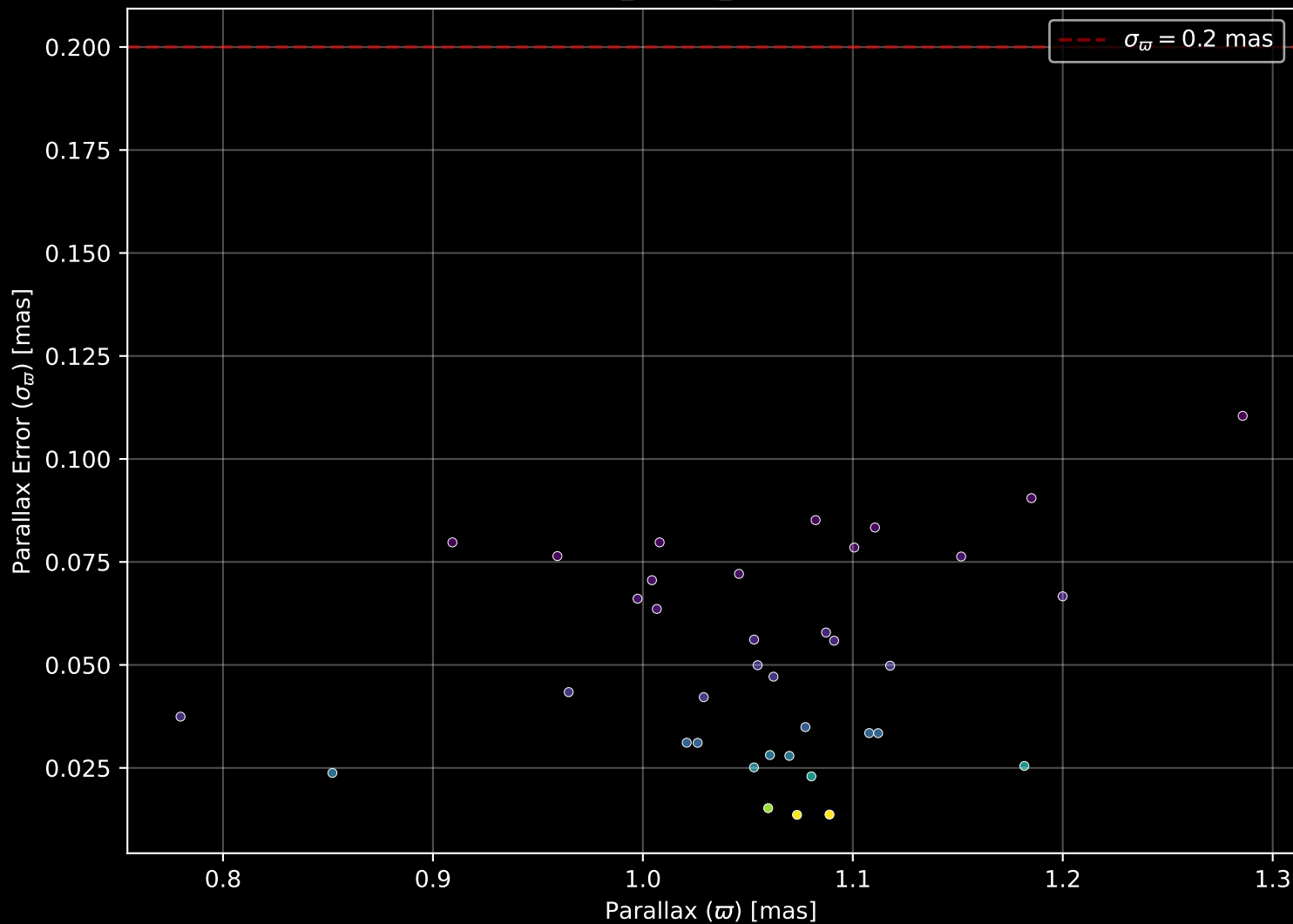
Gaia Cluster: [Pismis_Moreno_1] Parallax Quality (n= 37)
