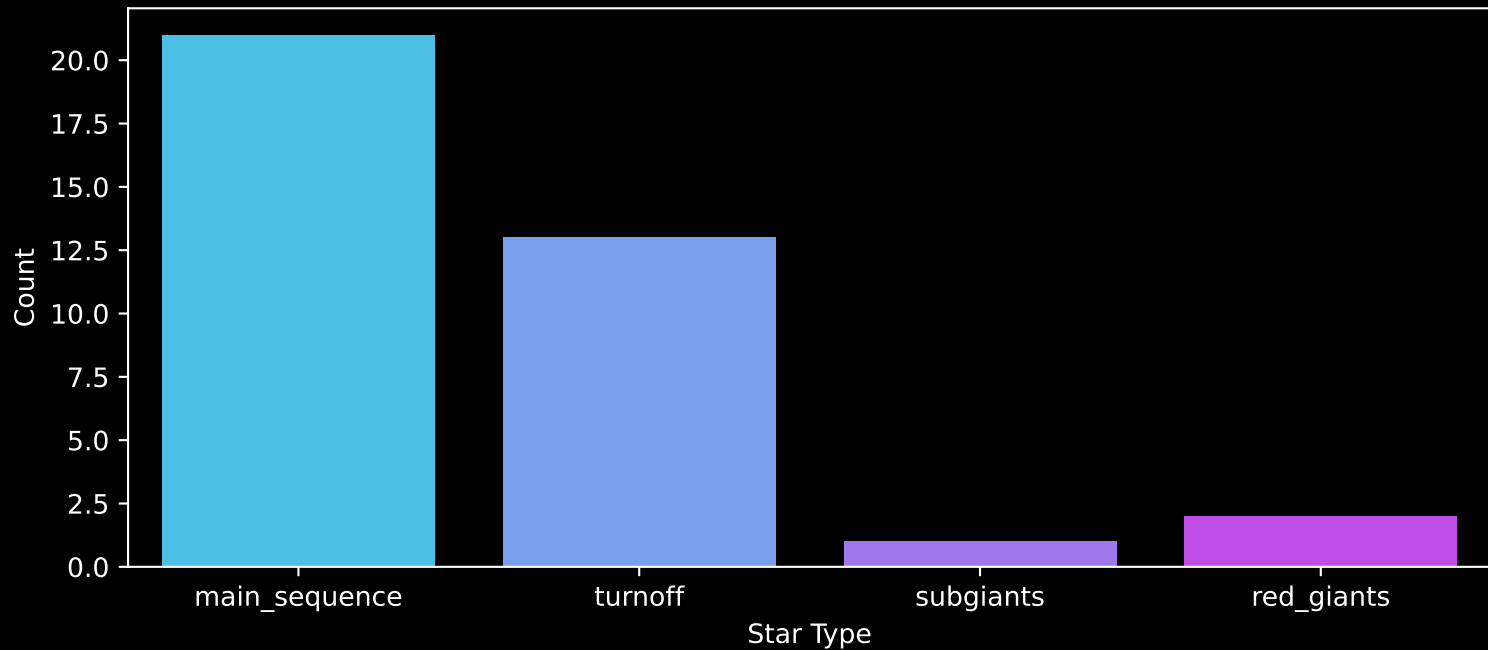
Gaia Cluster: [Pismis_Moreno_1] Count plot of Star Type
