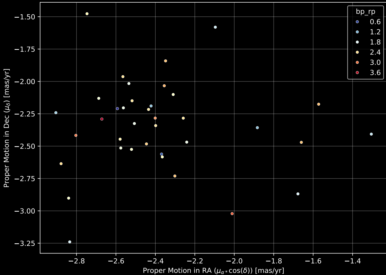
Gaia Cluster: [Pismis_Moreno_1] Proper Motion Diagram (n= 37)
