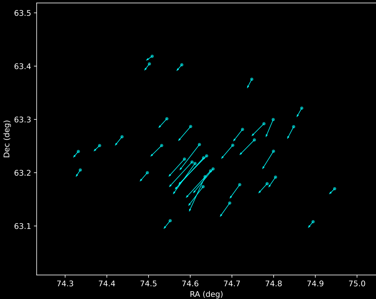
Gaia DR3 Noise Stream Proper Motion Vectors (n=37)
