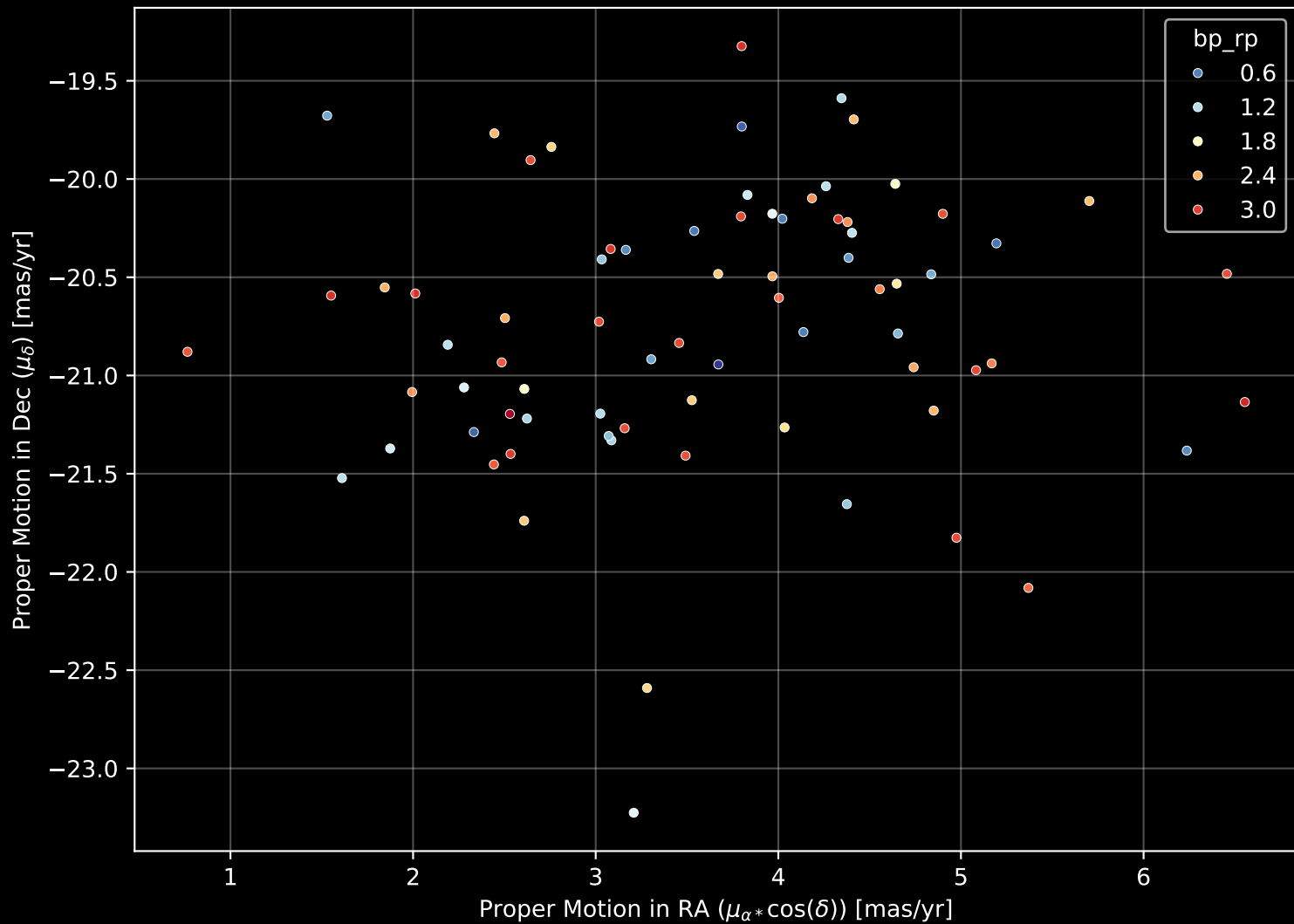
Gaia Cluster: [Platais_3] Proper Motion Diagram (n= 75)
