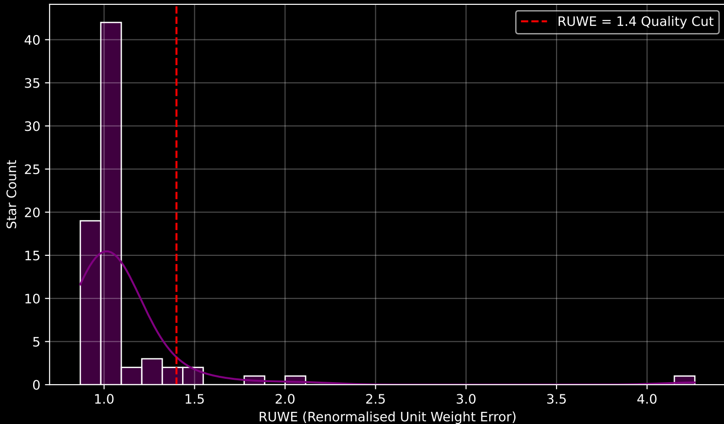
Gaia Cluster: [Platais_3] RUWE Distribution (n= 73)
