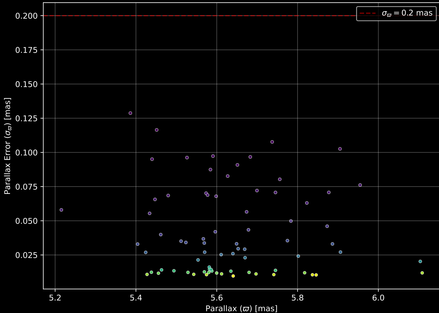
Gaia Cluster: [Platais_3] Parallax Quality (n= 75)
