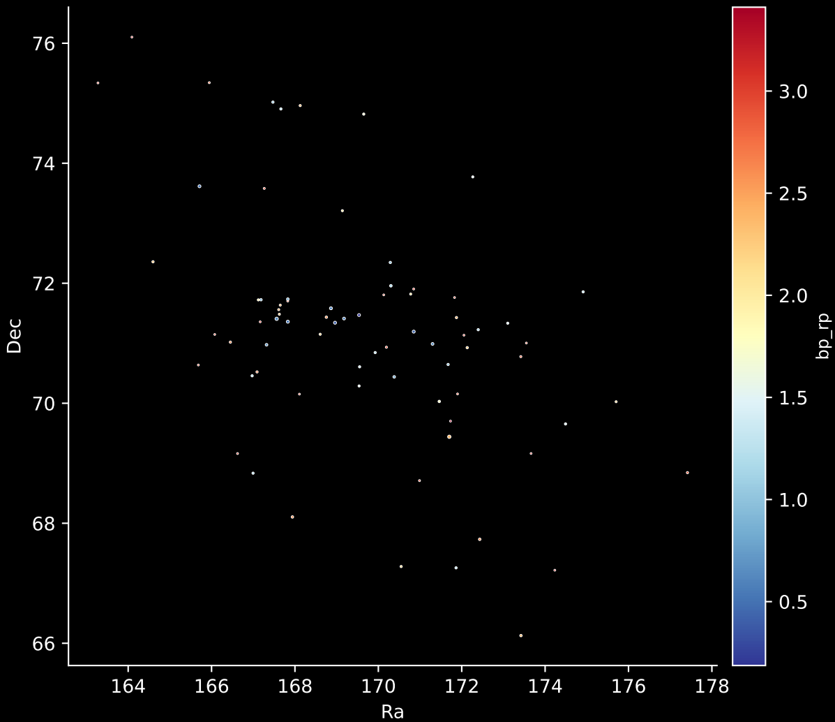
Gaia Cluster: [Platais_3] Stars: 75
