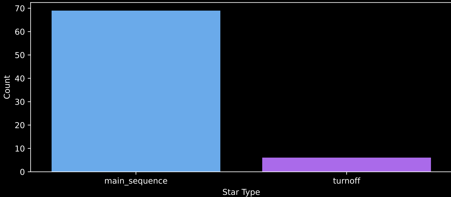
Gaia Cluster: [Platais_3] Count plot of Star Type
